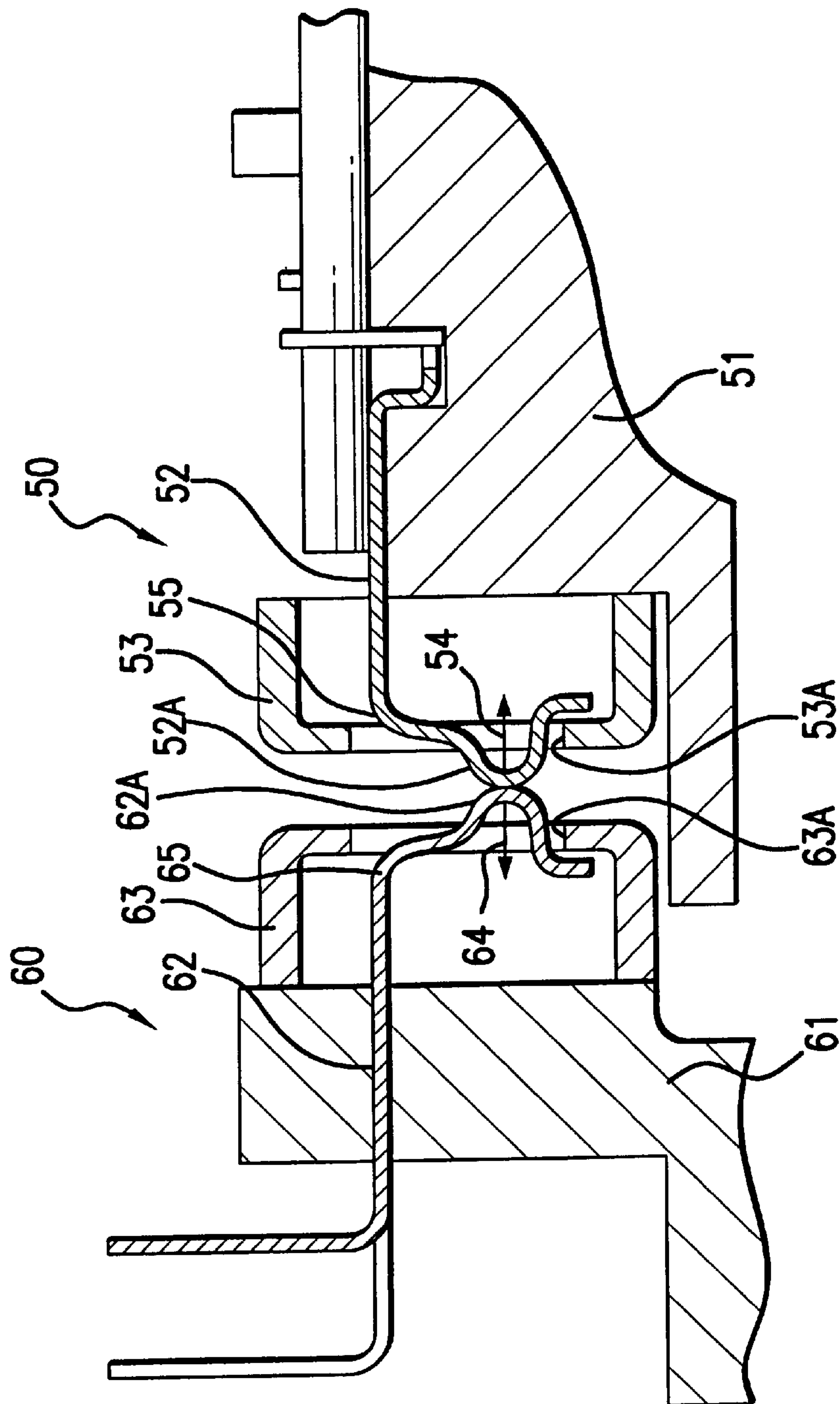
FIG. 3 (PRIOR ART)
