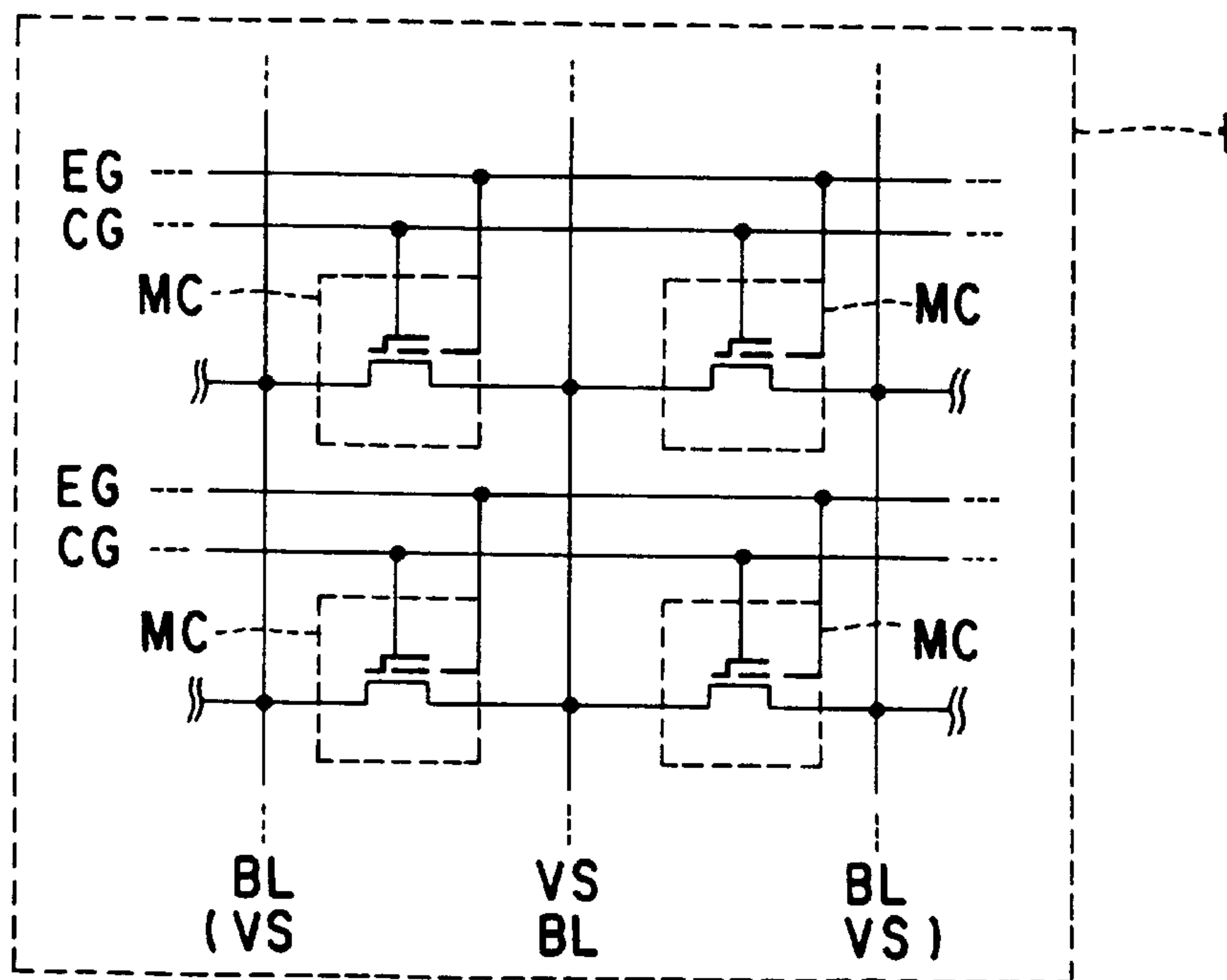
ALTERNATE GROUND ARRAY TYPE (NOR TYPE)
