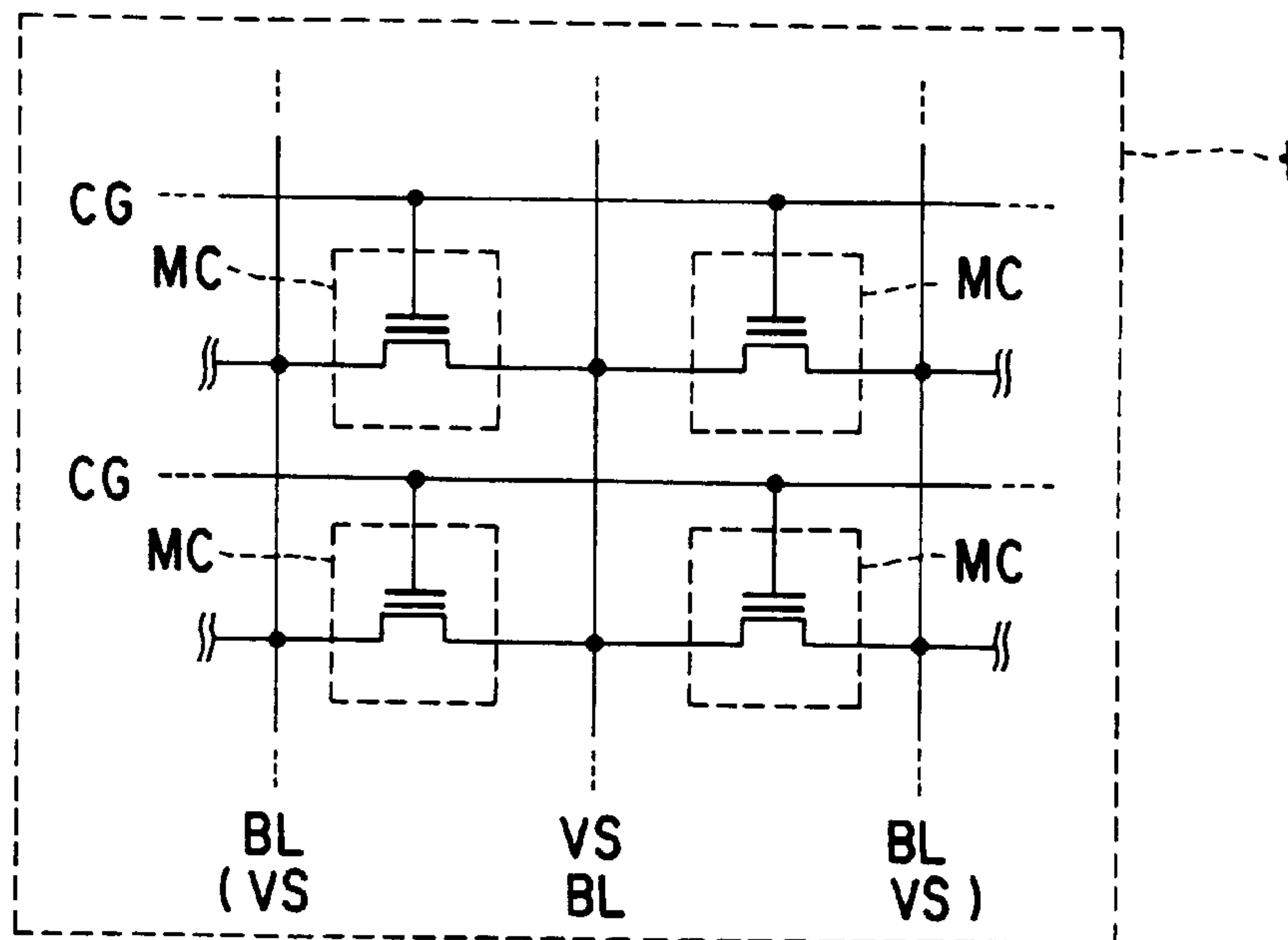
ALTERNATE GROUND ARRAY TYPE (NOR TYPE)
