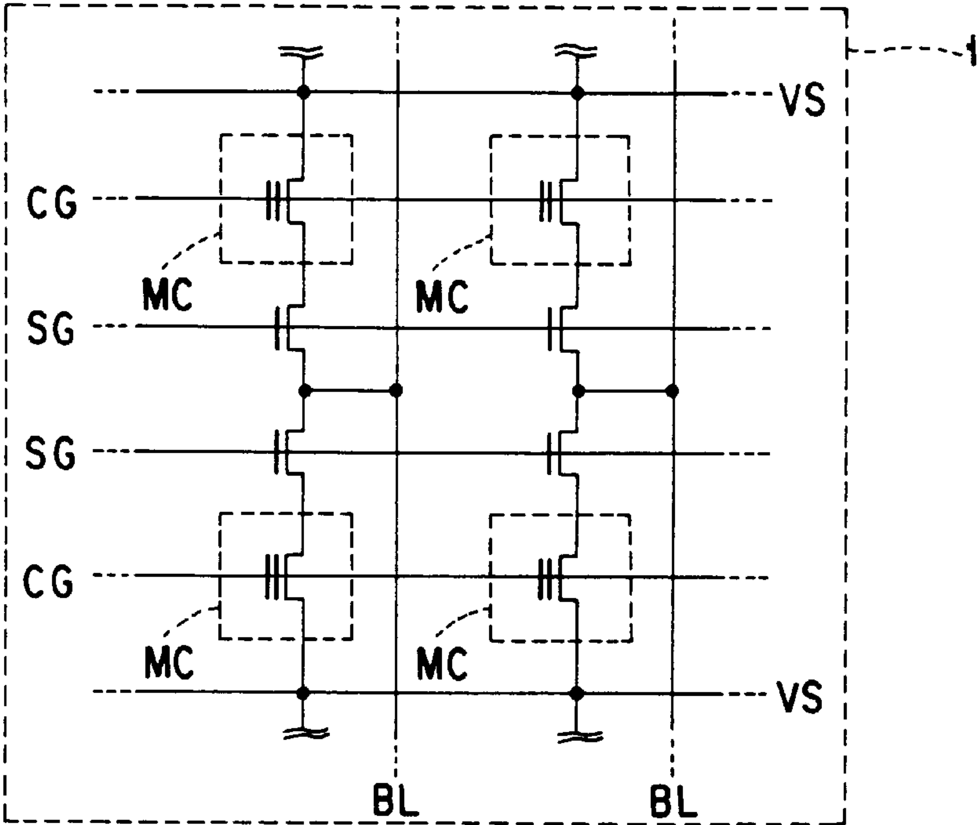
NOR TYPE
