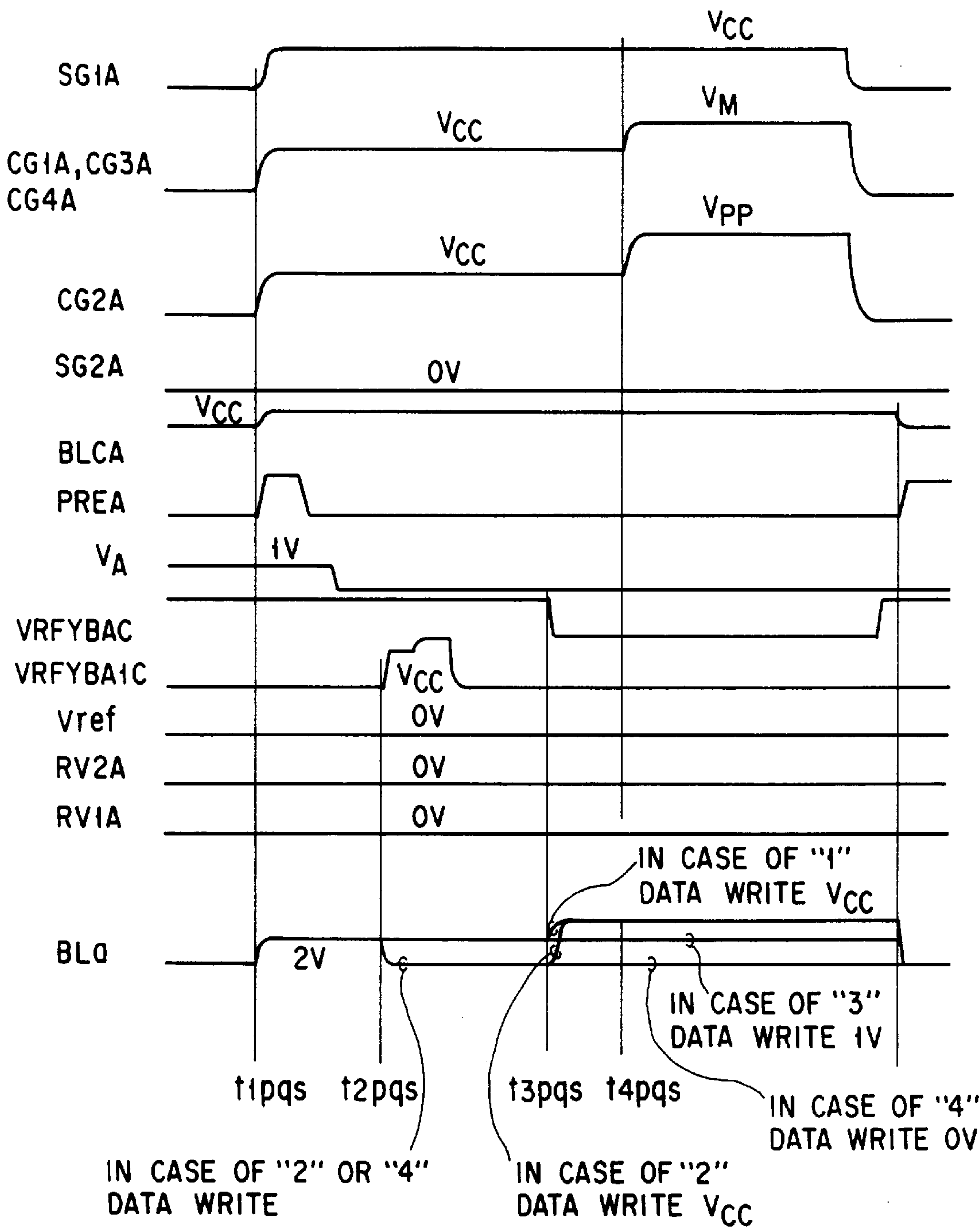
ANOTHER PROGRAMMING METHOD OF LOWER PAGE
