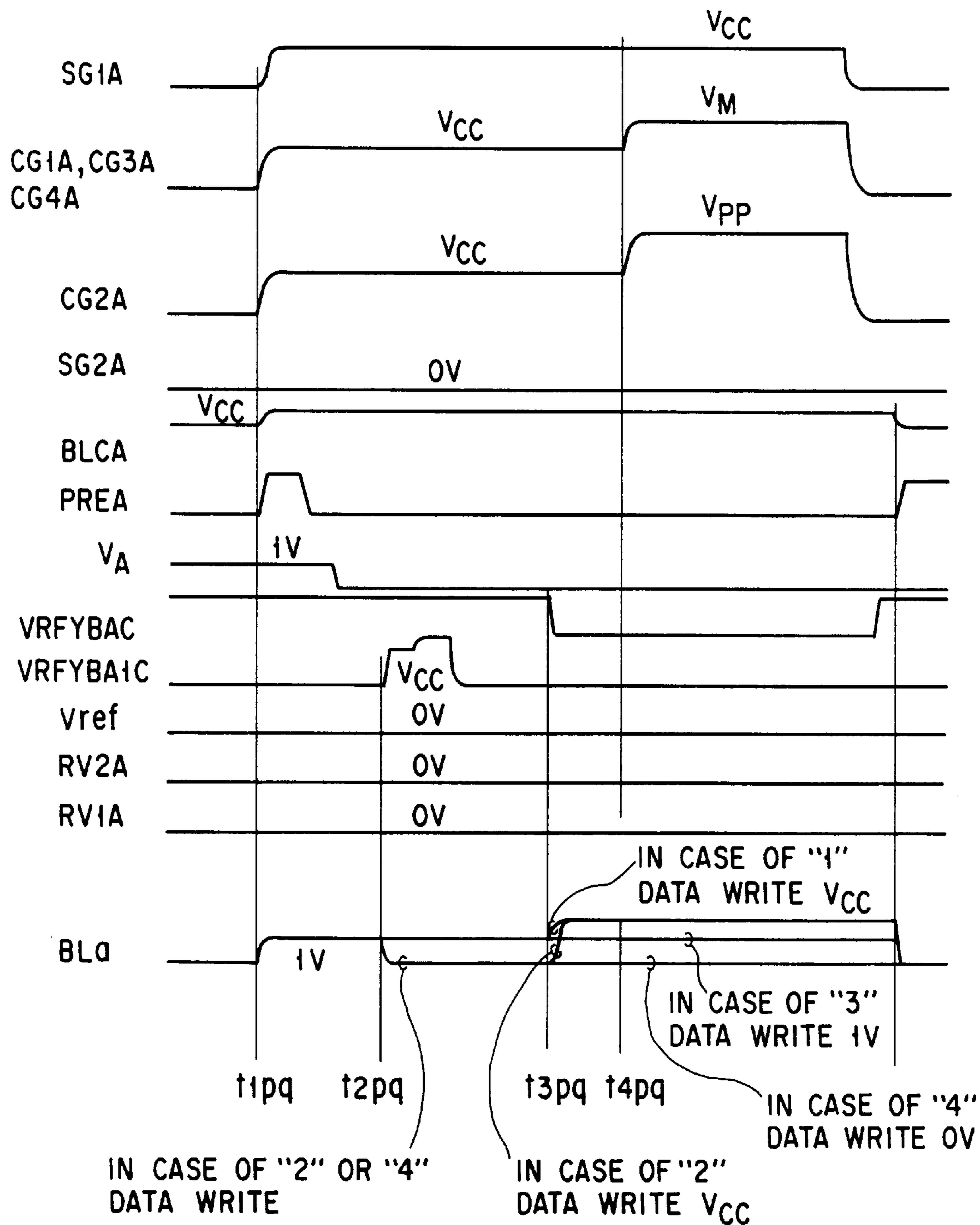
ANOTHER PROGRAMMING METHOD OF LOWER PAGE
