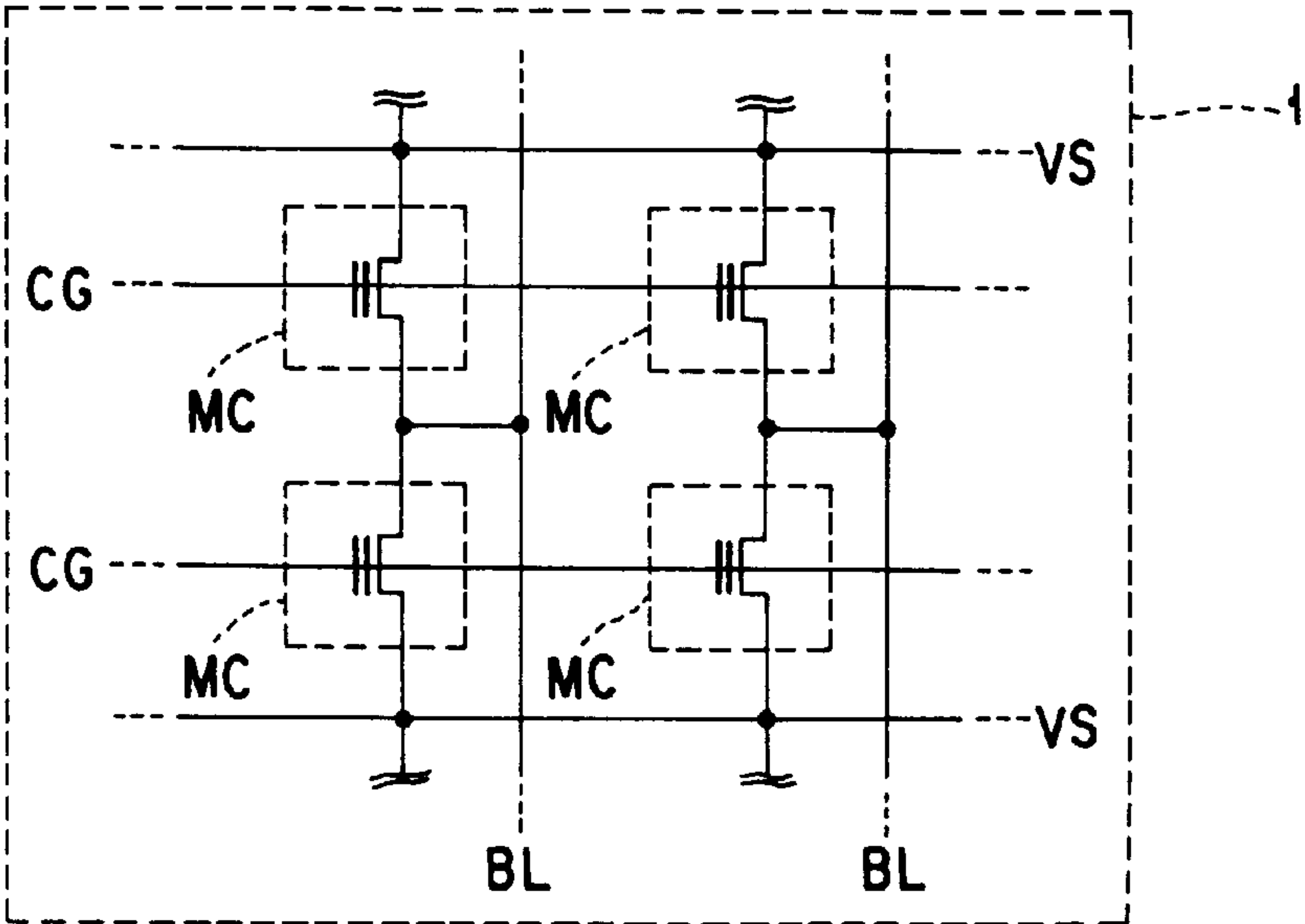
NOR TYPE
