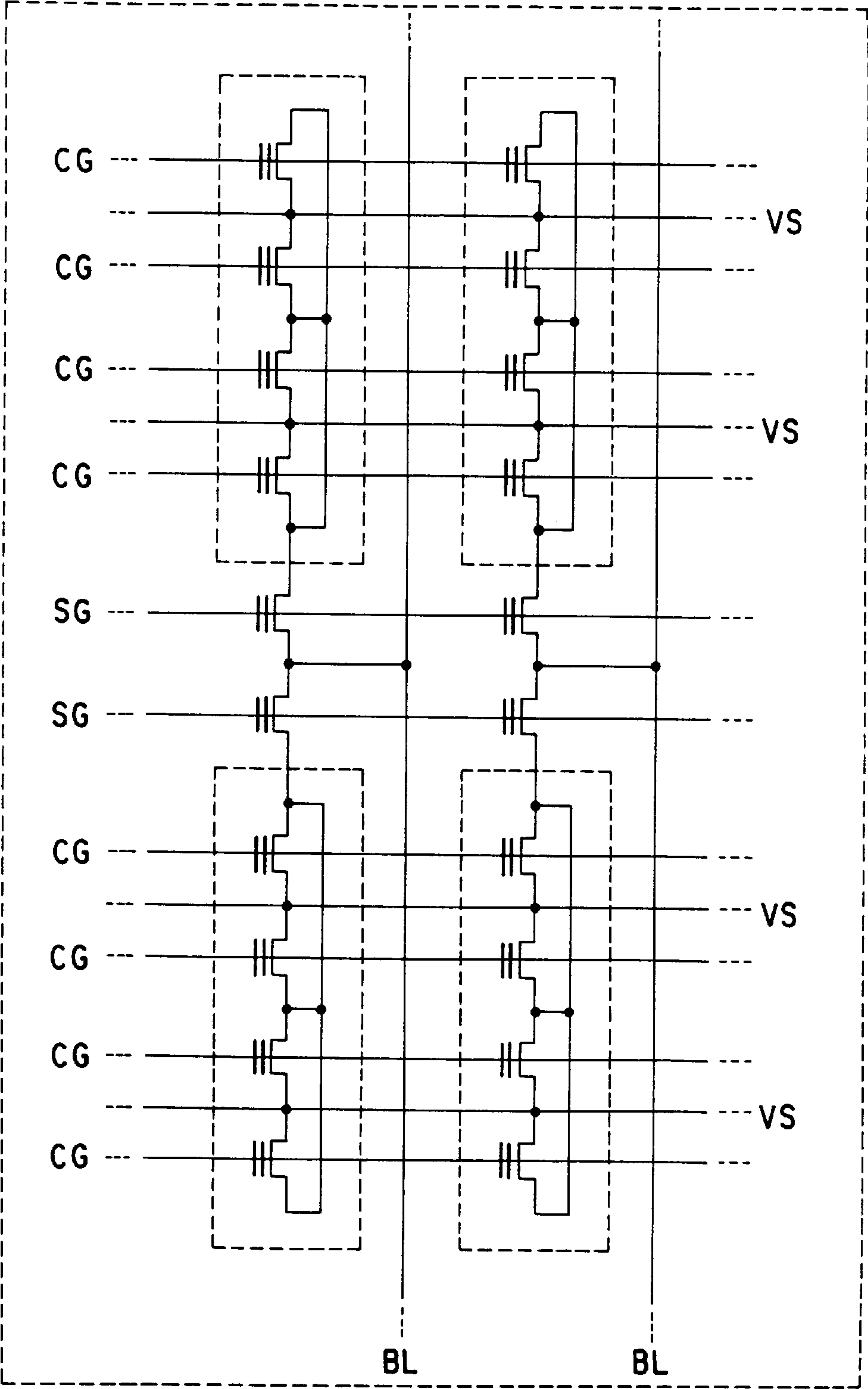
DIVIDED NOR TYPE (DINOR TYPE)
