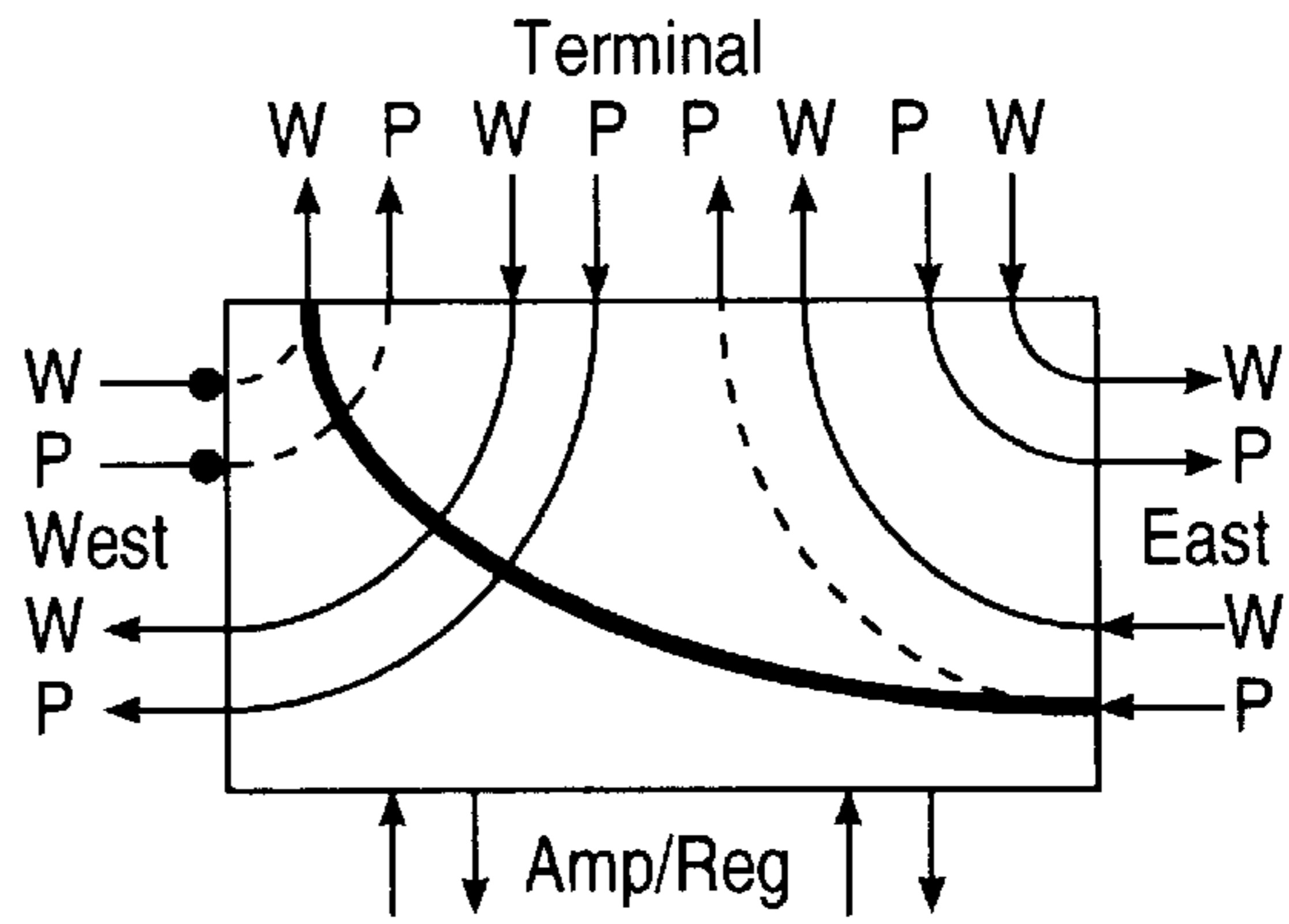
(iii) 4. Ring Switch East-In
