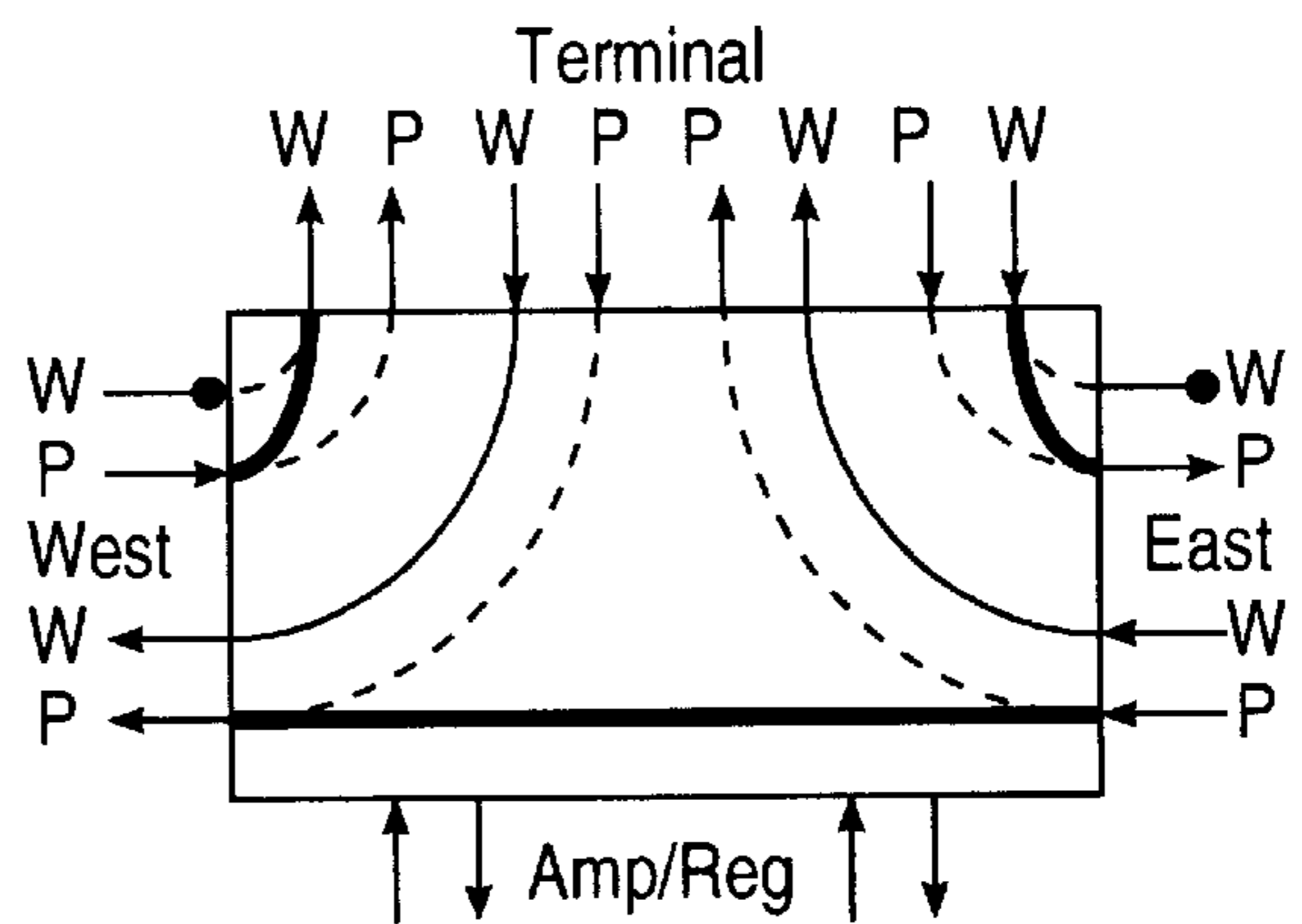
(iv) 8. P-Transit East-to-West, Span Switch West-In, East-Out
