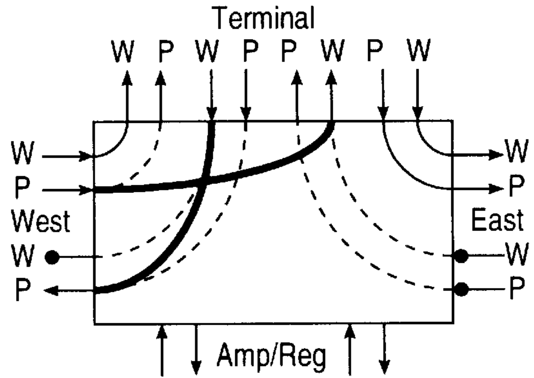
(iii) 10. Ring Switch West-In, Span Switch West-Out
