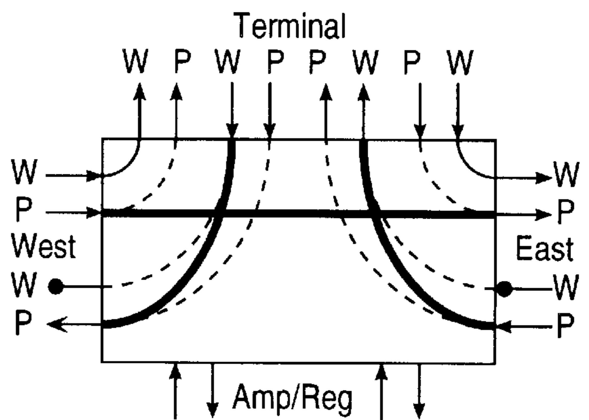
(iv) 4. P-Transit West-to-East, Span Switch West-Out, East-In
