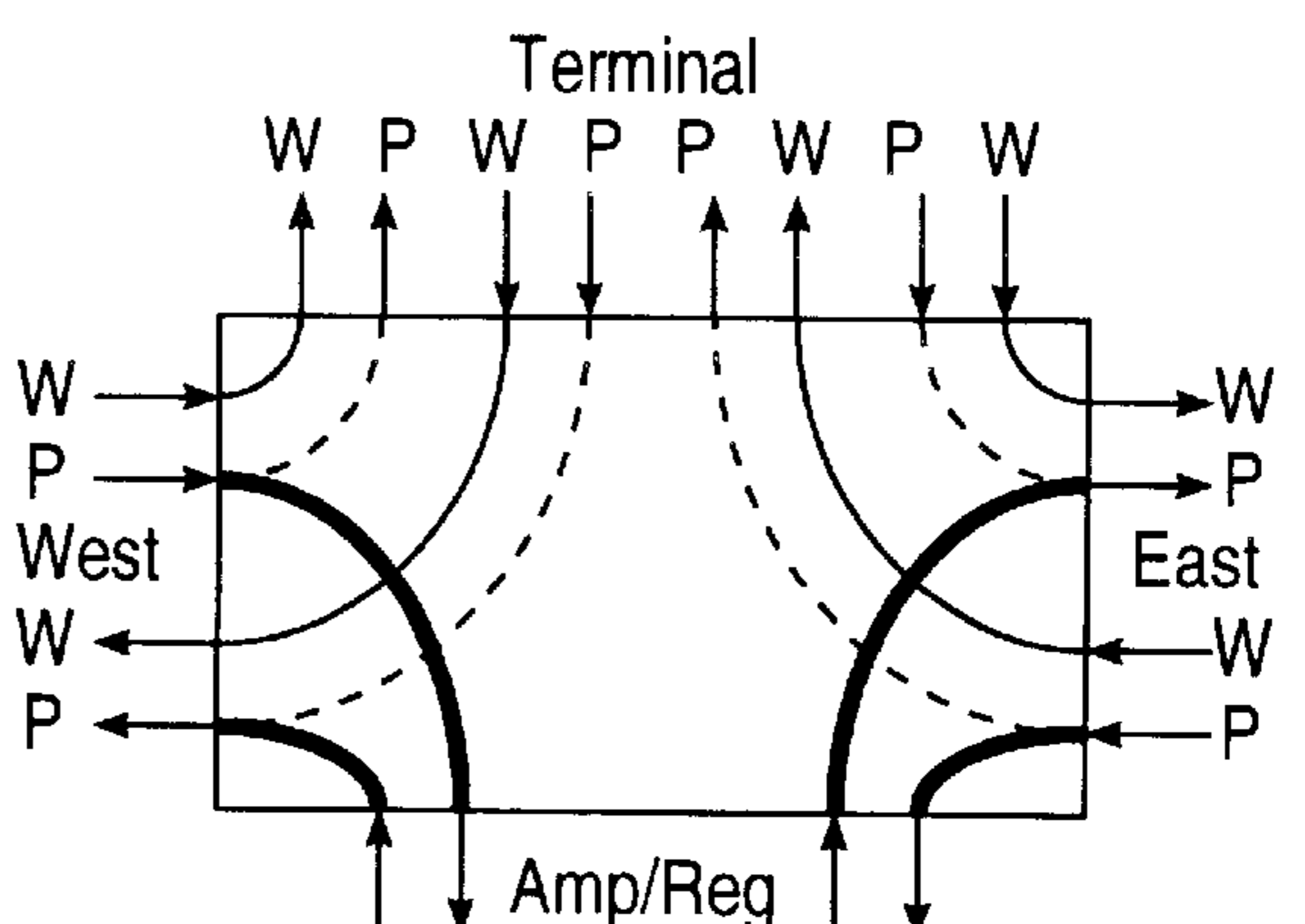
(iv) 18. P-Transit (Amp/Regen) West-to-East and East-to-West
