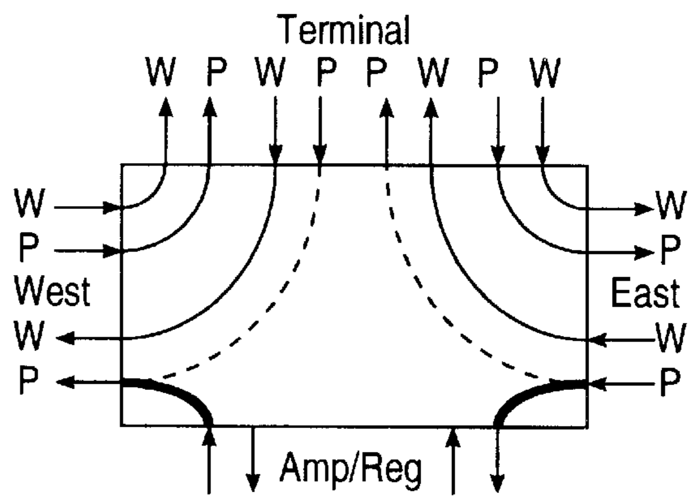
(iv) 14. P-Transit (Amp/Regen) East-to-West
