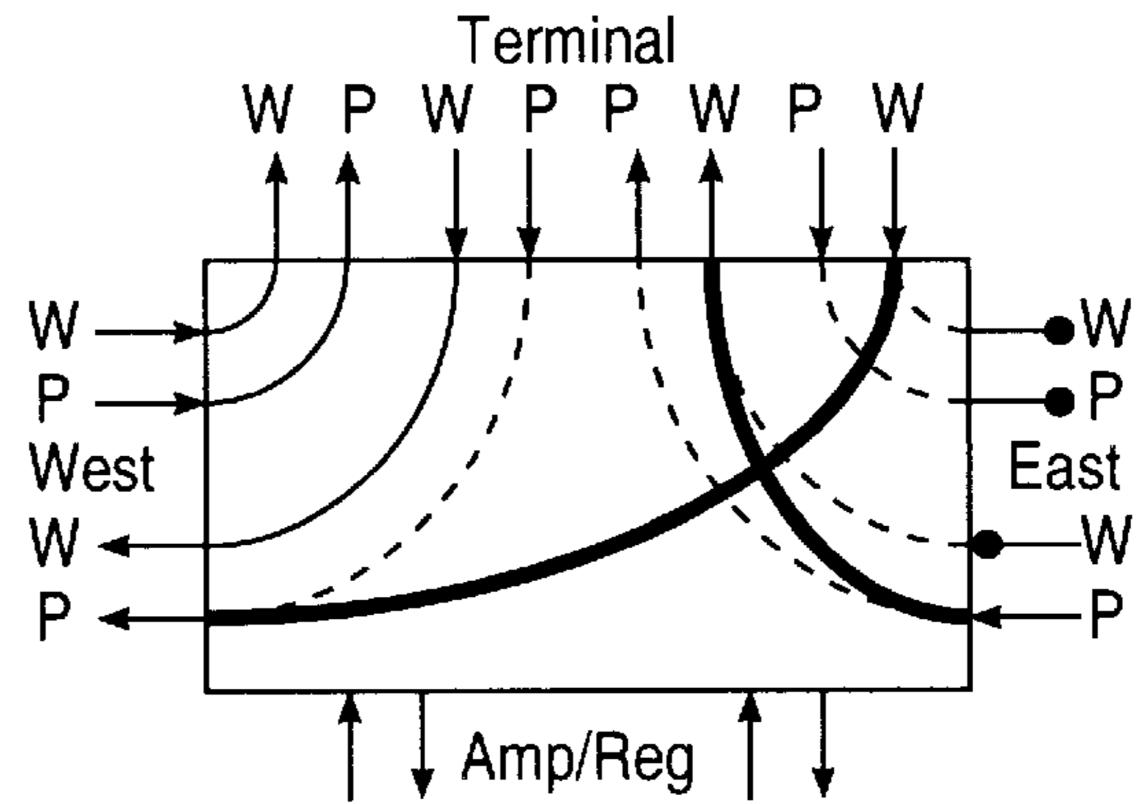
(iii) 12. Ring Switch West-Out, Span Switch East-In
