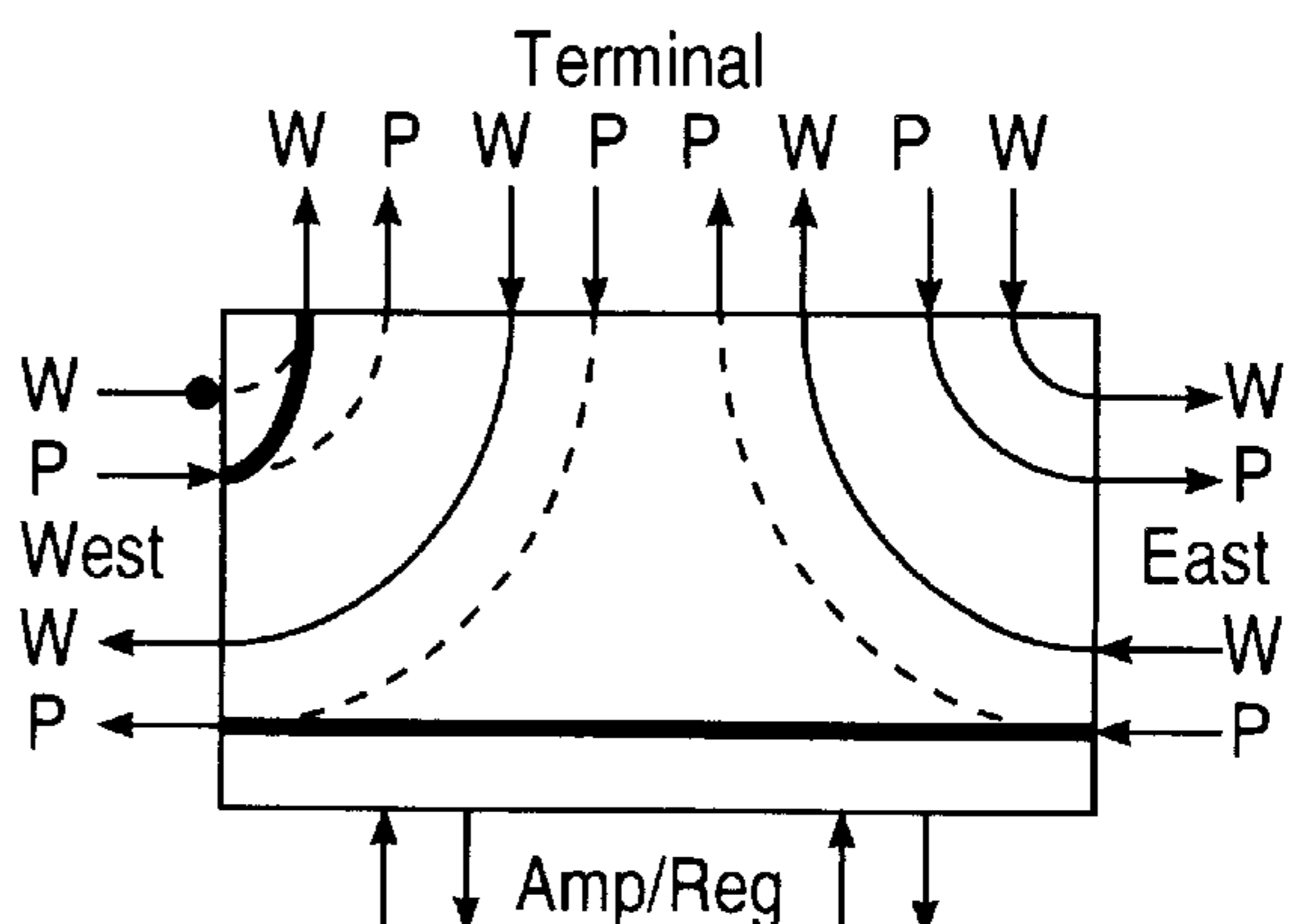
(iv) 6. P-Transit East-to-West, Span Switch West-In
