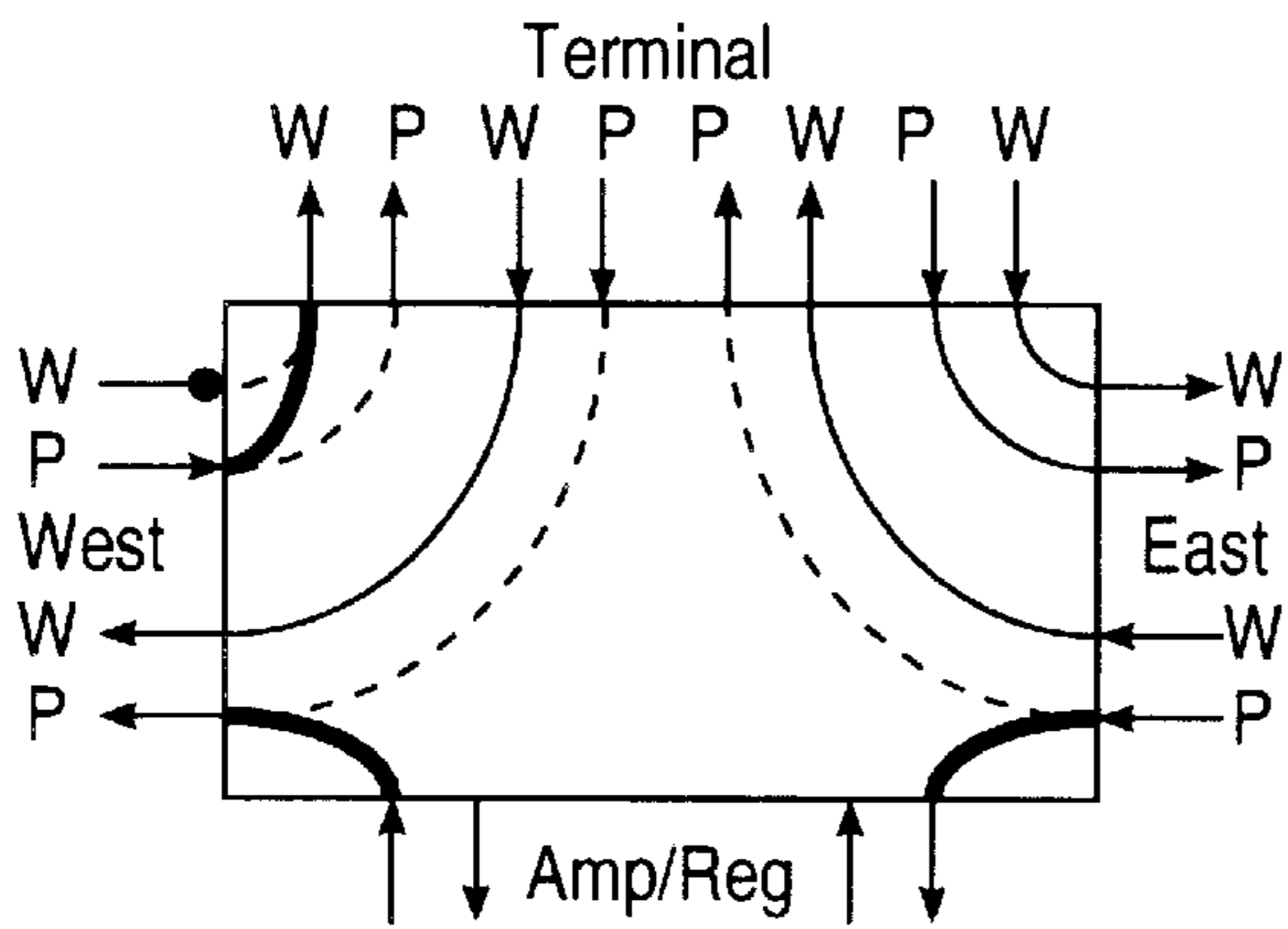
(iv) 15. P-Transit (Amp/Regen) East-to-West. Span Switch West-In
