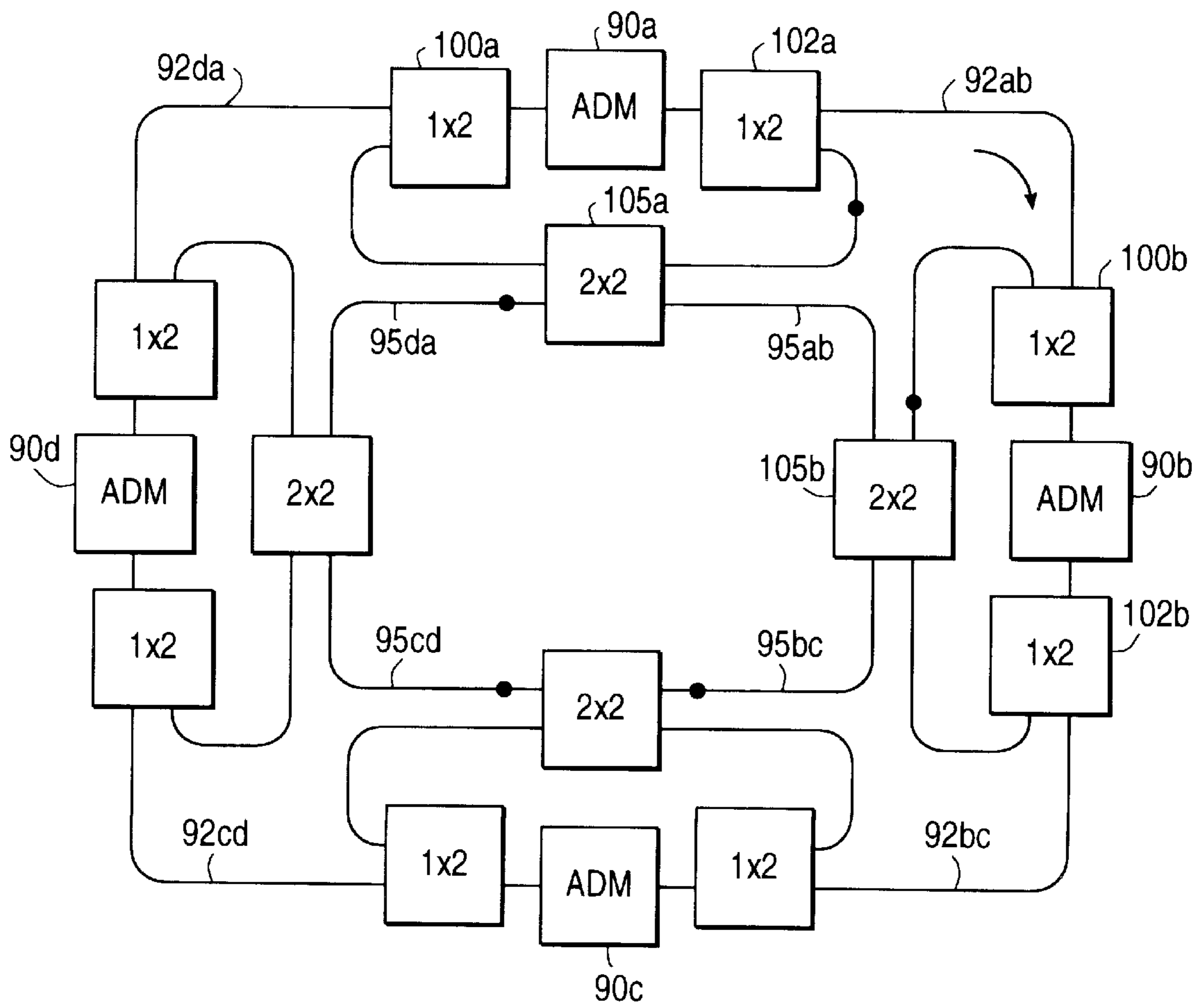
FIG. 5 (PRIOR ART)
