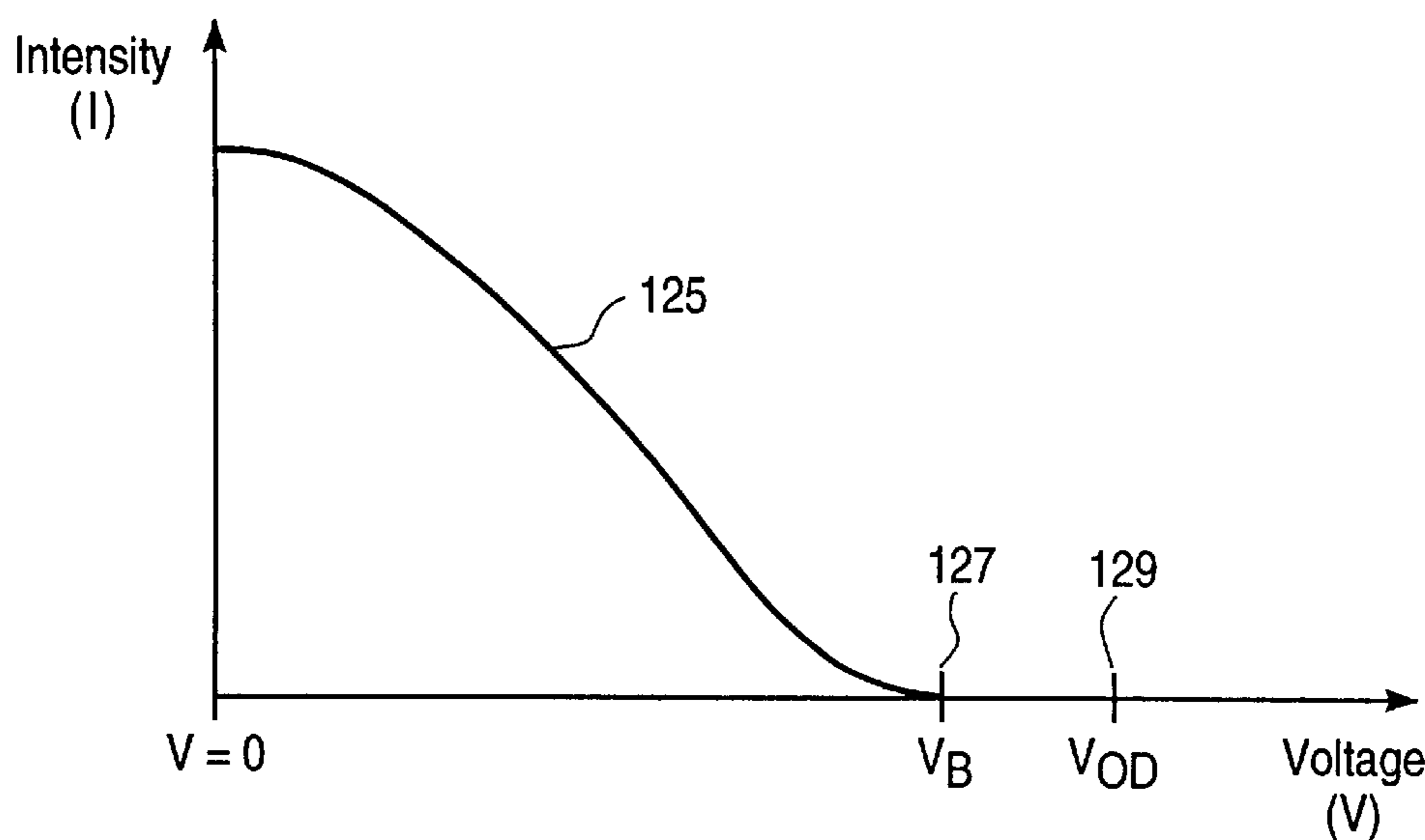
Electro-optic Curve for Normally White Liquid Crystal
