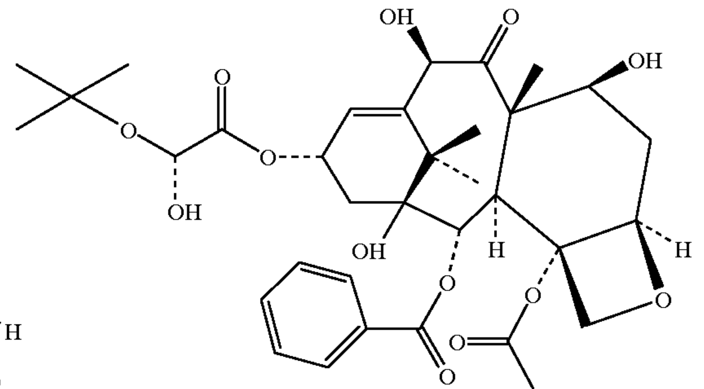
Taxotere
