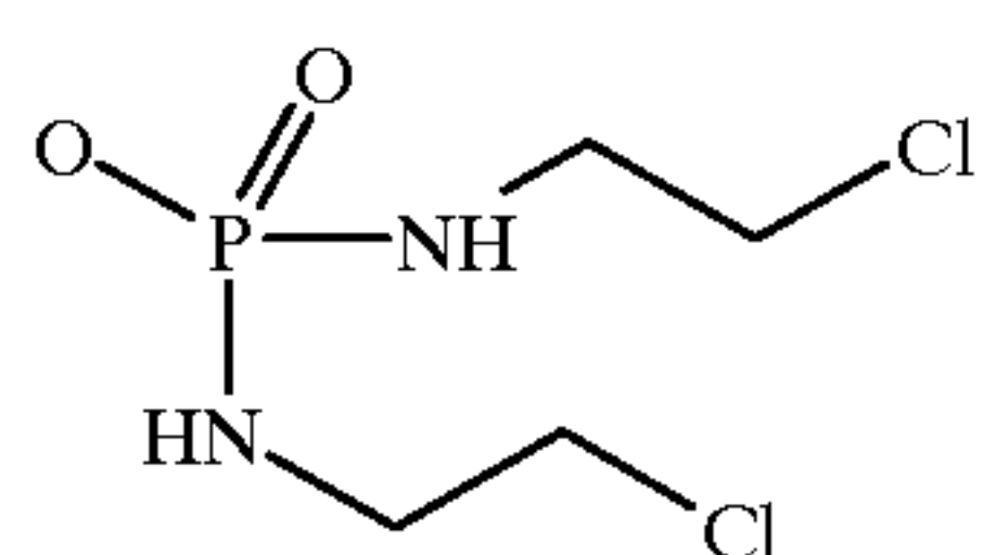
Isophosphoramidate Mustard
