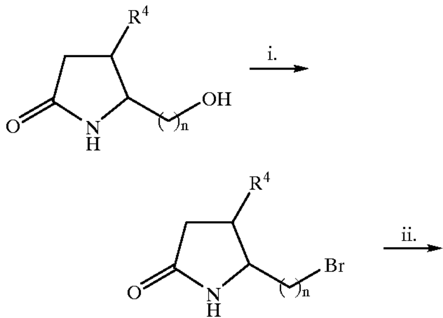
SCHEME III
