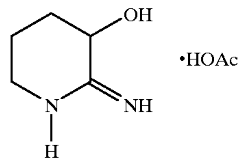
2-Imino-3-hydroxypiperidine acetate
