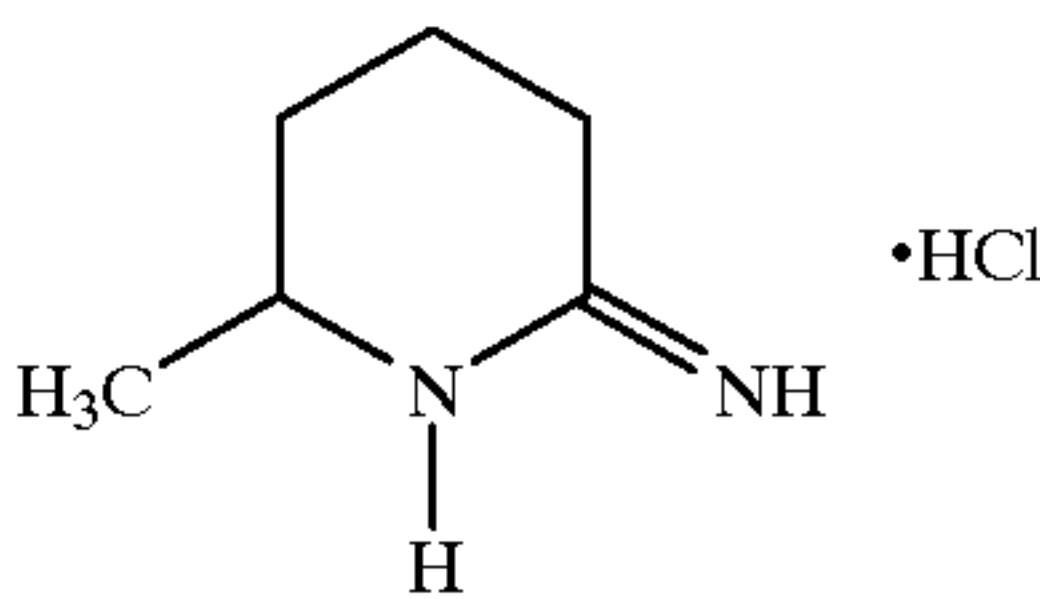
2-Imino-6-methylpiperidine hydrochloride
