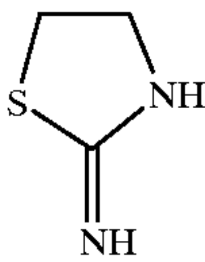
2-Iminothiazolidine hydrochloride; Aldrich Chemical Co.
