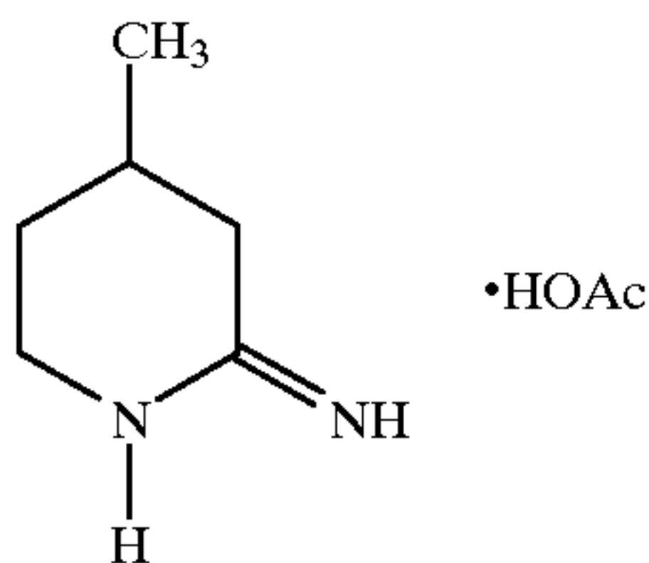
2-Imino-4-methylpiperidine acetate
