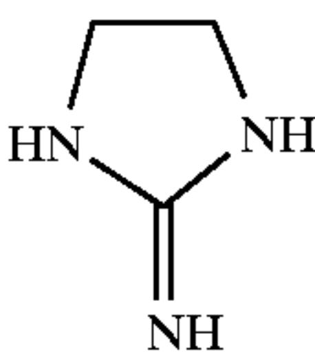
2-Iminoimidazolidine D. Stefanye and W. C. Howard, J. Amer. Chem. Soc., 77, 761–762 (1955).
