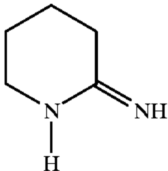
2-Iminopiperidine hydrochloride; Aldrich Chemical Co.
