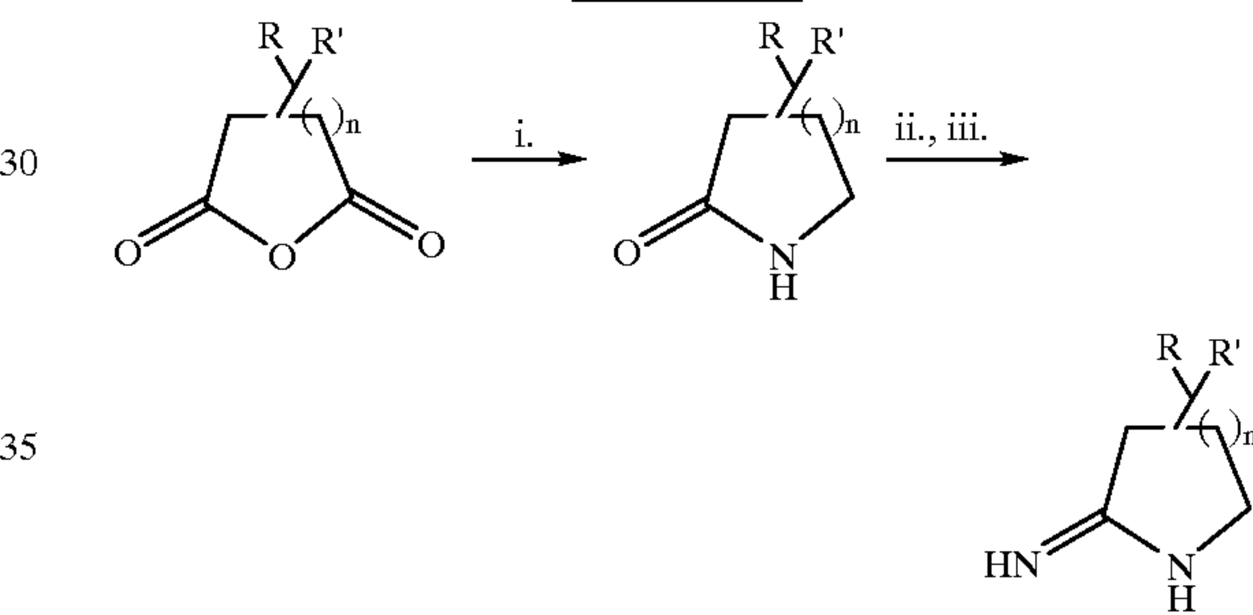
SCHEME IV
