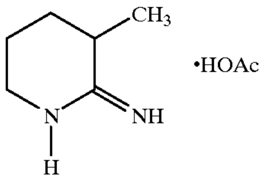
2-imino-3-methylpiperidine acetate
