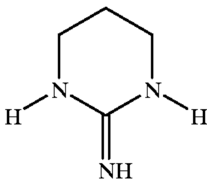
2-Iminotetrahydropyrimidine hemihydrosulfate; D. J. Brown and R. F. Evans, J. Chem. Soc. 4039–4045 (1962).
