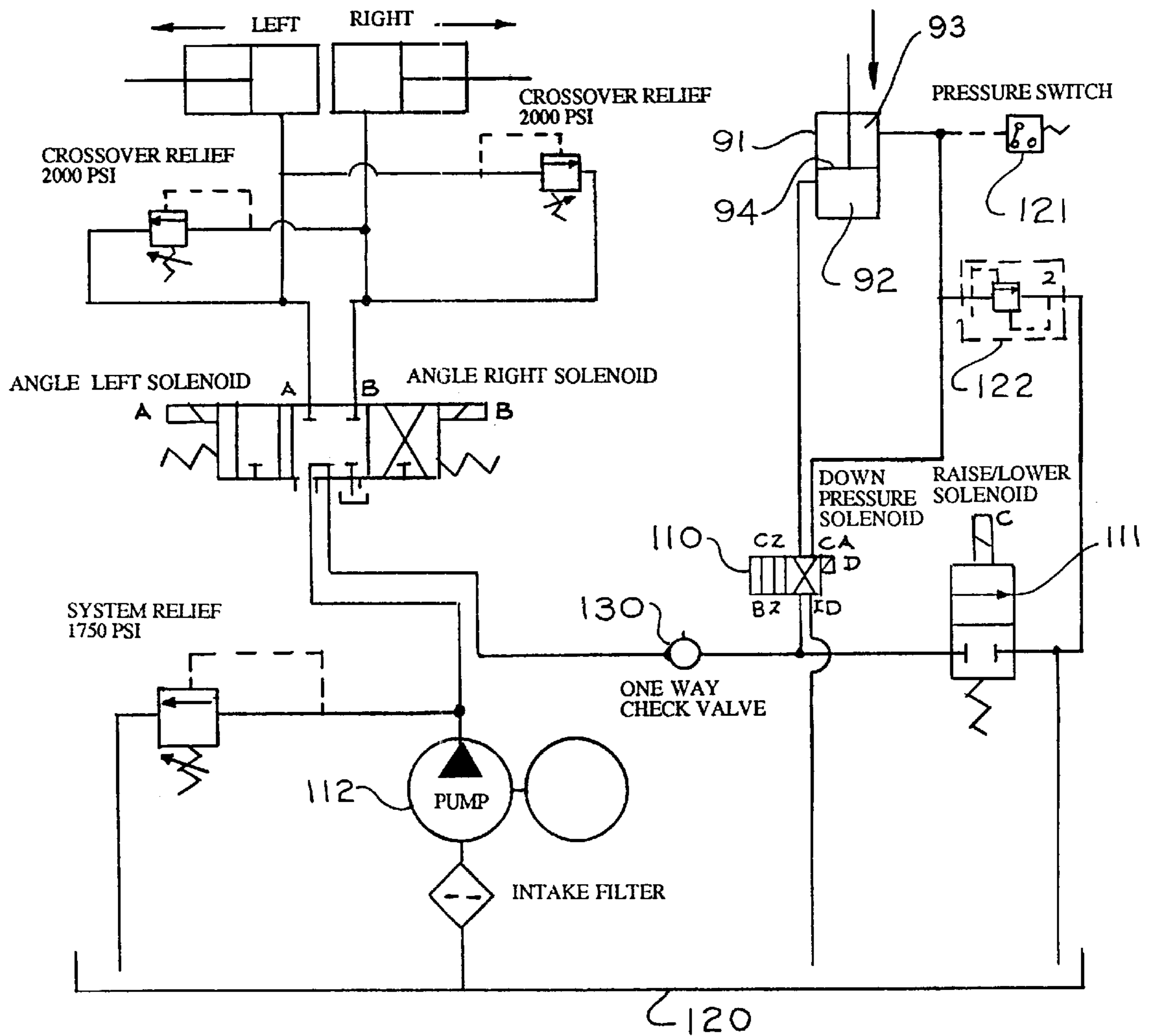
PRESSURE DOWN HYDRAULIC SYSTEM SCHEMATIC
