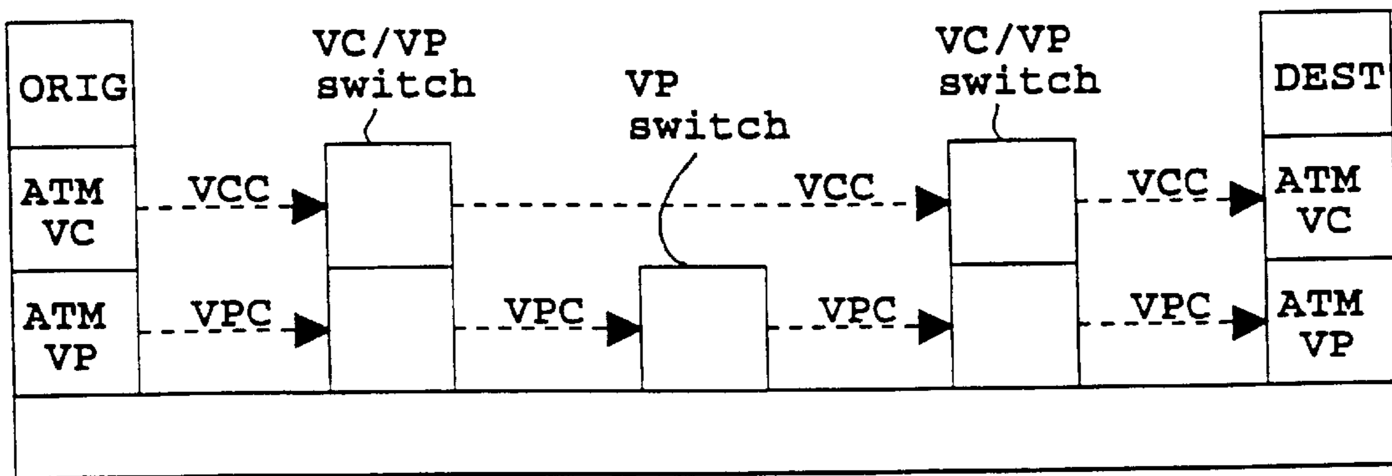
Fig. 2 (Prior art)
