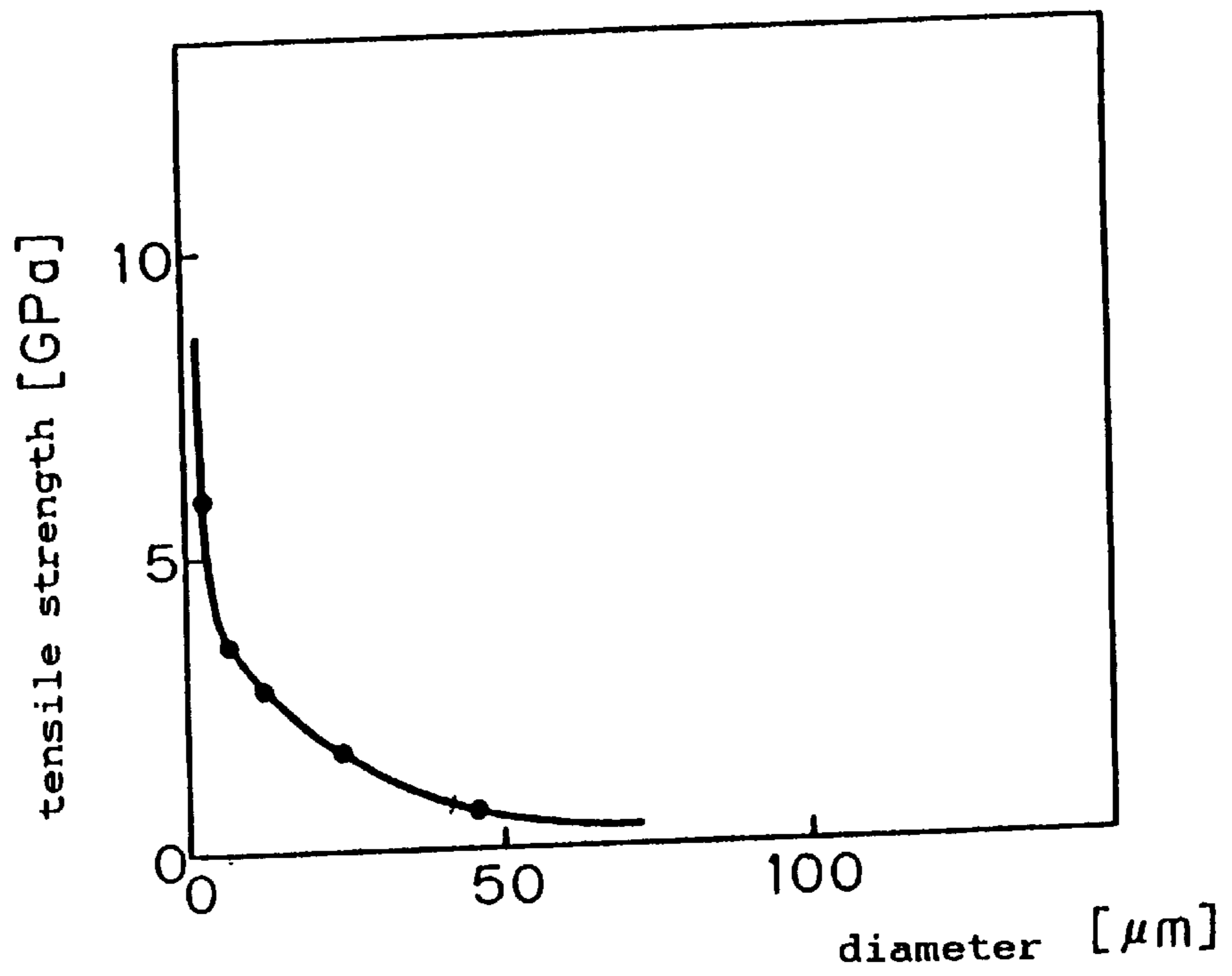
Relation between fiber diameter and tensile strength
