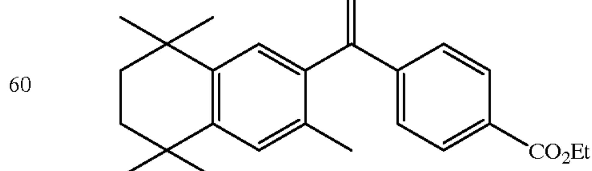
Ethyl-4-[1-(3,5,5,8,8-pentamethyl-5,6,7,8-tetrahydro-2-naphthyl) ethenyl] benzoate
