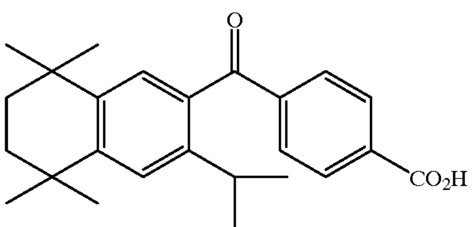
4-[(3-isopropyl-5, 5, 8, 8-tetramethyl-5, 6, 7, 8-tetrahydro-2-naphthyl) carbonyl] benzoic acid (3-1Pr-TTNCB)
