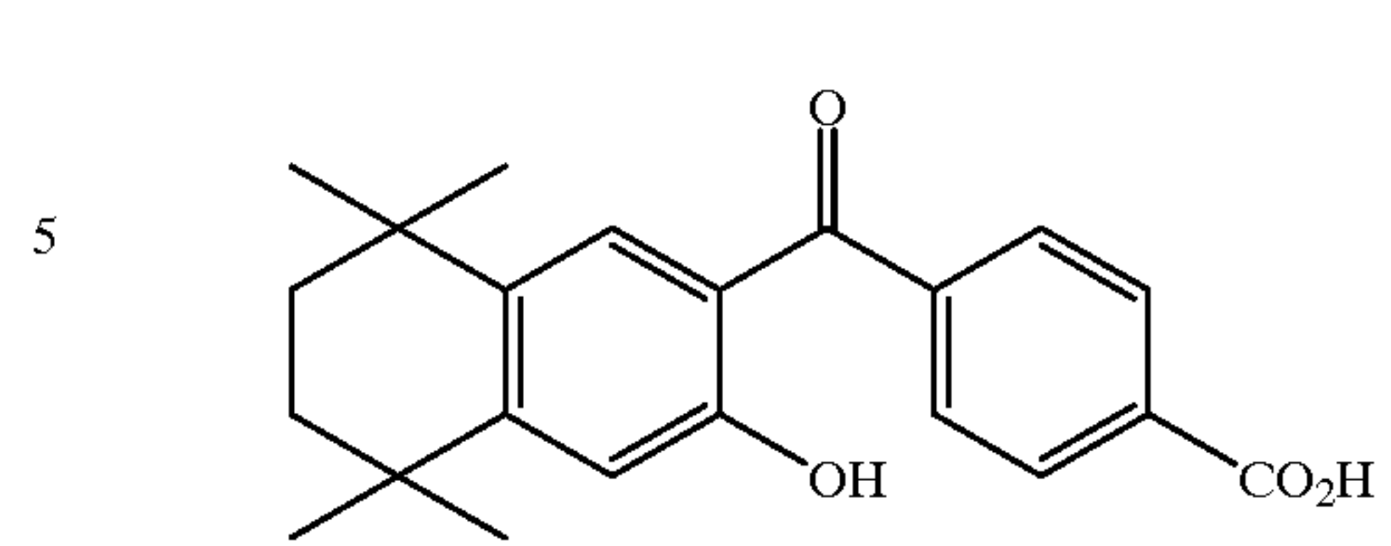
4-[(3-hydroxy-5, 5, 8, 8-tetramethyl-5, 6, 7, 8-tetrahydro-2-naphthyl) carbonyl] benzoic acid (3-hydroxy-TTNCB)
