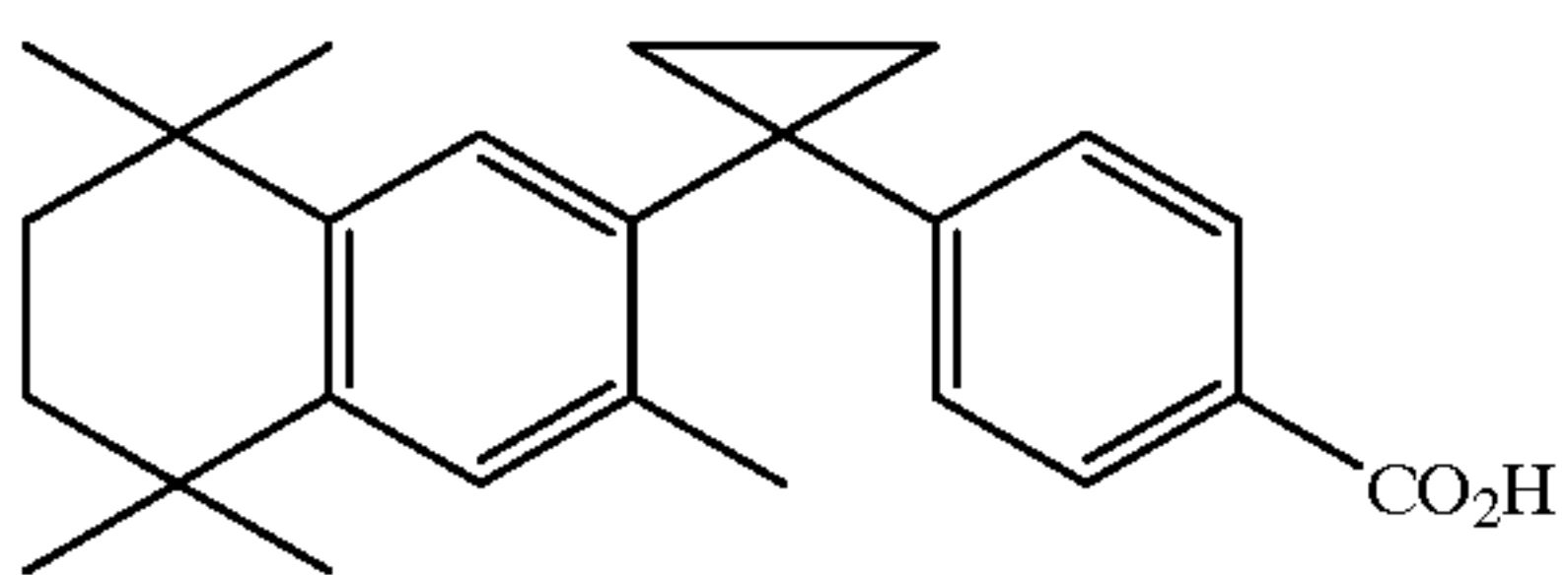
4-[1-(3,5,5,8,8-pentamethyl-5,6,7,8-tetrahydro-2-naphthyl) cyclopropyl] benzoic acid (TPNCB)
