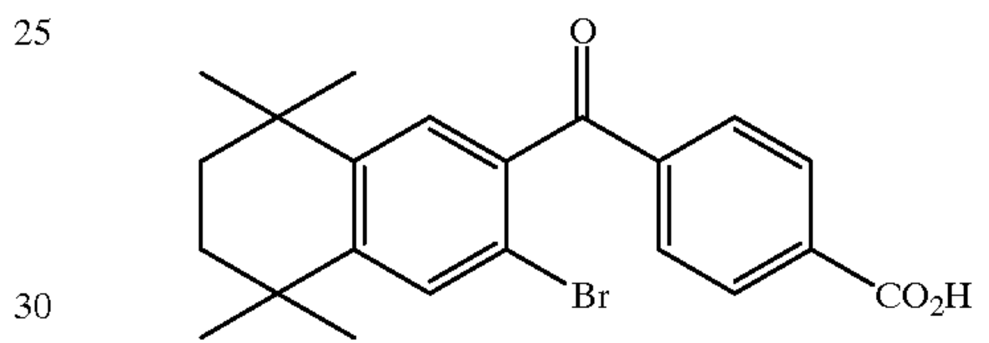
4-[(3-bromo-5, 5, 8, 8-tetramethyl-5, 6, 7, 8-tetrahydro-2-naphthyl) carbonyl] benzoic acid (3-bromo-TTNCB)
