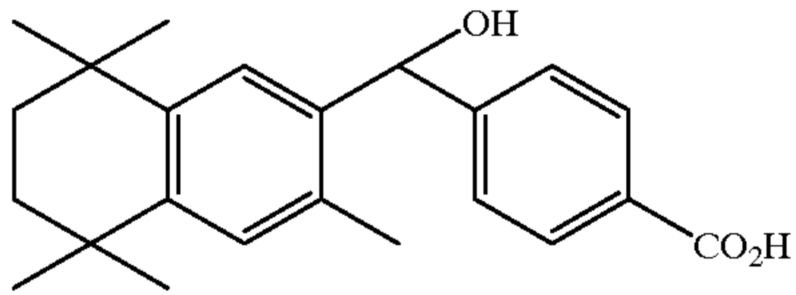
3-methyl-TTNHMB
