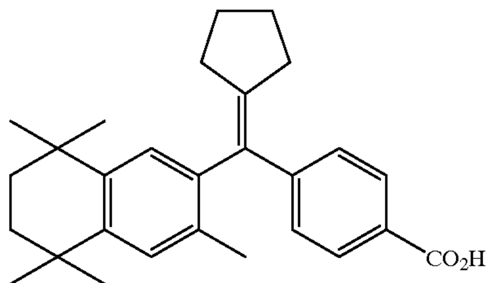
4-[1-(3,5,5,8,8-pentamethyl-5,6,7,8-tetrahydro-2-naphthyl) methylidene cyclopentane] benzoic acid (PTNCB)
