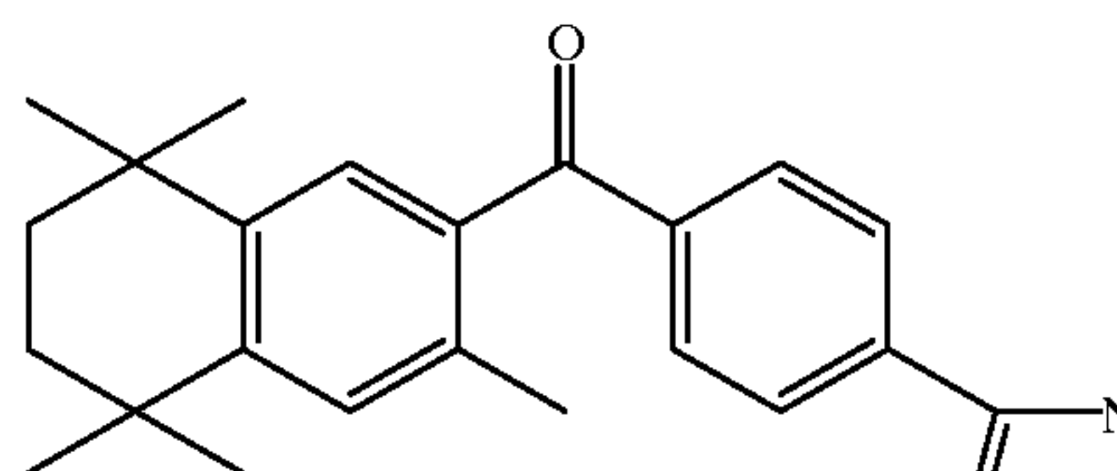
2-[1-(3,5,5,8,8-pentamethyl-5,6,7,8-tetrahydro-2-naphthyl) ethenyl] thiophene-5-carboxylic acid (TTNETC)
