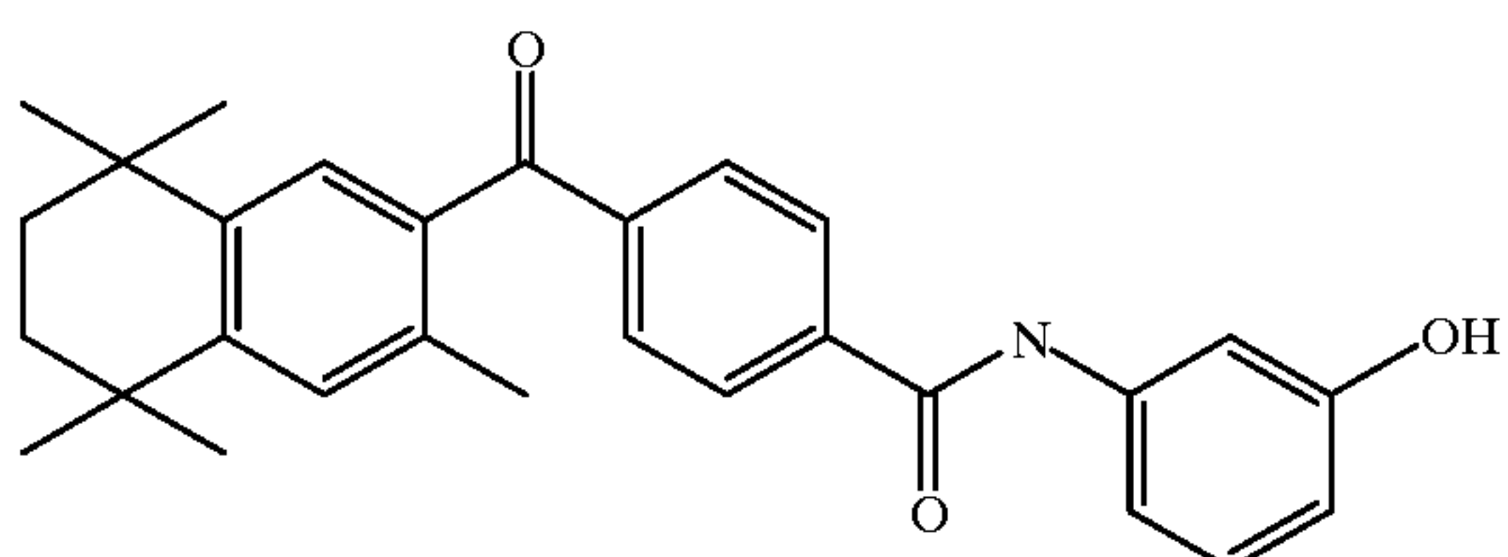
4-[(3,5,5,8,8-pentamethyl-5,6,7,8-tetrahydro-2-naphthyl) carbonyl]-N-(3-hydroxyphenyl) benzamide (3-Me-m-TTNCHBP)
