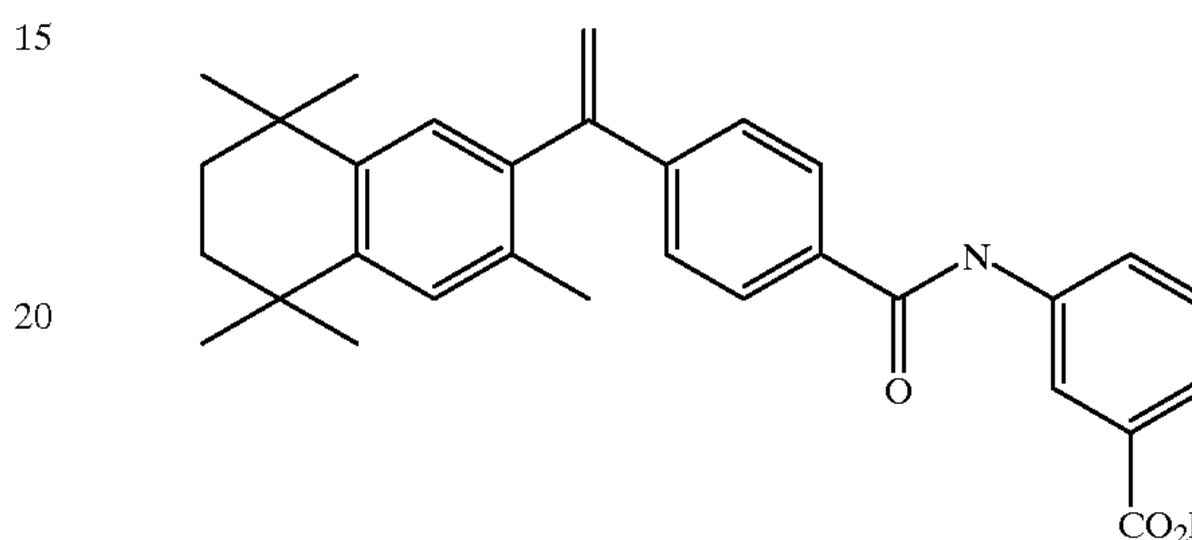
4-[1-(3,5,5,8,8-pentamethyl-5,6,7,8-tetrahydro-2-naphthyl) ethenyl]-N-(3-carboxyphenyl) benzamide (3-Me-m-TTNECBP)
