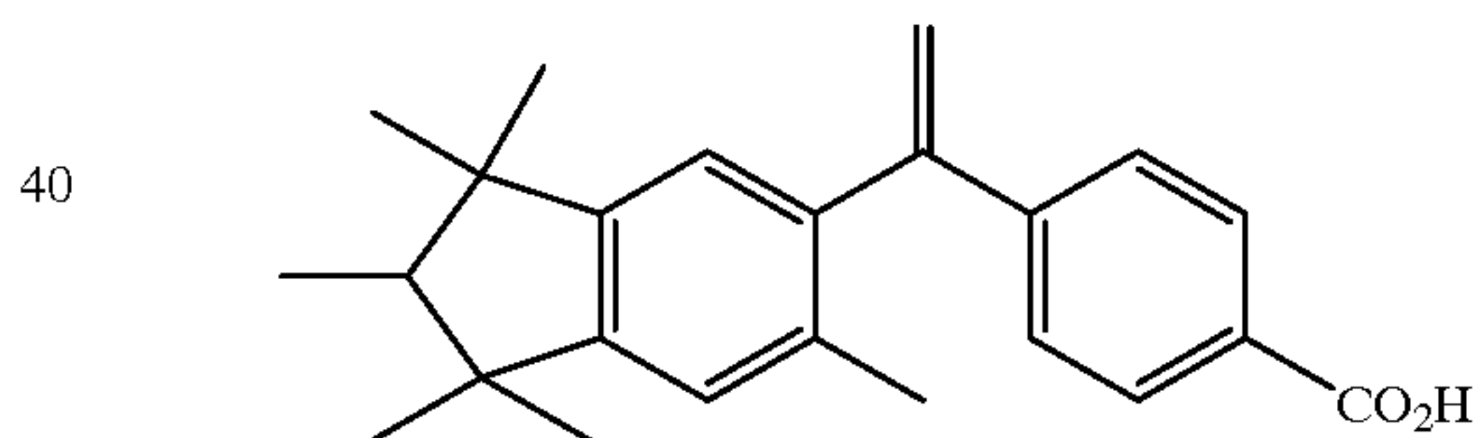
4-[1-(3,5,5,6,7,7-hexamethyl-2-indanyl) ethenyl] benzoic acid
