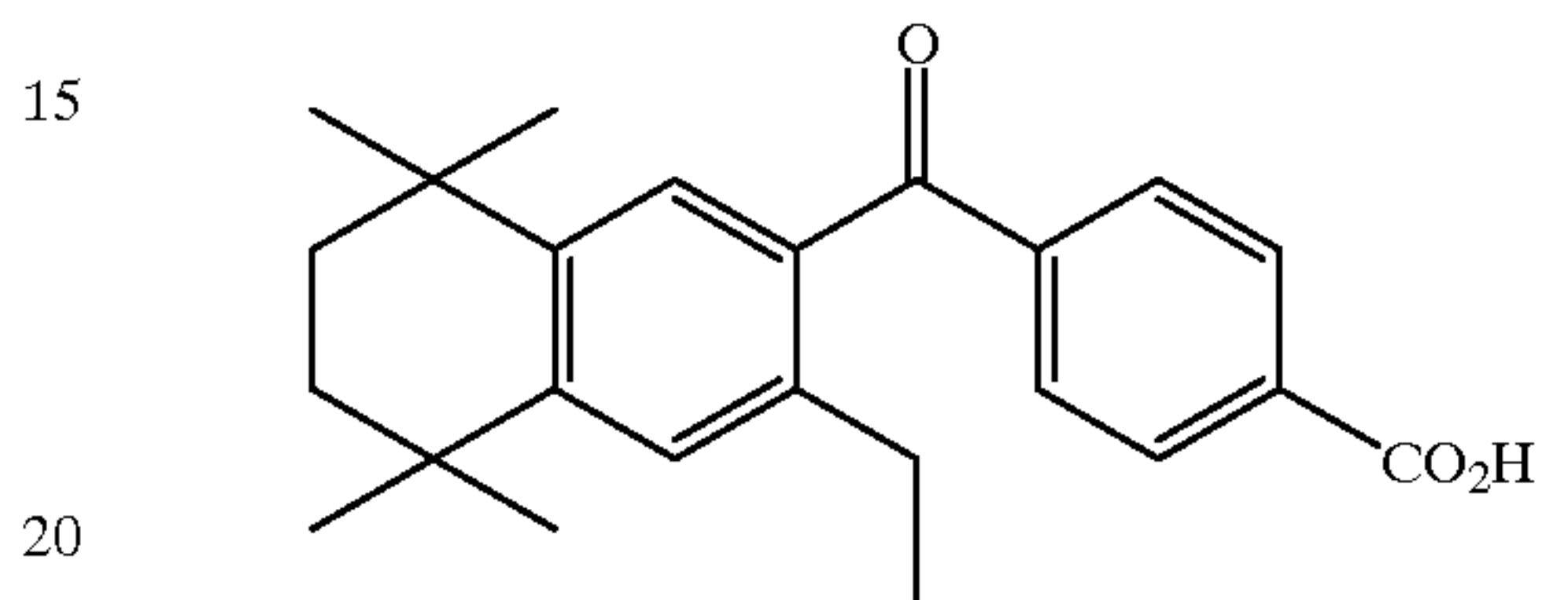
4-[(3-ethyl-5, 5, 8, 8-tetramethyl-5, 6, 7, 8-tetrahydro-2-naphthyl) carbonyl] benzoic acid (3-Et-TTNCB)
