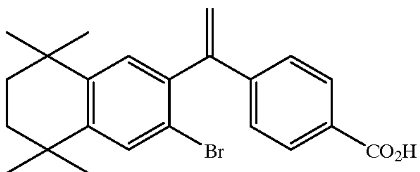
4-[1-(3-bromo-5,5,8,8-tetramethyl-5,6,7,8-tetrahydro-2-naphthyl) ethenyl] benzoic acid (3-bromo-TTNEB)
