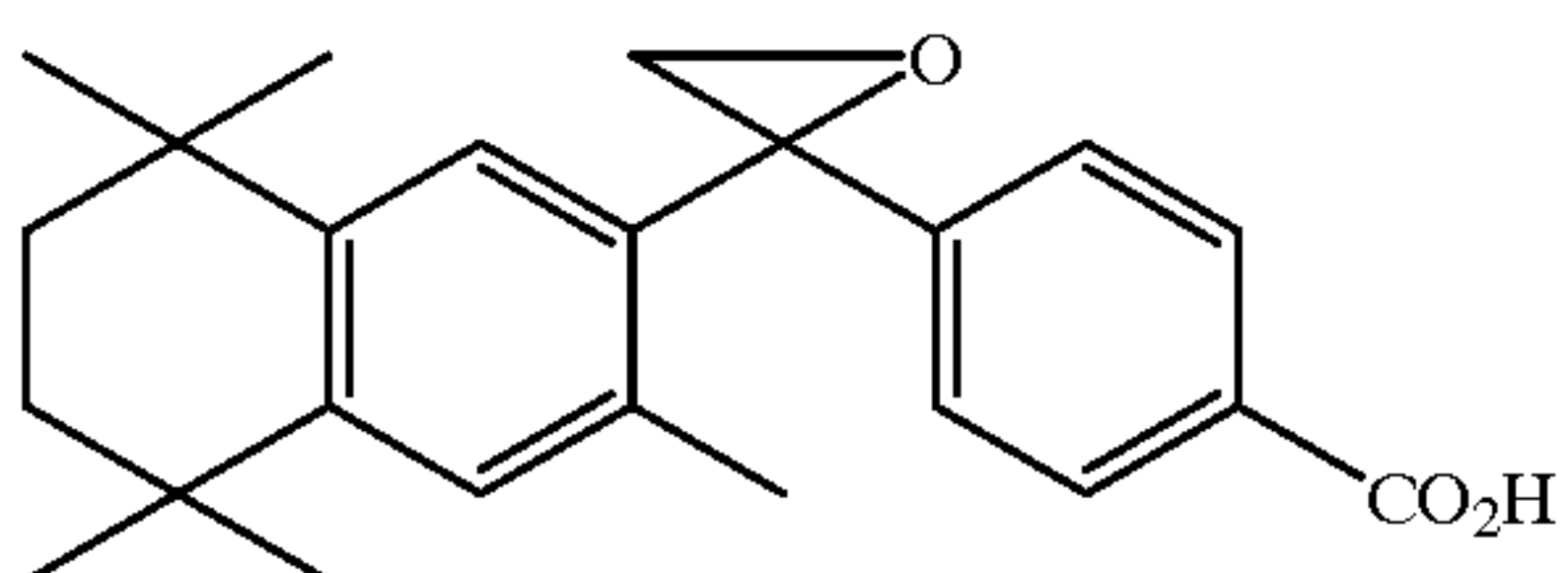
4-[1-(3,5,5,8,8-pentamethyl-5,6,7,8-tetrahydro-2-naphthyl) epoxy] benzoic acid (TPNEB)
