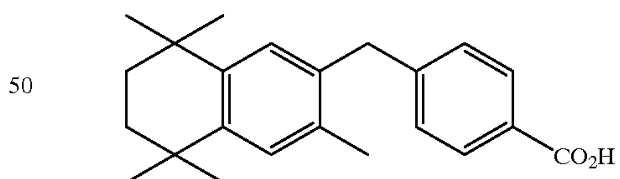
4-[1-(3,5,5,8,8-pentamethyl-5,6,7,8-tetrahydro-2-naphthyl) methyl] benzoic acid
