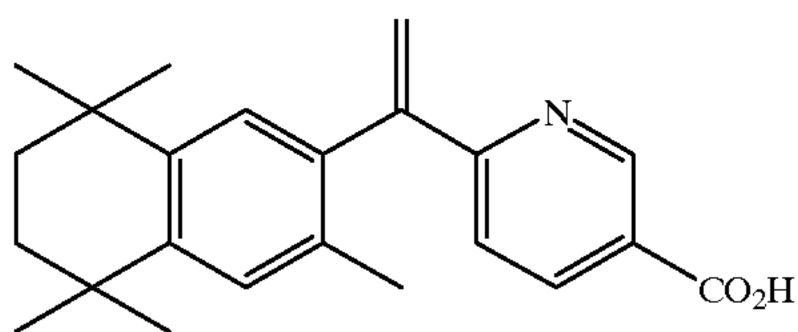
2-[1-(3,5,5,8,8-pentamethyl-5,6,7,8-tetrahydro-2-naphthyl) ethenyl] pyridine-5-carboxylic acid (TPNEP)
