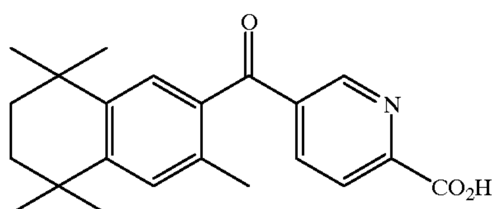
5-[(3,5,5,8,8-pentamethyl-5,6,7,8-tetrahydro-2-naphthyl) carbonyl] pyridine-2-carboxylic acid (TTNCP)
