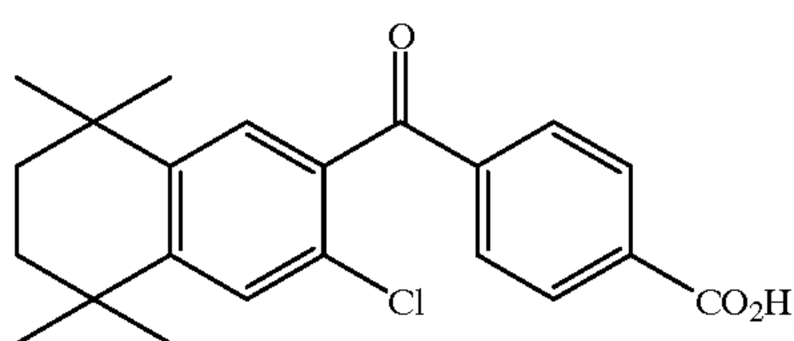
4-[(3-chloro-5, 5, 8, 8-tetramethyl-5, 6, 7, 8-tetrahydro-2-naphthyl) carbonyl] benzoic acid (3-chloro-TTNCB)
