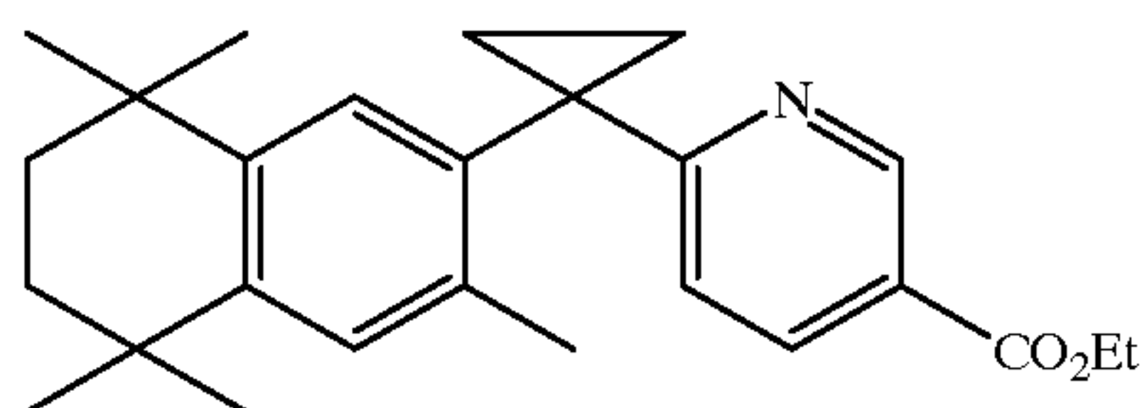
Ethyl-2-[1-(3,5,5,8,8-pentamethyl-5,6,7,8-tetrahydro-2-naphthyl) cyclopropyl] pyridine-5-carboxylate
