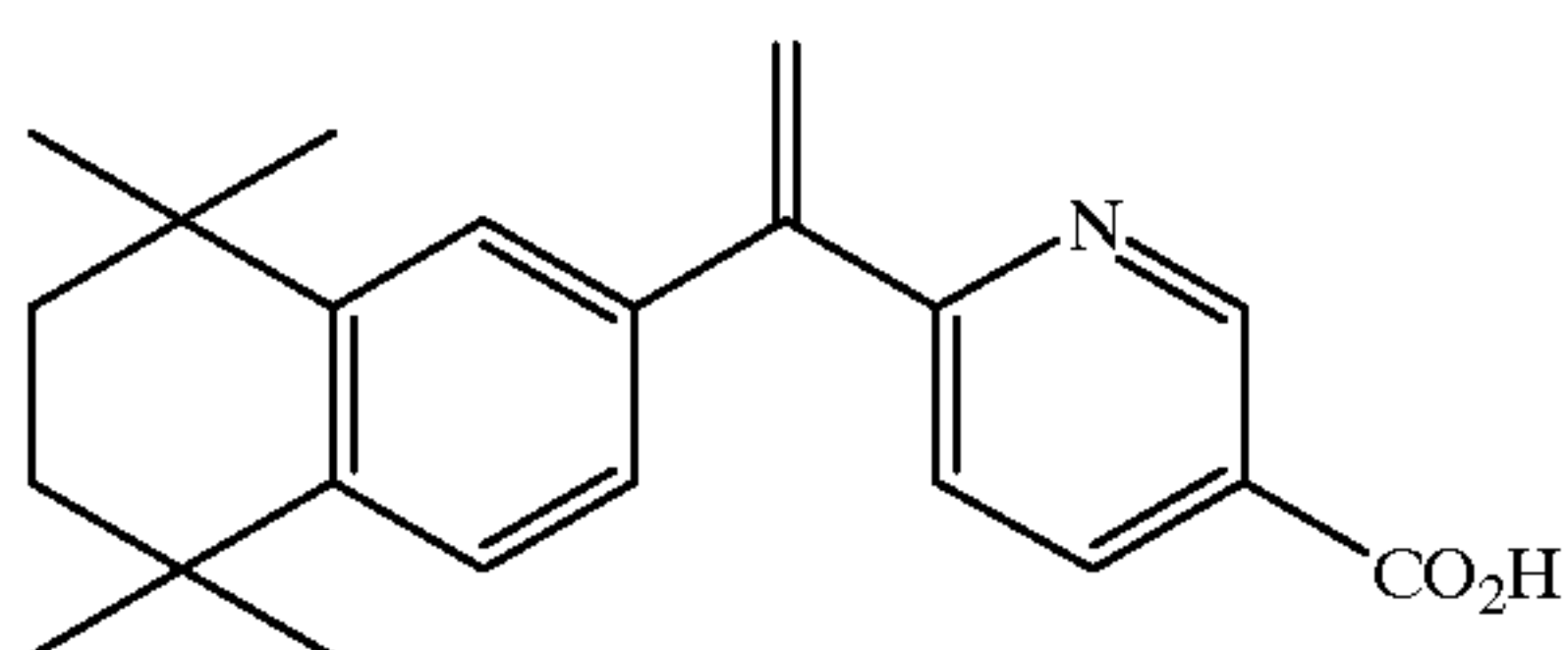
2-[1-(5,5,8,8-tetramethyl-5,6,7,8-tetrahydro-2-naphthyl) ethenyl] pyridine-5-carboxylic acid (TTNEP)
