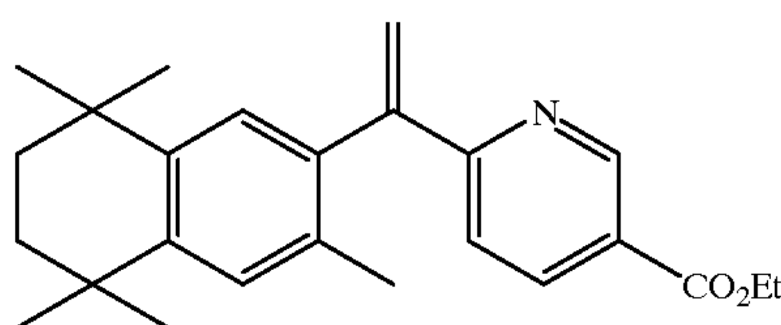
Ethyl-2-[1-(3,5,5,8,8-pentamethyl-5,6,7,8-tetrahydro-2-naphthyl) ethenyl] pyridine-5-carboxylate
