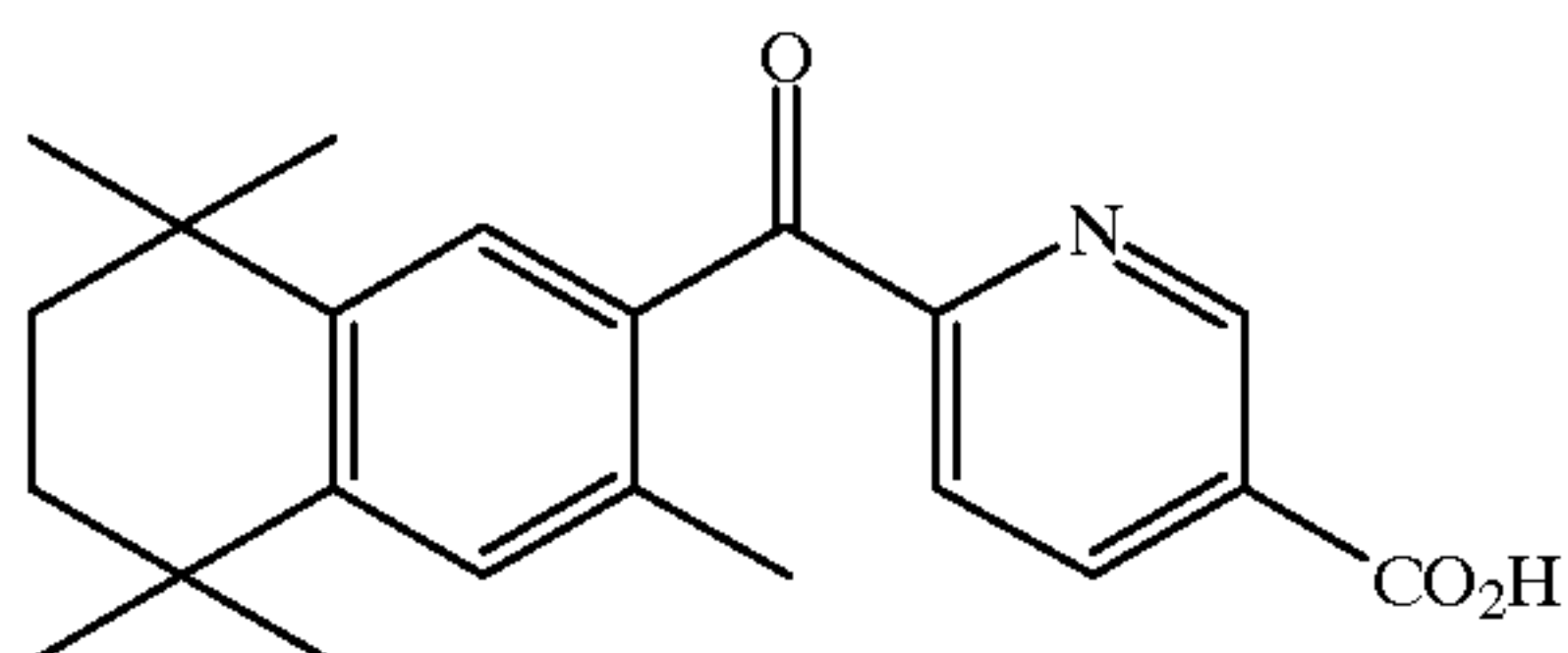
2-[(3,5,5,8,8-pentamethyl-5,6,7,8-tetrahydro-2-naphthyl) carbonyl] pyridine-5-carboxylic acid
