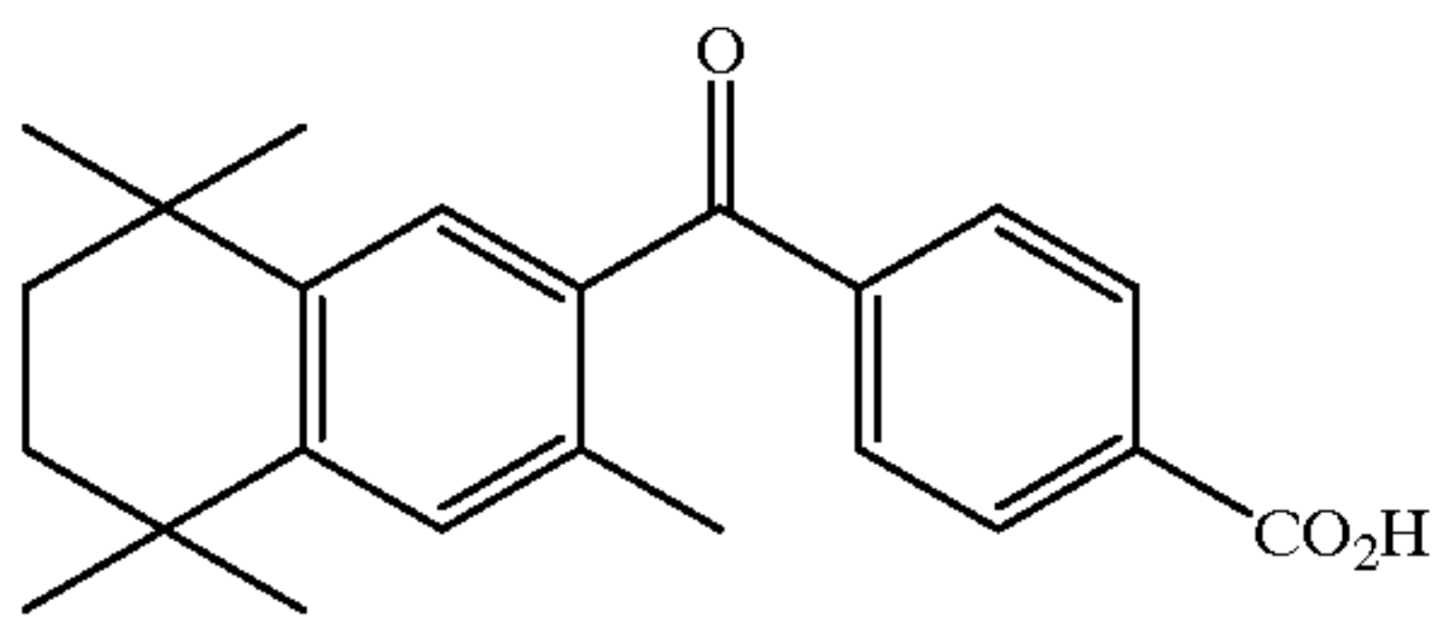
3-methyl-TTNCB
