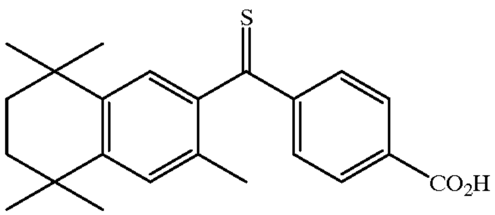
thioketone
