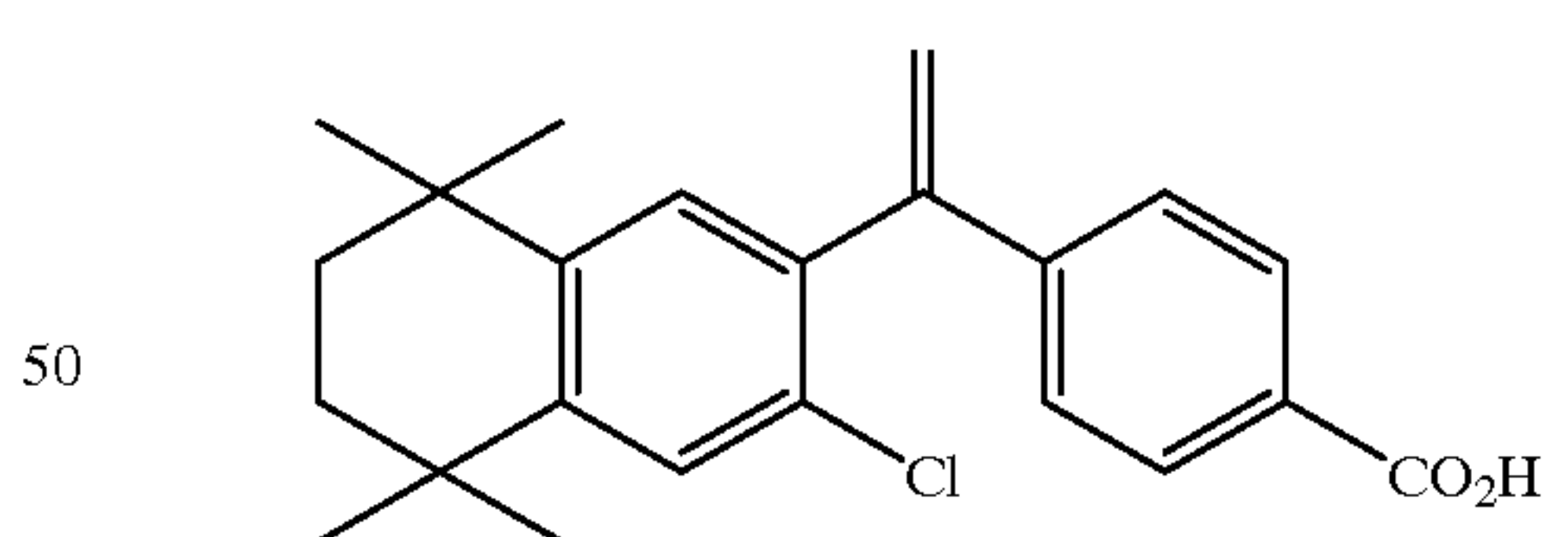
4-[1-(3-chloro-5, 5, 8, 8-tetramethyl-5, 6, 7, 8-tetrahydro-2-naphthyl) ethenyl] benzoic acid (3-chloro-TTNEB)
