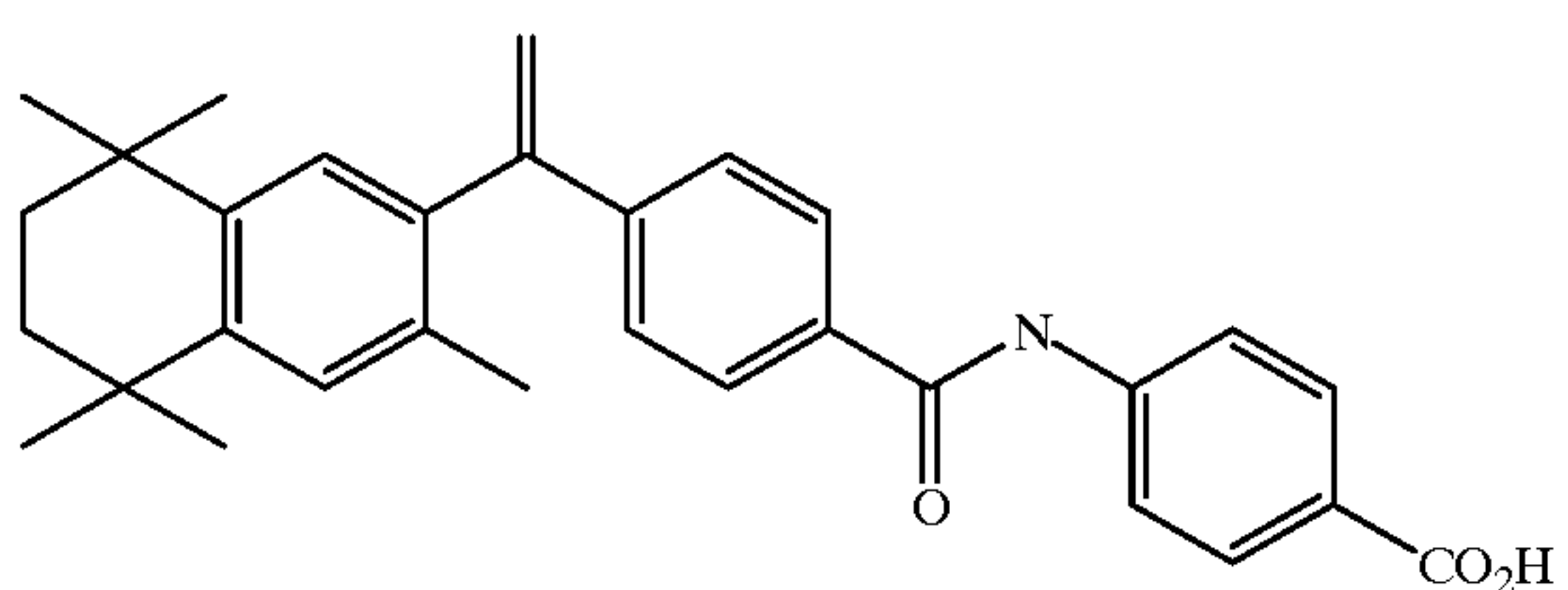
4-[1-(3,5,5,8,8-pentamethyl-5,6,7,8-tetrahydro-2-naphthyl) ethenyl]-N-(4-carboxyphenyl) benzamide (3-Me-TTNECBP)
