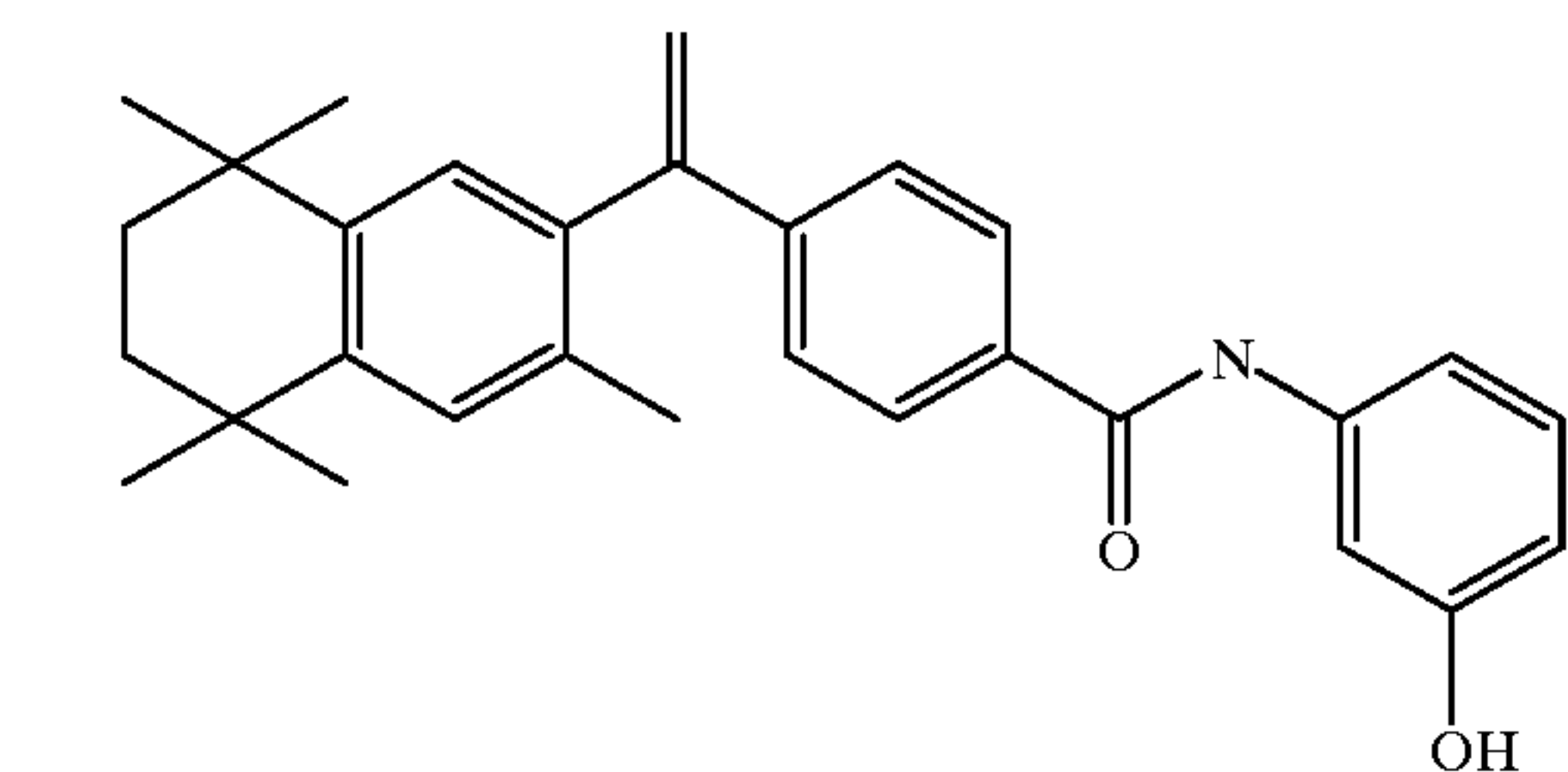
4-[1-(3,5,5,8,8-pentamethyl-5,6,7,8-tetrahydro-2-naphthyl) ethenyl]-N-(3-hydroxyphenyl) benzamide (3-Me-m-TTNEHBP)
