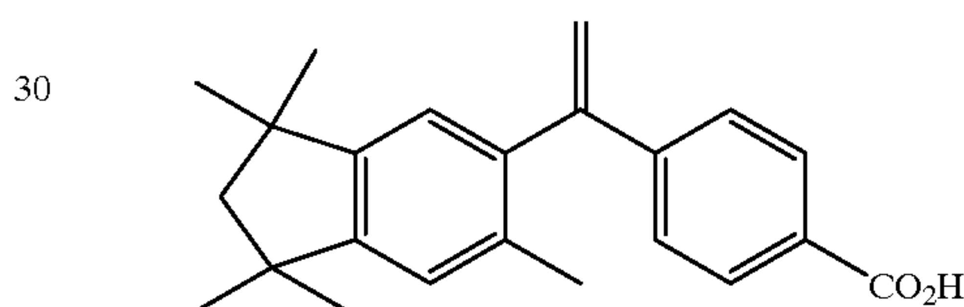
4-[1-(3,5,5,7,7-pentamethyl-2-indanyl) ethenyl] benzoic acid
