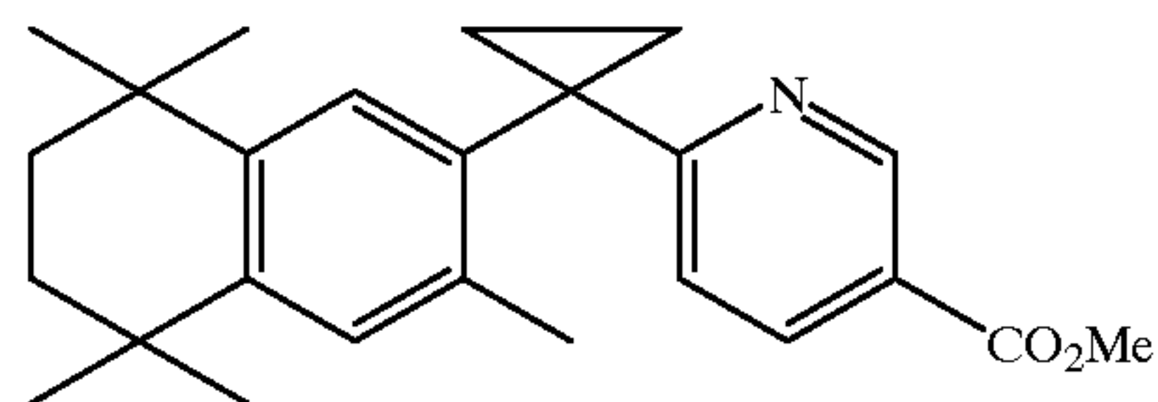
Methyl 2-[1-(3,5,5,8,8-pentamethyl-5,6,7,8-tetrahydro-2-naphthyl) cyclopropyl] pyridine-5-carboxylate
