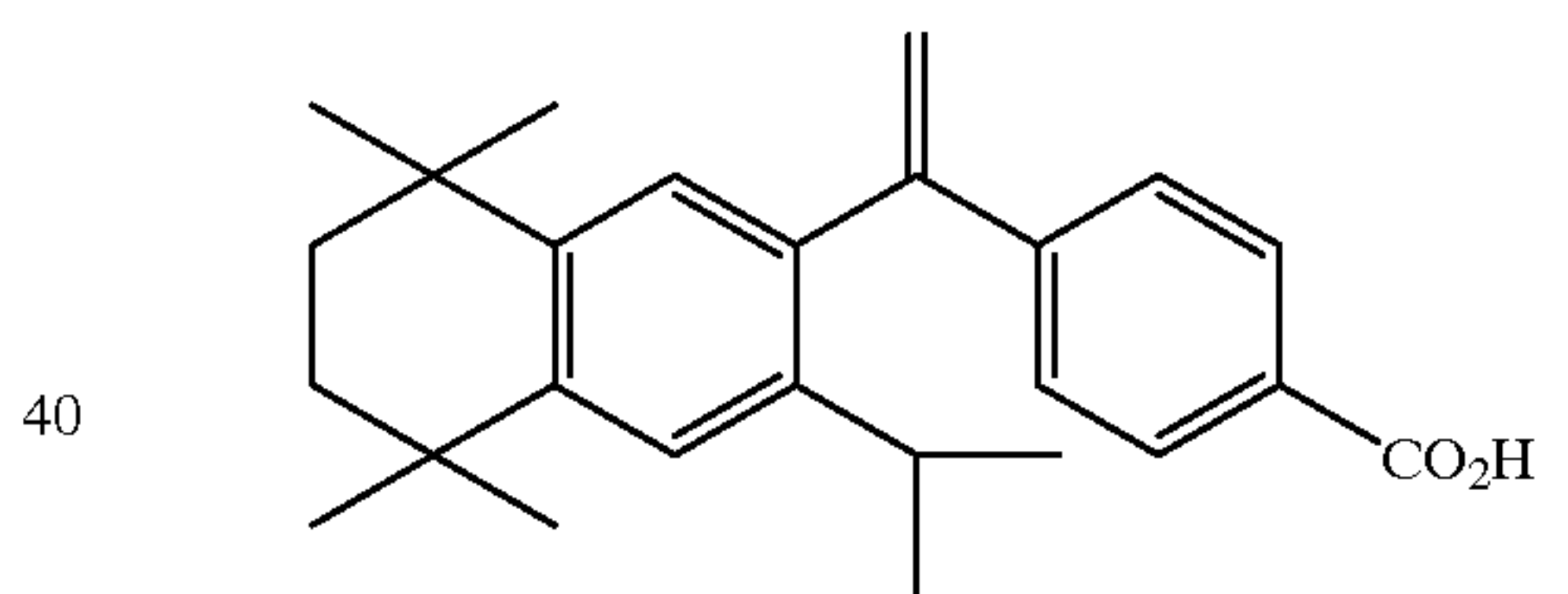
4-[1-(3-isopropyl-5, 5, 8, 8-tetramethyl-5, 6, 7, 8-tetrahydro-2-naphthyl) ethenyl] benzoic acid (3-iPr-TTNEB)
