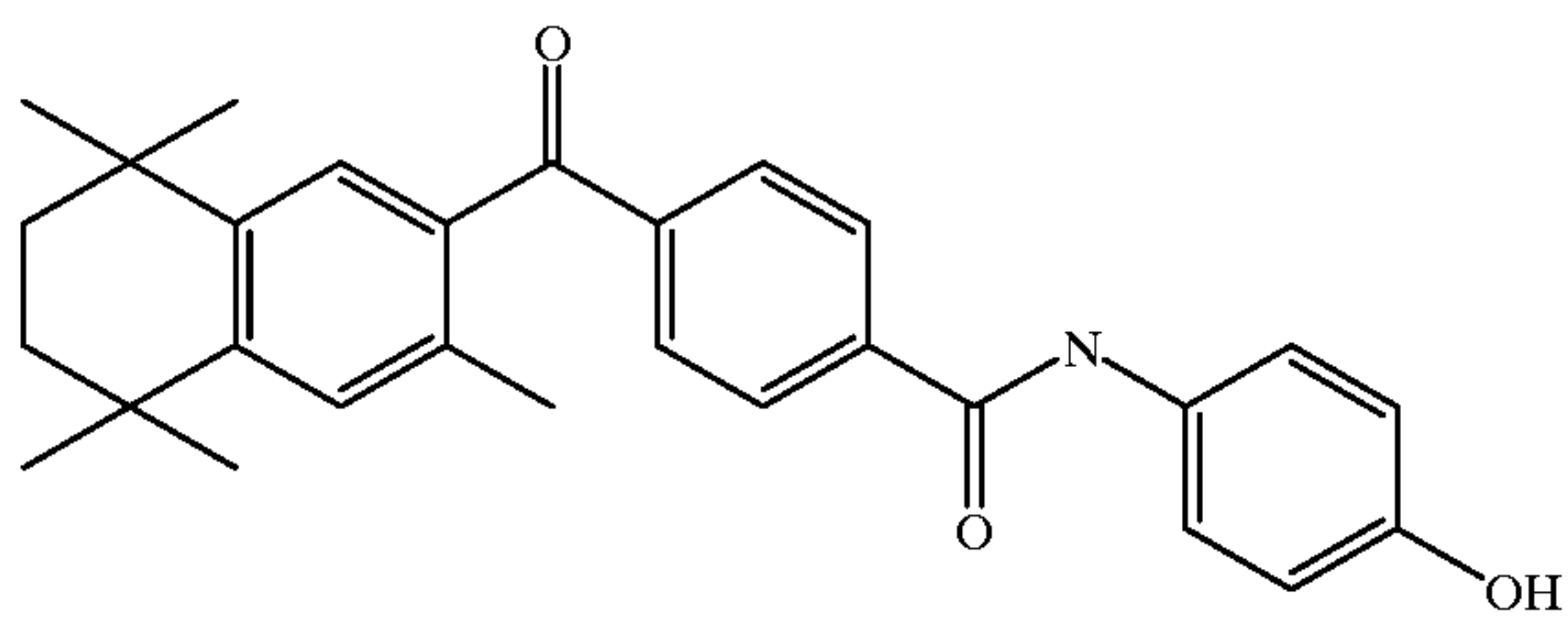
3-methyl-TTNCHBP
