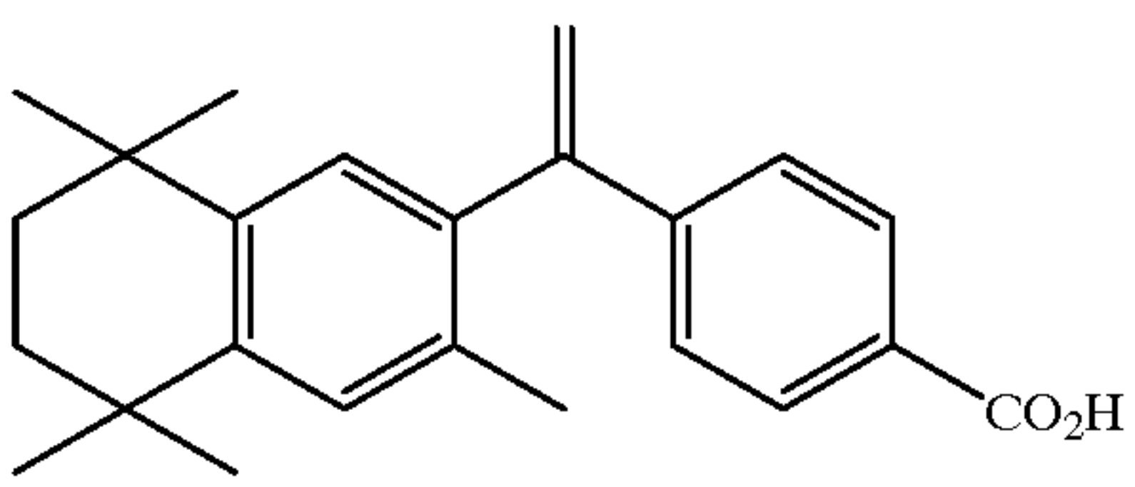
3-methyl-TTNEB
