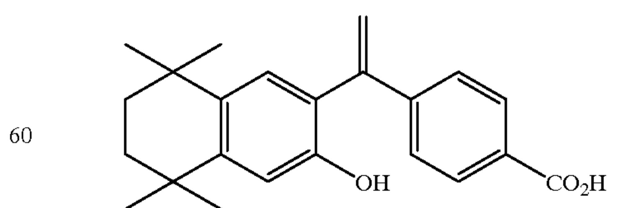
4-[1-(3-hydroxy-5, 5, 8, 8-tetramethyl-5, 6, 7, 8-tetrahydro-2-naphthyl) ethenyl] benzoic acid (3-hydroxy-TTNEB)
