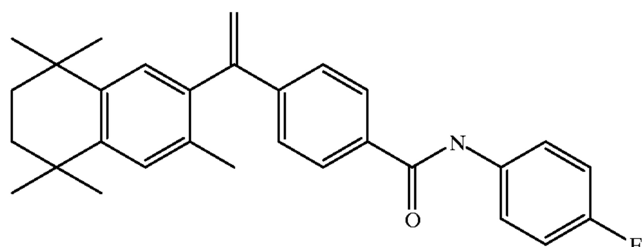
4-[1-(3,5,5,8,8-pentamethyl-5,6,7,8-tetrahydro-2-naphthyl) ethenyl]-N-(4-fluorophenyl) benzamide (3-Me-TTNEFBP)
