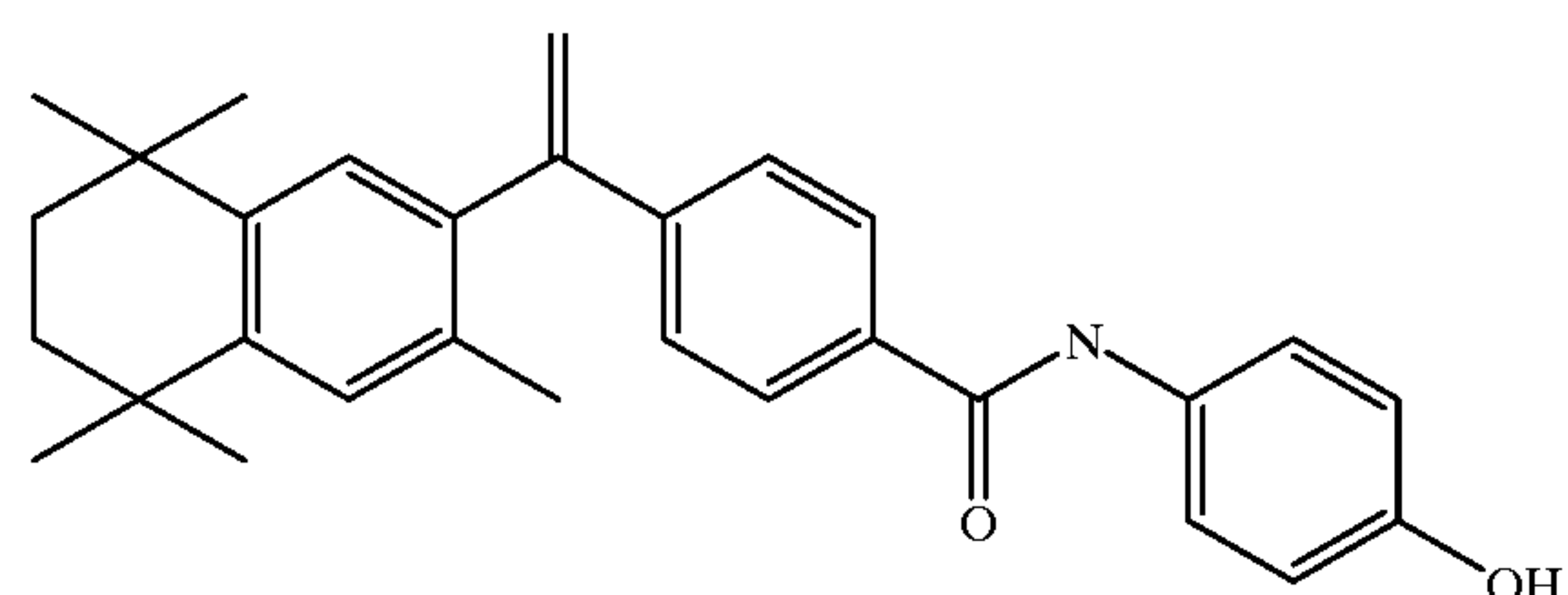
4-[1-(3,5,5,8,8-pentamethyl-5,6,7,8-tetrahydro-2-naphthyl) ethenyl]-N-(4-hydroxyphenyl) benzamide (3-Me-TTNEHBP)
