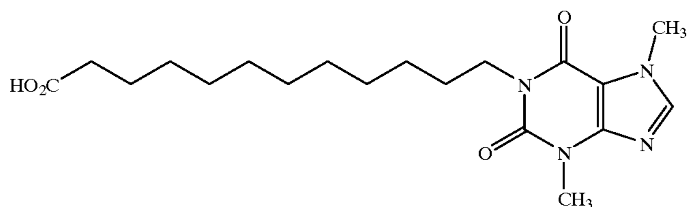
1-12-yl-Dodecanoic acid)-3,7-dimethylxanthine
