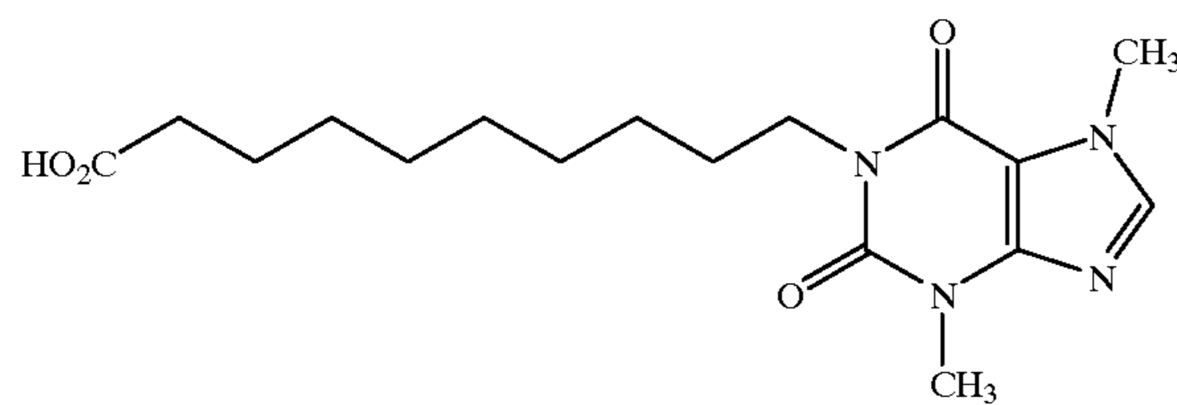
1-(10-yl-Decanoic acid)-3, 7-dimethylxanthine
