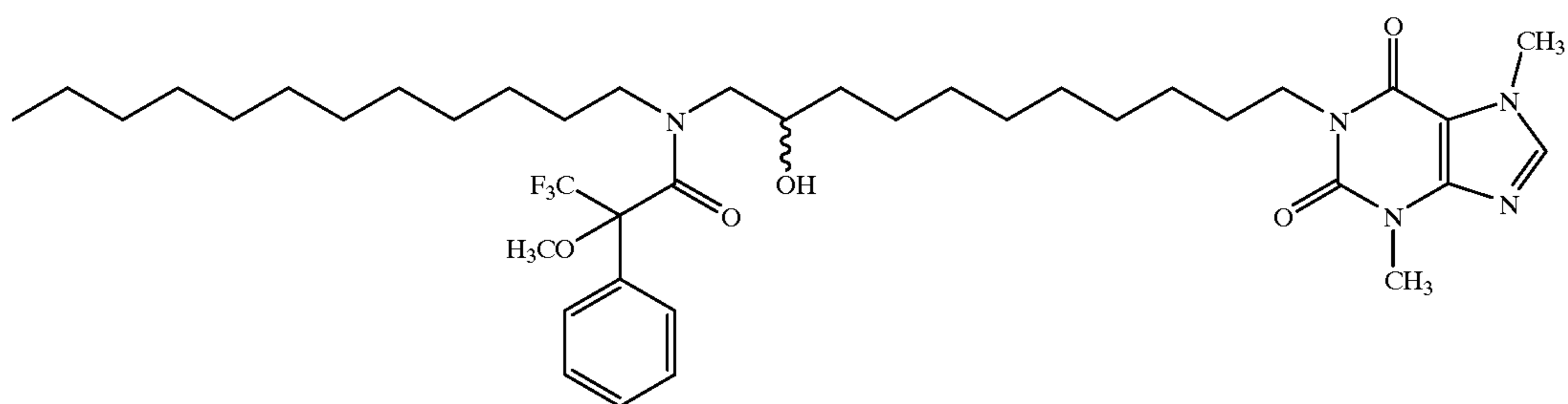
1-[11-[N-Dodecyl(R)-2-methoxy-2-phenylacetamido]-10-hydroxyundecyl]-3,7-dimethylxanthine
