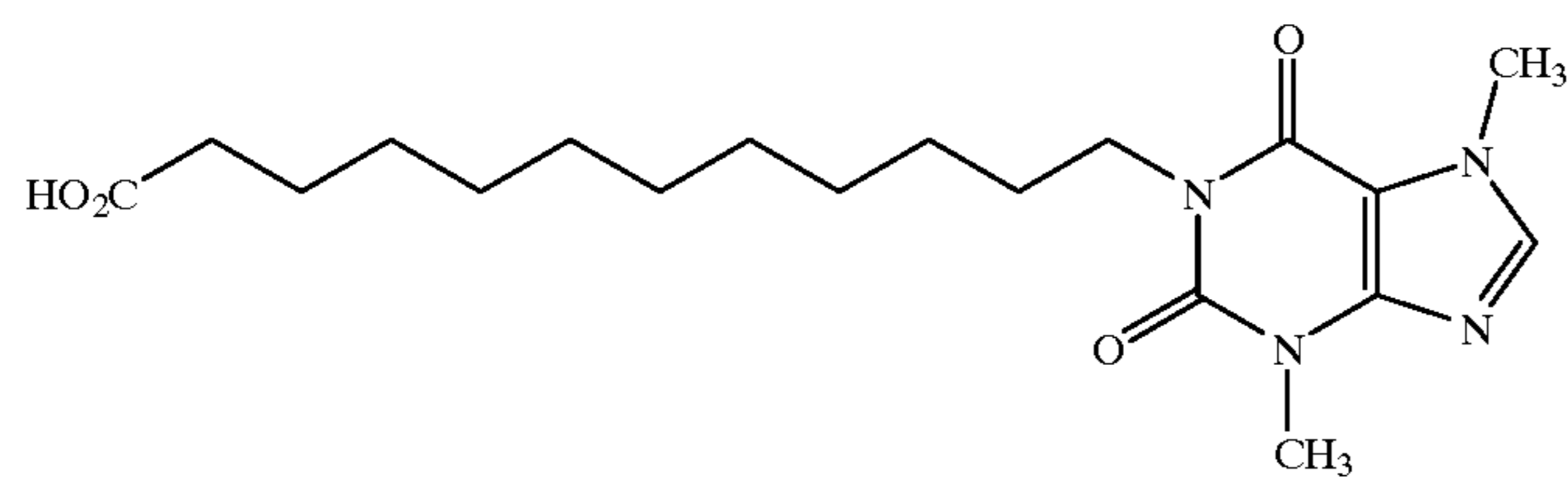
1-12-yl-Dodecanoic acid)-3,7-dimethylxanthine
