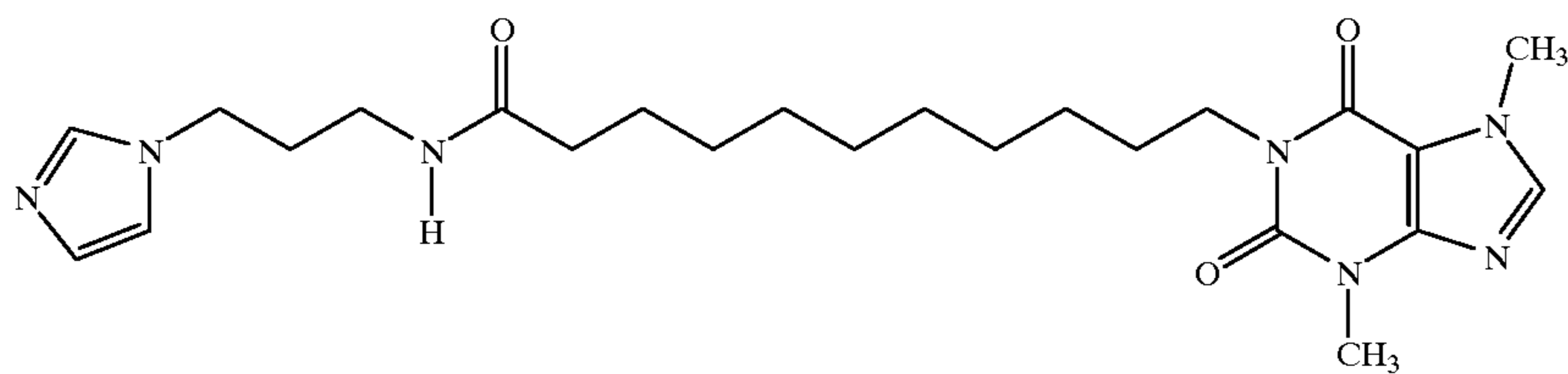
1-[N-(3-Imidazolopropyl)-11-yl-undecanoamide]-3,7-dimethylxanthine
