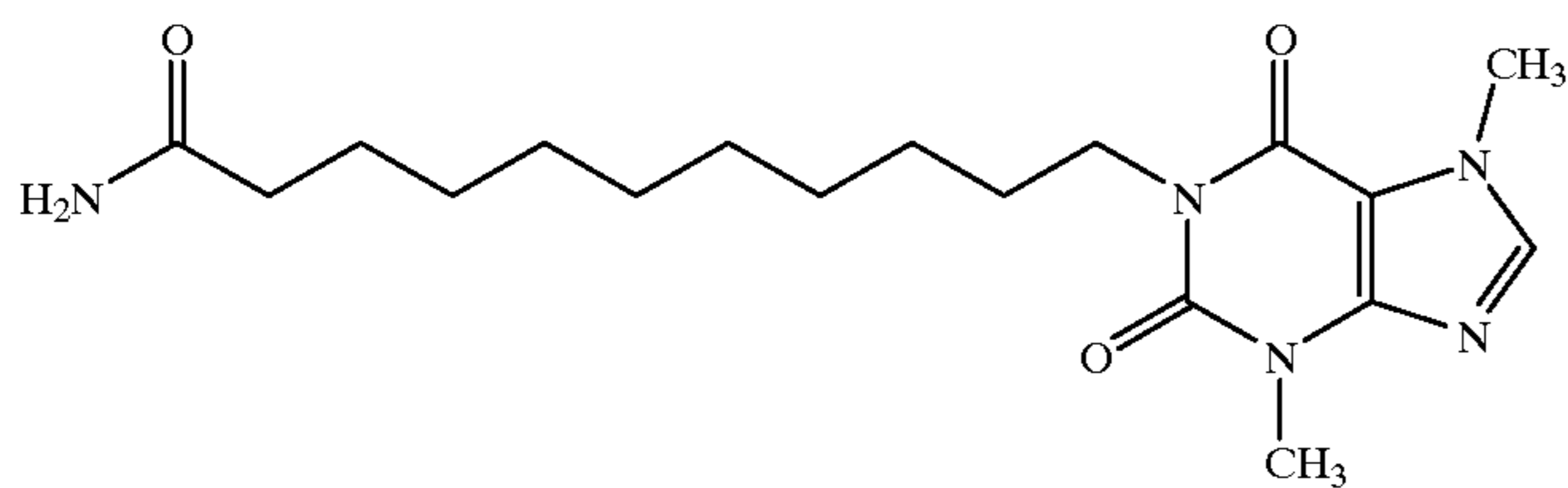
1-(11-yl-Undecanamide)-3,7-dimethylxanthine
