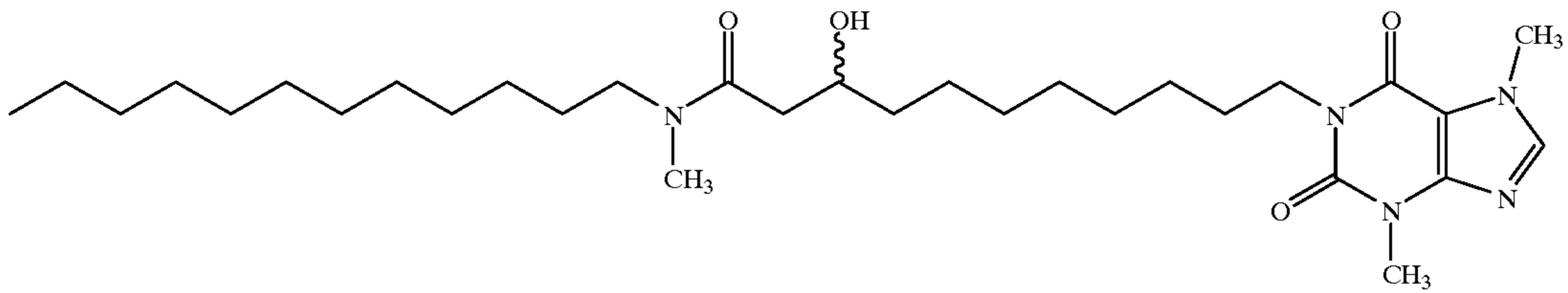
1-(11-Dodecylmethylamino-9-hydroxy-11-oxoundecyl)-3,7-dimethylxanthine
