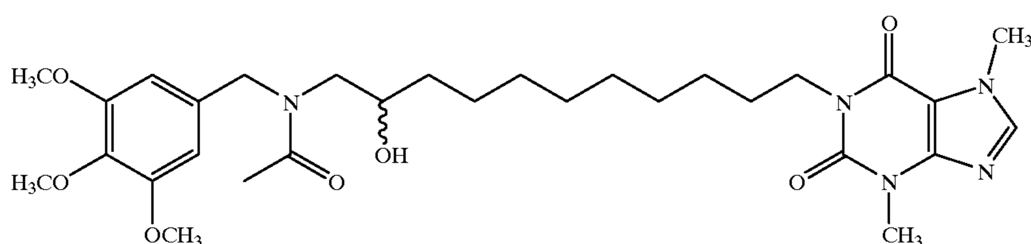
1-[11-(3,4,5-Trimethoxybenzylacetamido)-10-hydroxyundecyl]-3,7-dimethylxanthine
