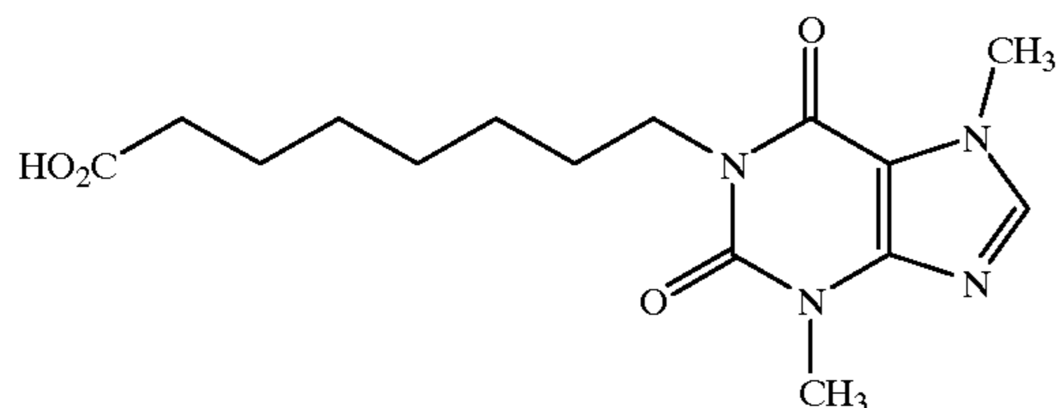
1-(8-yl-Octanoic acid)-3,7-dimethylxanthine
