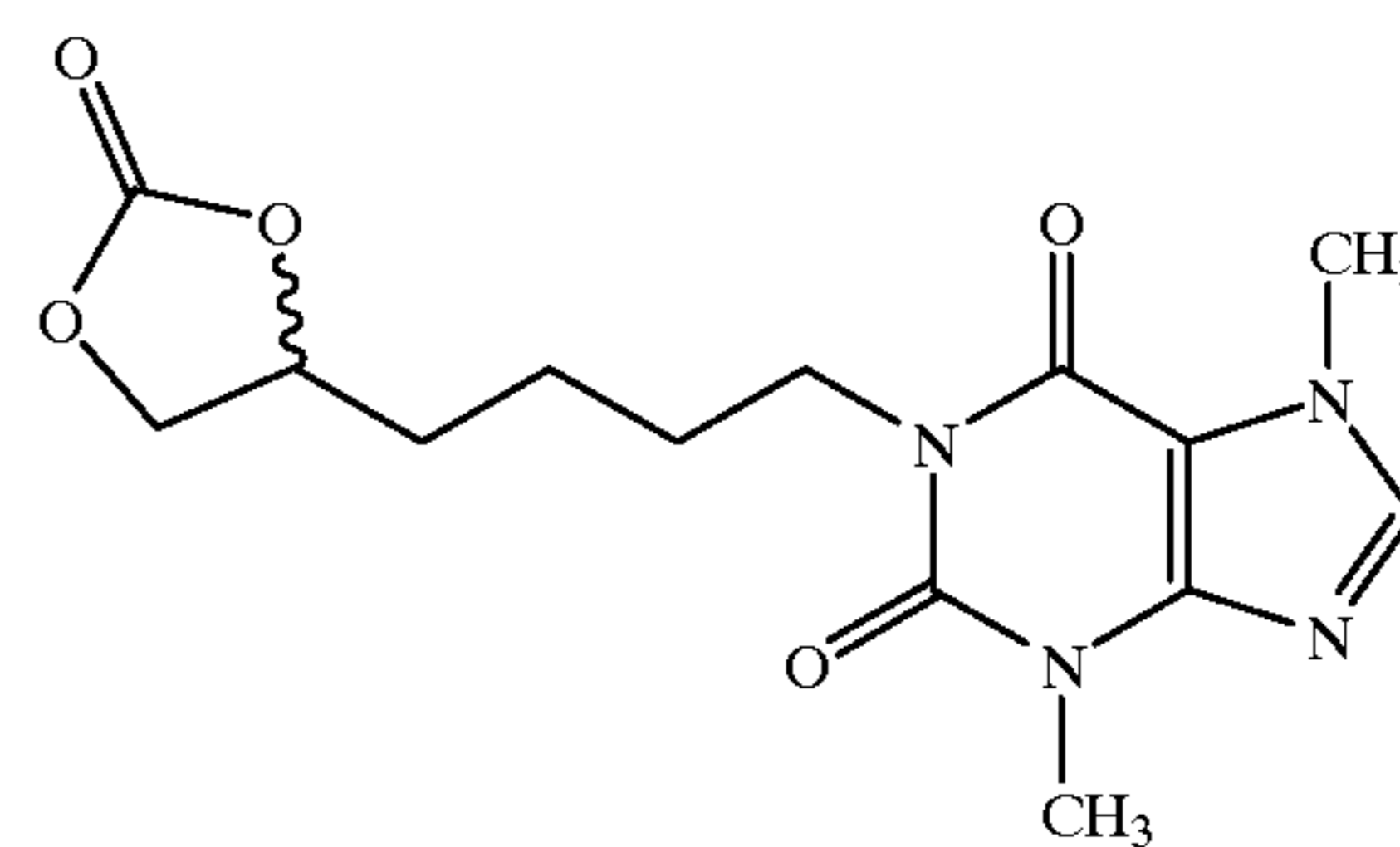
1-(5,6-Carbonyldioxyhexyl)-3,7-dimethylxanthine
