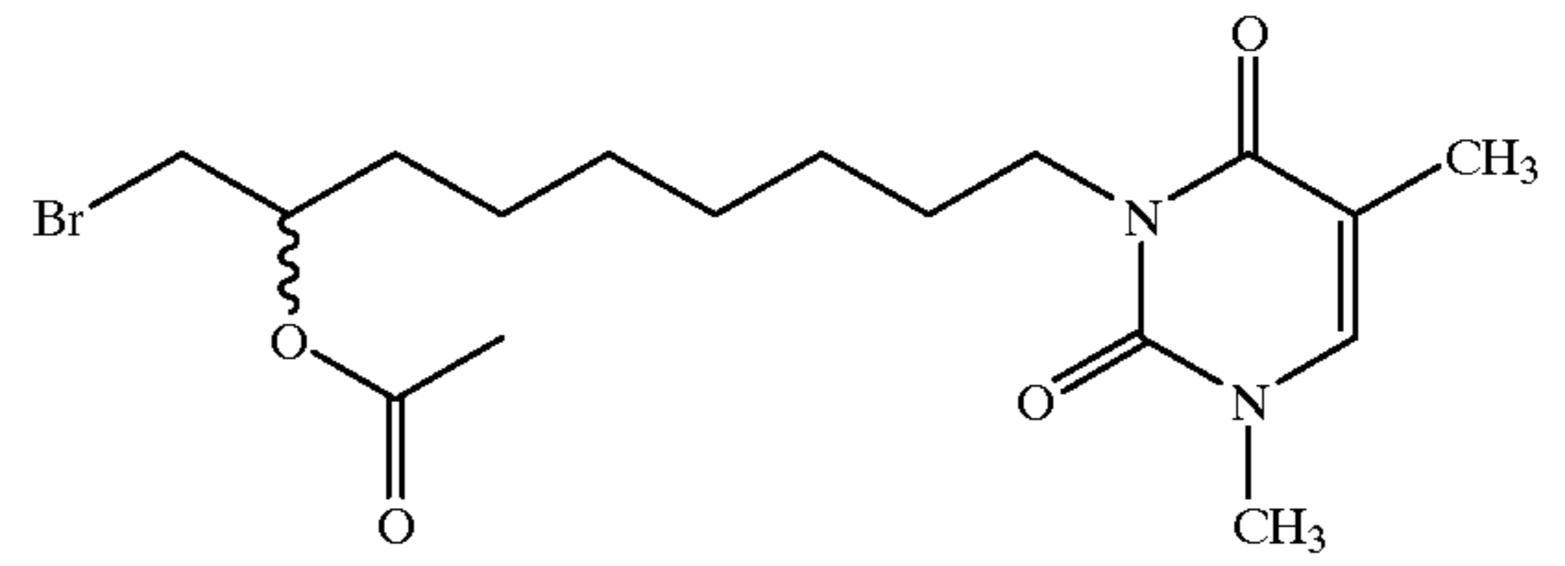
3-(8-Acetoxy-9-bromononyl)-1-methylthymine
