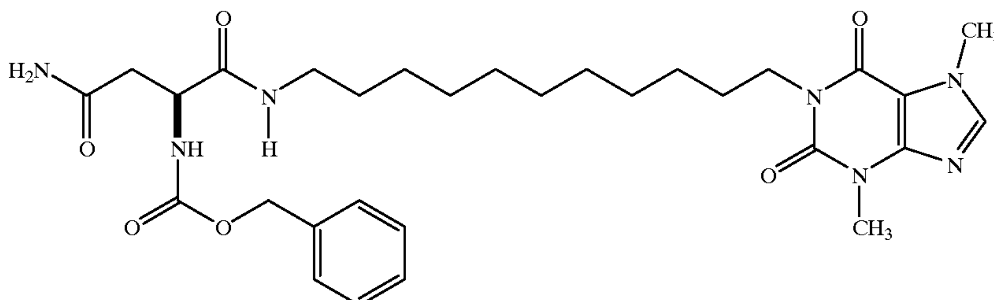
1-(11-[4-Amino-2-carbobenzyloxyamino-4-oxobutyronamido]undecyl)-3,7-dimethylxanthine
