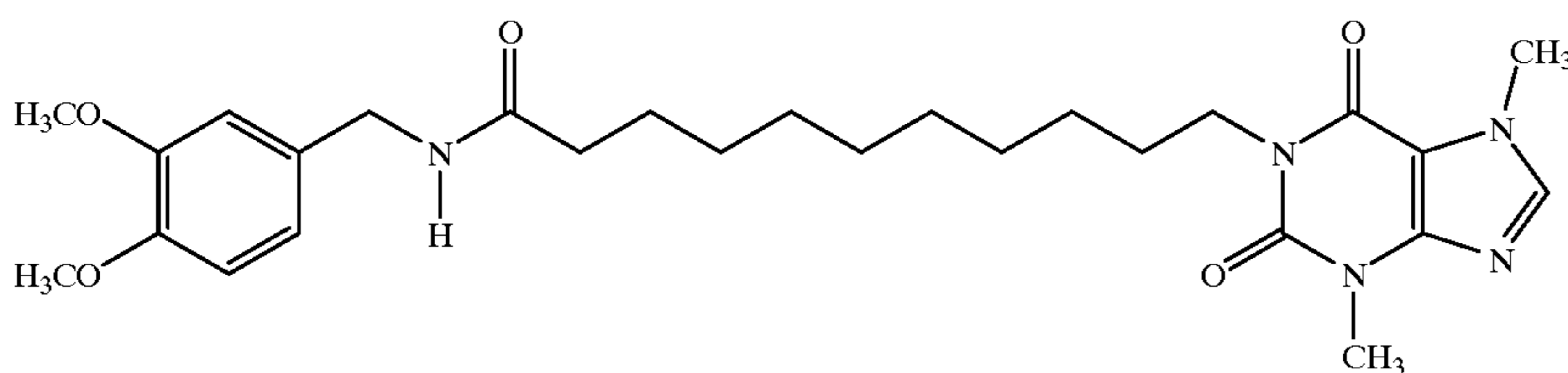
1-[N-(3,4-Dimethoxybenzyl)-11-yl-undecanoamide]-3,7-dimethylxanthine
