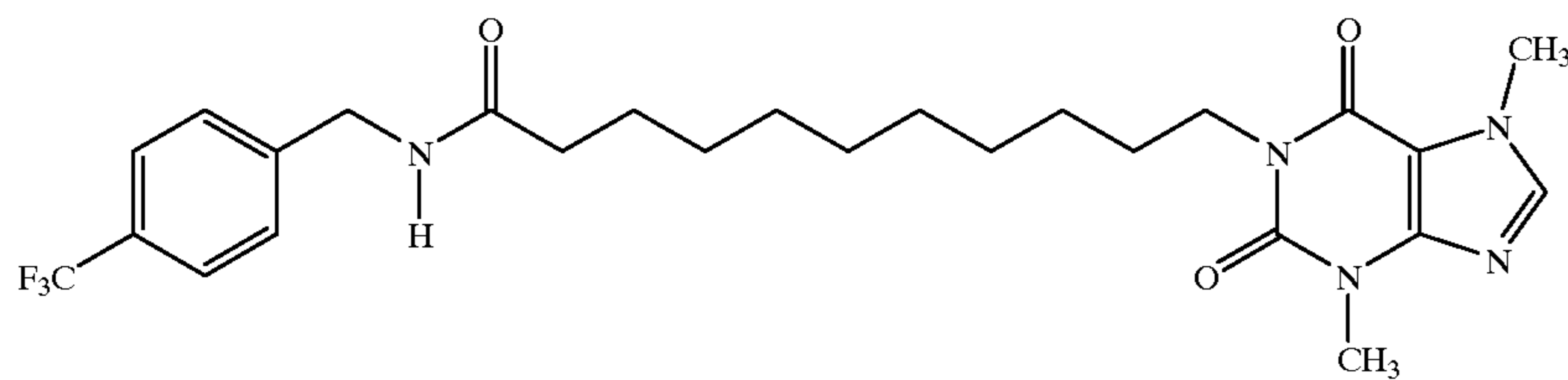
1-[N-(4-Trifluoromethylbenzyl)-11-yl-undecanamide]-3, 7-dimethylxanthine
