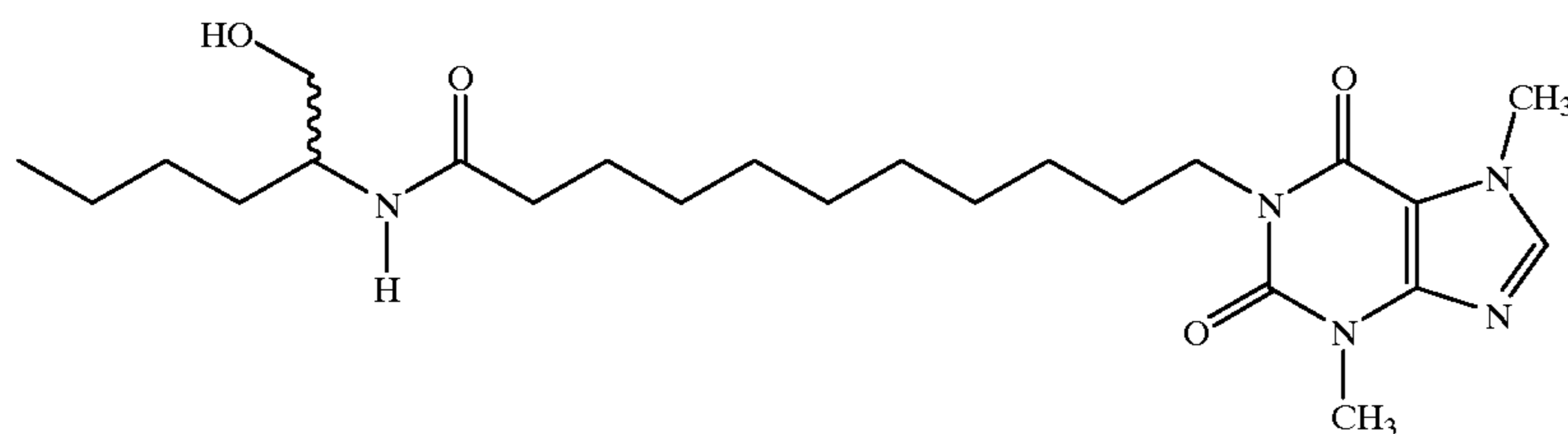
1-[N-(1-Hydroxymethyl)pentyl-11-yl-undecanamide]-3,7-dimethylxanthine
