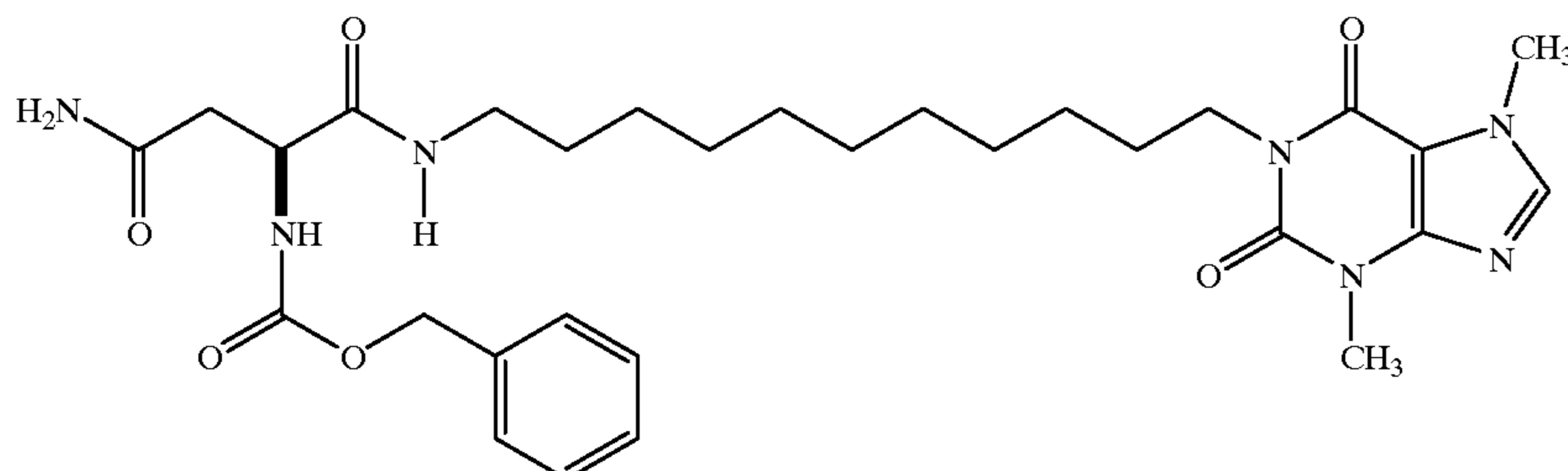
1-(11-[4-Amino-2-carbobenzyloxyamino-4-oxobutyronamido]undecyl)-3,7-dimethylxanthine
