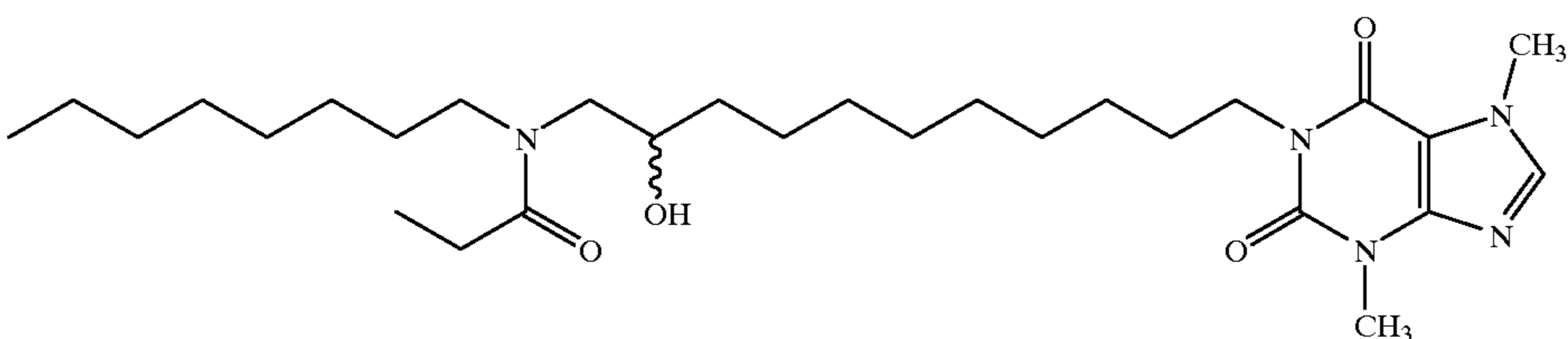
1-[11-(N-Octyl propionamido)-10-hydroxyundecyl]-3,7-dimethylxanthine
