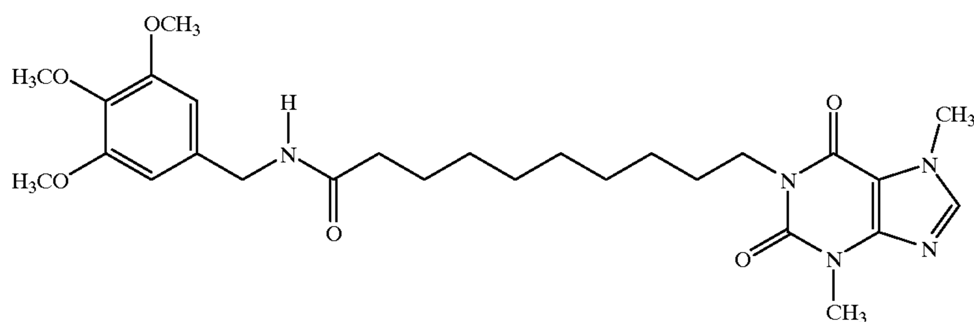
1-[N-(3,4,5-Trimethoxybenzyl)-10-yl-decanamide]-3,7-dimethylxanthine
