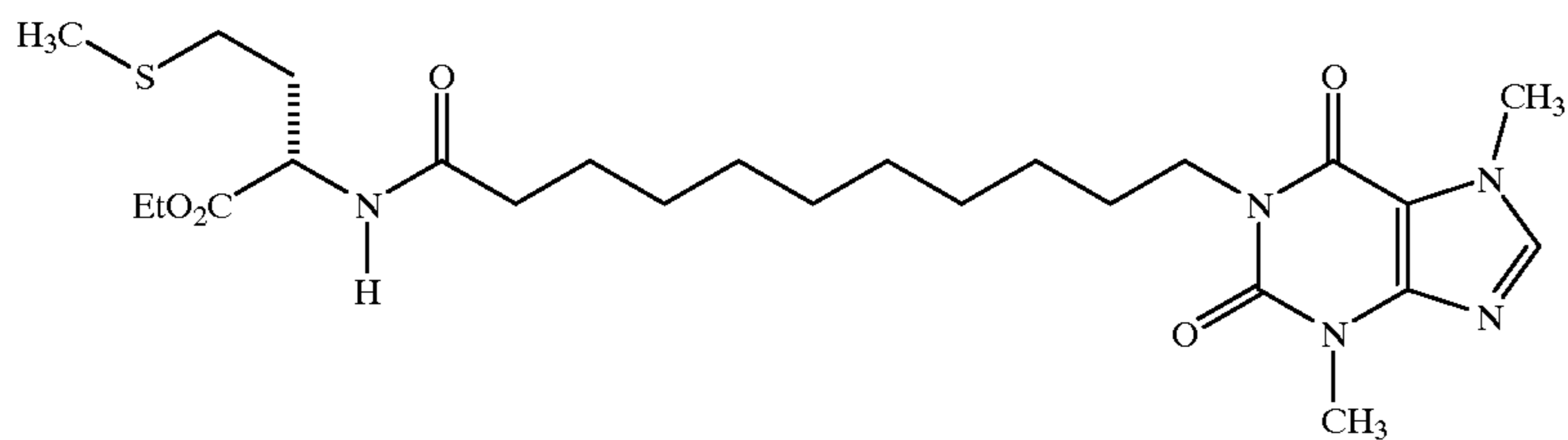
1-[11-(1-Ethoxycarbonyl-3-methylthiopropylamino)-11-oxoundecyl]-3,7-dimethylxanthine
