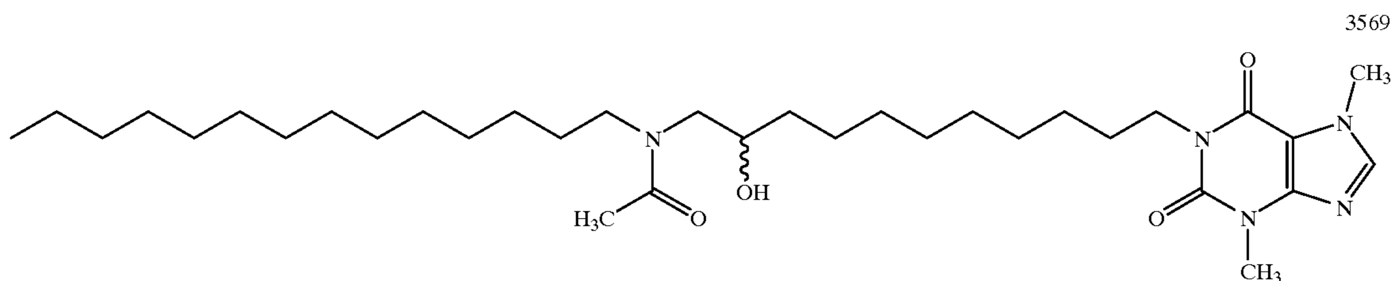
1-[11-(N-Tetradecylacetamido)-10-hydroxyundecyl]-3, 7-dimethylxanthine
