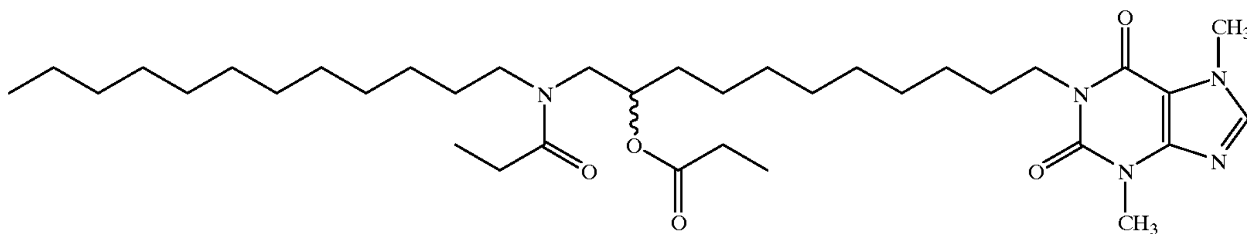
1-[11-(N-Dodecyl propionamido)-10-propionylundecyl]-3,7-dimethylxanthine
