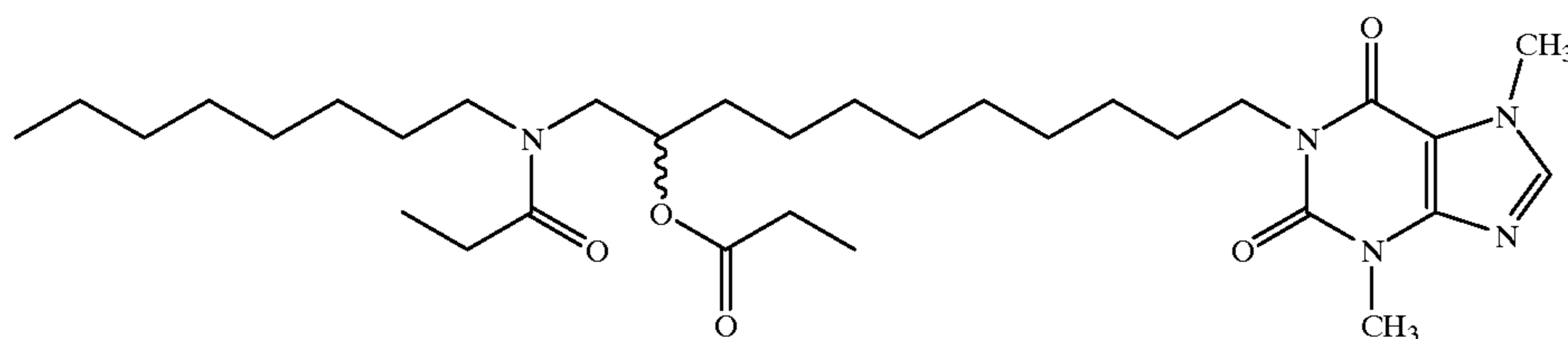
1-[11-(N-Octyl propionamido)-10-propionoxyundecyl]-3,7-dimethylxanthine
