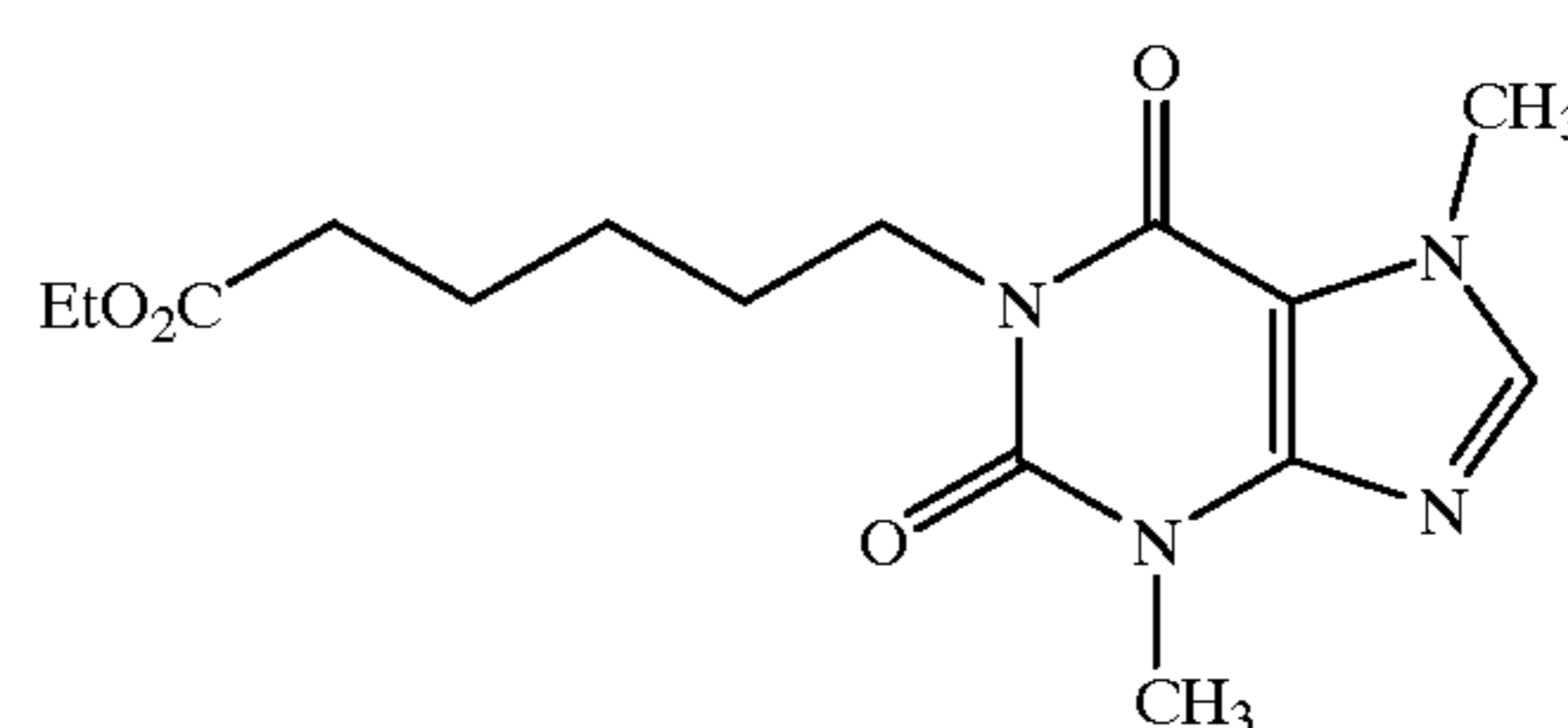
1-(Ethyl 6-yl-hexanoate)-3,7-dimethylxanthine
