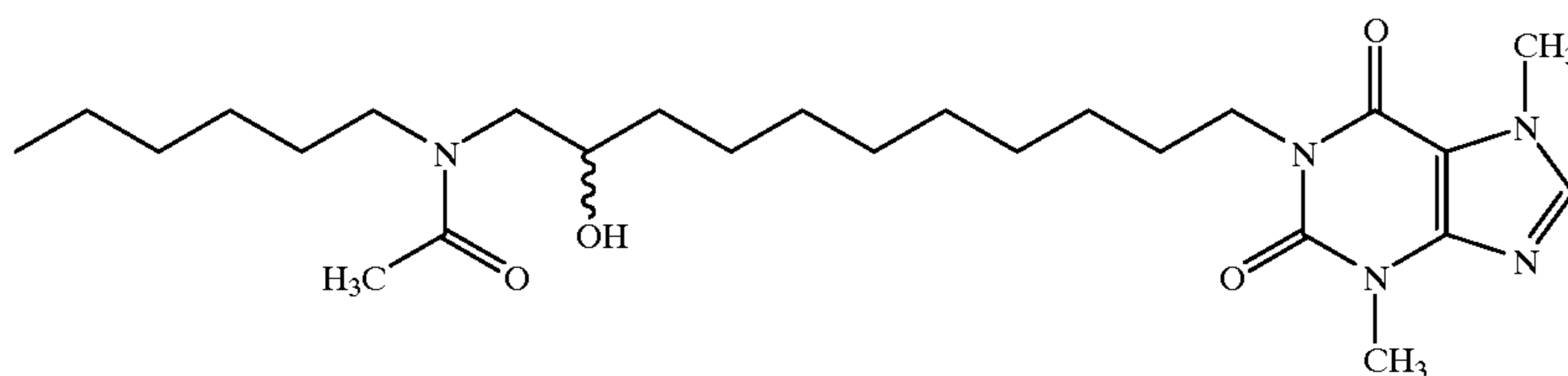
1-[11-(N-Hexylacetamido)-10-hydroxyundecyl]-3,7-dimethylxanthine
