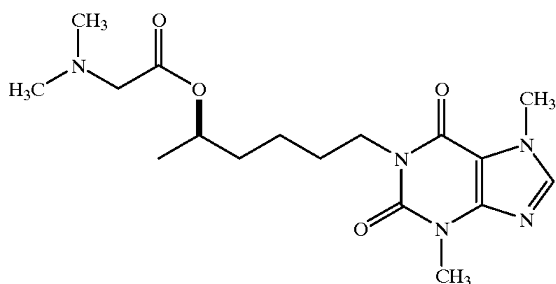
R-1-(5-Hydroxy)hexyl)-3,7-dimethylxanthine N,N-dimethylglycinate
