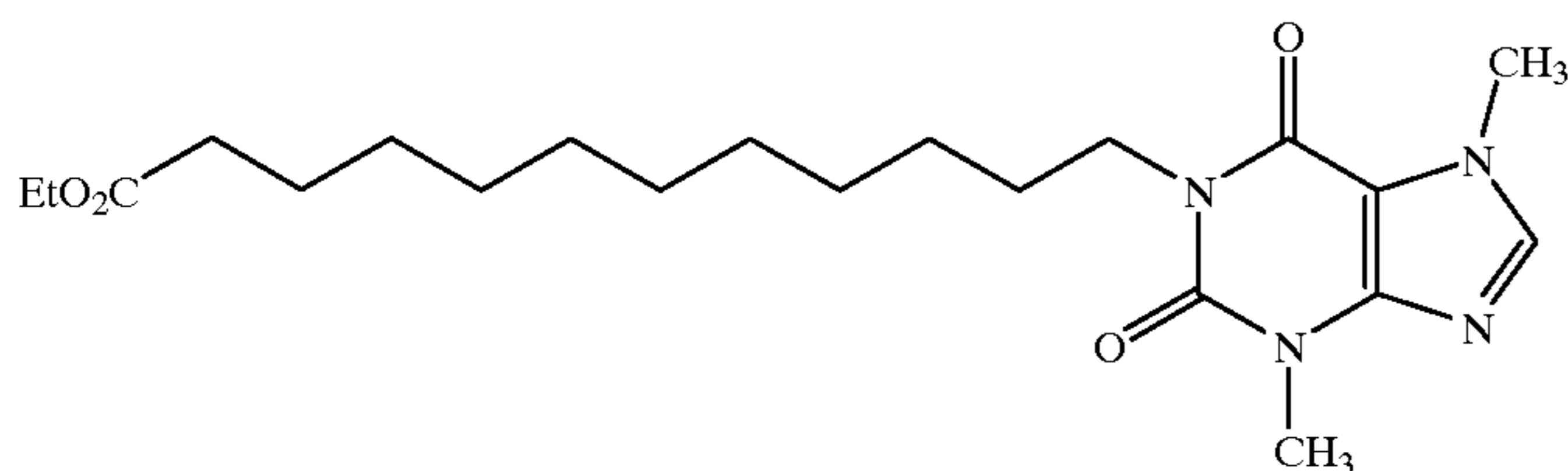
1-(Ethyl 12-yl-dodecanoate)-3,7-dimethylxanthine
