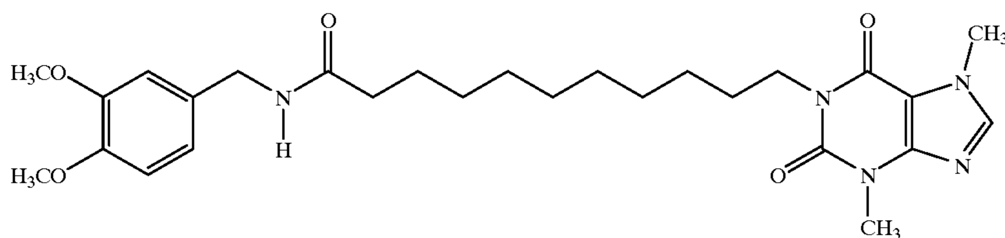
1-[N-(3,4-Dimethoxybenzyl)-11-yl-undecanoamide]-3,7-dimethylxanthine
