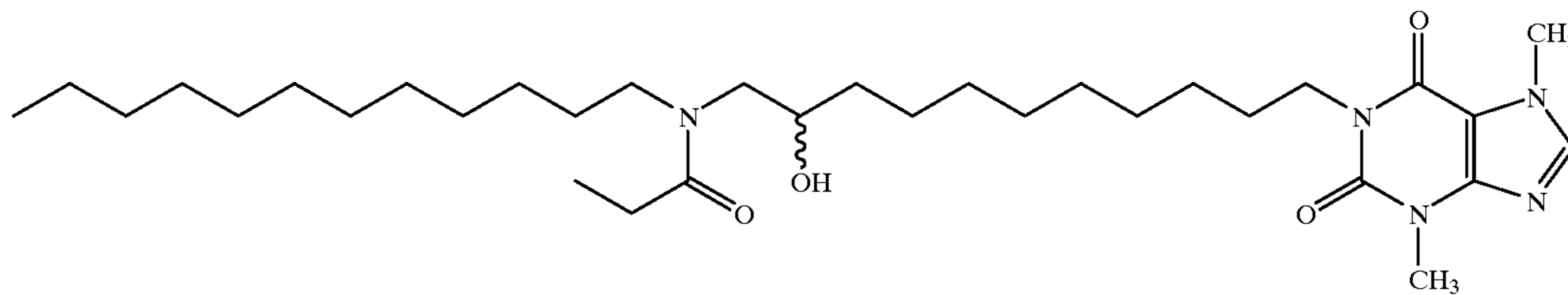
1-[11-(N-Dodecyl propionamido)-10-hydroxyundecyl]-3,7-dimethylxanthine
