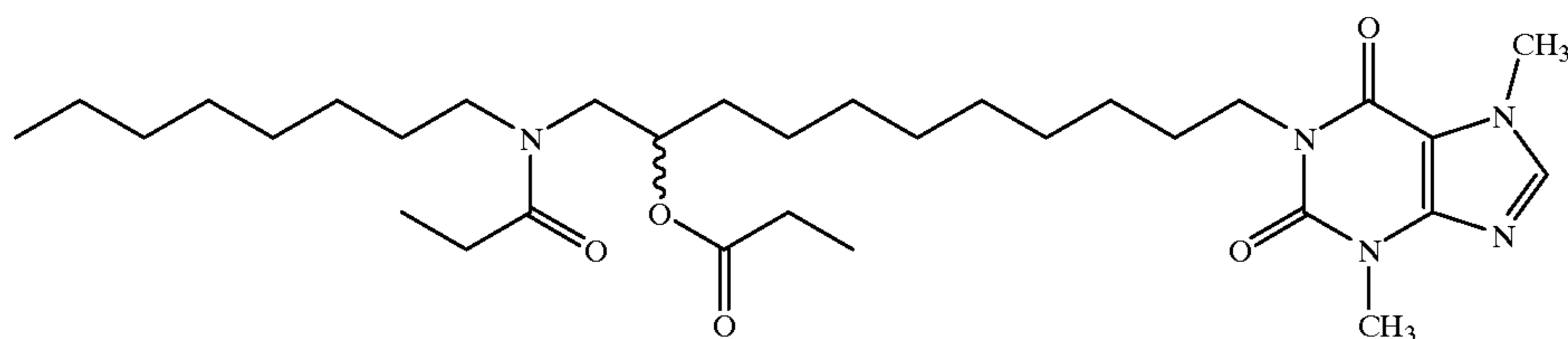
1-[11-(N-Octyl propionamido)-10-propionoxyundecyl]-3,7-dimethylxanthine
