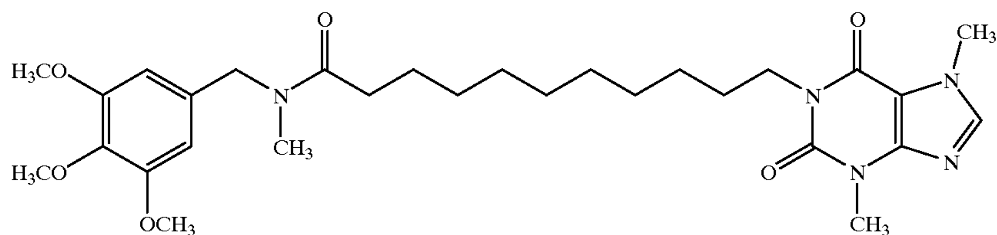
1-[N-Methyl-N-(3, 4, 5-trimethoxybenzyl)-11-yl-undecanamide]-3, 7-dimethylxanthine
