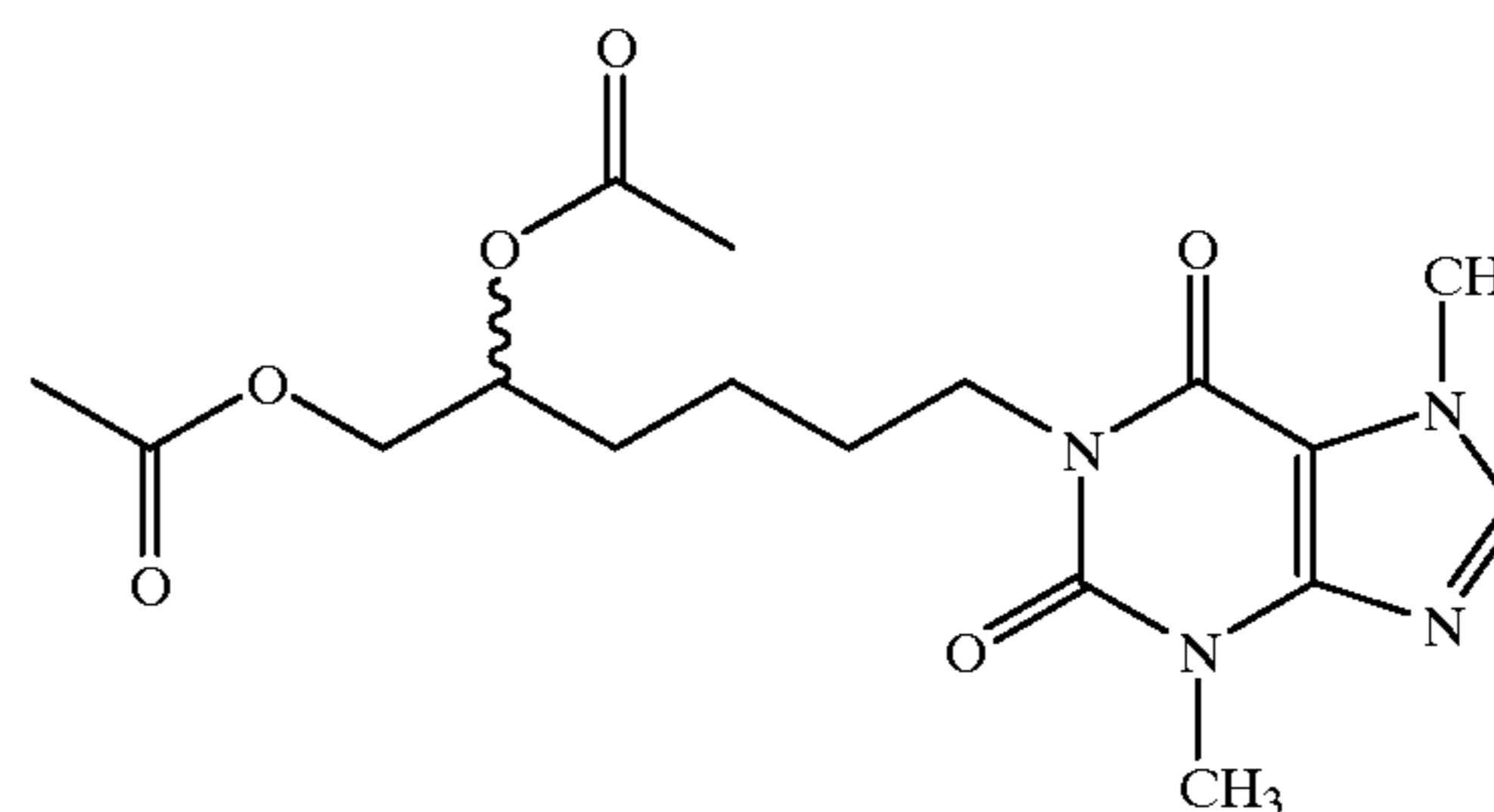
1-(5,6-Diacetoxyhexyl)-3,7-dimethylxanthine
