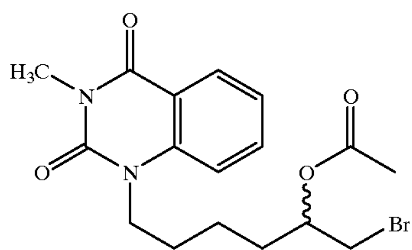
1-(5-Acetoxy-6-bromohexyl)-3-methylbenzoyleneurea
