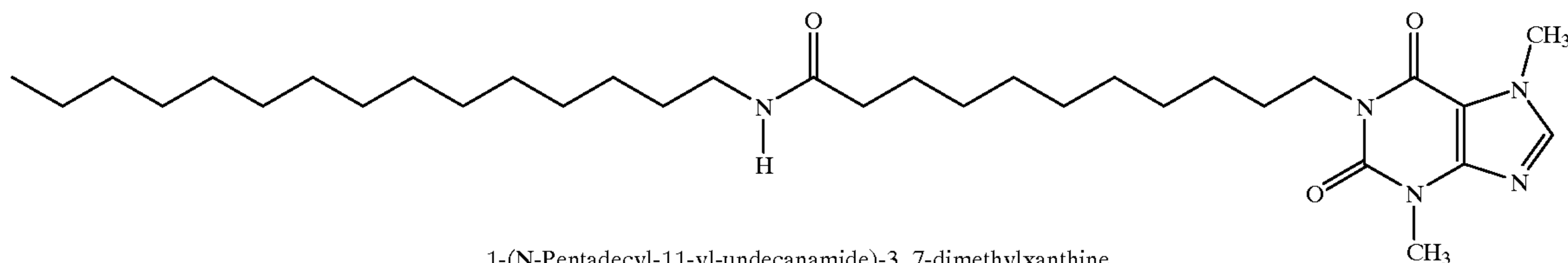
1-(N-Pentadecyl-11-yl-undecanamide)-3, 7-dimethylxanthine
