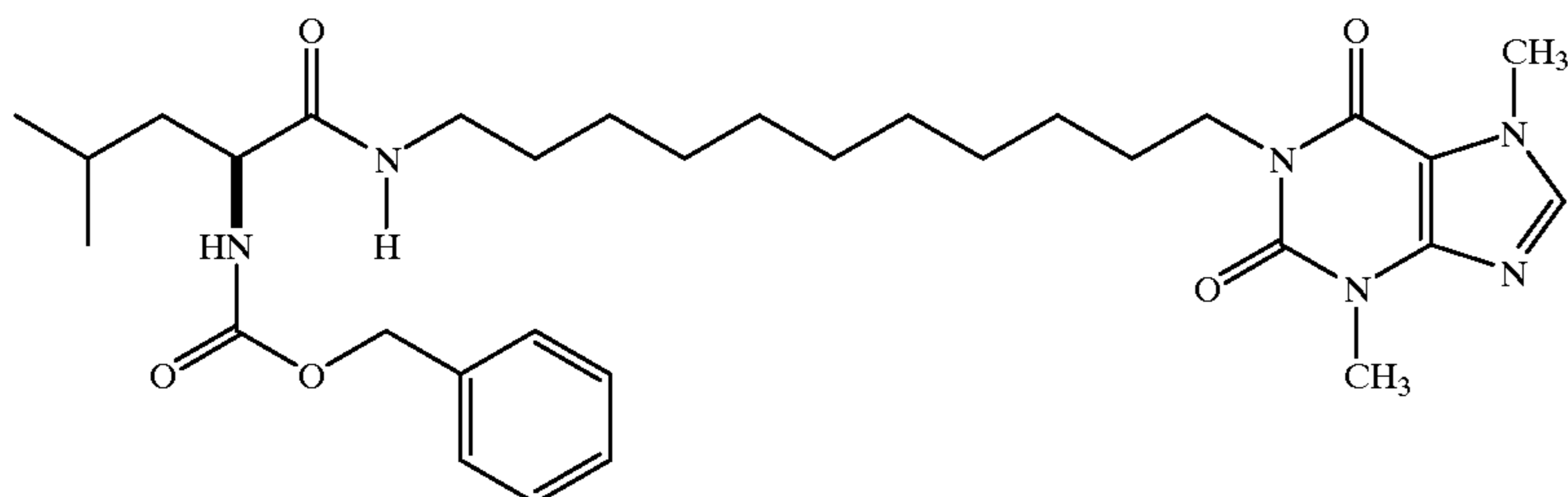
1-[11-(N-carbobenzyloxy)leucine]amidoundecyl]-3, 7-dimethylxanthine
