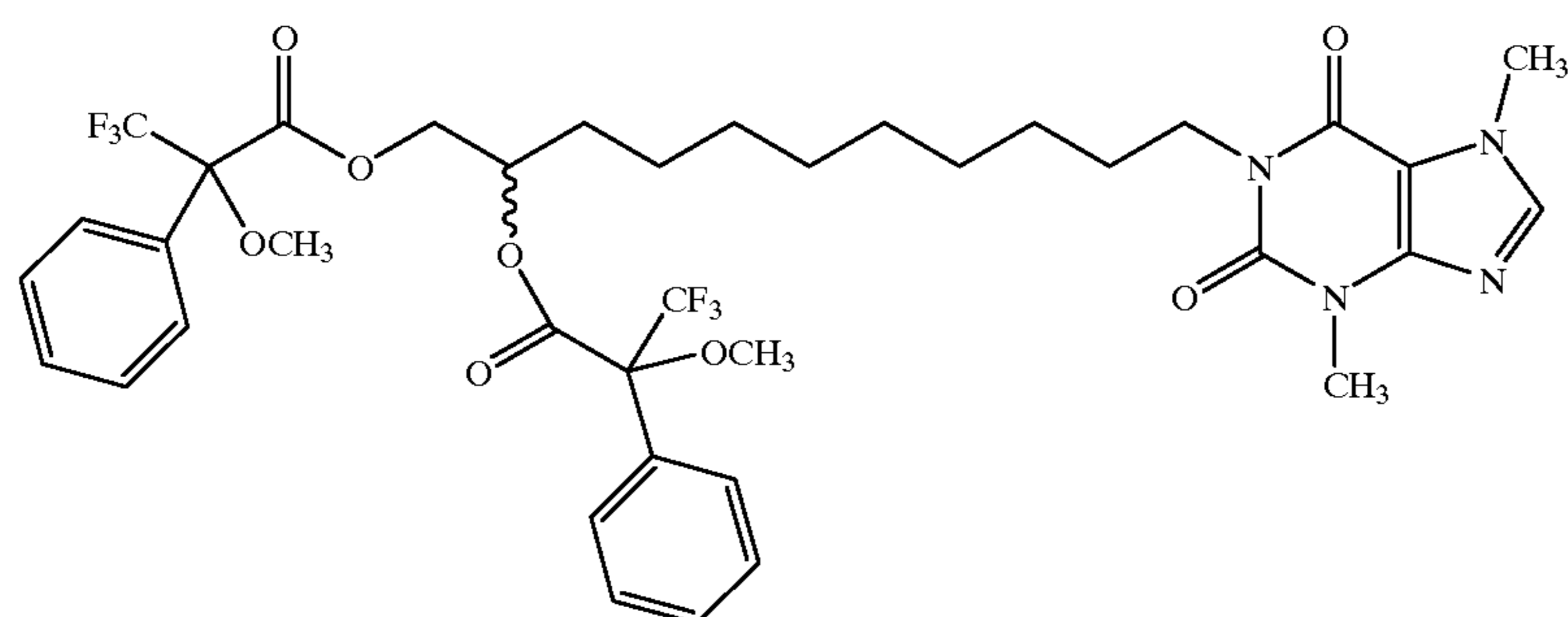
1-[11, 10-di( \alpha -methoxy- \alpha -(trifluoromethyl)phenylacetoxy)undecyl]-3, 7-dimethylxanthine
