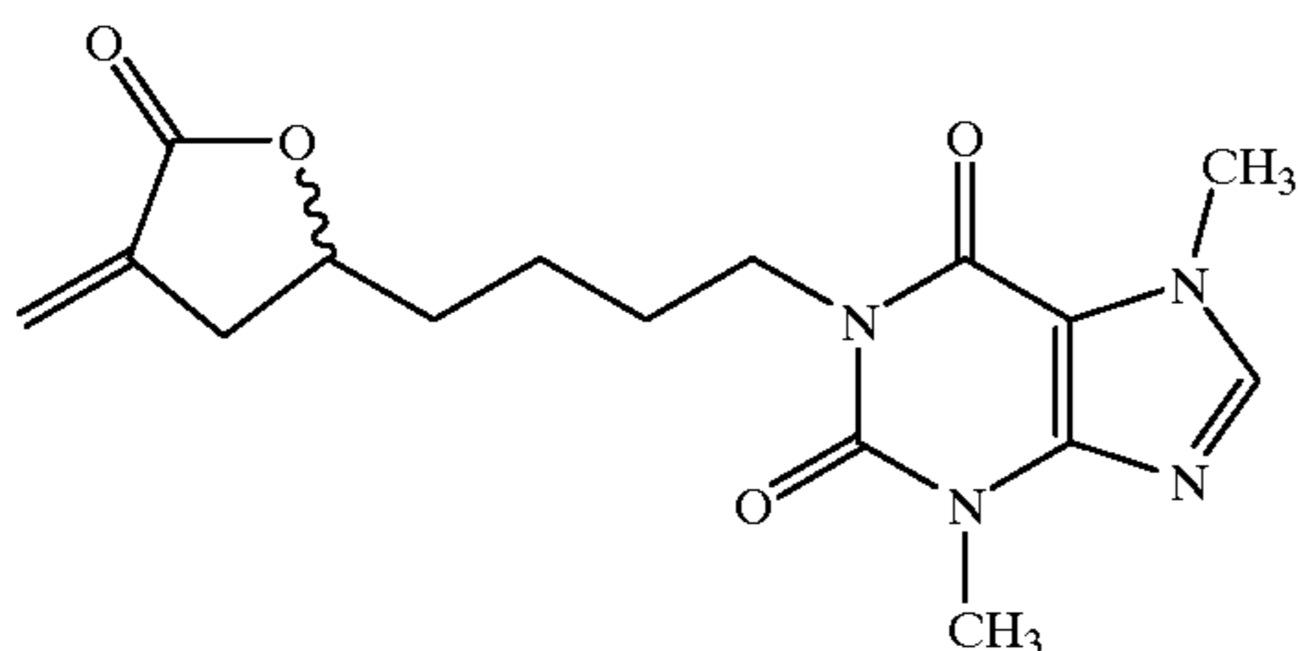
1-(5-hydroxy-7-carboxy-7-octenyl)-3,7-dimethylxanthine-γ-lactone
