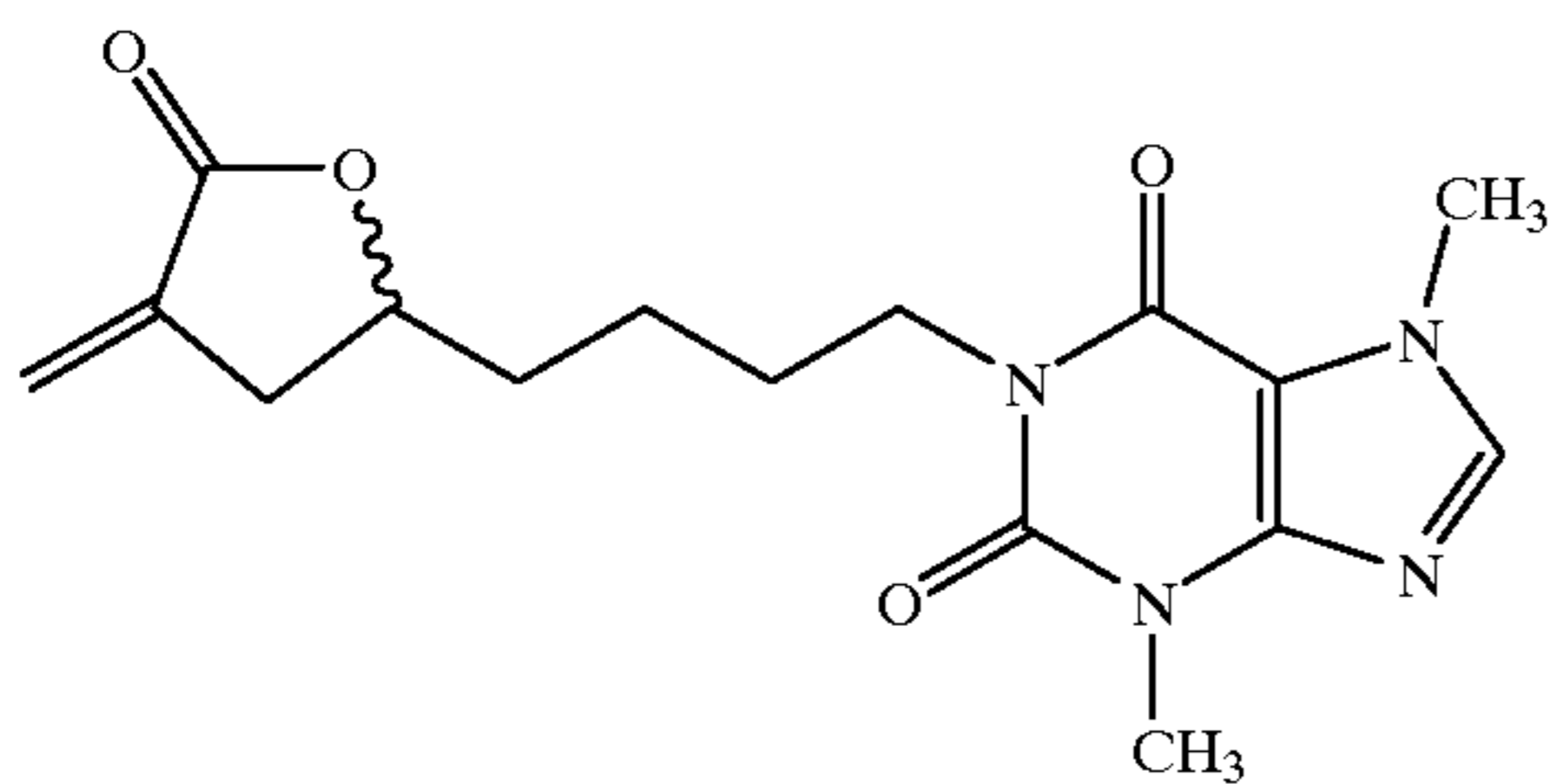
1-(5-hydroxy-7-carboxy-7-octenyl)-3,7-dimethylxanthine- \gamma -lactone
