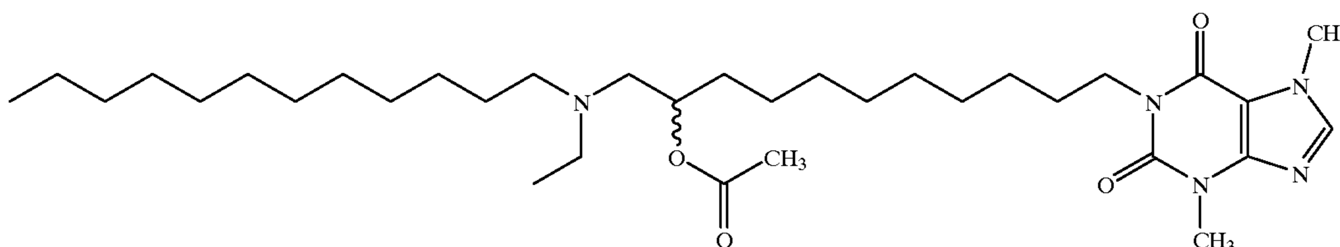
1-(11-Dodecylethylamino-10-acetoxyundecyl)-3,7-dimethylxanthine
