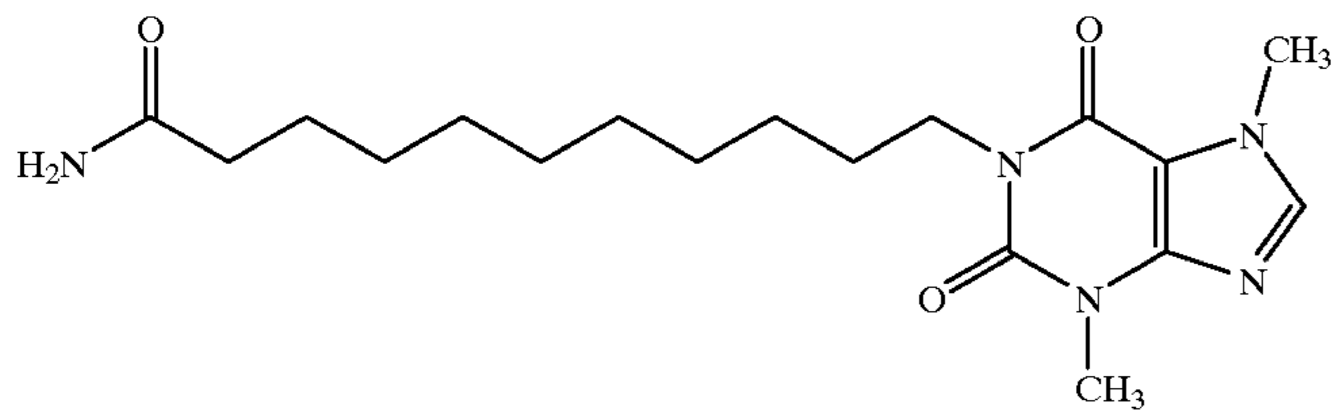
1-(11-yl-Undecanamide)-3,7-dimethylxanthine
