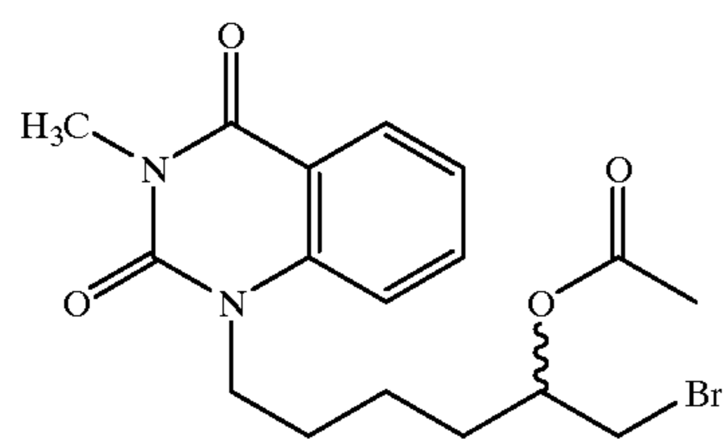
1-(5-Acetoxy-6-bromohexyl)-3-methylbenzoyleneurea
