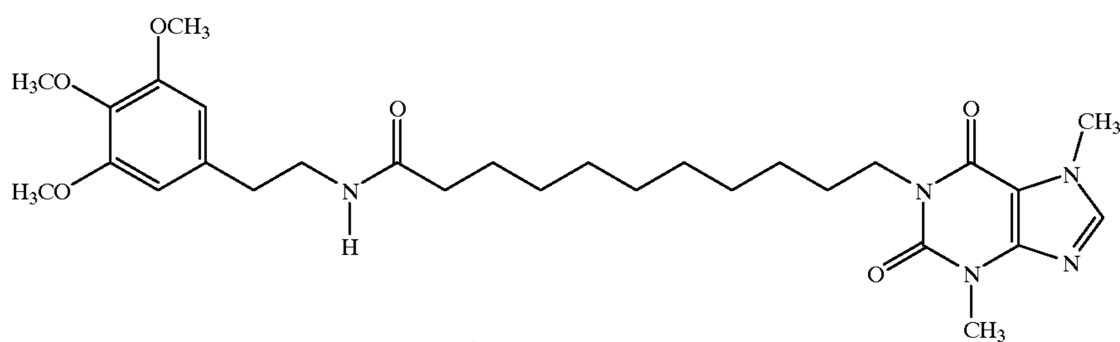
1-[N-(3,4,5-Trimethoxyphenethyl)-11-yl-undecanamide]-3,7-dimethylxanthine
