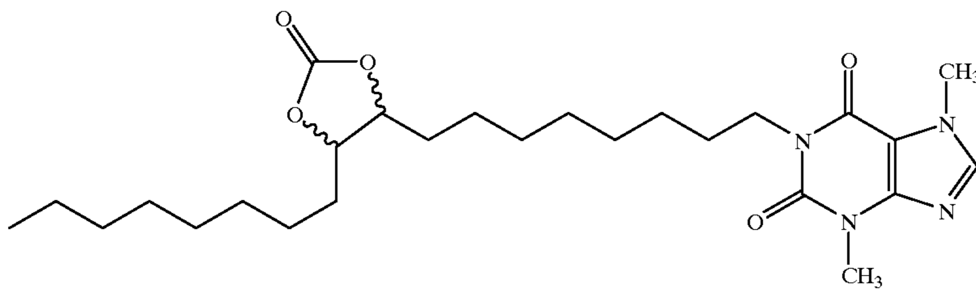
1-(9,10-Carbonyldioxyoctadecyl)-3,7-dimethylxanthine
