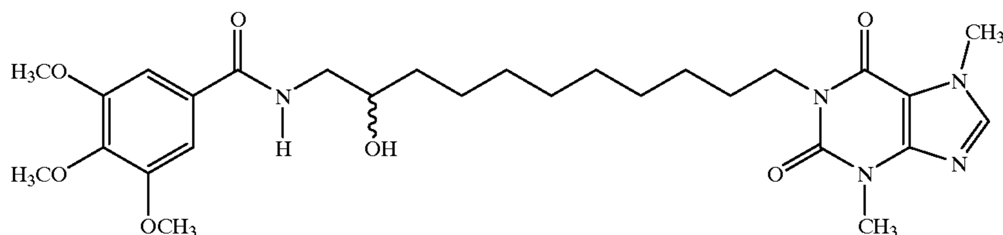
1-[11-(3,4,5-Trimethoxybenzamido)-10-hydroxyundecyl]-3,7-dimethylxanthine
