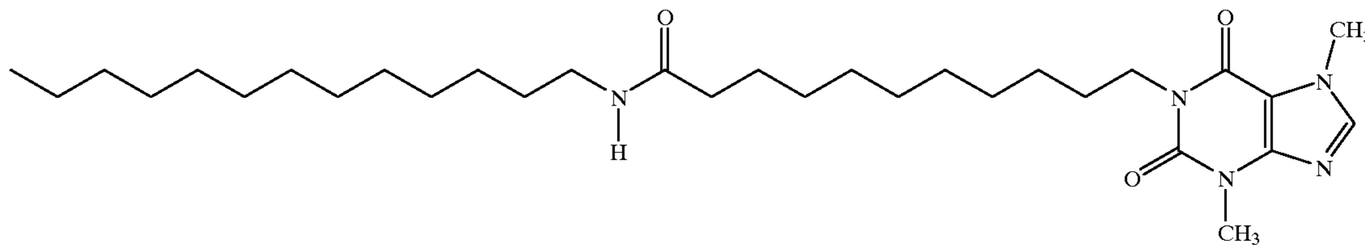
1-(N-Tridecyl-11-yl-undecanamide)-3, 7-dimethylxanthine
