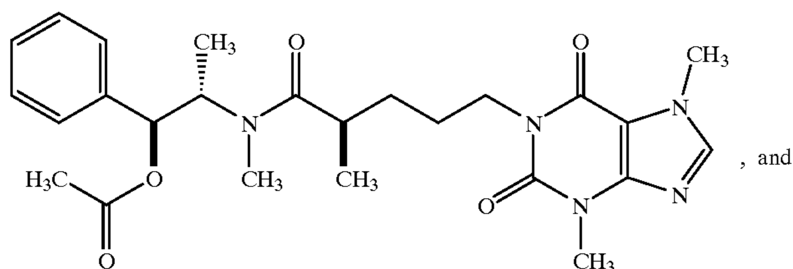
(1'S, 2'S, 4R)-1-(5-[N-(2-Acetoxy-1-methyl-2-phenylethyl)-N-methylamino]-4-methyl-5-oxopentyl)-3,7-dimethylxanthine
