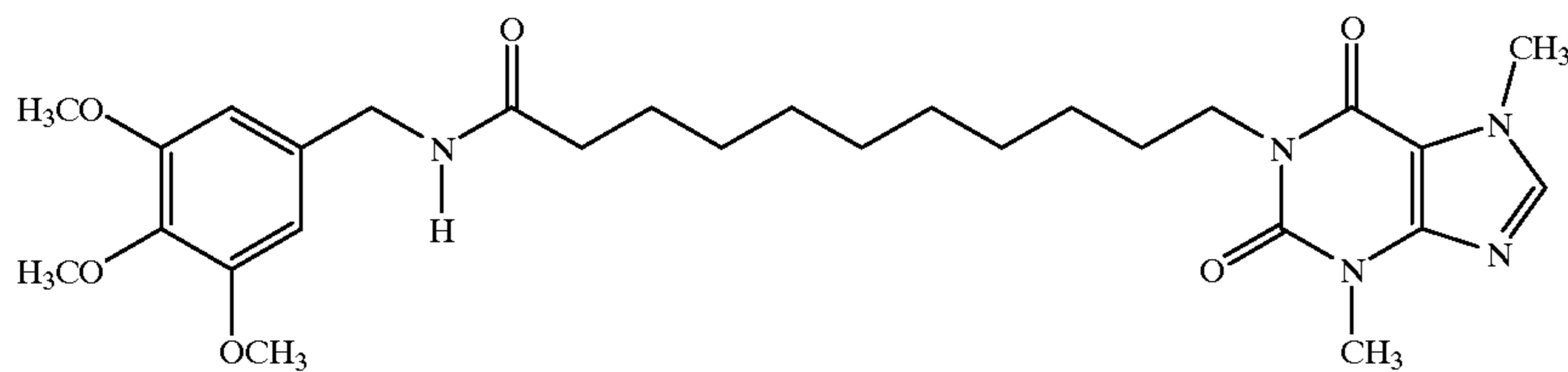
1-[N-(3,4,5-Trimethoxybenzyl)-11-yl-undecanamide]-3,7-dimethylxanthine
