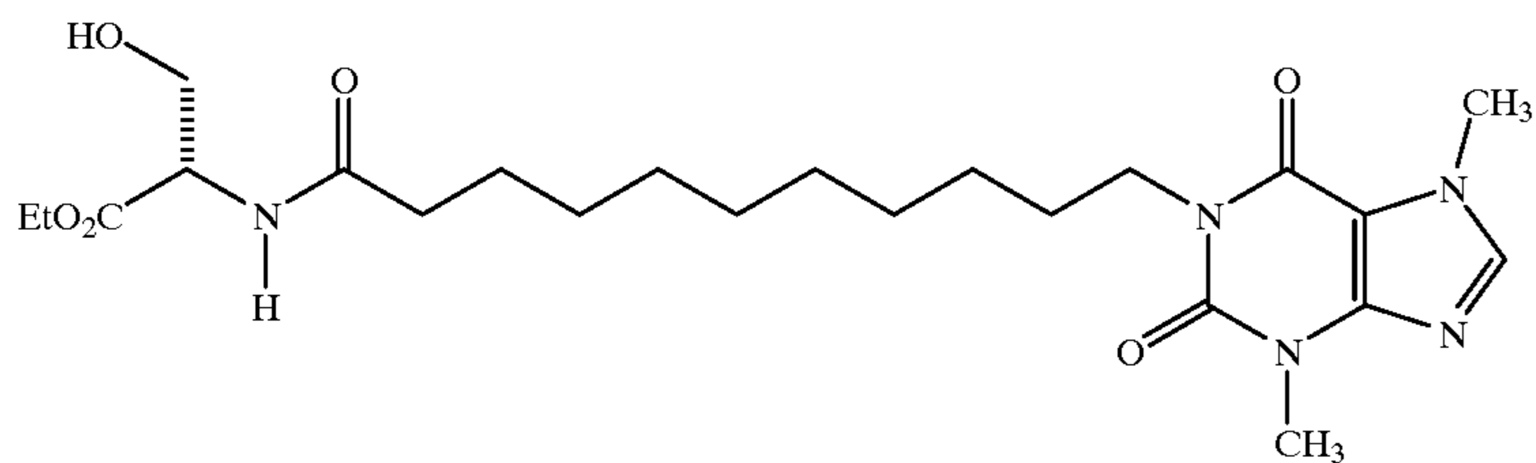
1-[11-(1-Ethoxycarbonyl-2-hydroxyethylamino)-11-oxoundecyl]-3,7-dimethylxanthine
