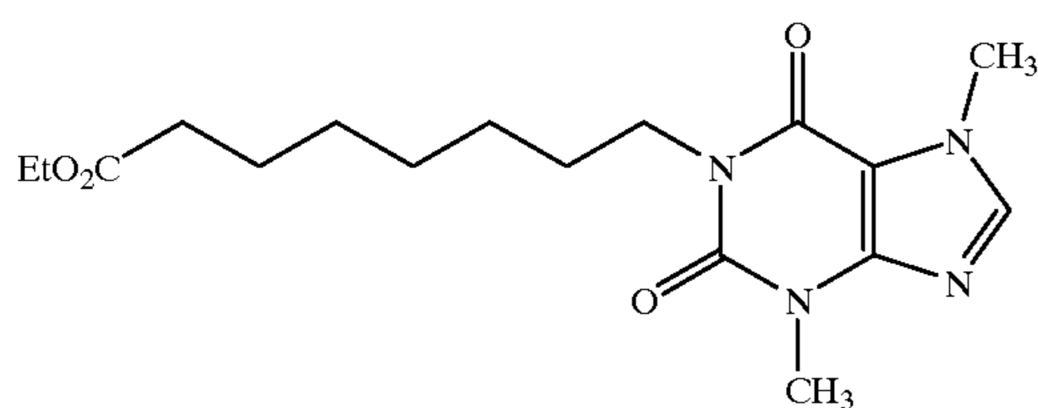
1-(Ethyl 8-yl-octanoate)-3,7-dimethylxanthine
