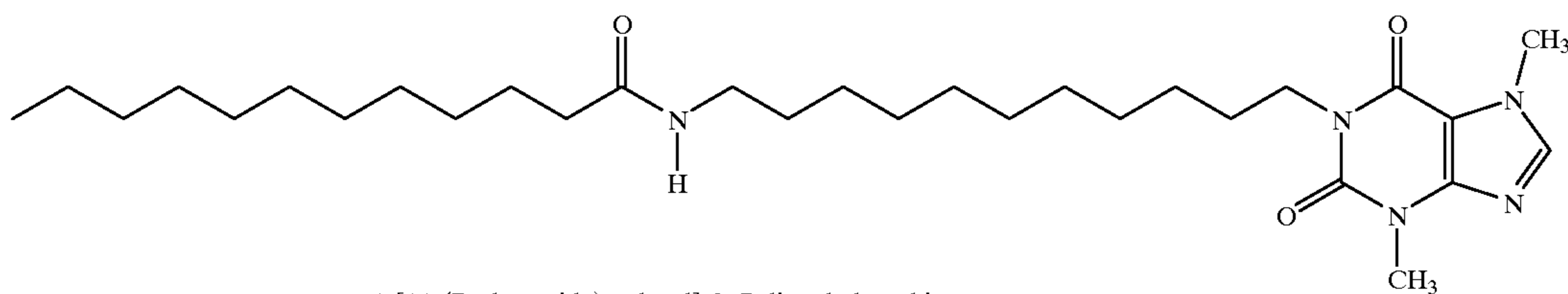
1-[11-(Dodecamido)undecyl]-3,7-dimethylxanthine
