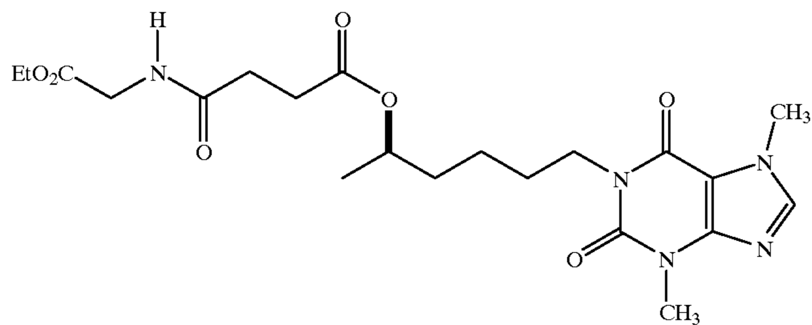
R-1-(5-Hydroxyhexyl)-3,7-dimethylxanthine ethyl glycyl succinate
