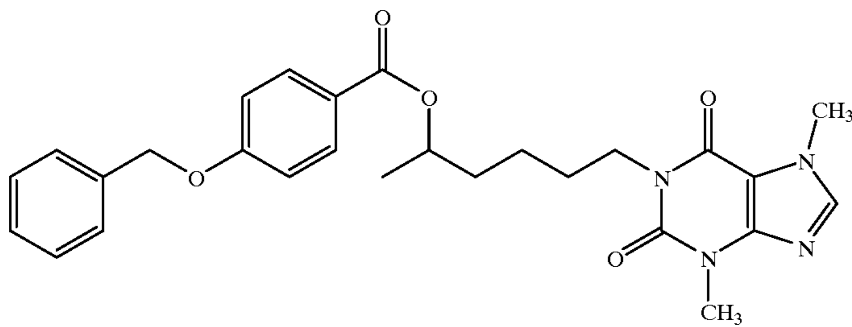
R-1-(5-(4'-benzyloxybenzoyloxy)hexyl)-3,7-dimethylxanthine
