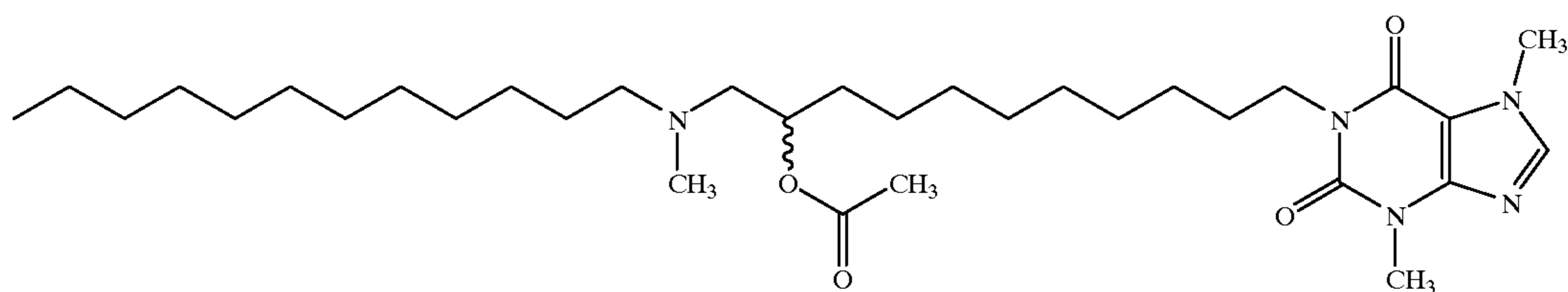
1-[11-(N-Methyl-N-dodecylamino)-10-acetoxyundecyl]-3, 7-dimethylxanthine
