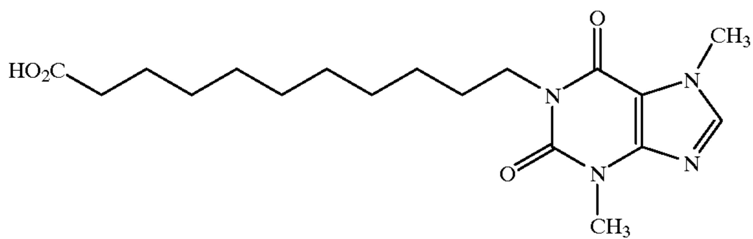
1-[11-yl-Undecanoic acid]-3, 7-dimethylxanthine
