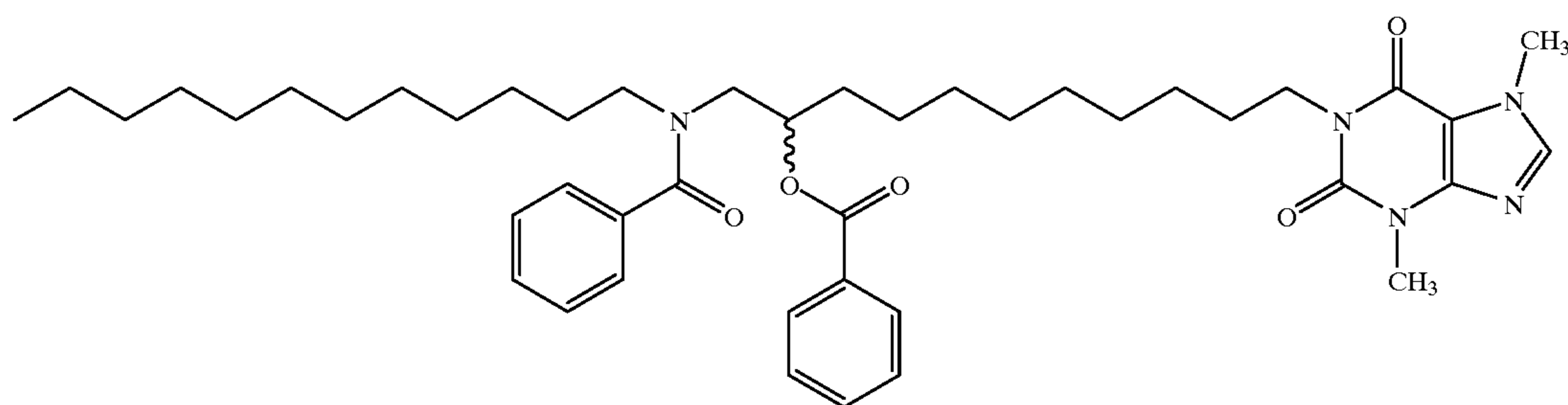
1-[11-(N-Dodecyl benzamido)-10-benzoylundecyl]-3,7-dimethylxanthine
