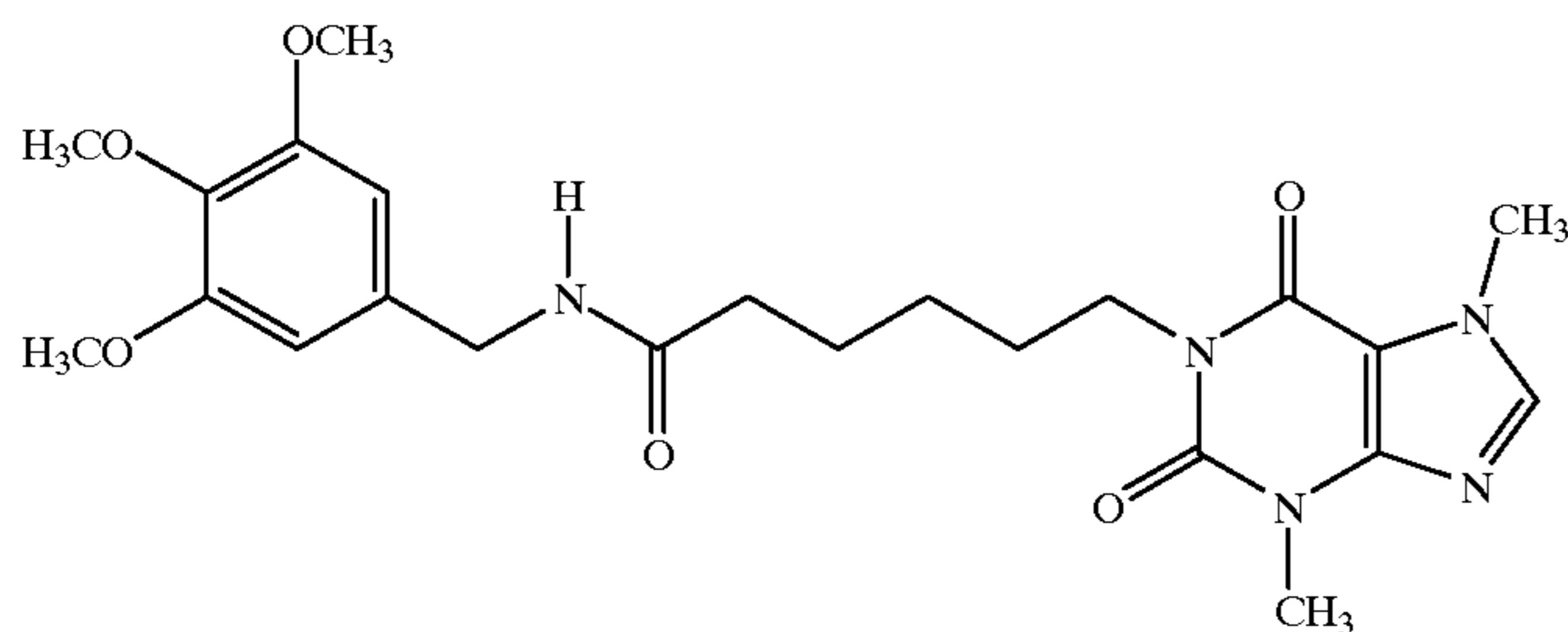
1-[N-(3, 4, 5-Trimethoxybenzyl)-6-yl-hexanamide]-3, 7-dimethylxanthine
