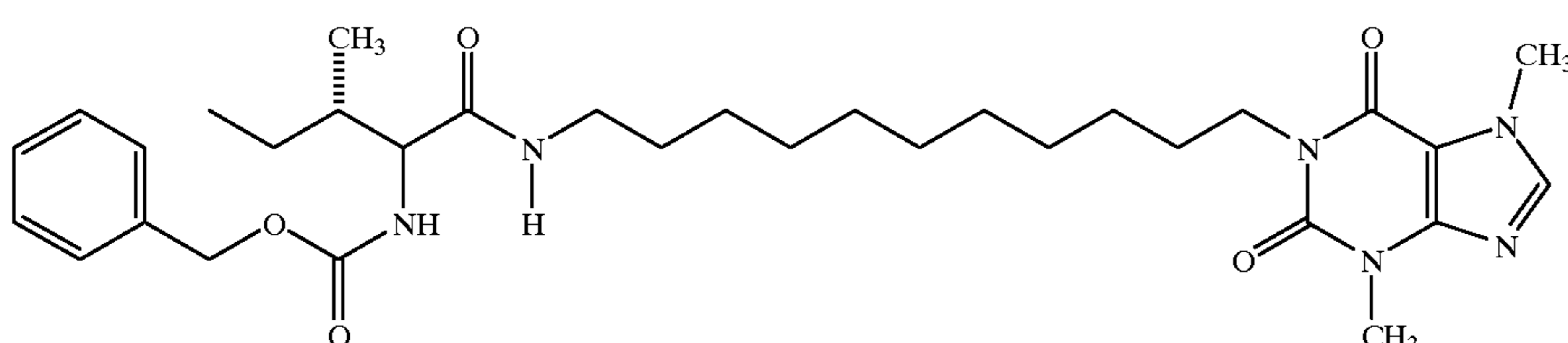
1-[N-(N-carbobenzyloxy isoleucine)-11-yl-undecanoamide]-3, 7-dimethylxanthine
