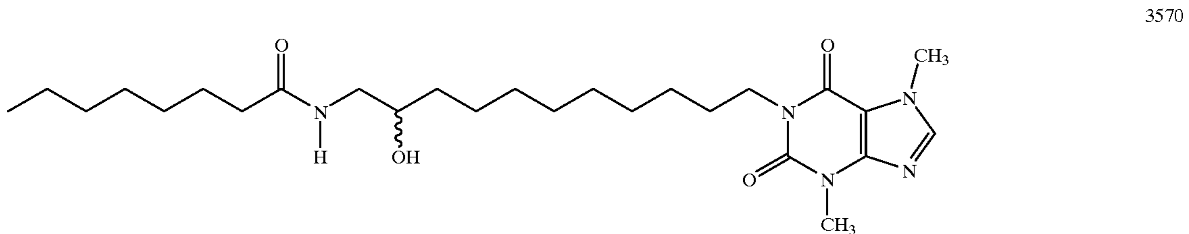
1-[11-Octanoamido-10-hydroxyundecyl)-3, 7-dimethylxanthine
