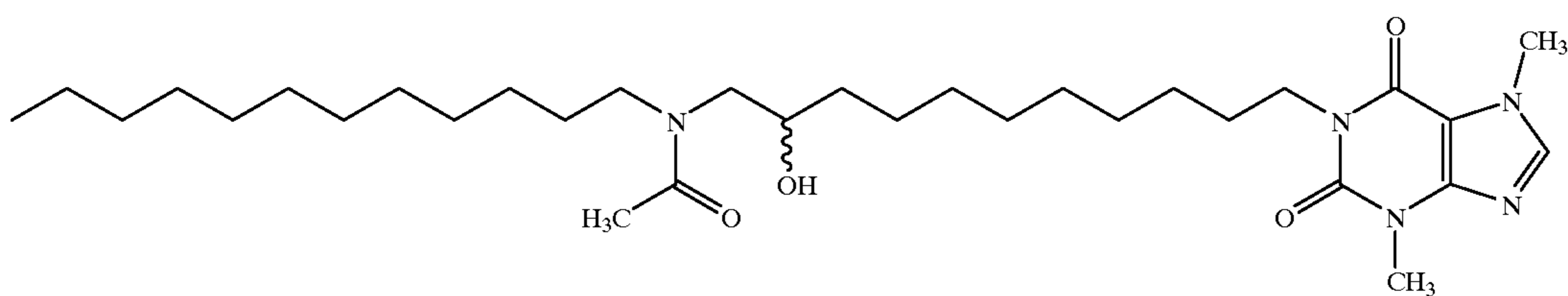
1[11-(N-Dodecylacetoamido)-10-hydroxyundecyl]-3,7-dimethylxanthine
