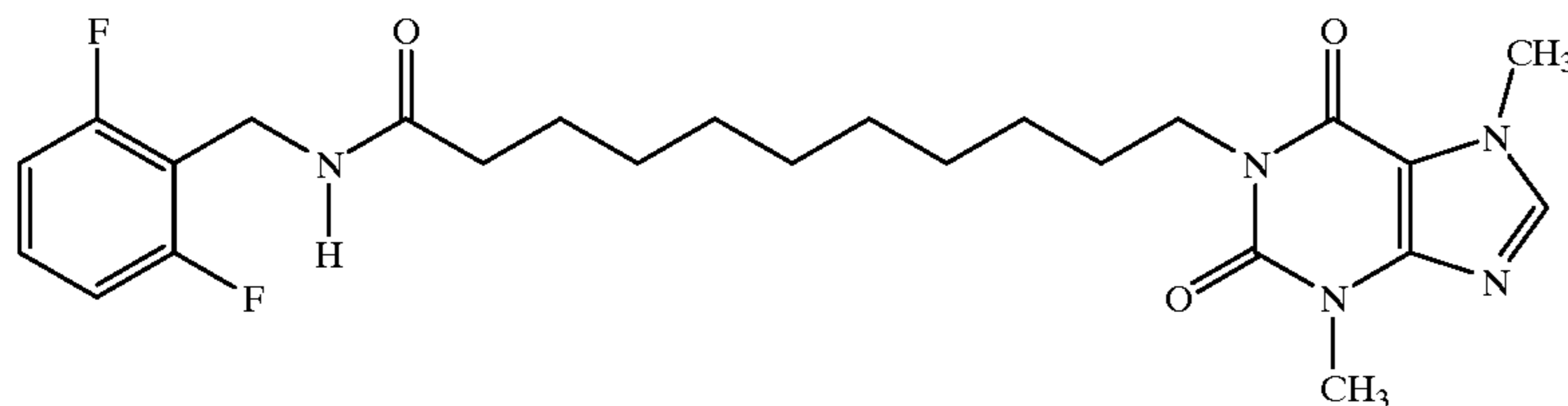
1-[N-(2,6-Difluorobenzyl)-11-yl-undecanoamide]-3,7-dimethylxanthine
