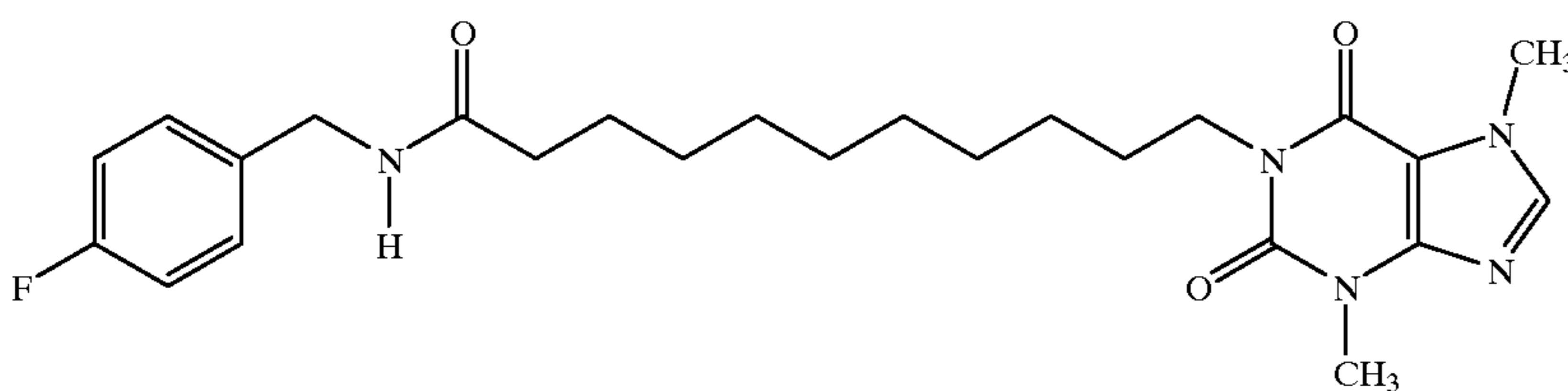
1-[N-(4-Fluorobenzyl)-11-yl-undecanamide]-3,7-dimethylxanthine
