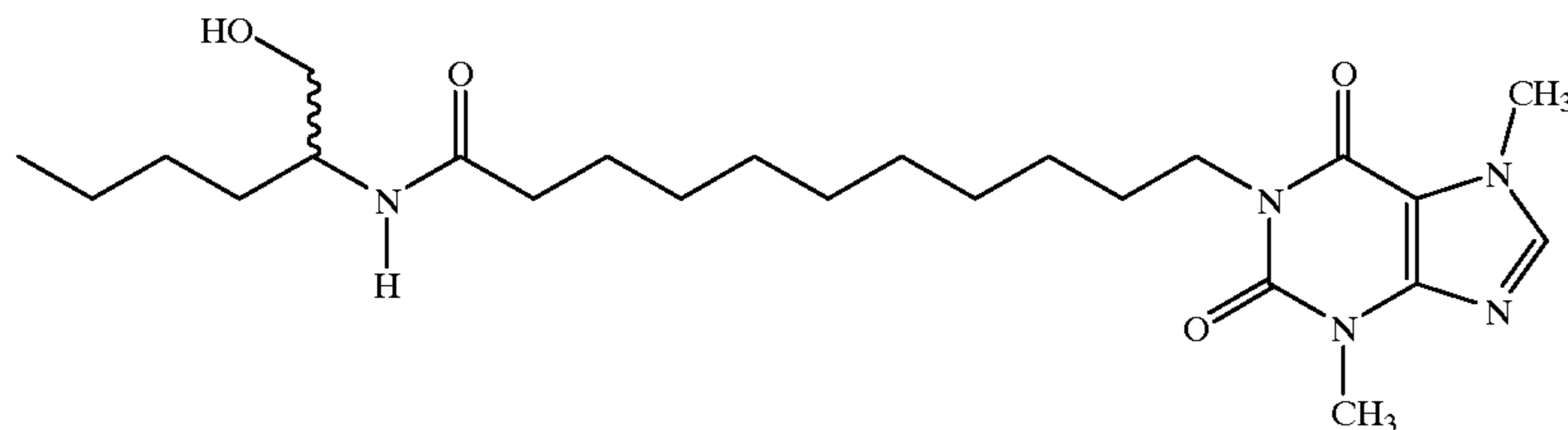
1-[N-(1-Hydroxymethyl)pentyl-11-yl-undecanamide]-3,7-dimethylxanthine
