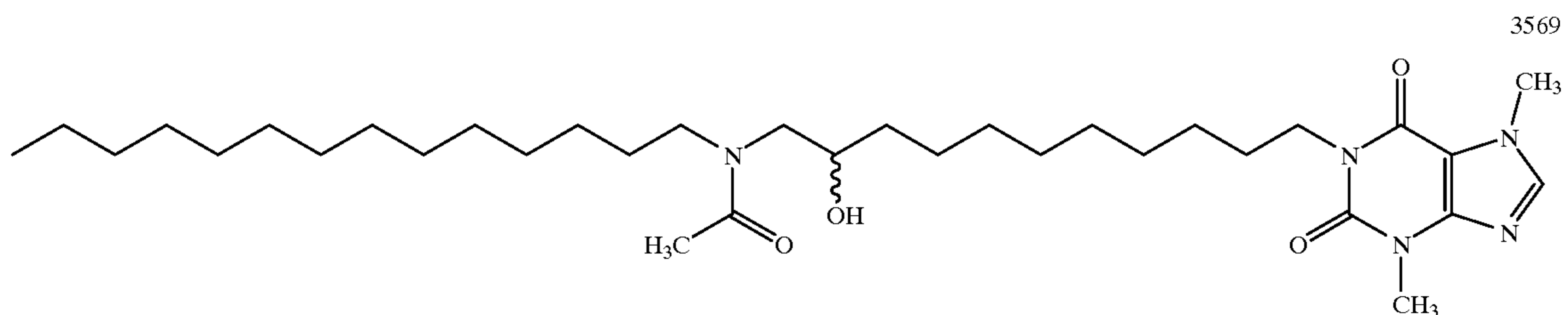
1-[11-(N-Tetradecylacetamido)-10-hydroxyundecyl]-3, 7-dimethylxanthine
