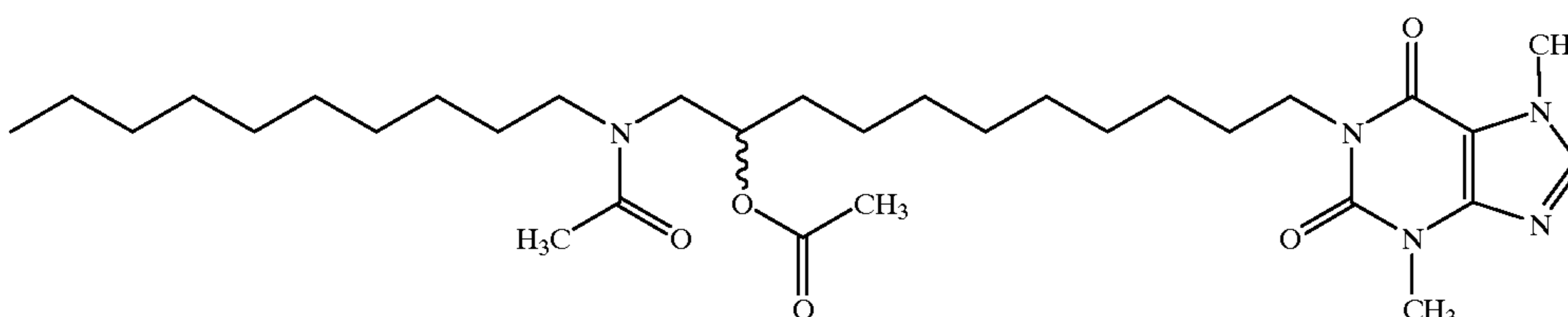
1-[11-(N-Decylacetamido)-10-acetoxyundecyl]-3, 7-dimethylxanthine
