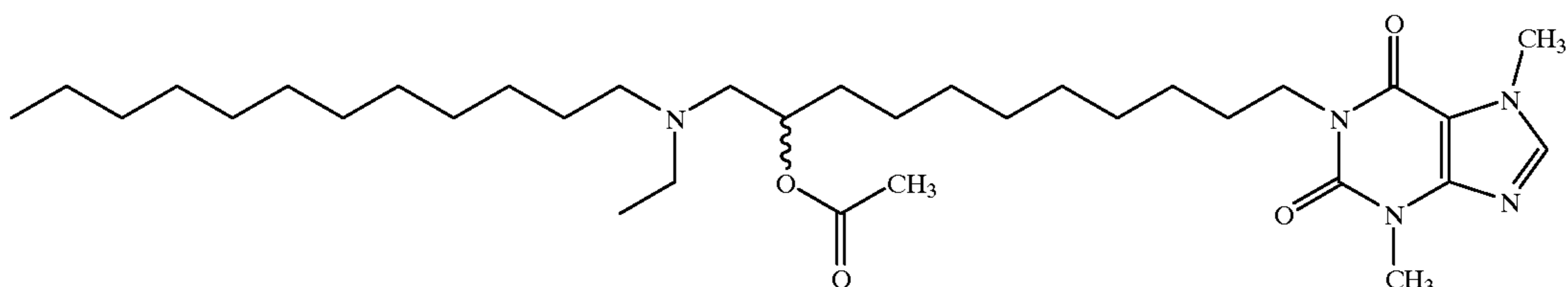
1-(11-Dodecylethylamino-10-acetoxyundecyl)-3,7-dimethylxanthine
