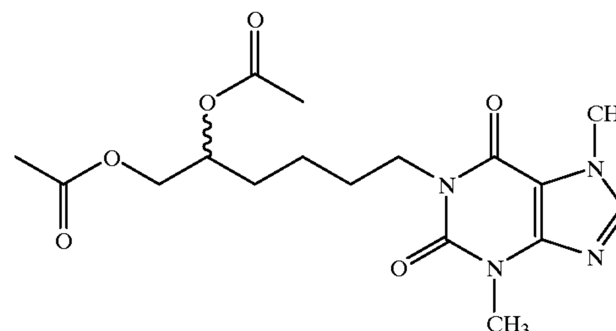
1-(5,6-Diacetoxyhexyl)-3,7-dimethylxanthine
