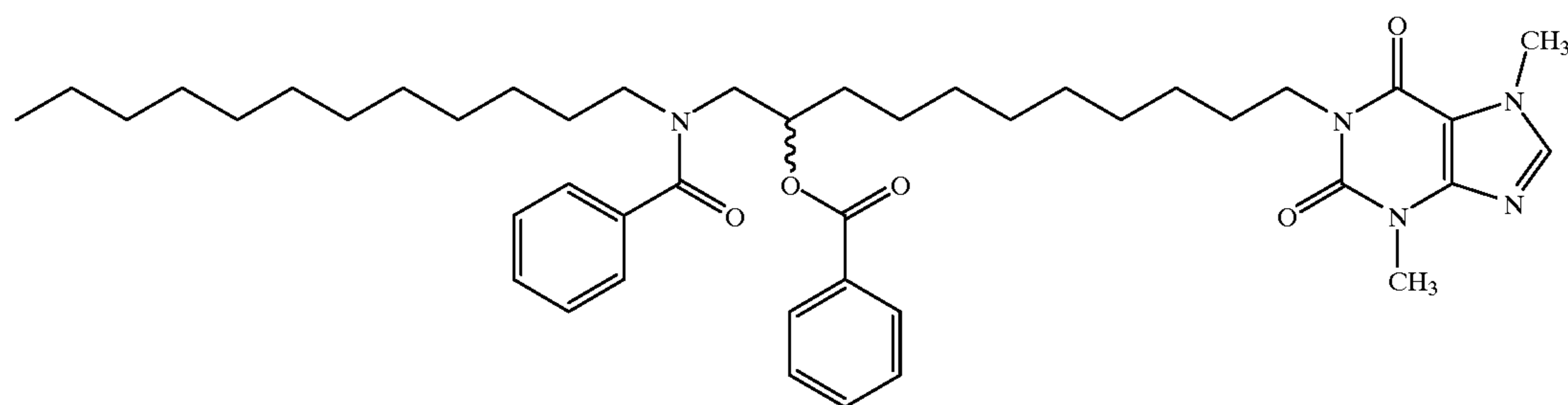
1-[11-(N-Dodecyl benzamido)-10-benzoylundecyl]-3,7-dimethylxanthine
