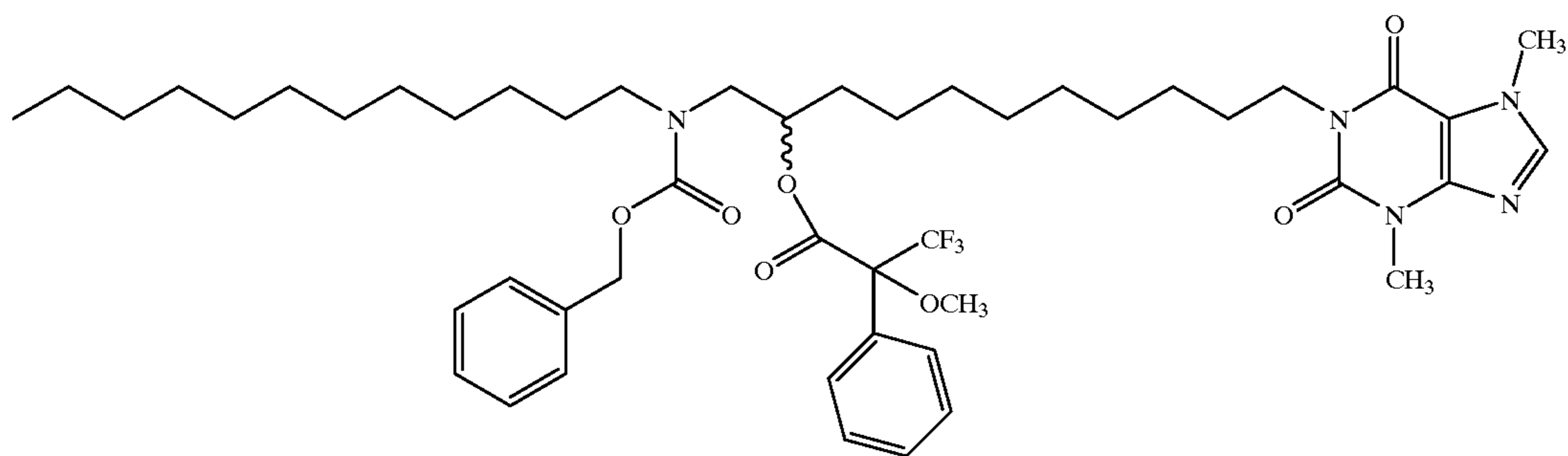
1-[11-Dodecylamino(N-benzyloxycarbonyl)-10-( \alpha -methoxy- \alpha -trifluoromethyl)-phenylacetoxy]-undecyl]-3, 7-dimethylxanthine
