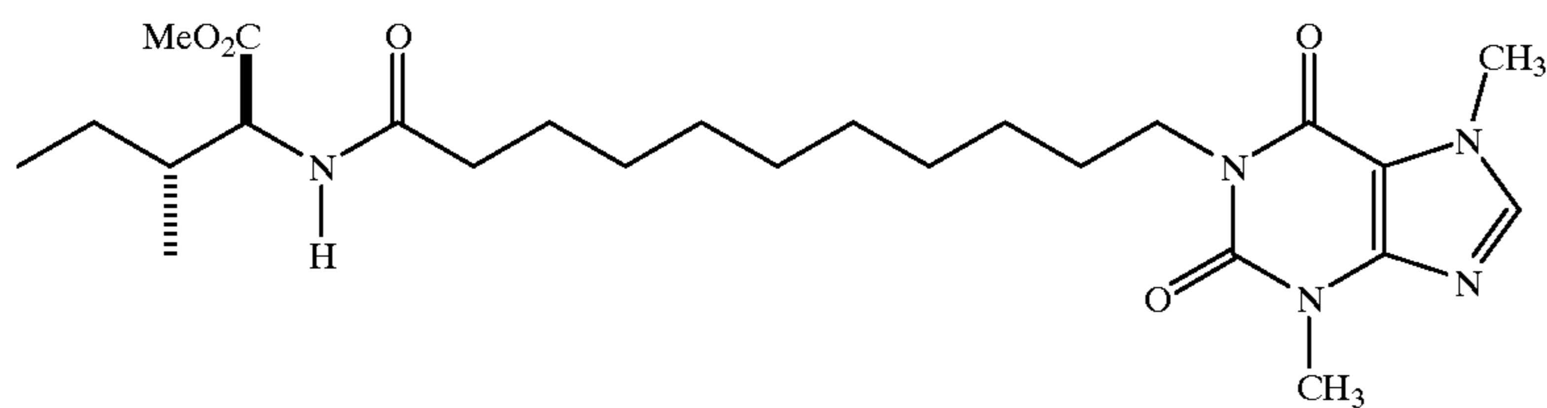
1-[11-(1-Methoxycarbonyl-2-methylbutylamino)-11-oxoundecyl]-3,7-dimethylxanthine
