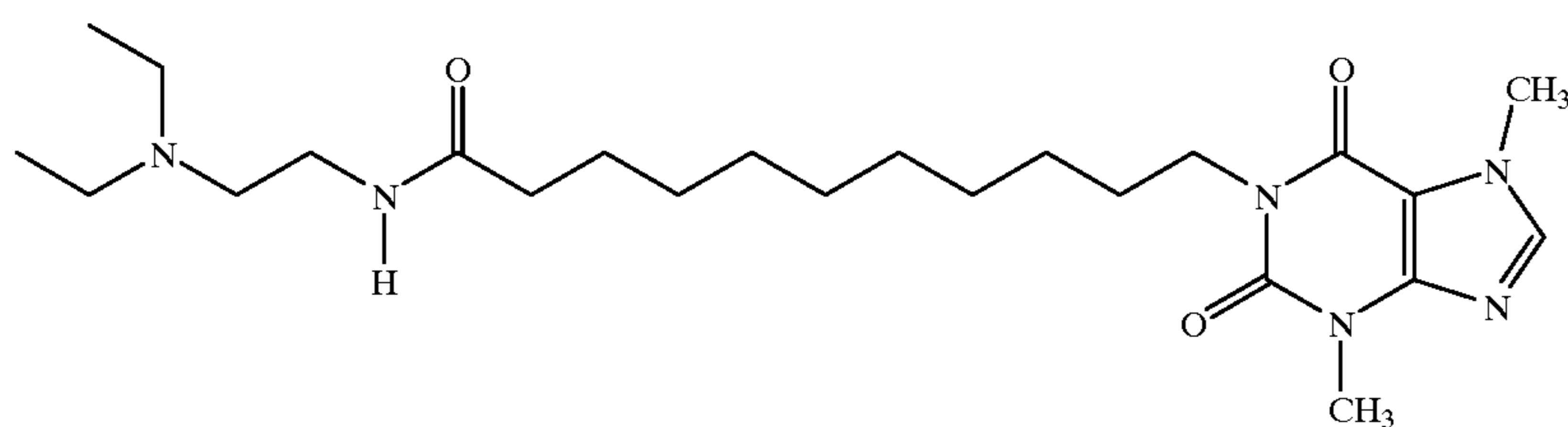
1-[N-(2-N',N'-Diethylaminoethyl)-11-yl-undecanamide]-3,7-dimethylxanthine
