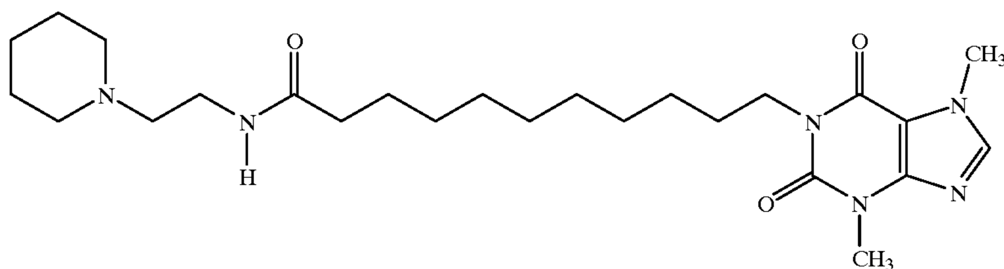
1-[N-(2-Piperidinoethyl)-11-yl-undecanamide]-3,7-dimethylxanthine
