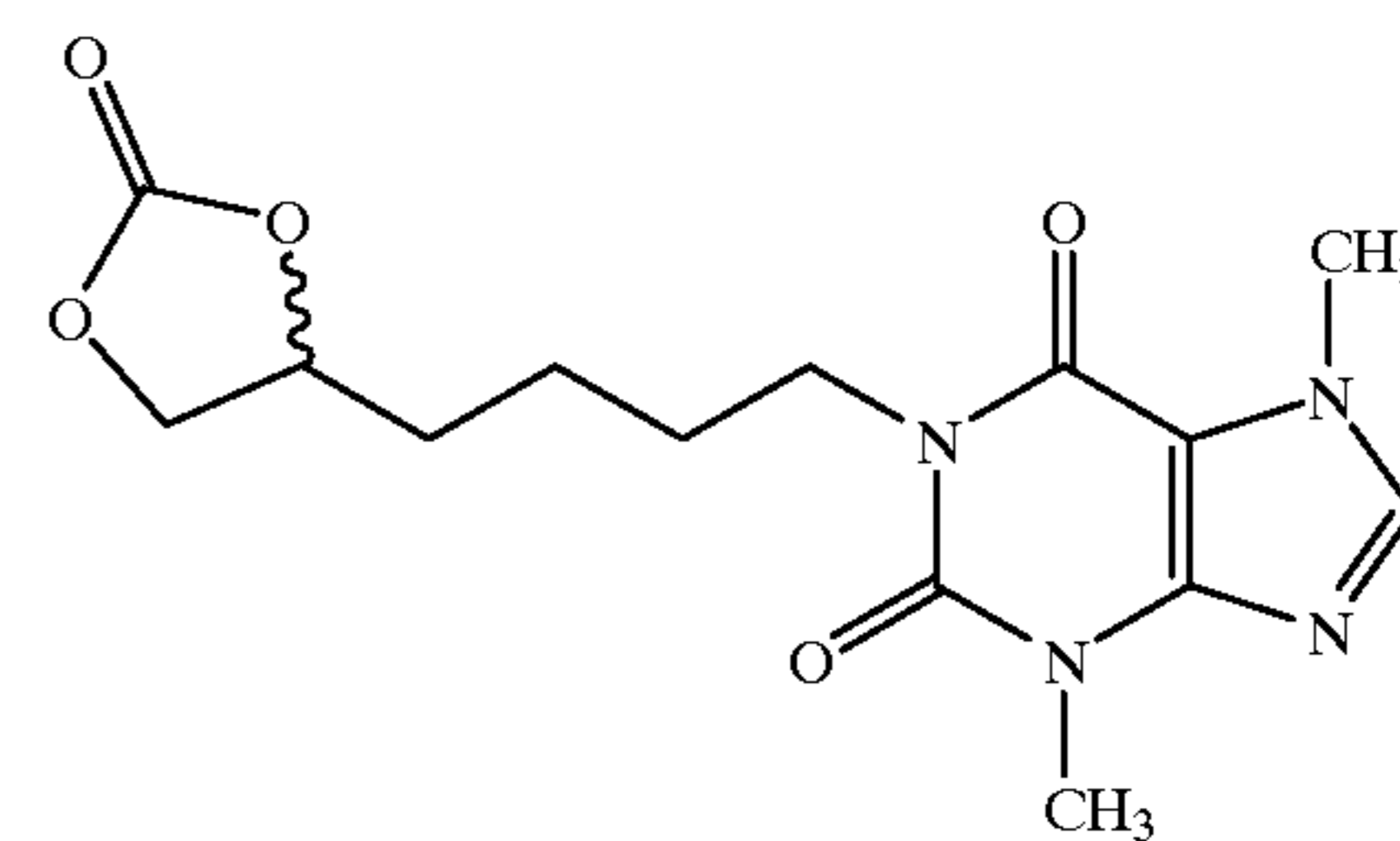
1-(5,6-Carbonyldioxyhexyl)-3,7-dimethylxanthine
