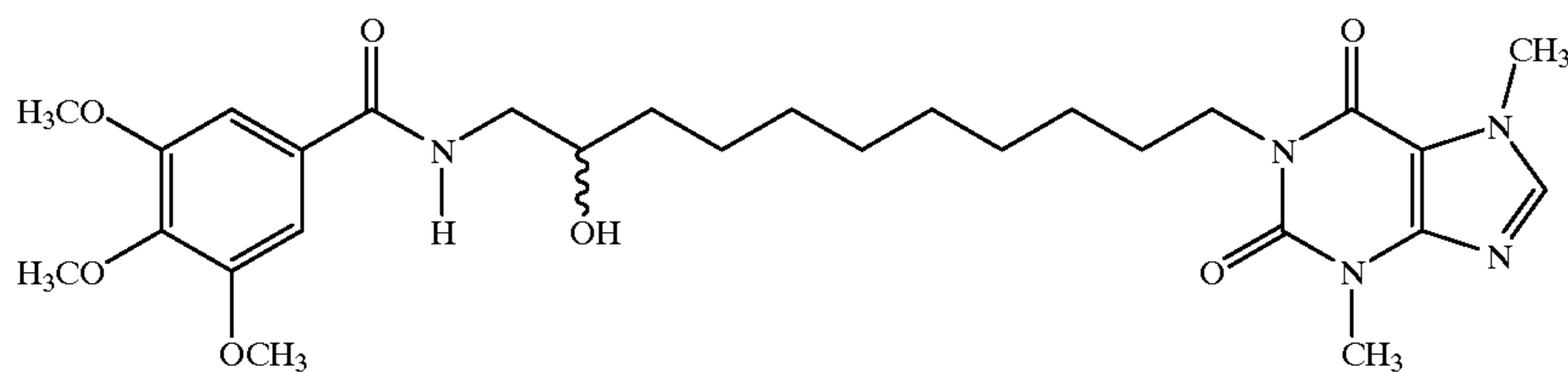
1-[11-(3,4,5-Trimethoxybenzamido)-10-hydroxyundecyl]-3,7-dimethylxanthine
