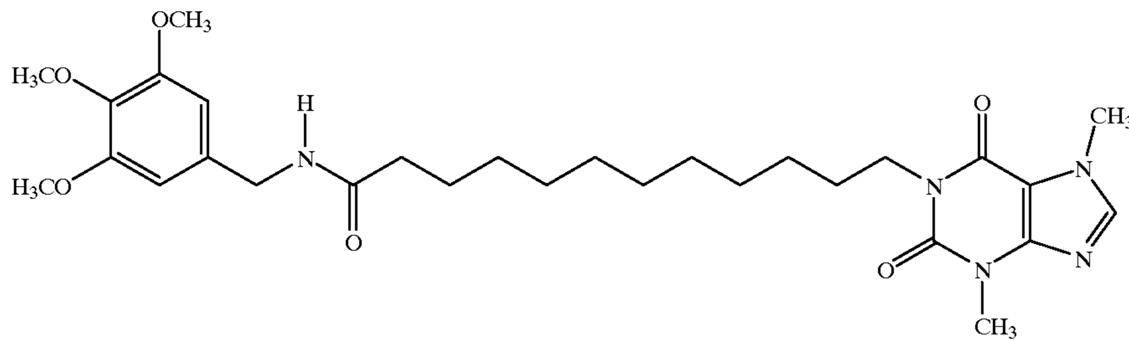
1-[N-(3, 4, 5-Trimethoxybenzyl)-12-yl-dodecanamide]-3, 7-dimethylxanthine
