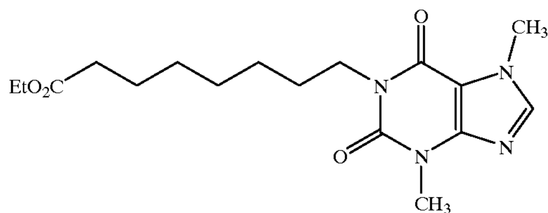
1-(Ethyl 8-yl-octanoate)-3,7-dimethylxanthine
