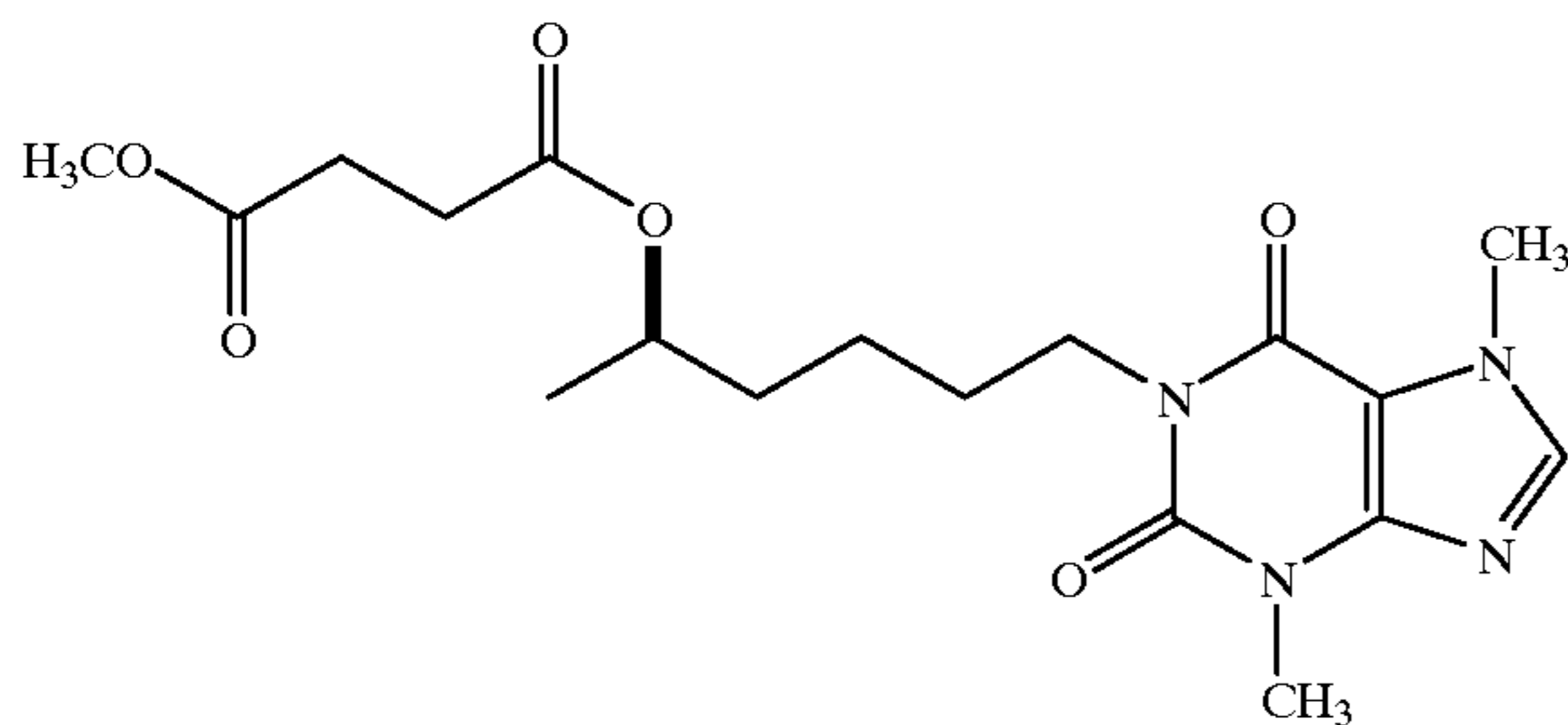
R-1-(5-Hydroxy)hexyl)-3,7-dimethylxanthine methyl succinate
