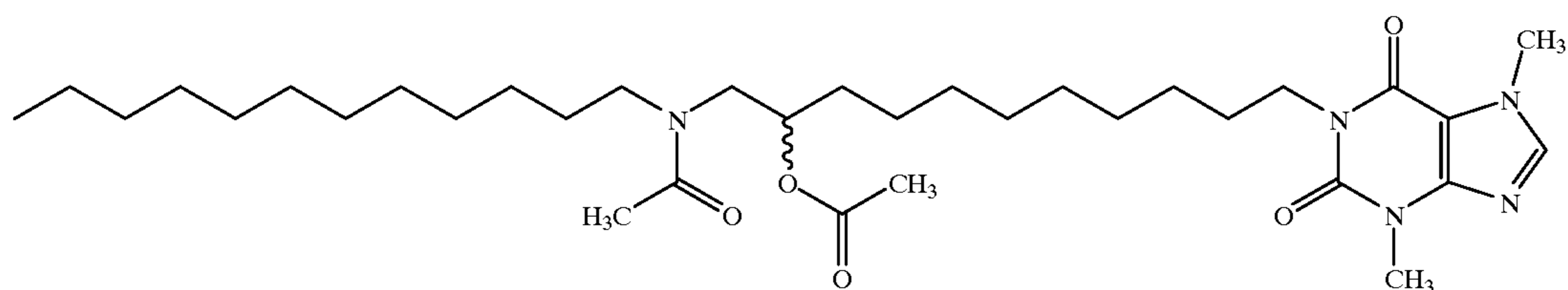
1-[11-(N-Dodecylacetamido)-10-acetoxyundecyl]-3,7-dimethylxanthine
