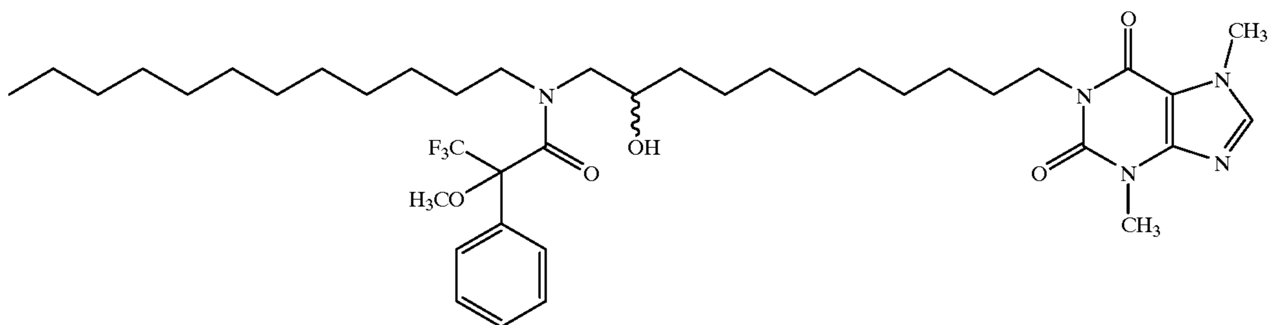
1-[11-[N-Dodecyl(R)-2-methoxy-2-phenylacetamido]-10-hydroxyundecyl]-3,7-dimethylxanthine
