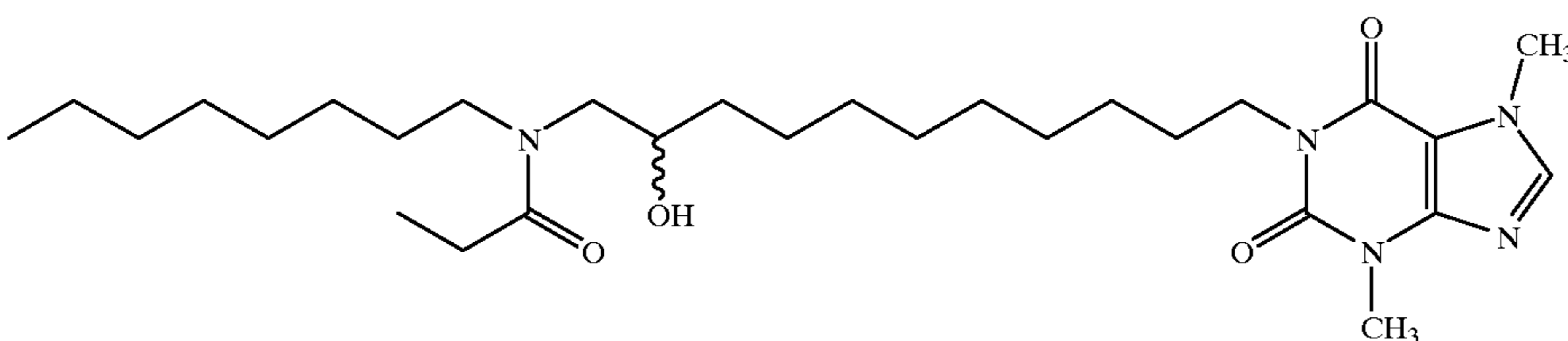
1-[11-(N-Octyl propionamido)-10-hydroxyundecyl]-3,7-dimethylxanthine
