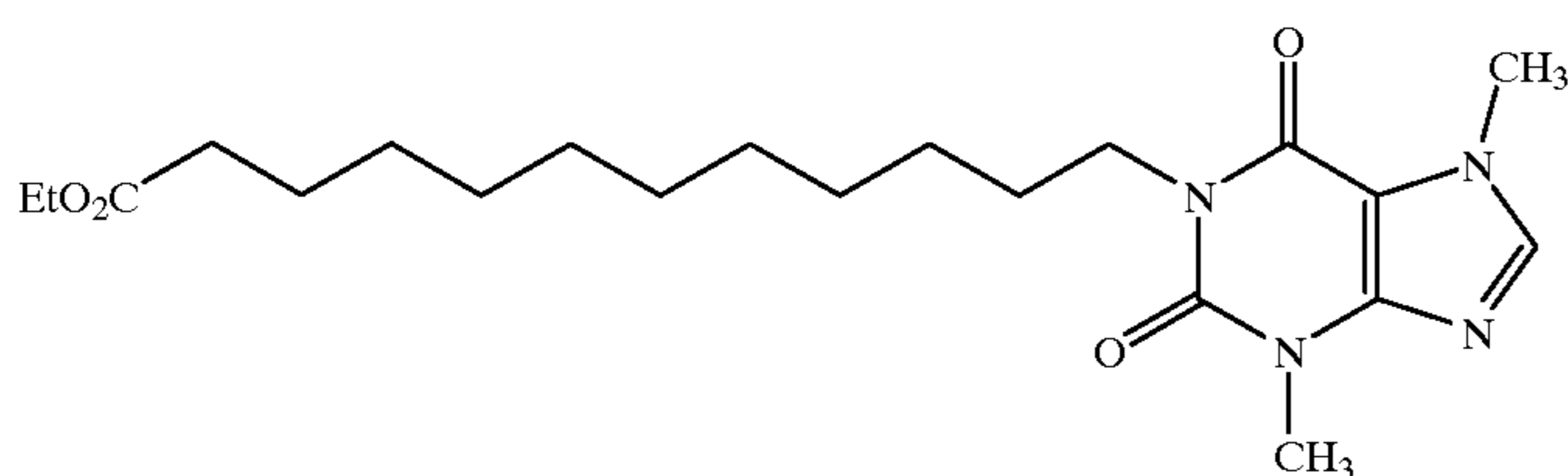
1-(Ethyl 12-yl-dodecanoate)-3,7-dimethylxanthine
