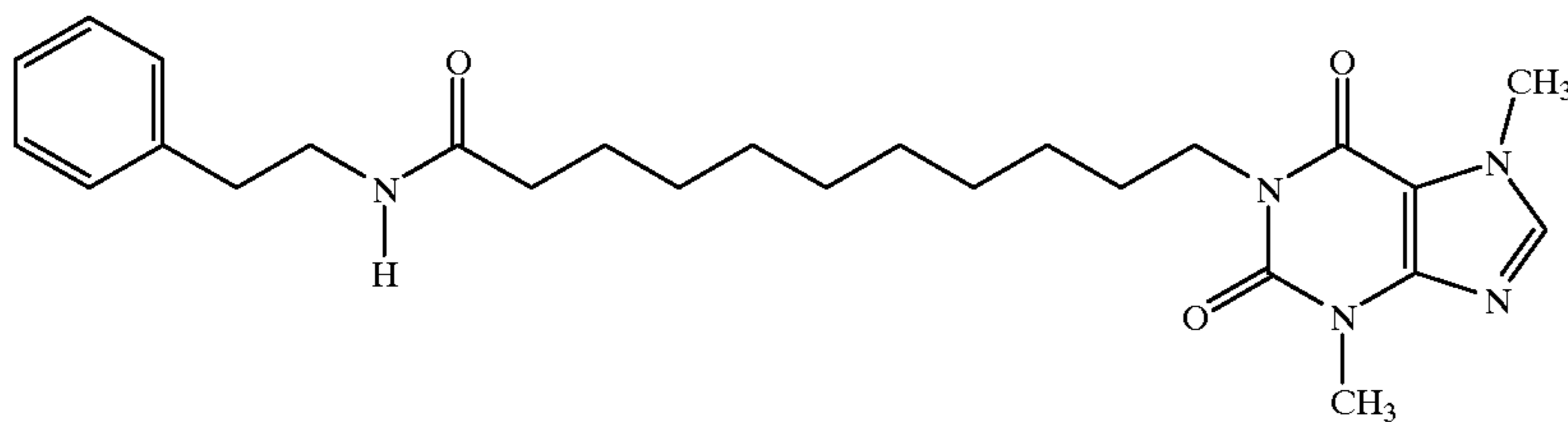
1-[N-(Phenethyl)-11-yl-undecanamide]-3,7-dimethylxanthine
