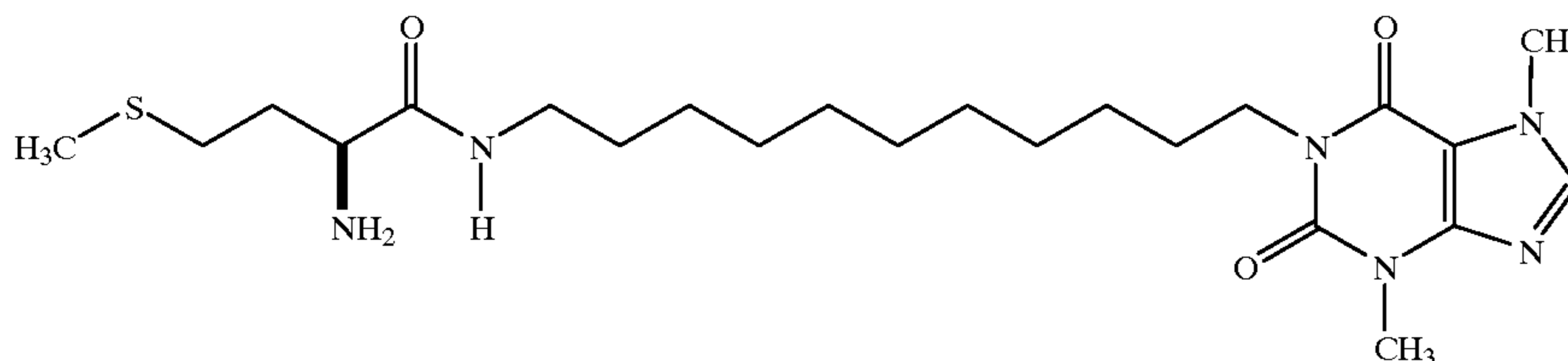
(S)-1-[11-(2-Amino-4-methylthiobutyronamido)undecyl]-3, 7-dimethylxanthine
