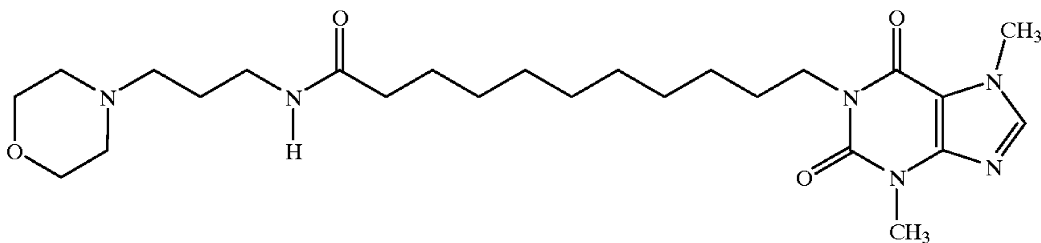
1-[N-(3-Morpholinopropyl)-11-yl-undecanoamide]-3,7-dimethylxanthine
