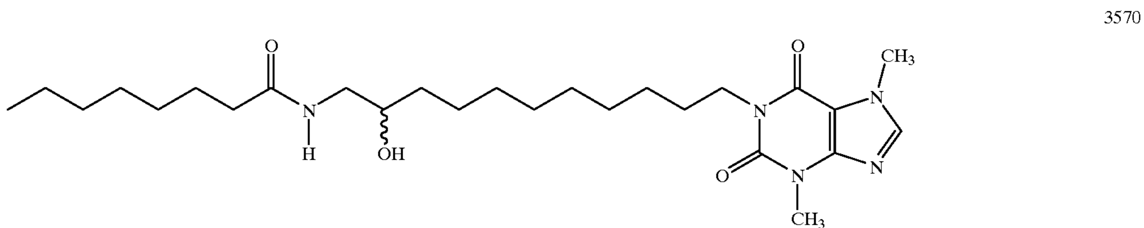
1-[11-Octanoamido-10-hydroxyundecyl)-3, 7-dimethylxanthine
