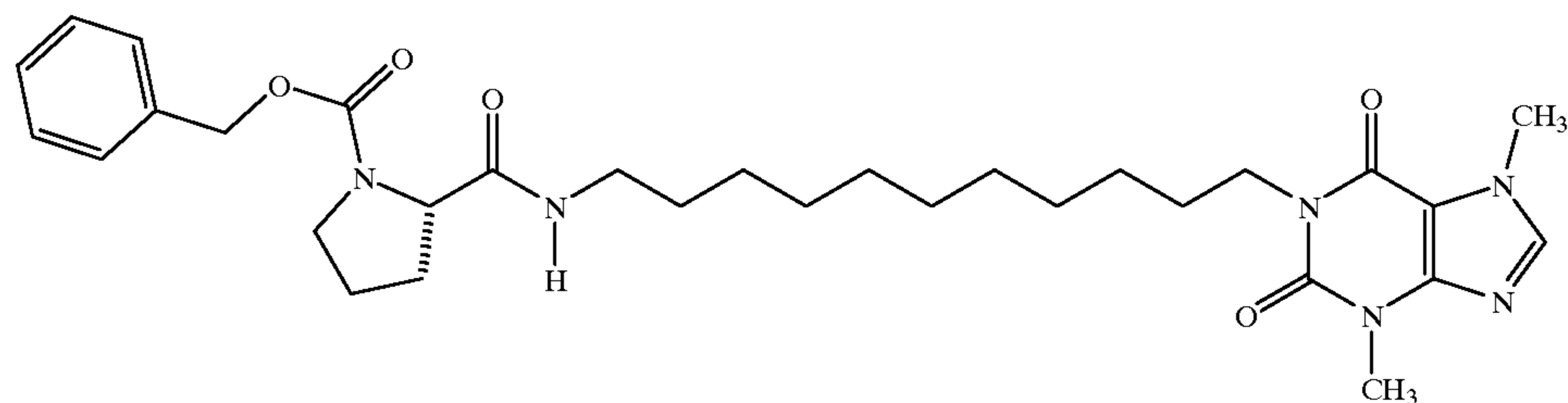
1-[11-(1-Carbobenzyloxypyrrolidin-2-yl-formamido)undecyl]-3,7-dimethylxanthine
