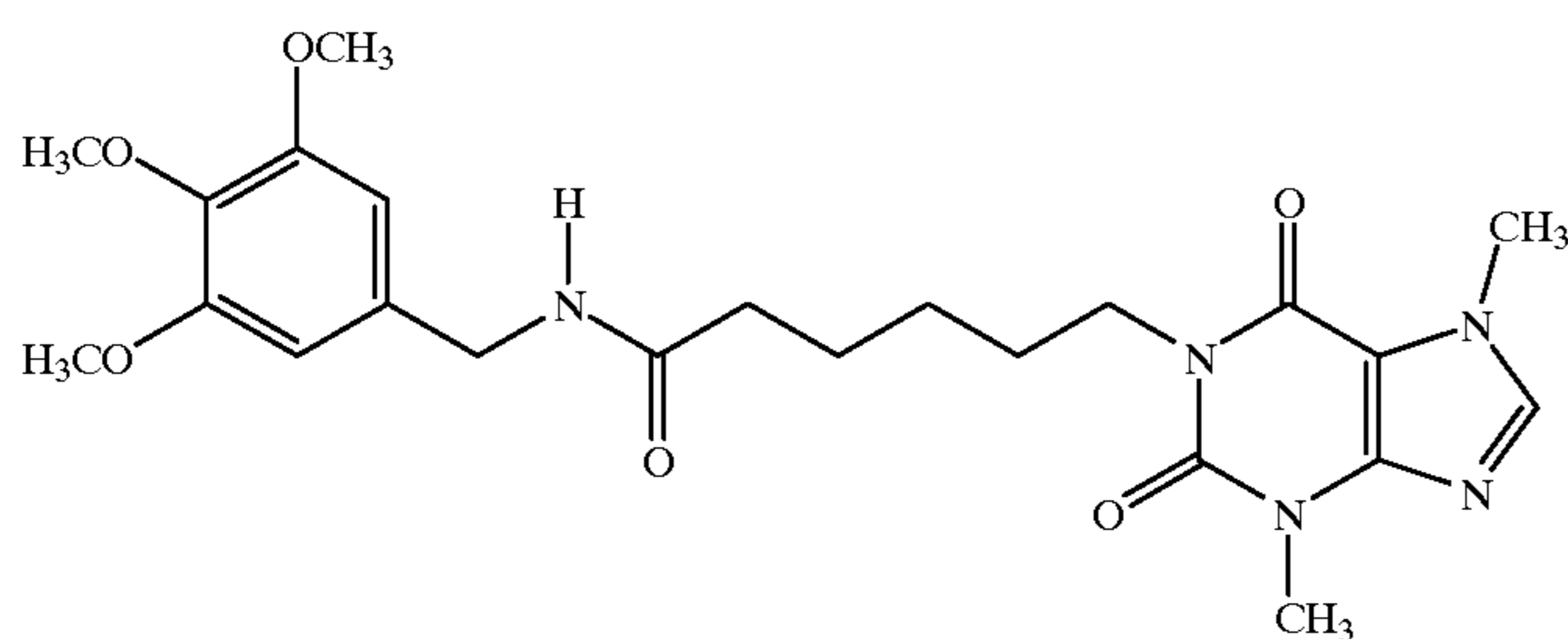
1-[N-(3, 4, 5-Trimethoxybenzyl)-6-yl-hexanamide]-3, 7-dimethylxanthine
