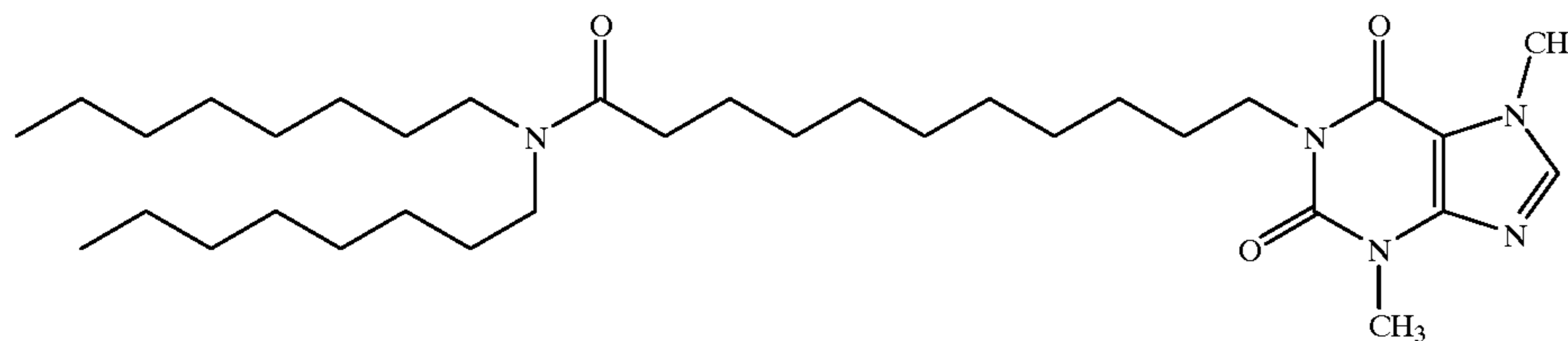
1-[N, N-Dioctyl-11-yl-undecanamide)-3, 7-dimethylxanthine
