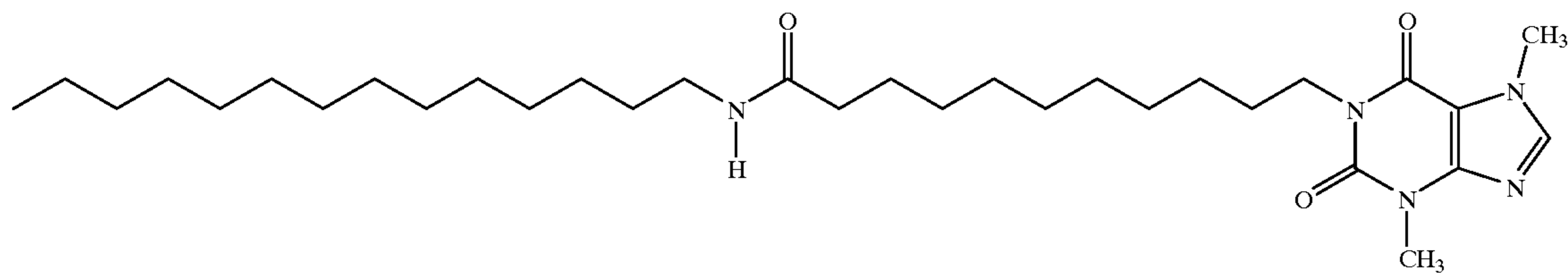
1-(N-Tetradecyl-11-yl-undecanamide)-3,7-dimethylxanthine
