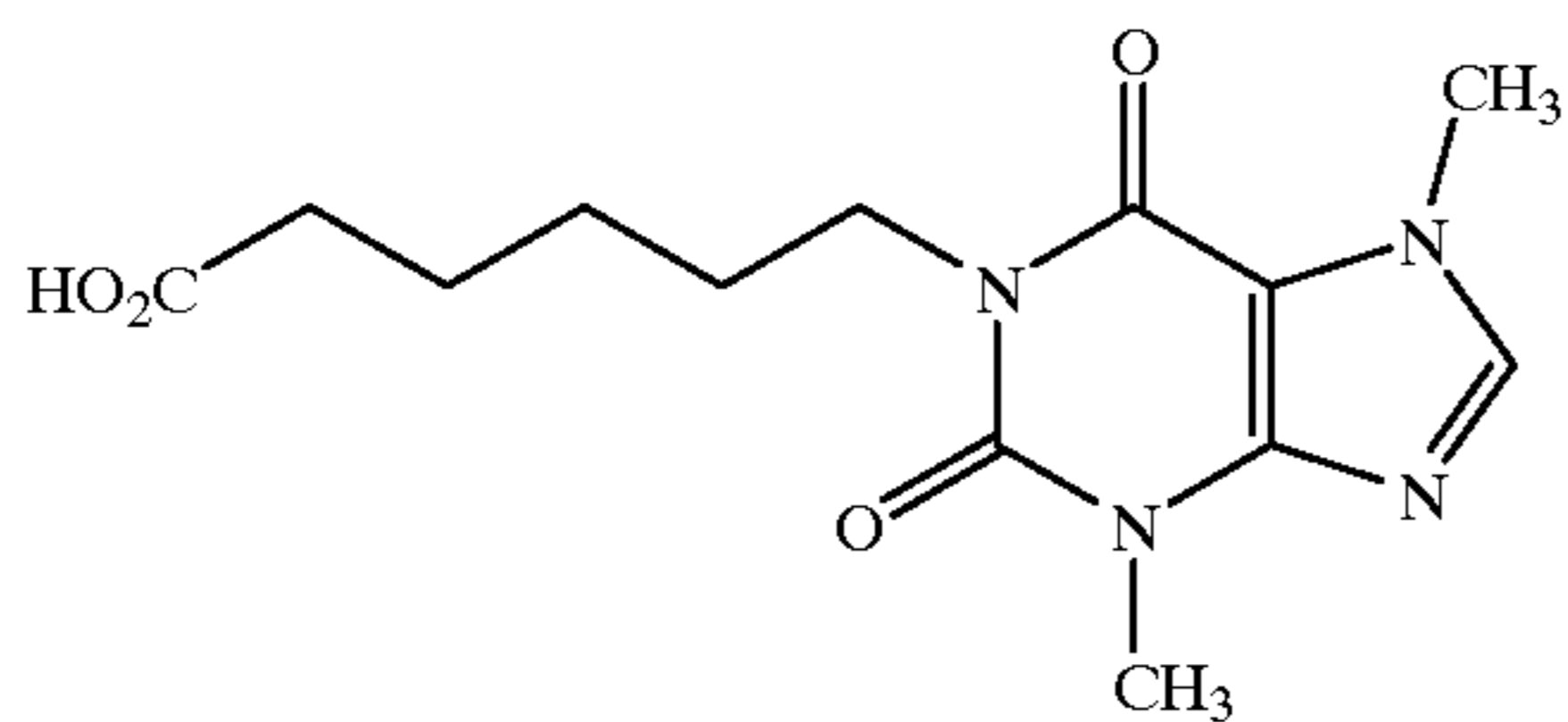
1-(6-yl-Hexanoic acid)-3, 7-dimethylxanthine
