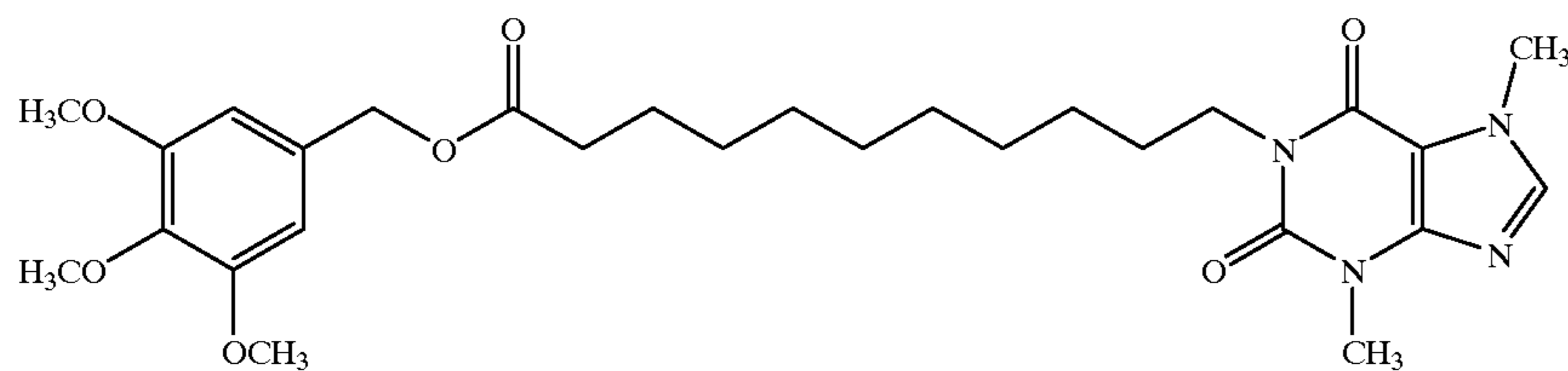
1-(3, 4, 5-Trimethoxybenzyl 11-yl-undecanoate)-3, 7-dimethylxanthine
