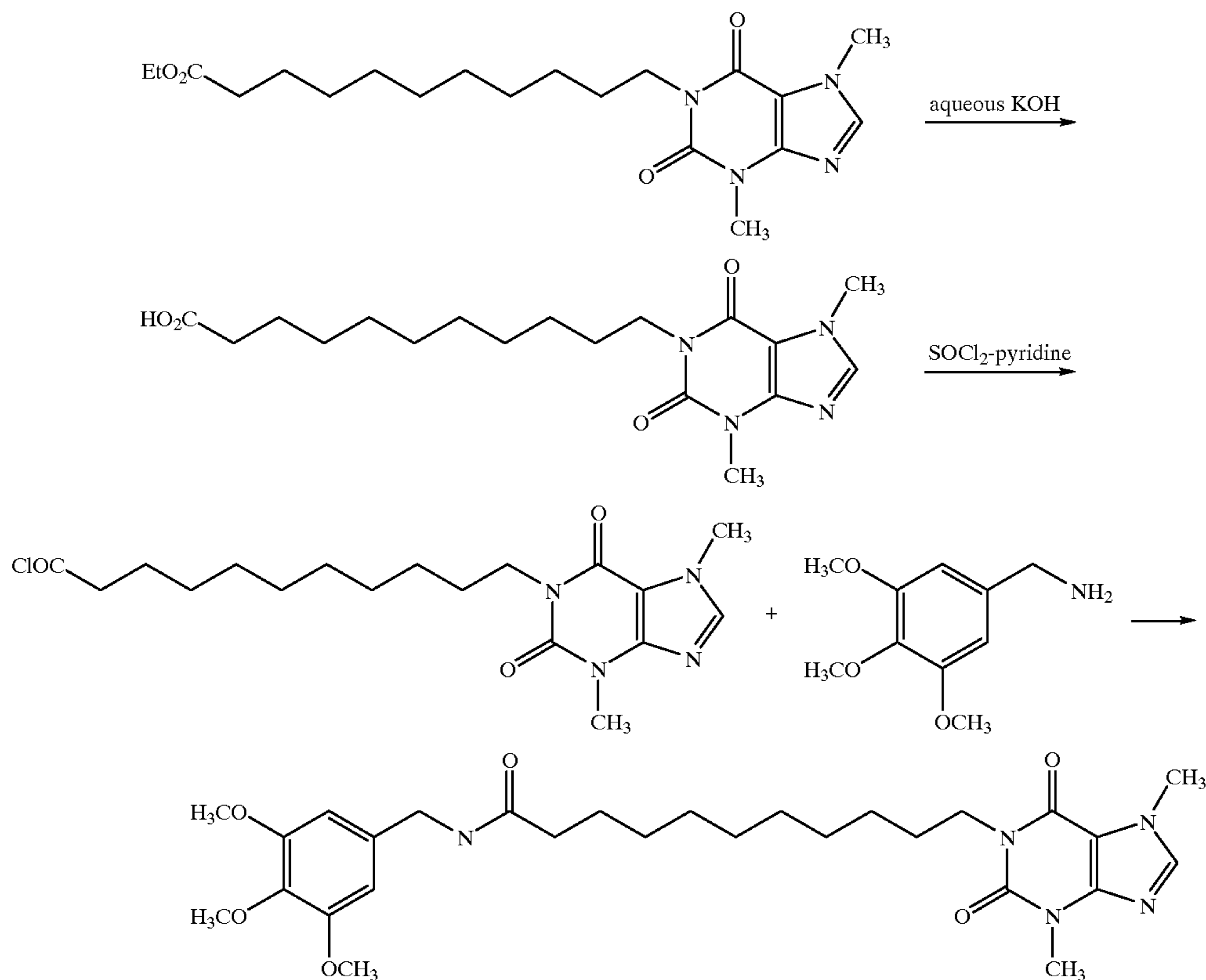
Inventive amide-containing compound
