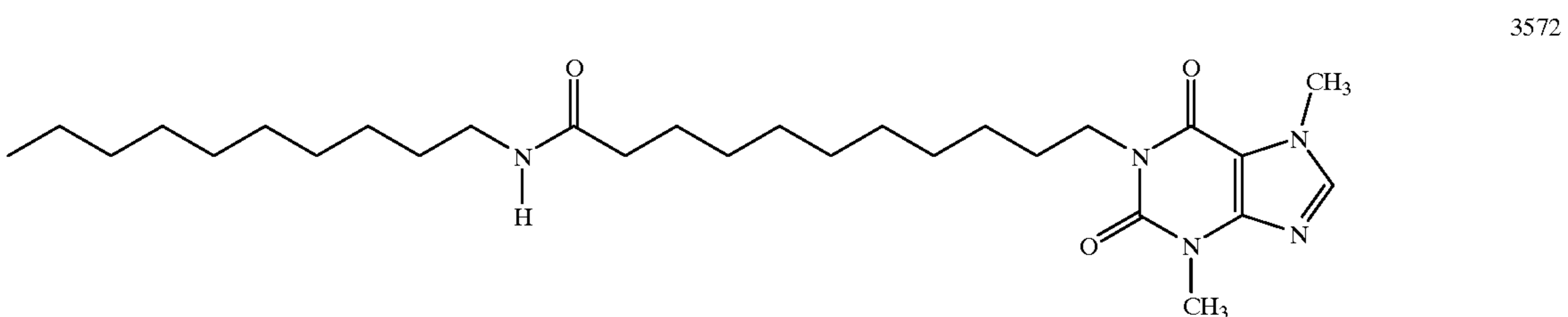
1-(N-Decyl-11-yl-undecanamide)-3, 7-dimethylxanthine
