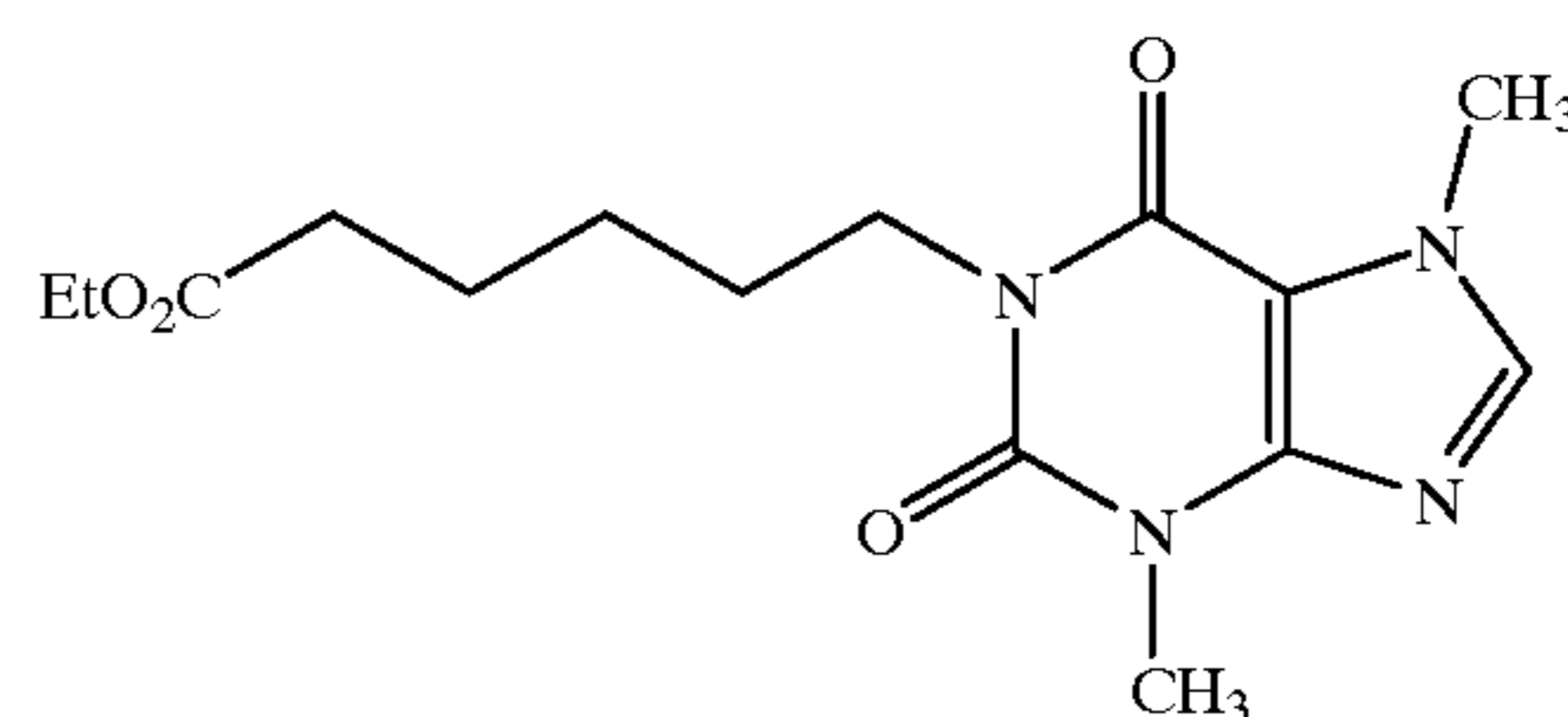
1-(Ethyl 6-yl-hexanoate)-3,7-dimethylxanthine
