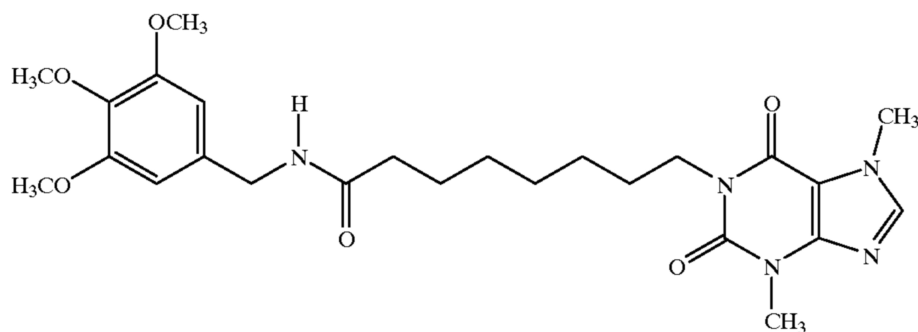
1-[N-(3,4,5-Trimethoxybenzyl)-8-yl-octanamide]-3,7-dimethylxanthine
