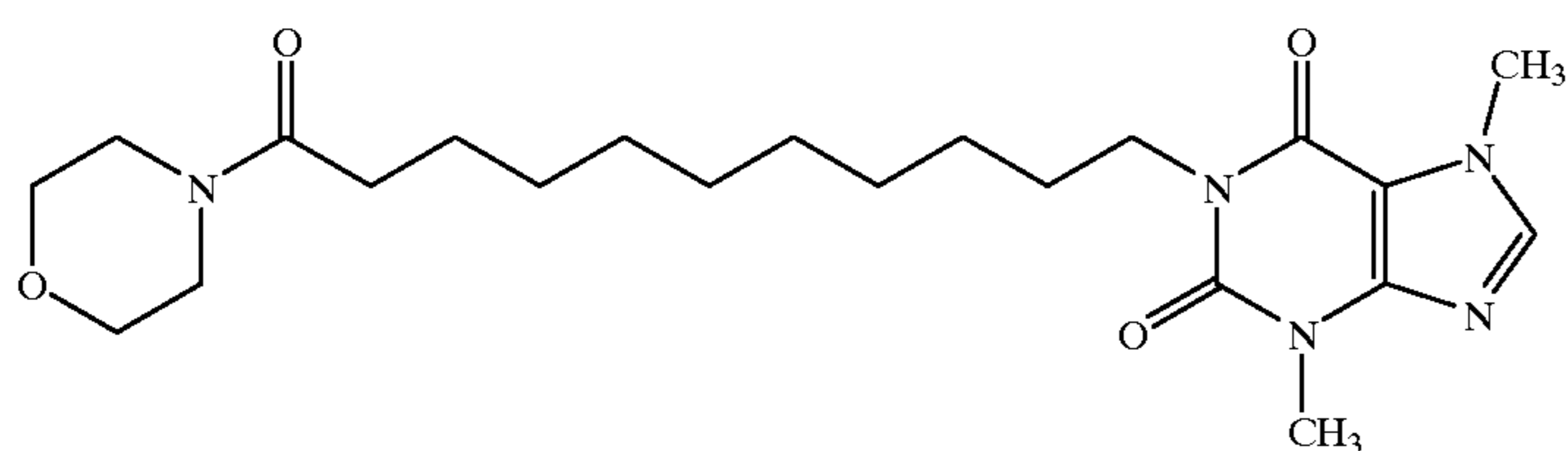
1-[N-(Morpholine)-11-yl-undecanoamide]-3, 7-dimethylxanthine
