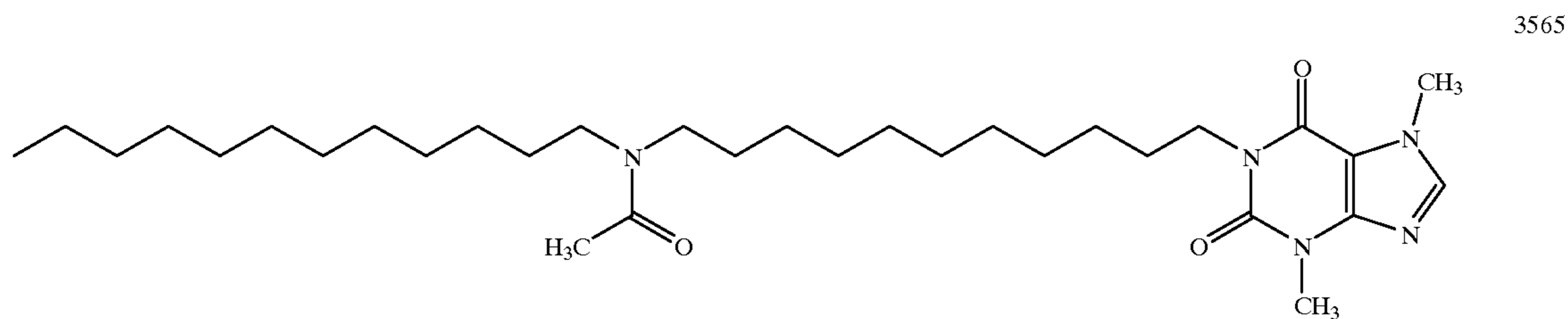
1[11-(N-Dodecylacetamido)undecyl]-3, 7-dimethylxanthine
