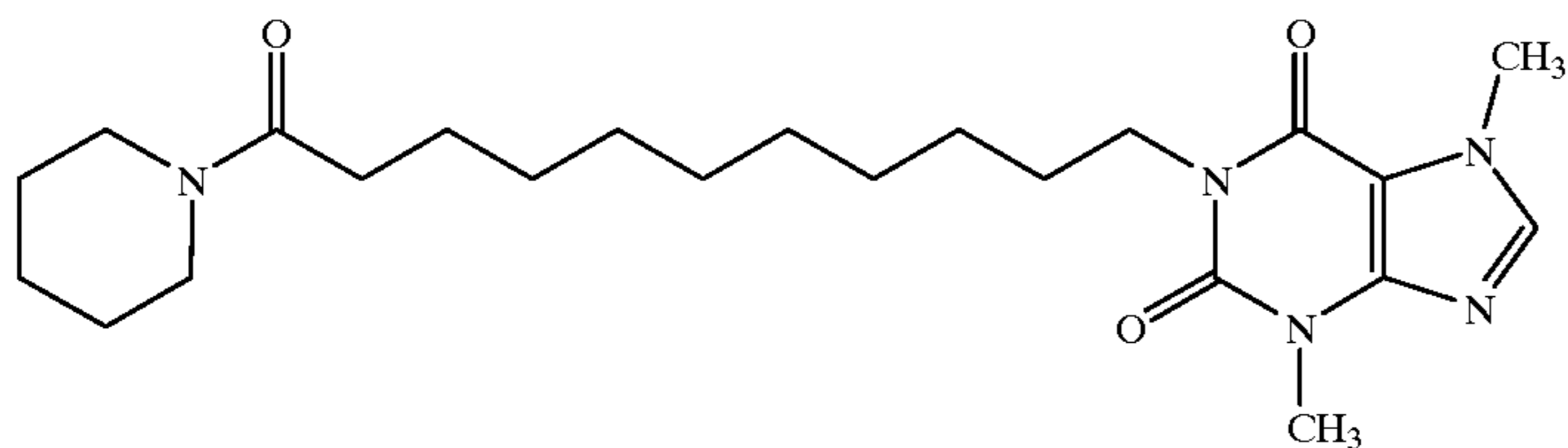
1-[N-(Piperidiny)-11-yl-undecanoamide]-3,7-dimethylxanthine
