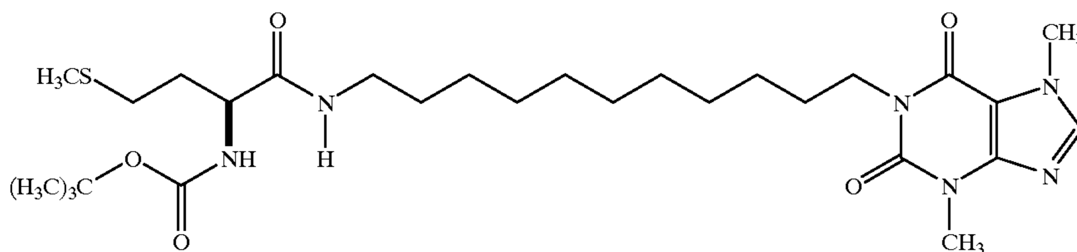
(S)-1-[11-(2-Carbobutoxyamino-4-methylthiobutyronamido)undecyl]-3, 7-dimethylxanthine
