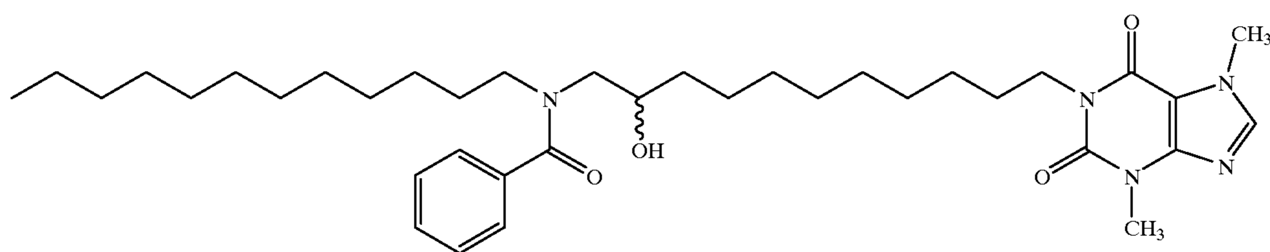
1-[11-(Dodecyl benzamido)-10-hydroxyundecyl]-3,7-dimethylxanthine
