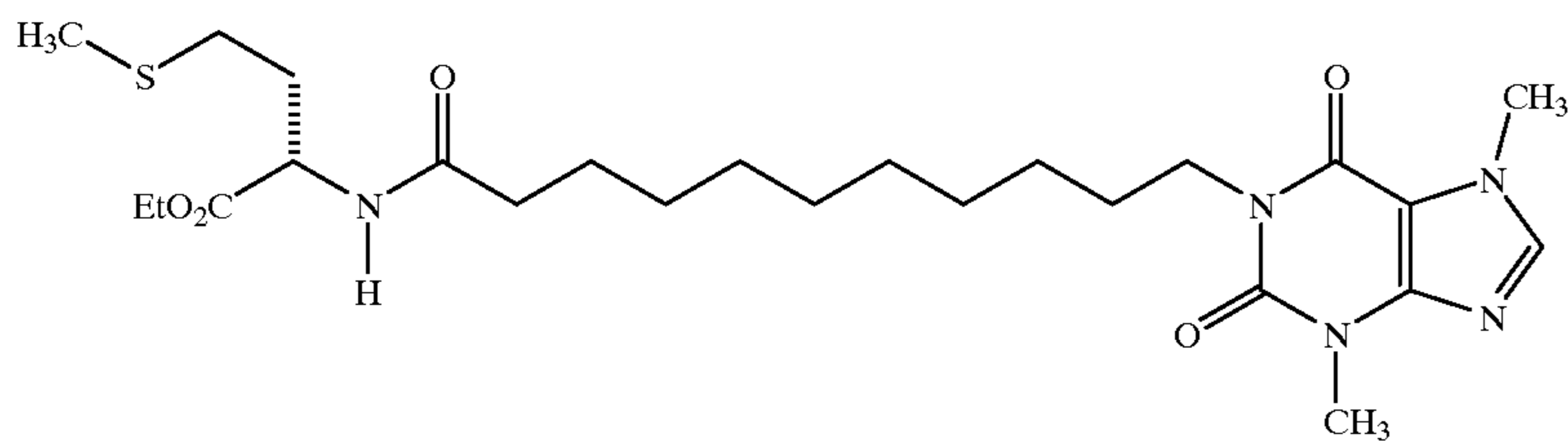
1-[11-(1-Ethoxycarbonyl-3-methylthiopropylamino)-11-oxoundecyl]-3,7-dimethylxanthine
