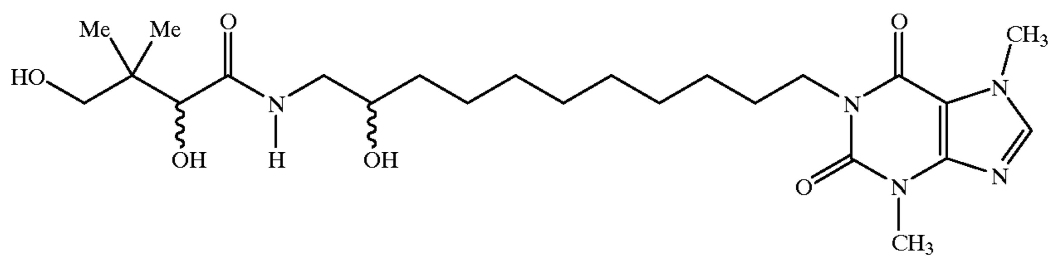
1-[11-Pantothenic acid amido-10-hydroxyundecyl]-3, 7-dimethylxanthine
