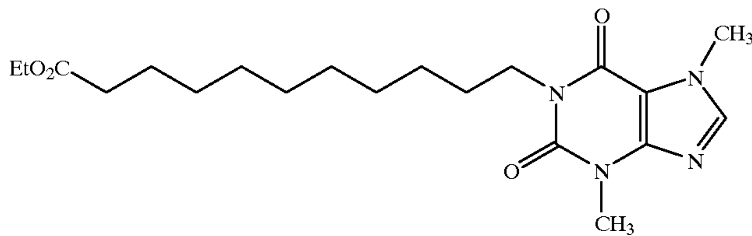
1-(Ethyl-11-yl-undecanoate)-3, 7-dimethylxanthine
