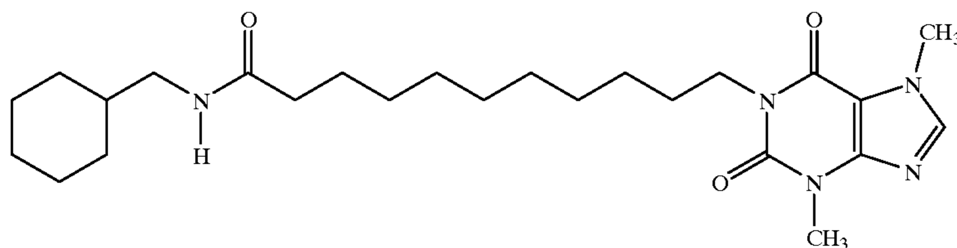
1-[N-(Cyclohexylmethyl)-11-yl-undecanoamide]-3,7-dimethylxanthine
