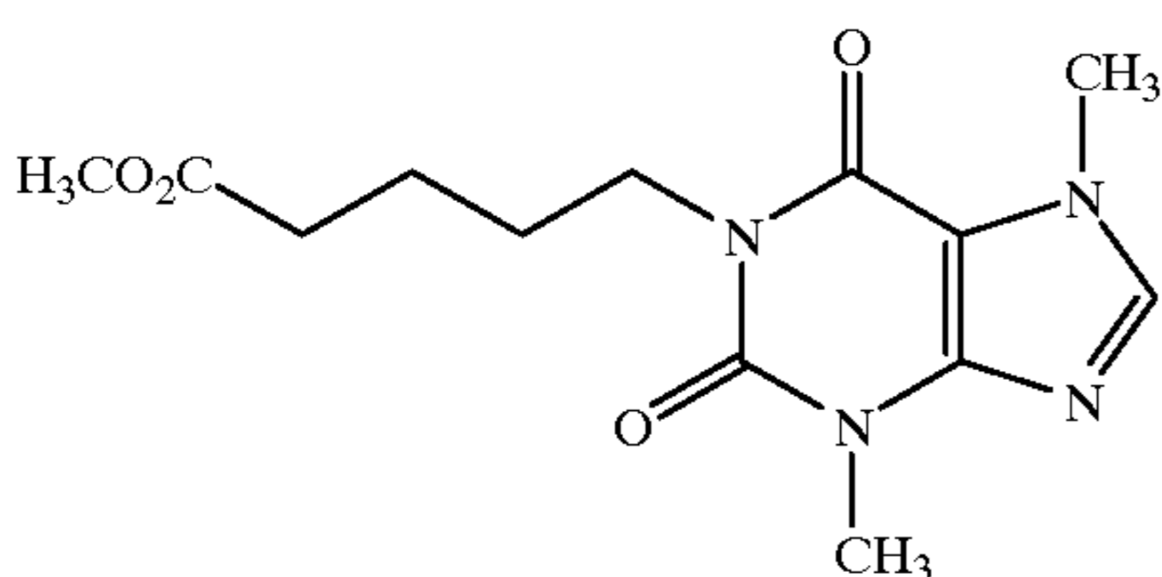
1-(Pentoyl)-3,7-dimethylxanthine carboxylic acid methyl ester
