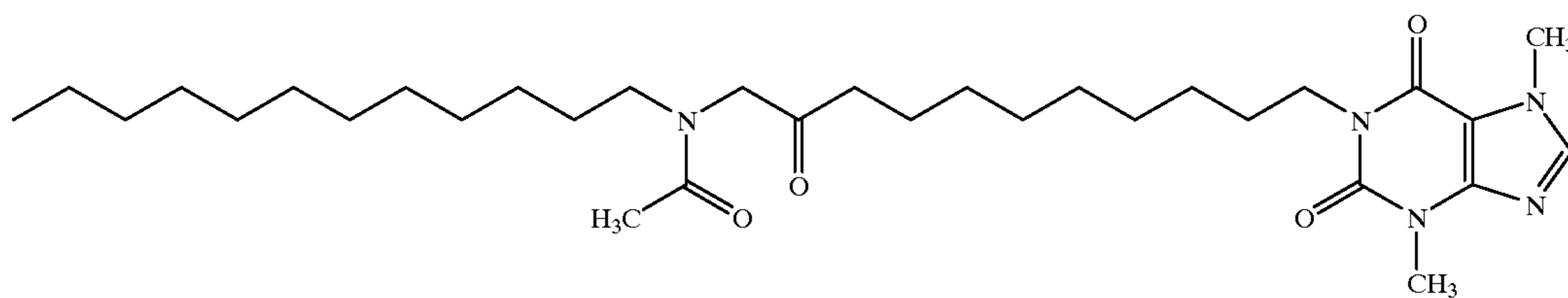
1-(11-[N-Dodecylacetamido]-10-oxoundecyl)-3,7-dimethylxanthine
