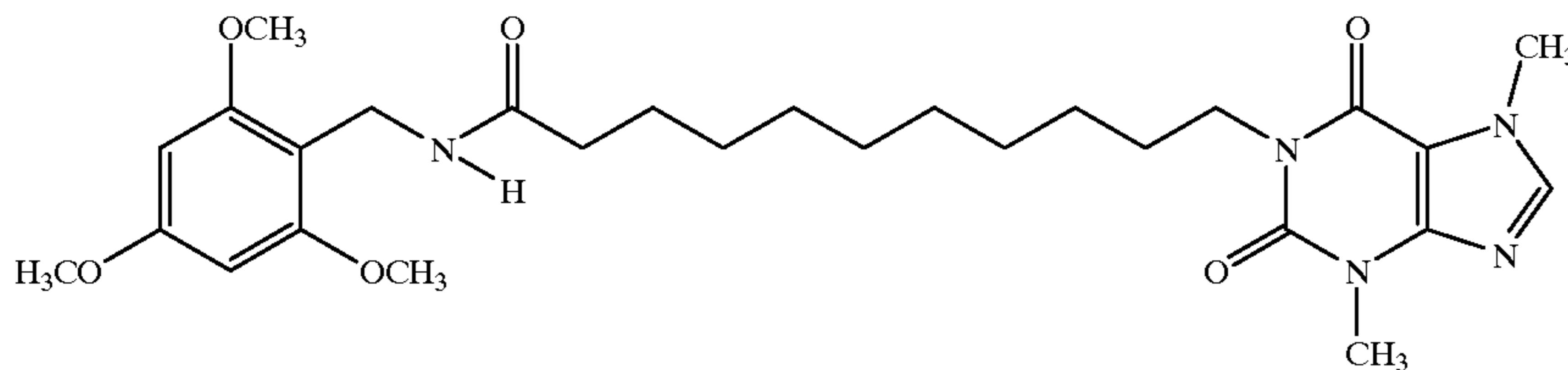
1-[N-(2,4,6-Trimethoxybenzyl)-11-yl-undecanamide]-3,7-dimethylxanthine
