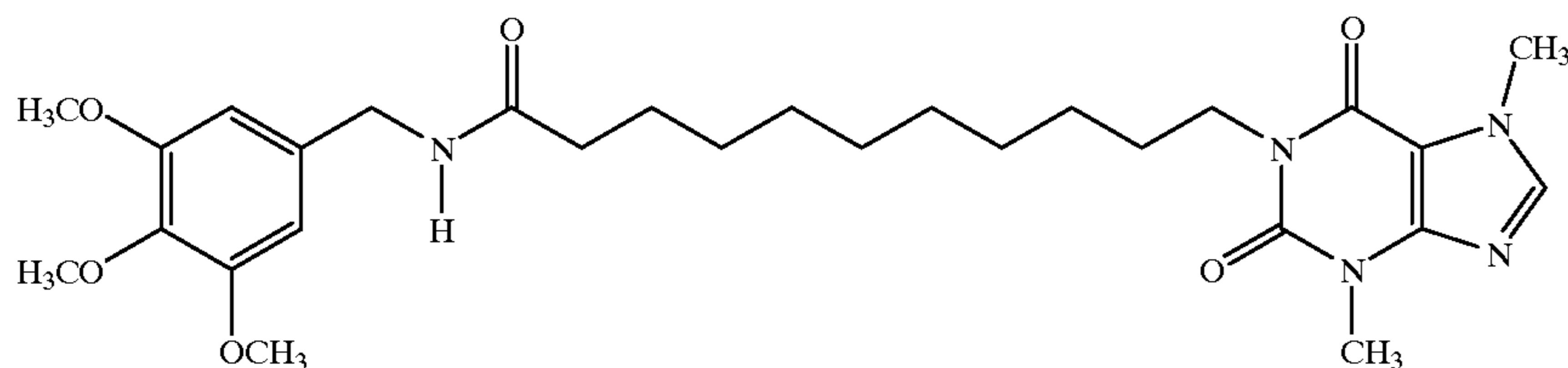
1-[N-(3,4,5-Trimethoxybenzyl)-11-yl-undecanamide]-3,7-dimethylxanthine
