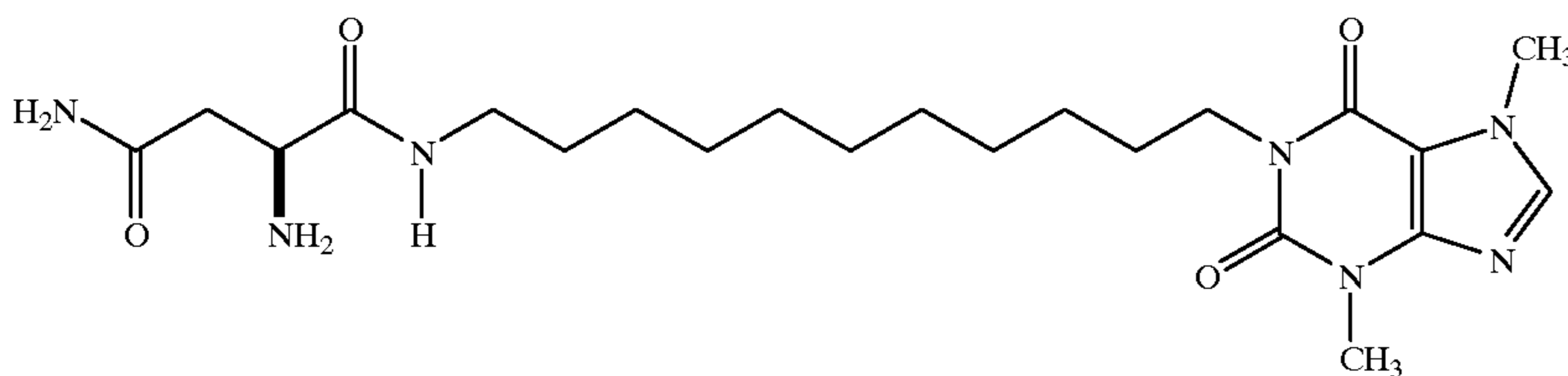
1-(11-[2,4-Diamino-4-oxobutyronamido]undecyl)-3,7-dimethylxanthine
