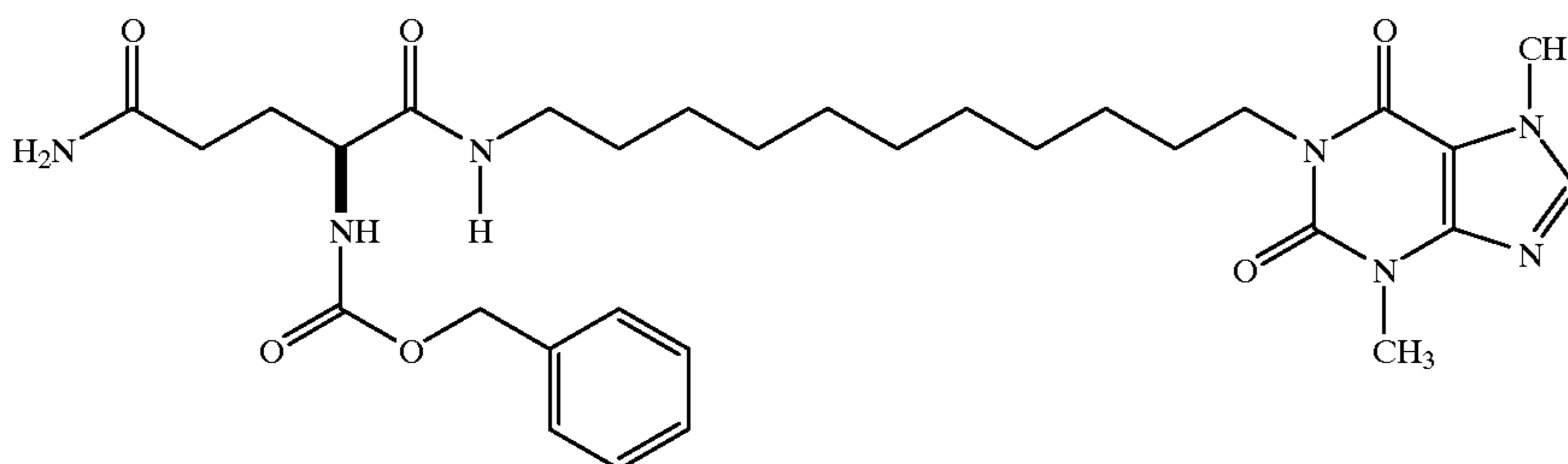
1-(11-[5-Amino-2-carbobenzyloxyamino-5-oxopentanamido]undecyl)-3,7-dimethylxanthine
