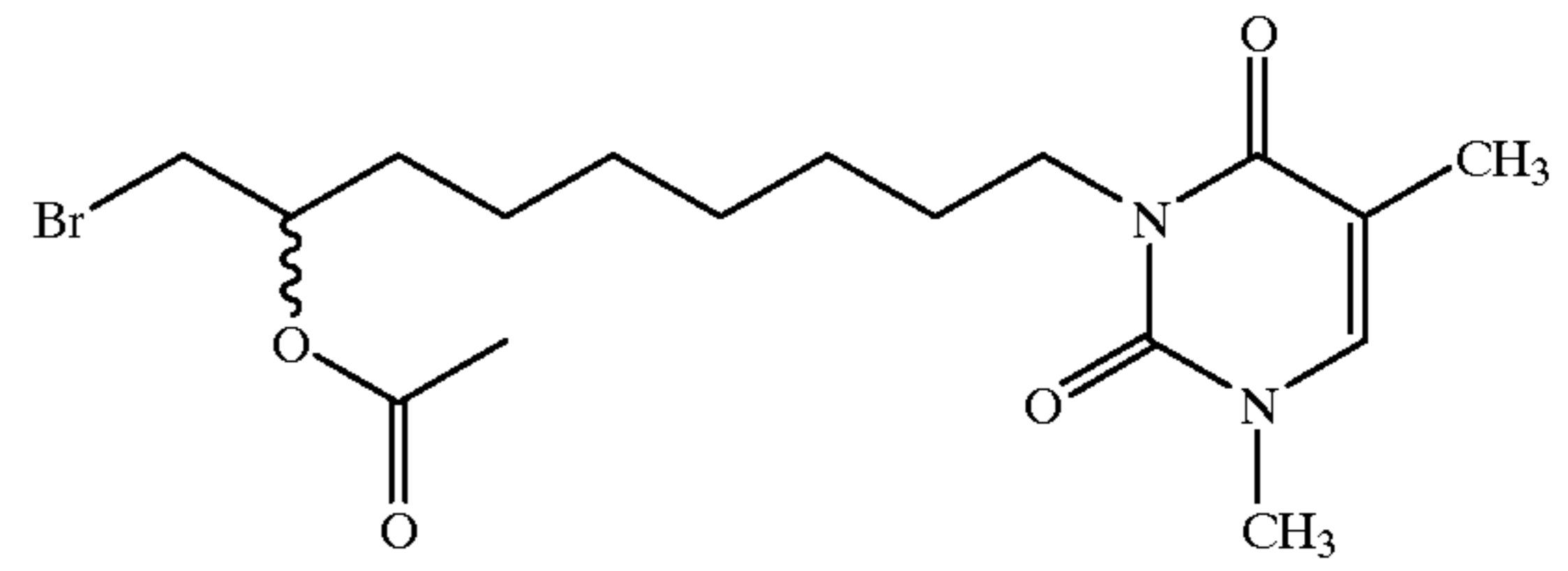
3-(8-Acetoxy-9-bromononyl)-1-methylthymine
