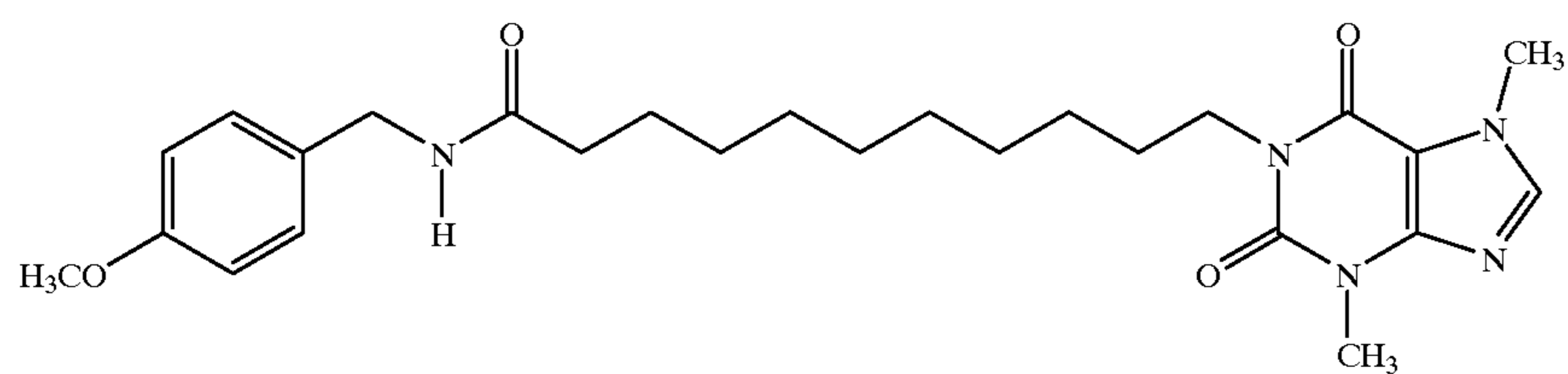
1-[N-(4-methoxybenzyl)-11-yl-undecanamide]-3,7-dimethylxanthine
