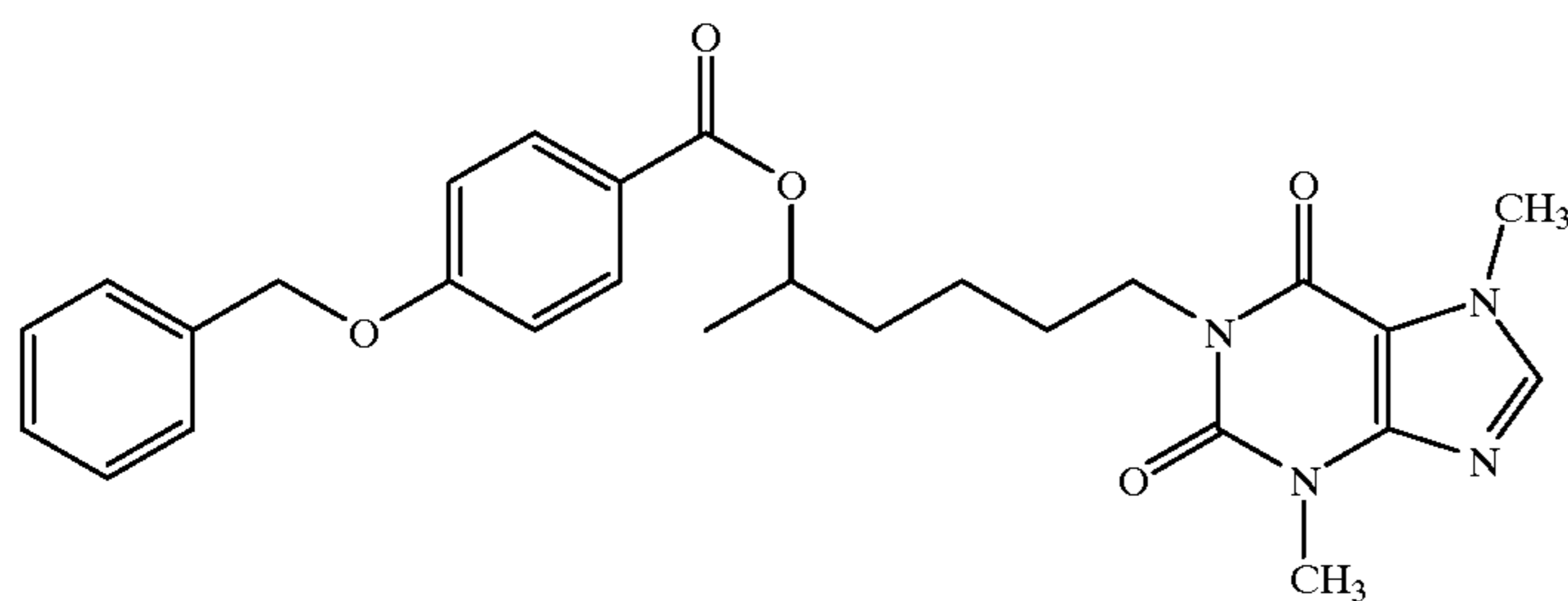
R-1-(5-(4'-benzyloxybenzoyloxy)hexyl)-3,7-dimethylxanthine
