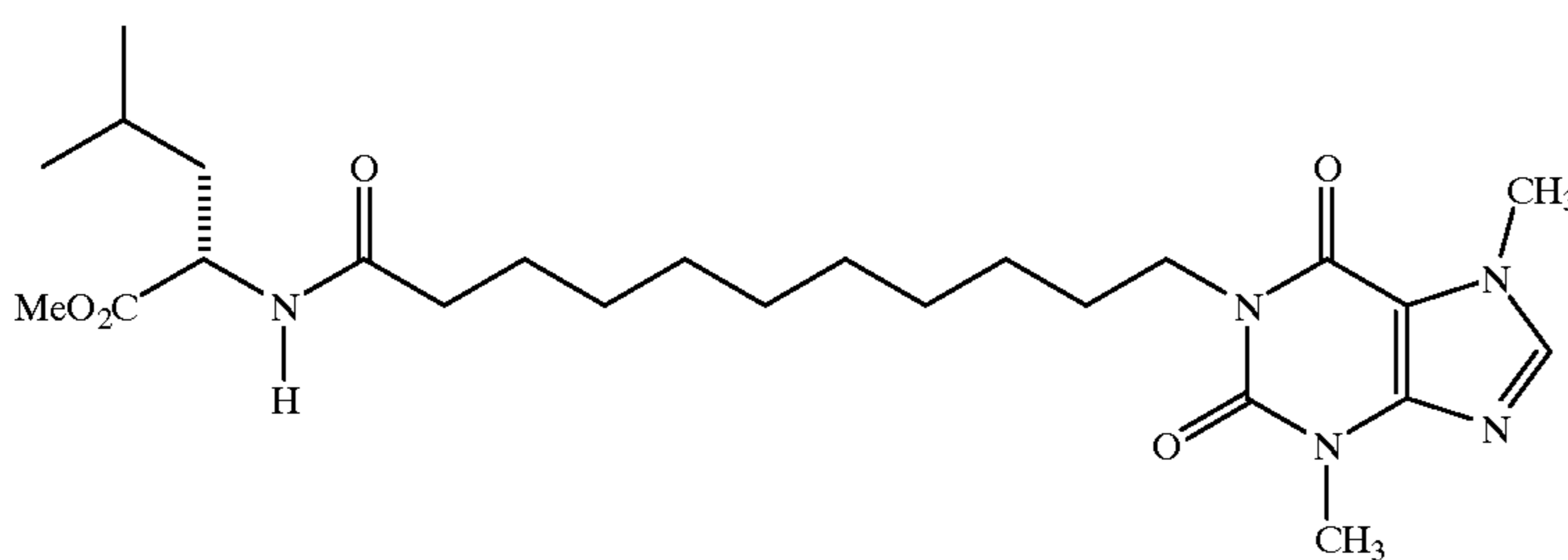
1-[11-(1-Methoxycarbonyl-3-methylbutylamino)-11-oxoundecyl]-3,7-dimethylxanthine
