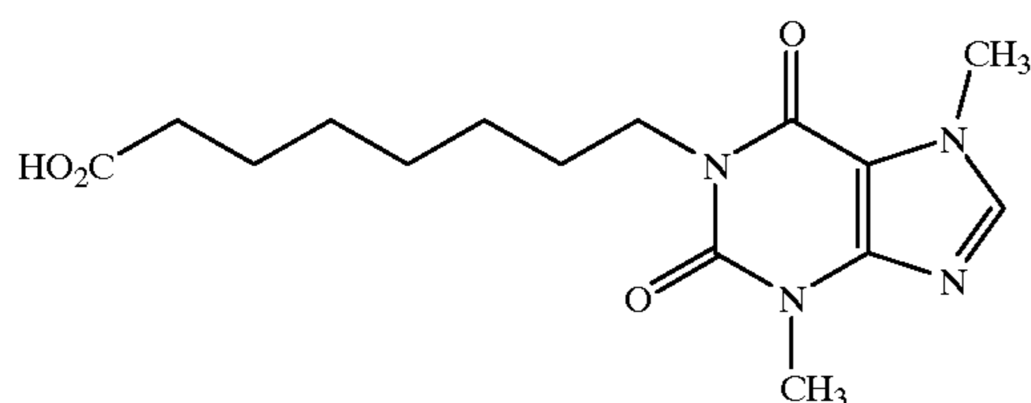
1-(8-yl-Octanoic acid)-3,7-dimethylxanthine
