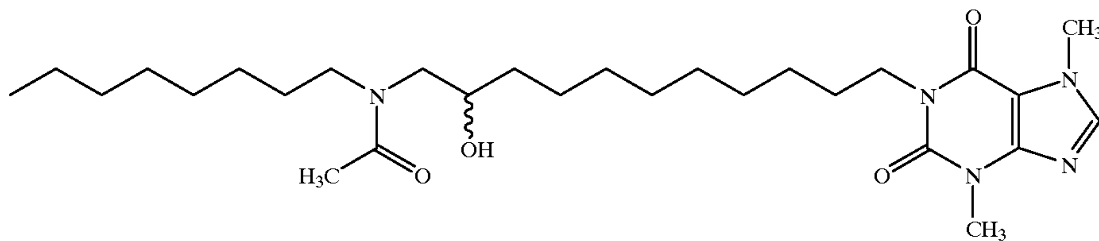
1-[11-(N-Ocylacetamido)-10-hydroxyundecyl]-3,7-dimethylxanthine
