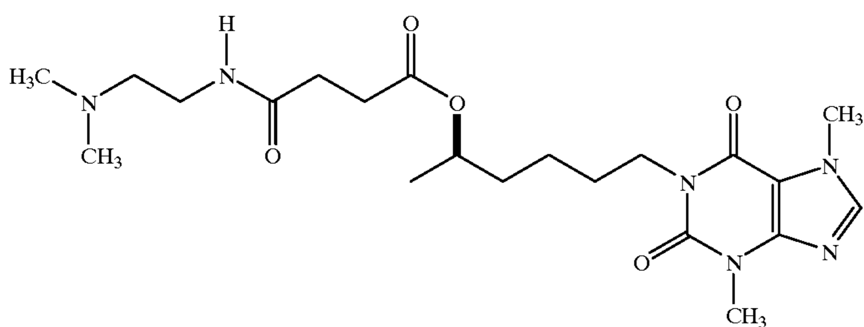
R-1-(5-[[2-(Dimethylamino)ethyl]amino]-1,4-dioxobutyl]oxy)hexyl)-3,7-dimethylxanthine
