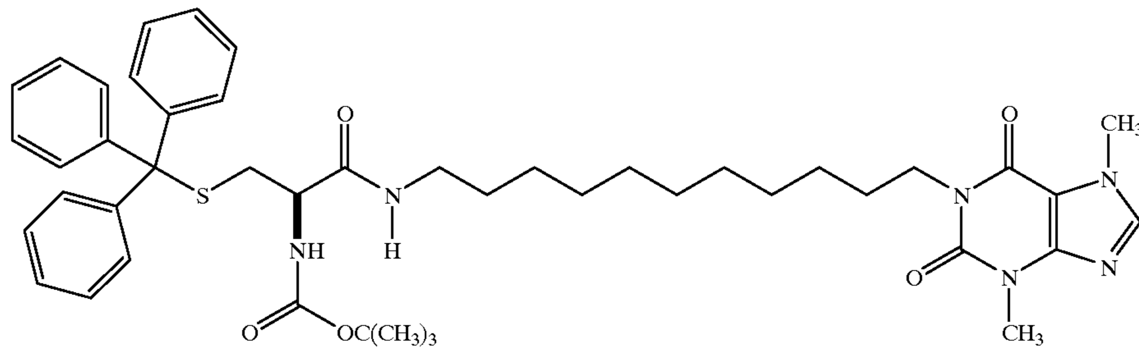
(S)-1-[11-(2-Carbobutoxyamino-3-tritylthiopropionamido)undecyl]-3,7-dimethylxanthine
