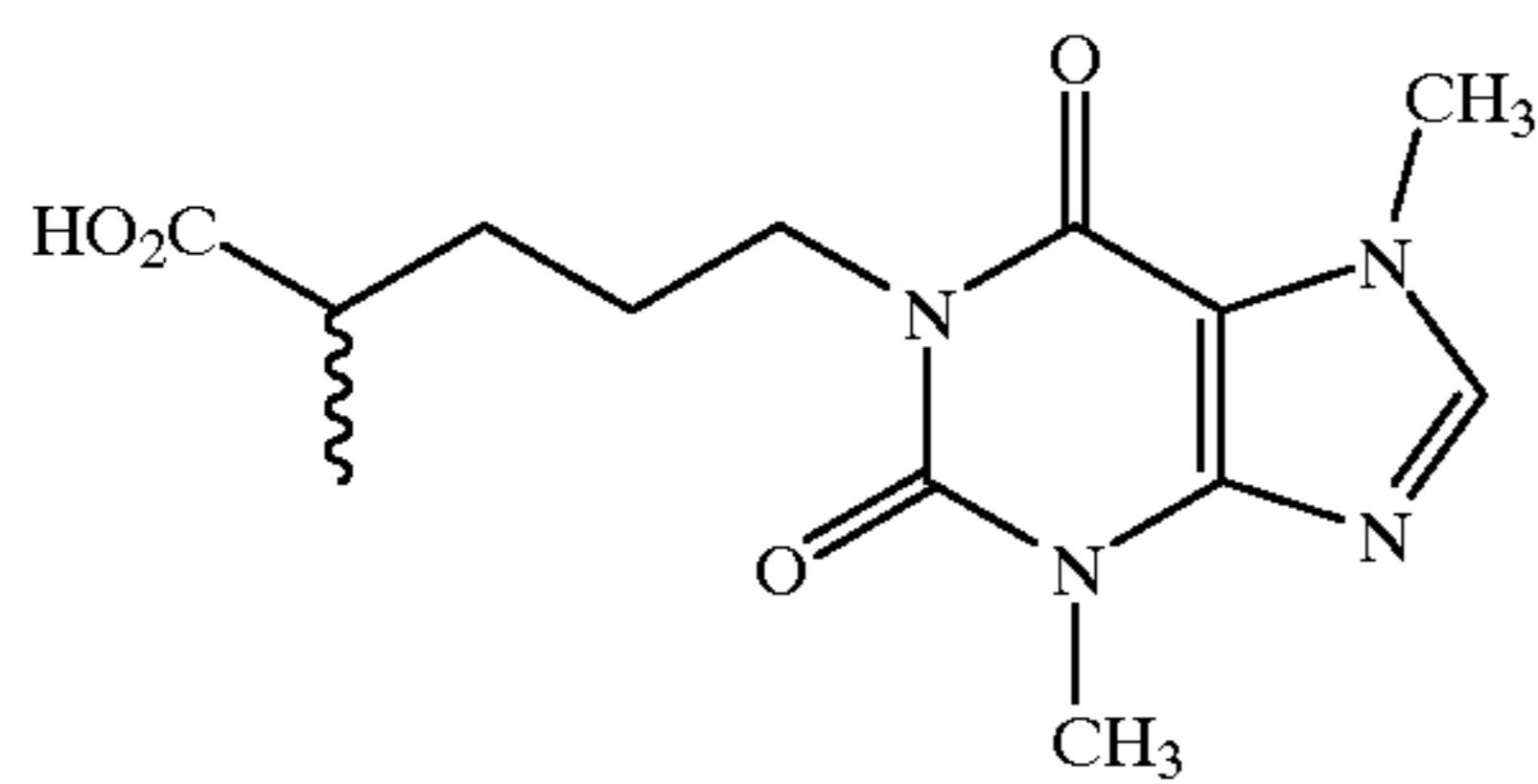
1-(4-Methyl-5-yl-pentanoic acid)-3, 7-dimethylxanthine
