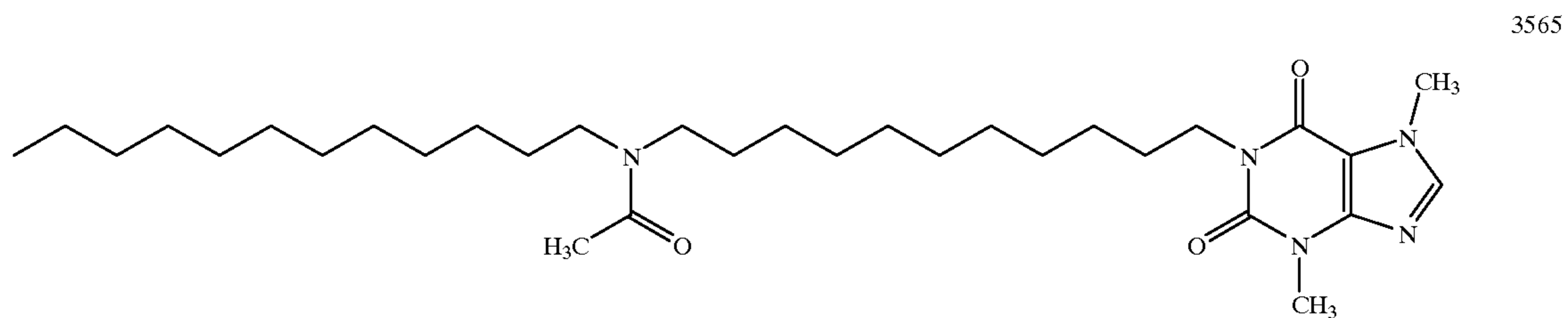
1[11-(N-Dodecylacetamido)undecyl]-3, 7-dimethylxanthine
