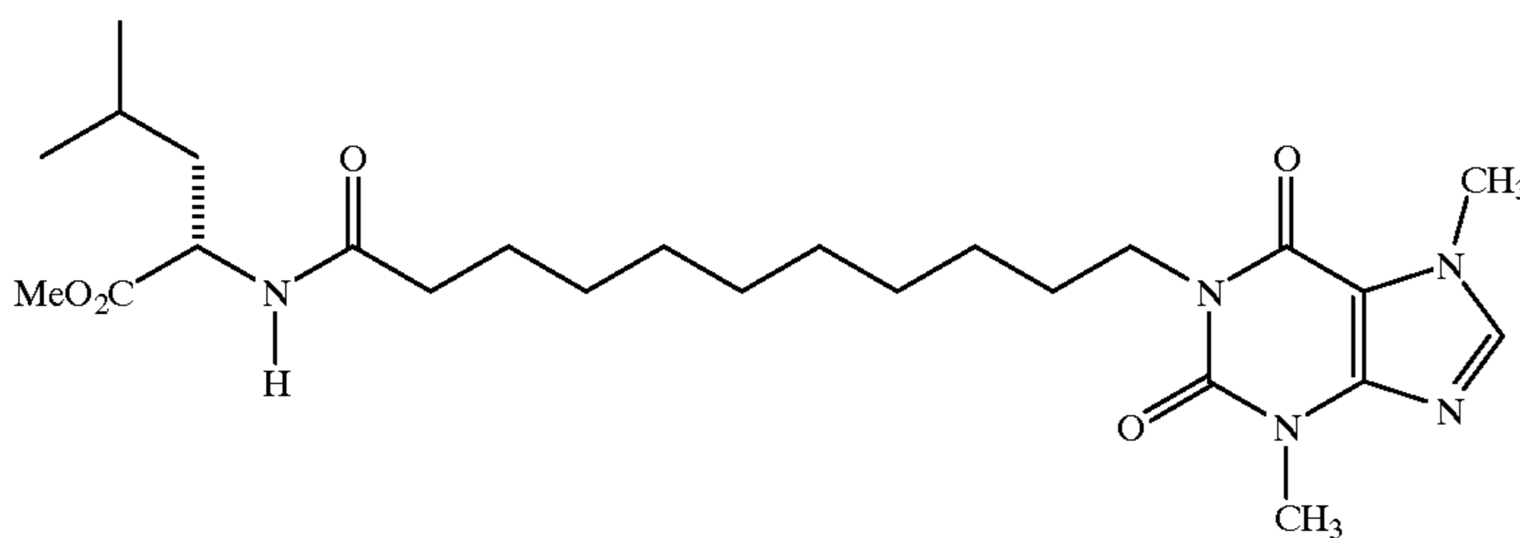
1-[11-(1-Methoxycarbonyl-3-methylbutylamino)-11-oxoundecyl]-3,7-dimethylxanthine
