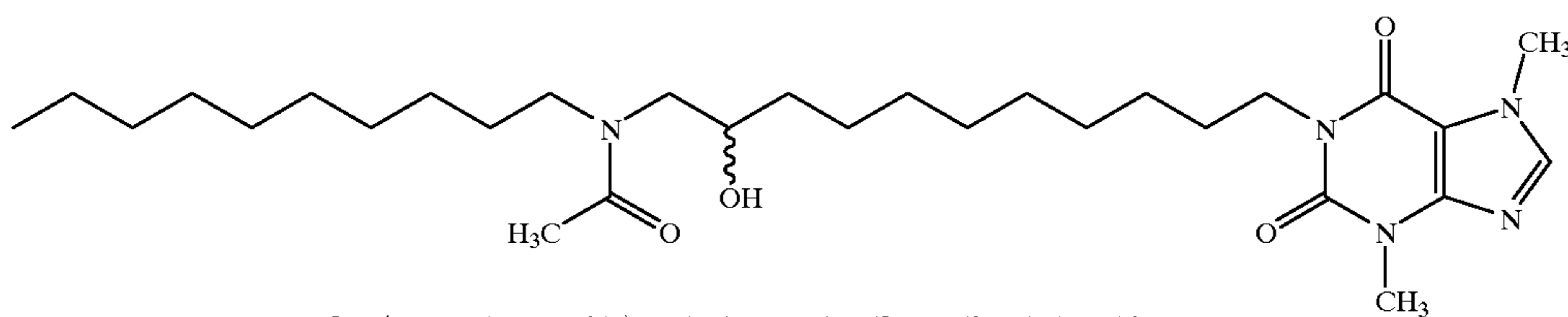
1-[11-(N-Decyl acetamido)-10-hydroxyundecyl]-3,7-dimethylxanthine
