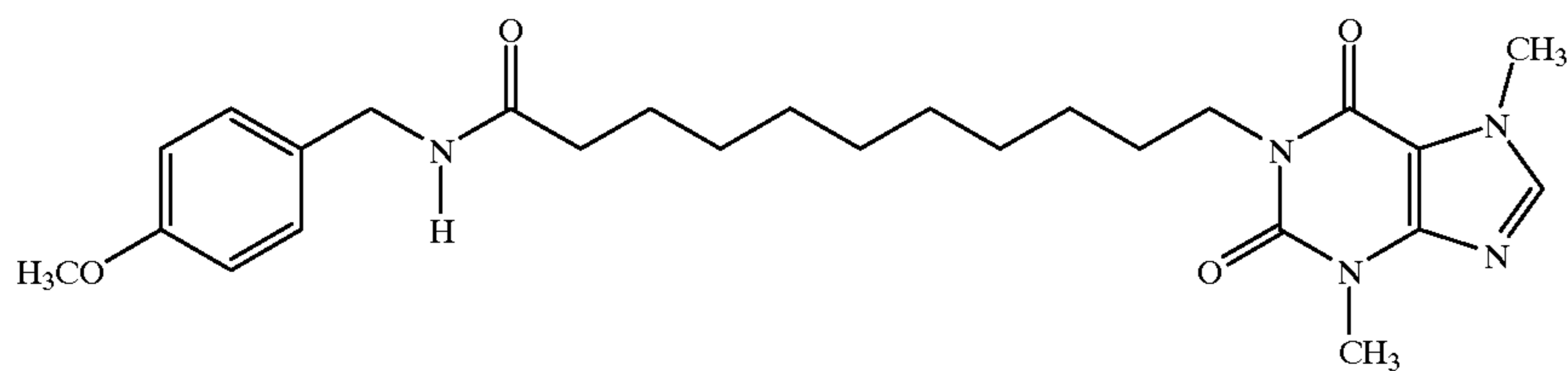
1-[N-(4-methoxybenzyl)-11-yl-undecanamide]-3,7-dimethylxanthine
