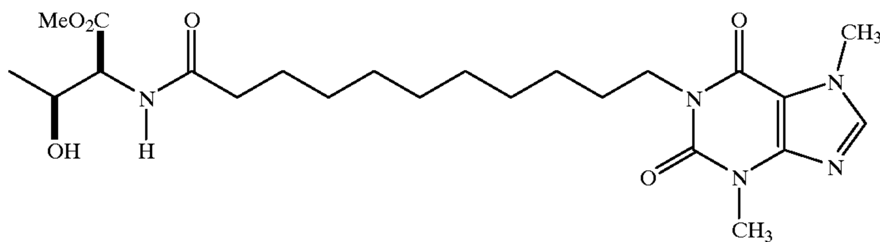
1-[11-(2-Hydroxy-1-methoxycarbonylpropylamino)-11-oxoundecyl]-3,7-dimethylxanthine
