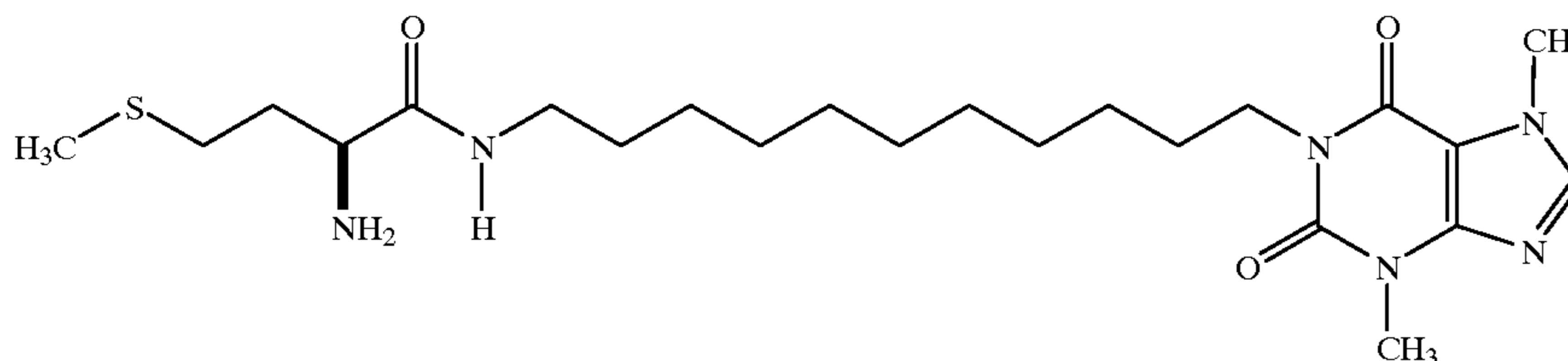
(S)-1-[11-(2-Amino-4-methylthiobutyronamido)undecyl]-3, 7-dimethylxanthine
