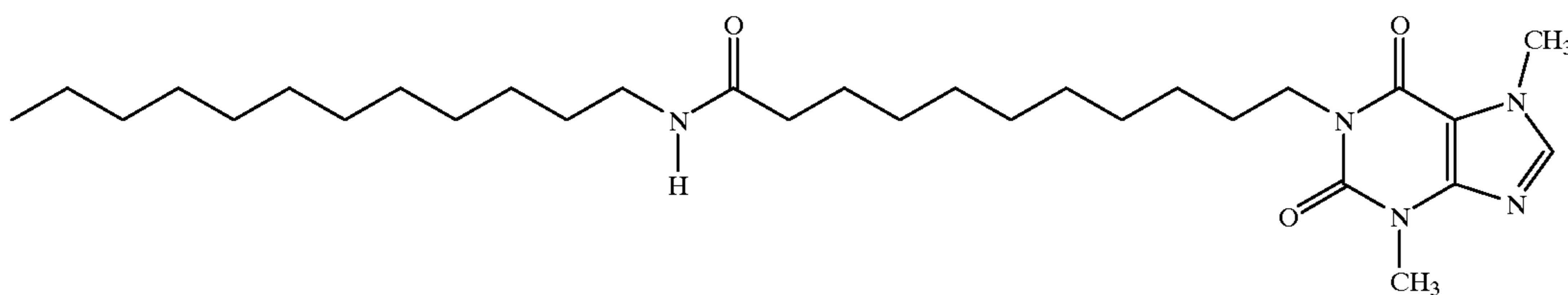
1-(N-Dodecyl-11-yl-undecanamide)-3,7-dimethylxanthine
