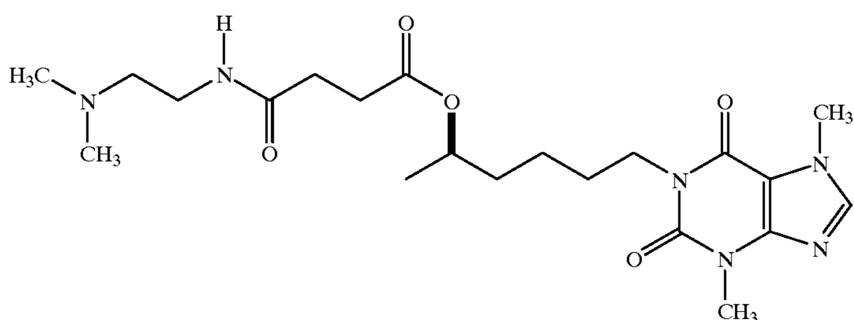
R-1-(5-[[2-(Dimethylamino)ethyl]amino]-1,4-dioxobutyl]oxy)hexyl)-3,7-dimethylxanthine
