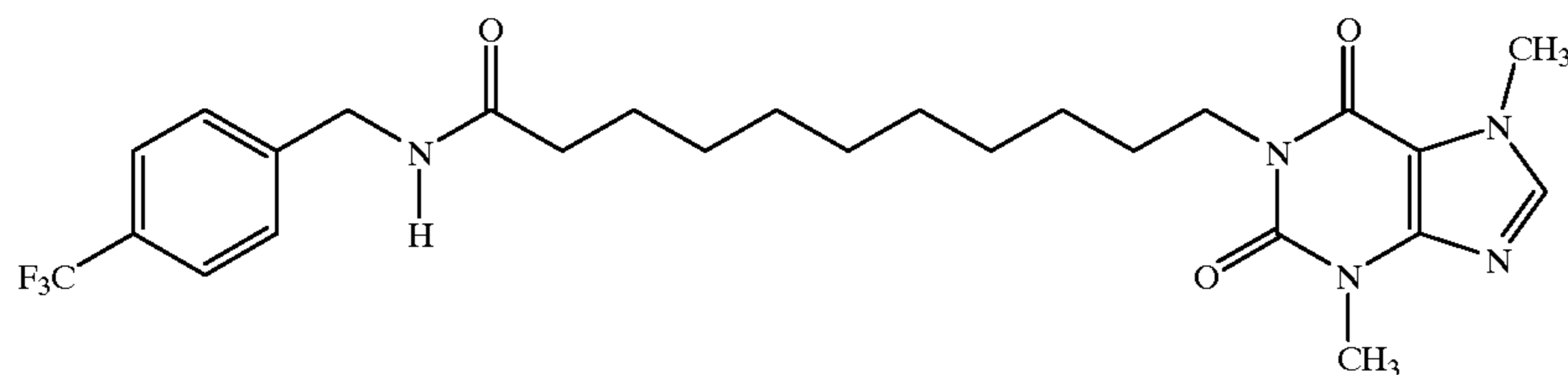
1-[N-(4-Trifluoromethylbenzyl)-11-yl-undecanamide]-3, 7-dimethylxanthine
