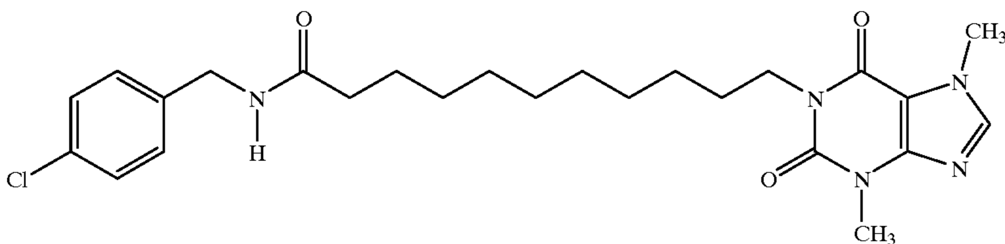
1-[N-(4-Chlorobenzyl)-11-yl-undecanamide]-3,7-dimethylxanthine
