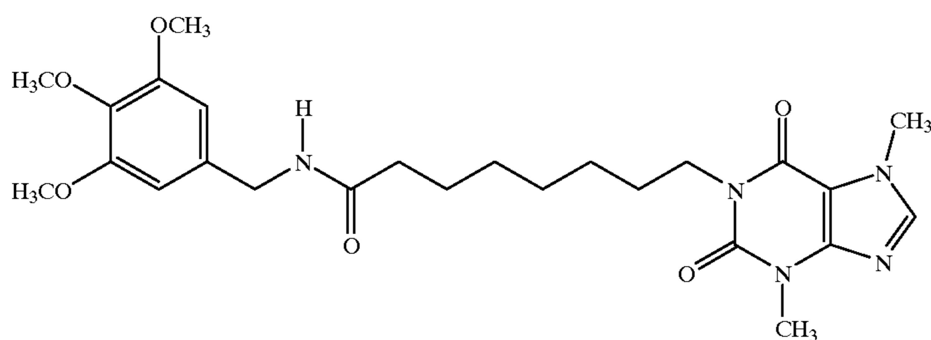
1-[N-(3,4,5-Trimethoxybenzyl)-8-yl-octanamide]-3,7-dimethylxanthine
