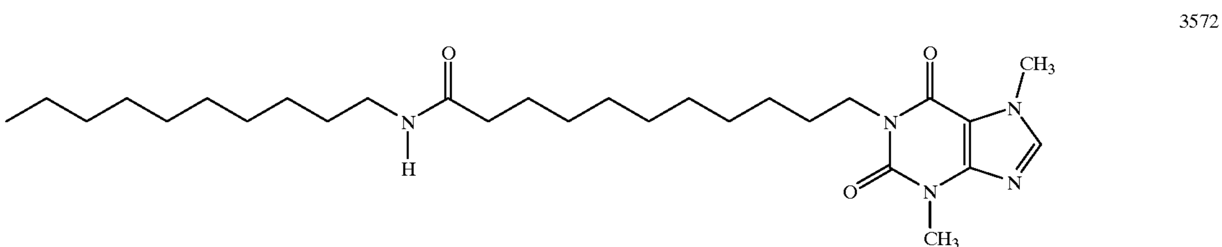
1-(N-Decyl-11-yl-undecanamide)-3, 7-dimethylxanthine
