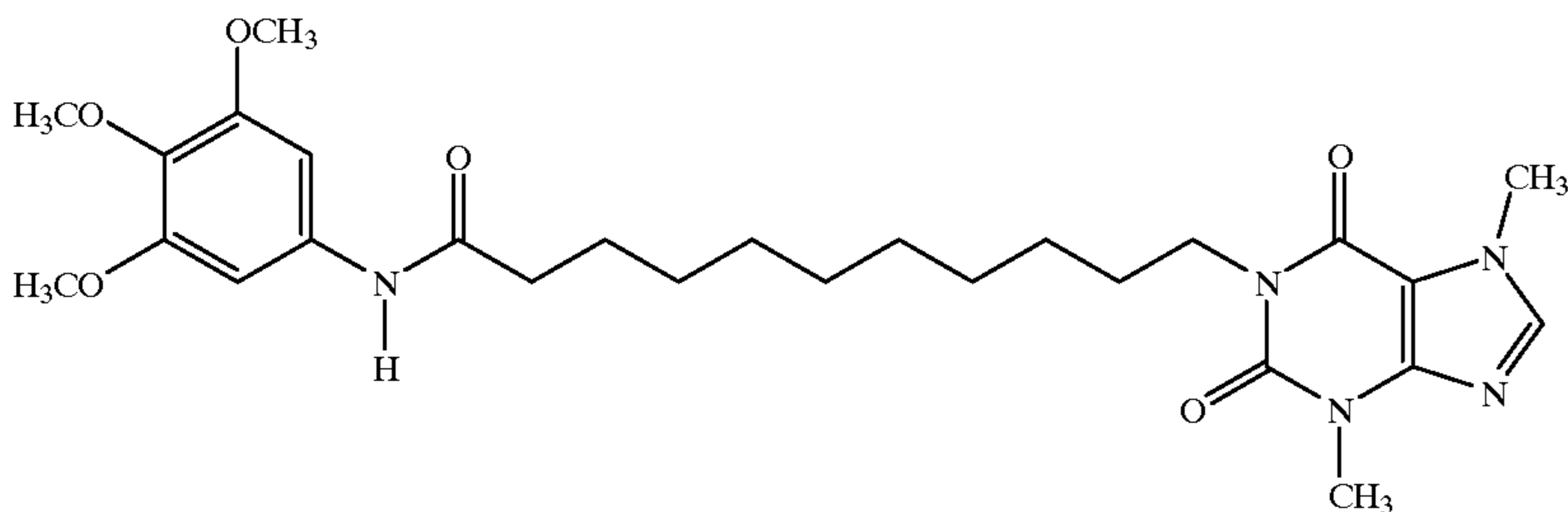
1-[N-(3,4,5-Trimethoxyphenyl)-11-yl-undecanamide]-3,7-dimethylxanthine
