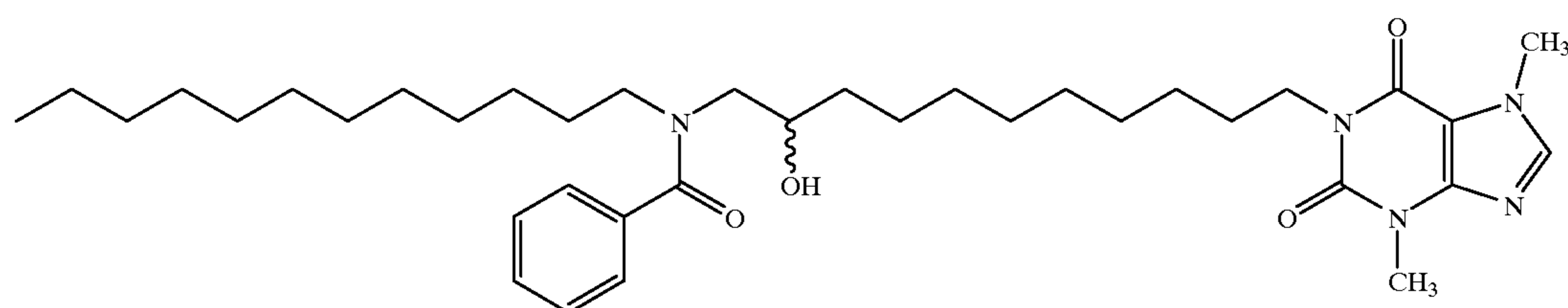
1-[11-(Dodecyl benzamido)-10-hydroxyundecyl]-3,7-dimethylxanthine
