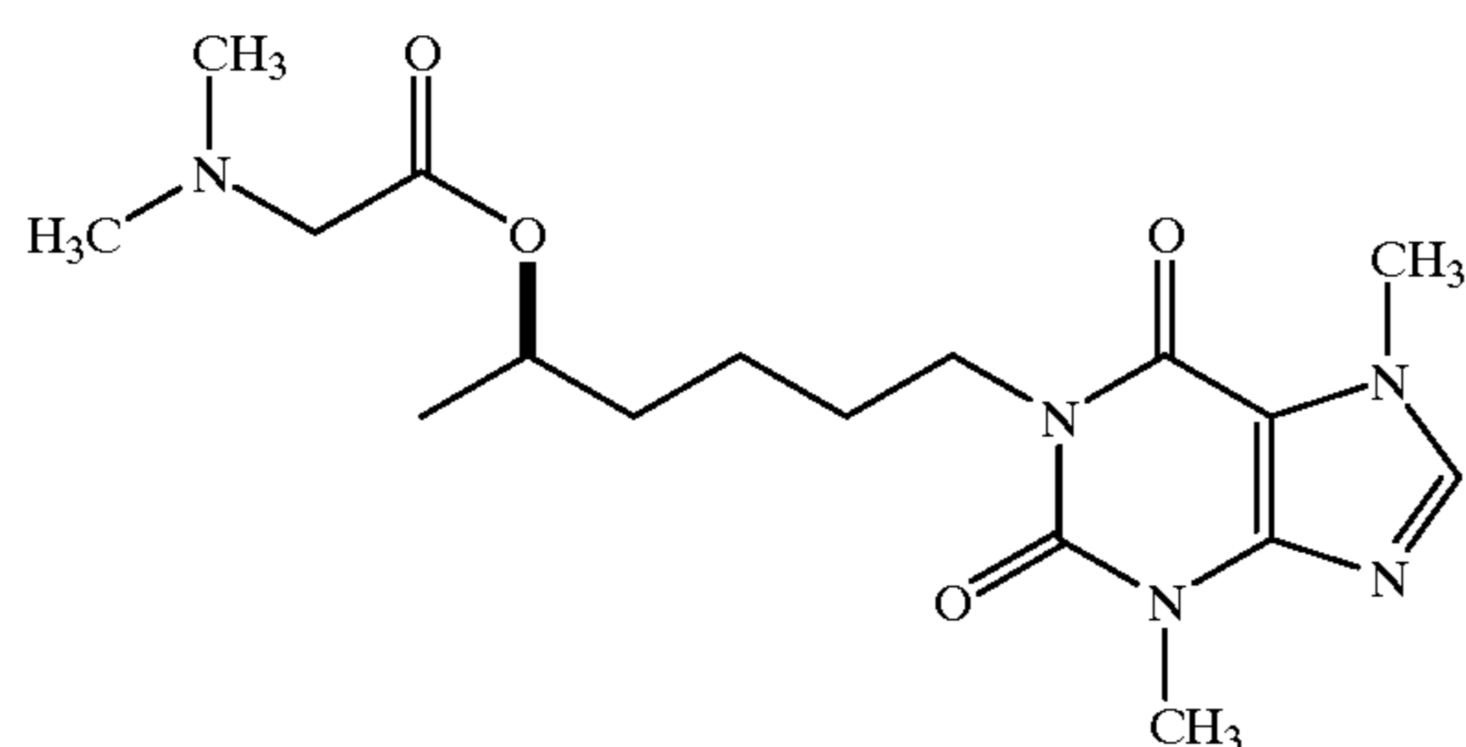
R-1-(5-Hydroxy)hexyl)-3,7-dimethylxanthine N,N-dimethylglycinate
