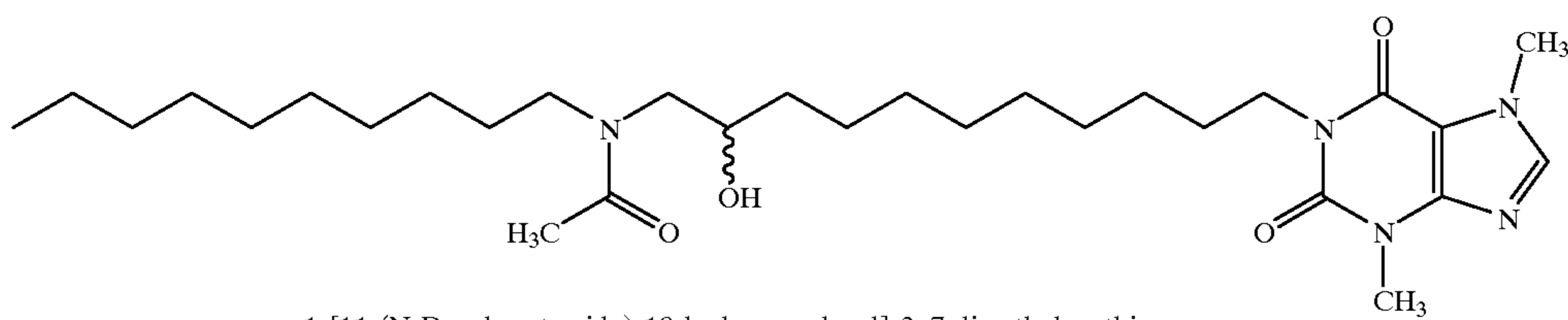
1-[11-(N-Decyl acetamido)-10-hydroxyundecyl]-3,7-dimethylxanthine
