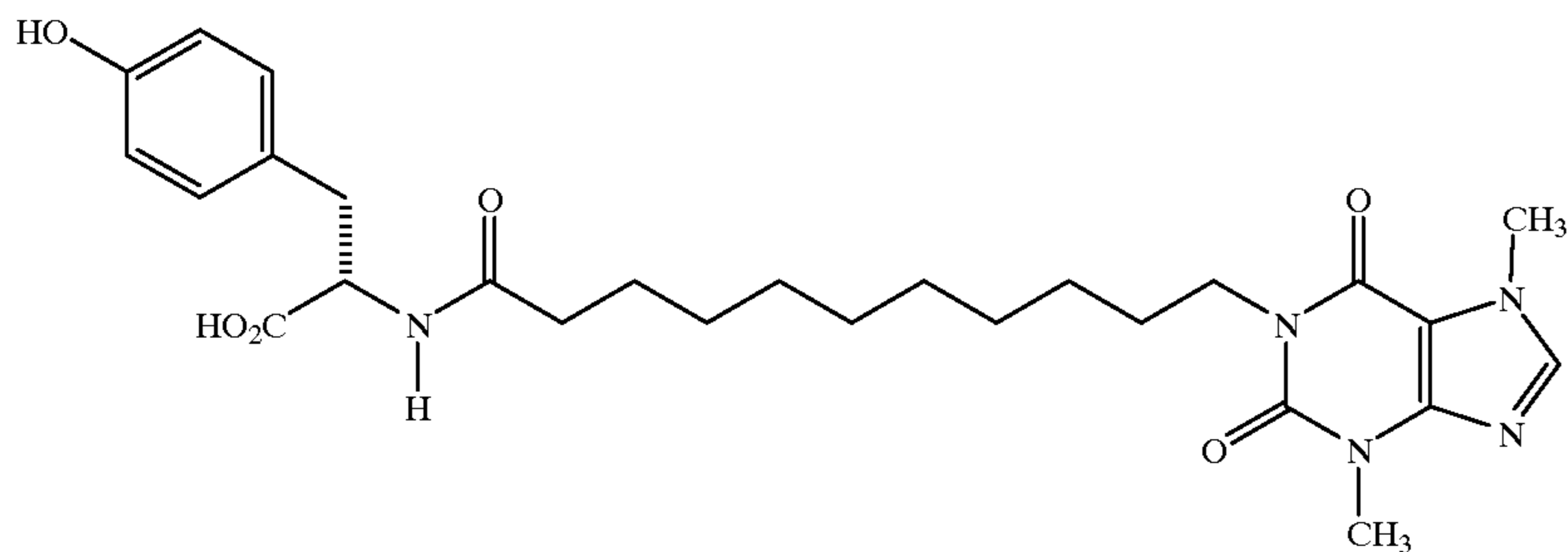
(S)-1-(11-[1-Carboxy-2-(4-hydroxyphenyl)ethylamino]-11-oxoundecyl)-3,7-dimethylxanthine
