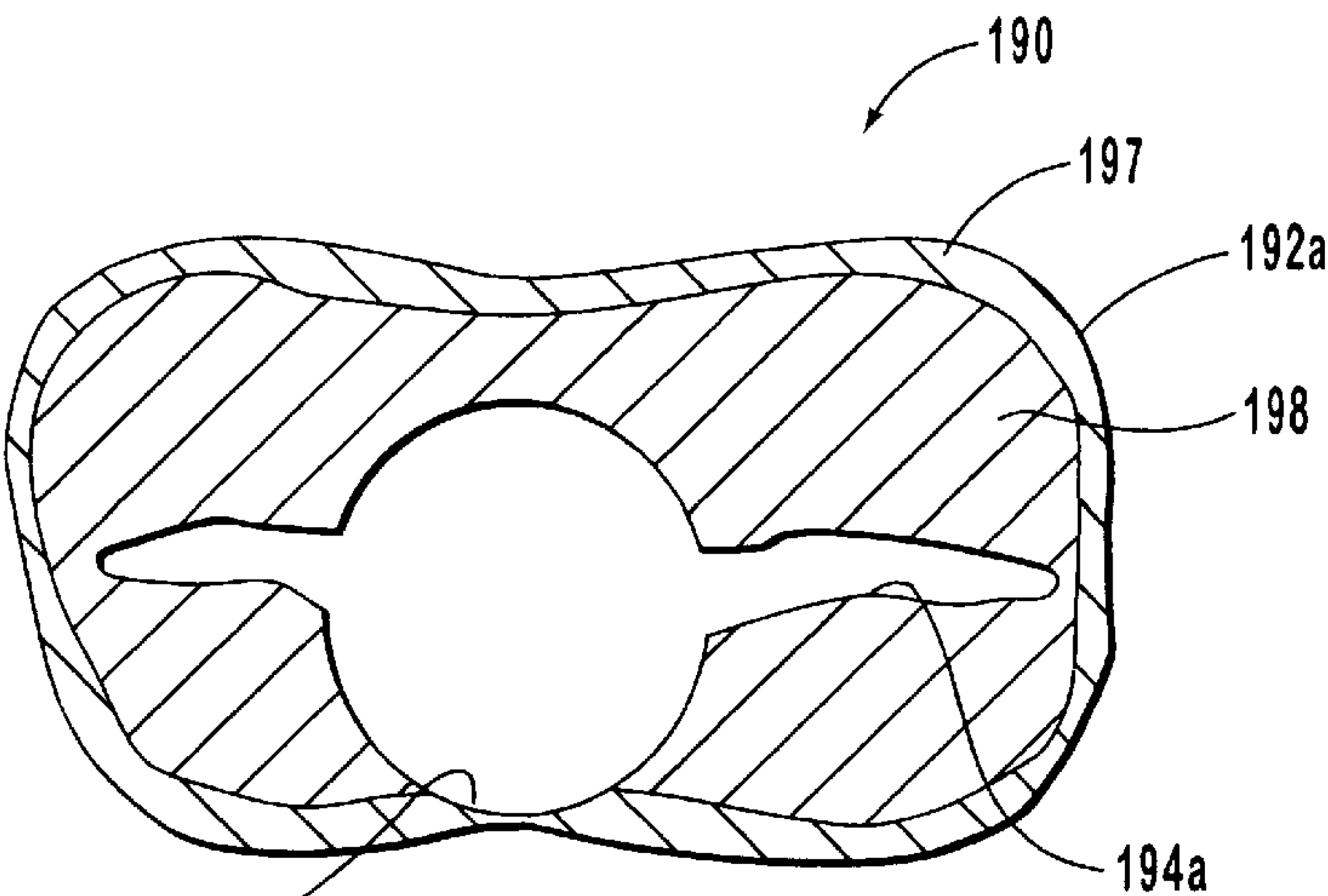
FIG. 15C (PRIOR ART)
