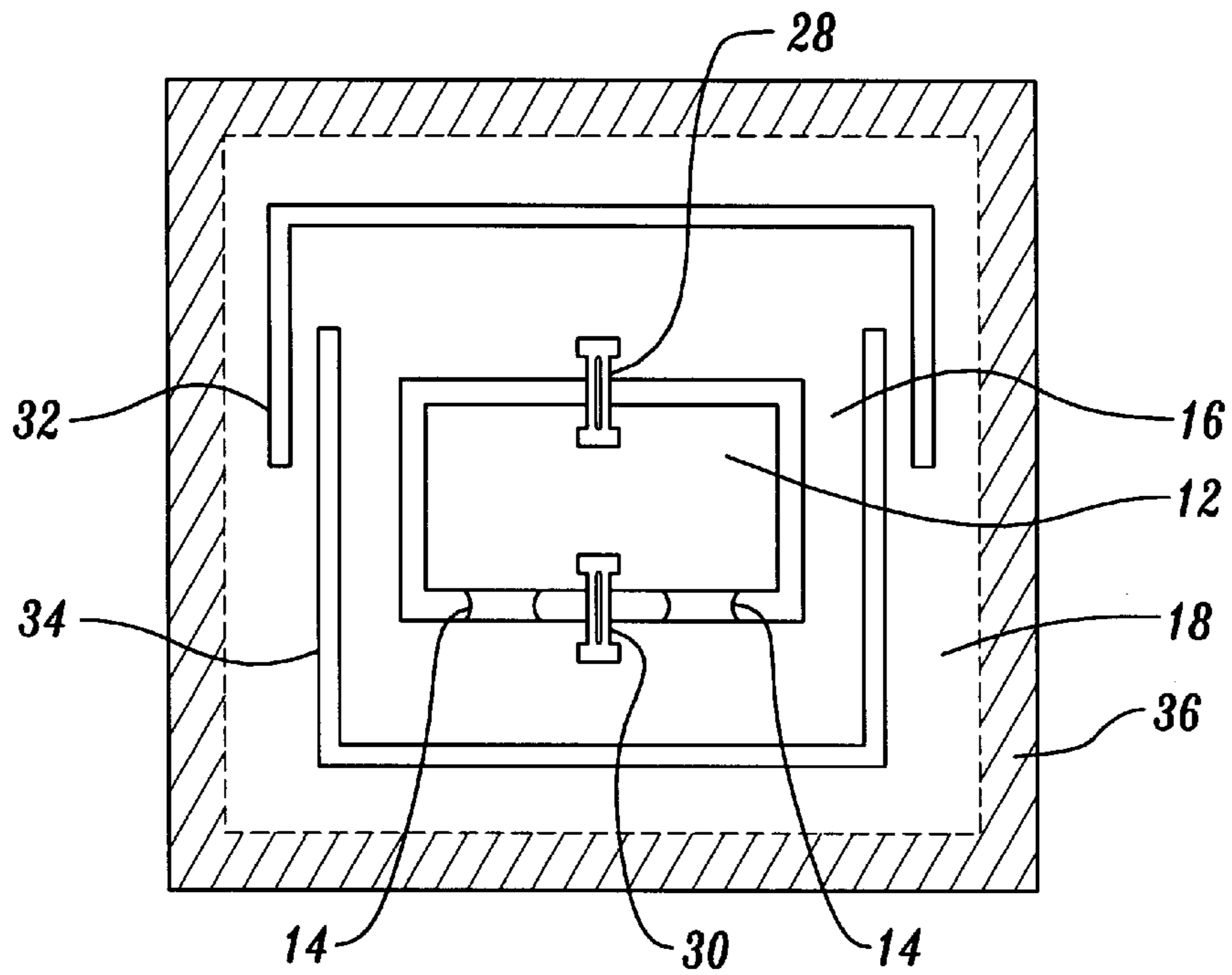
Fig. 2 (PRIOR ART)
