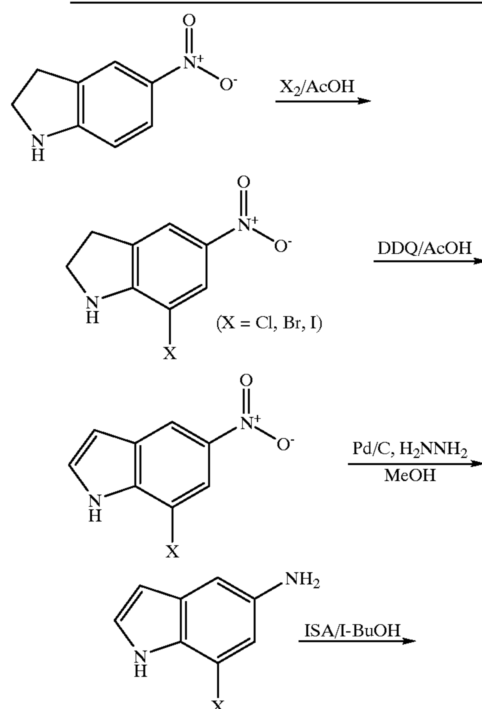
Scheme 1 illustrates schematically the synthesis of 7-substituted derivatives of 5-(2-imidazolin-2ylamino) indole.
