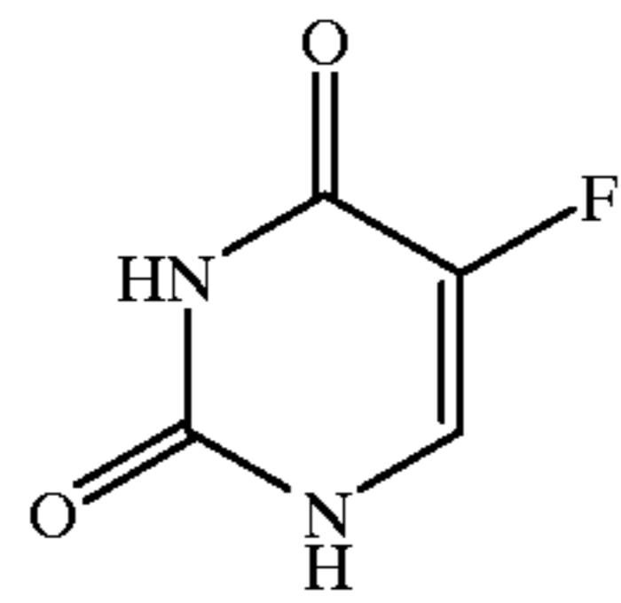
Fluorouracil (5-FU)
