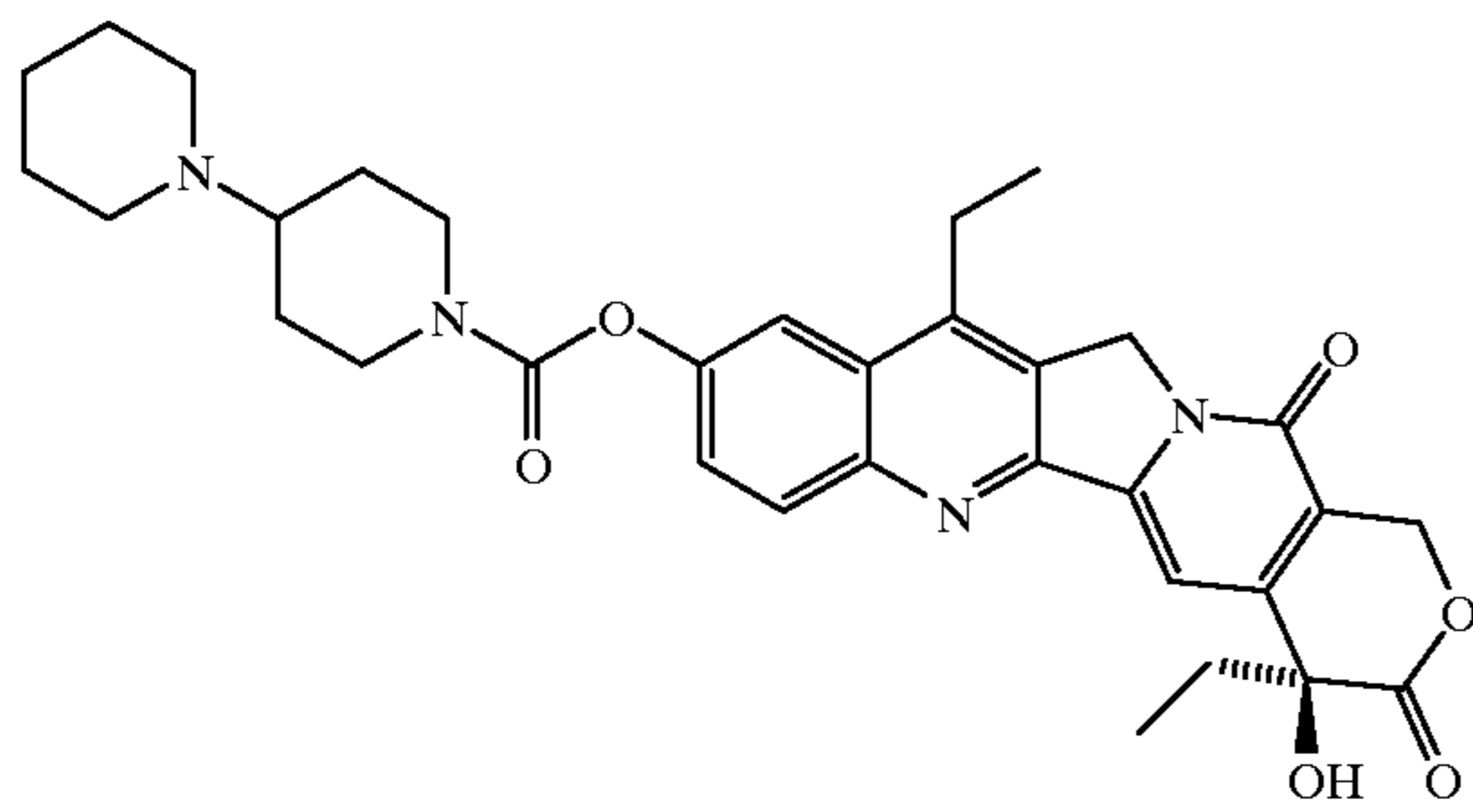
Irinotecan
