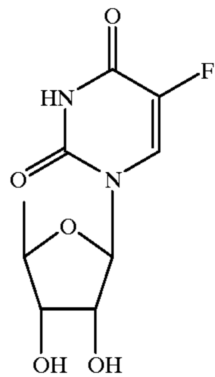
5'-deoxyfluorouridin
