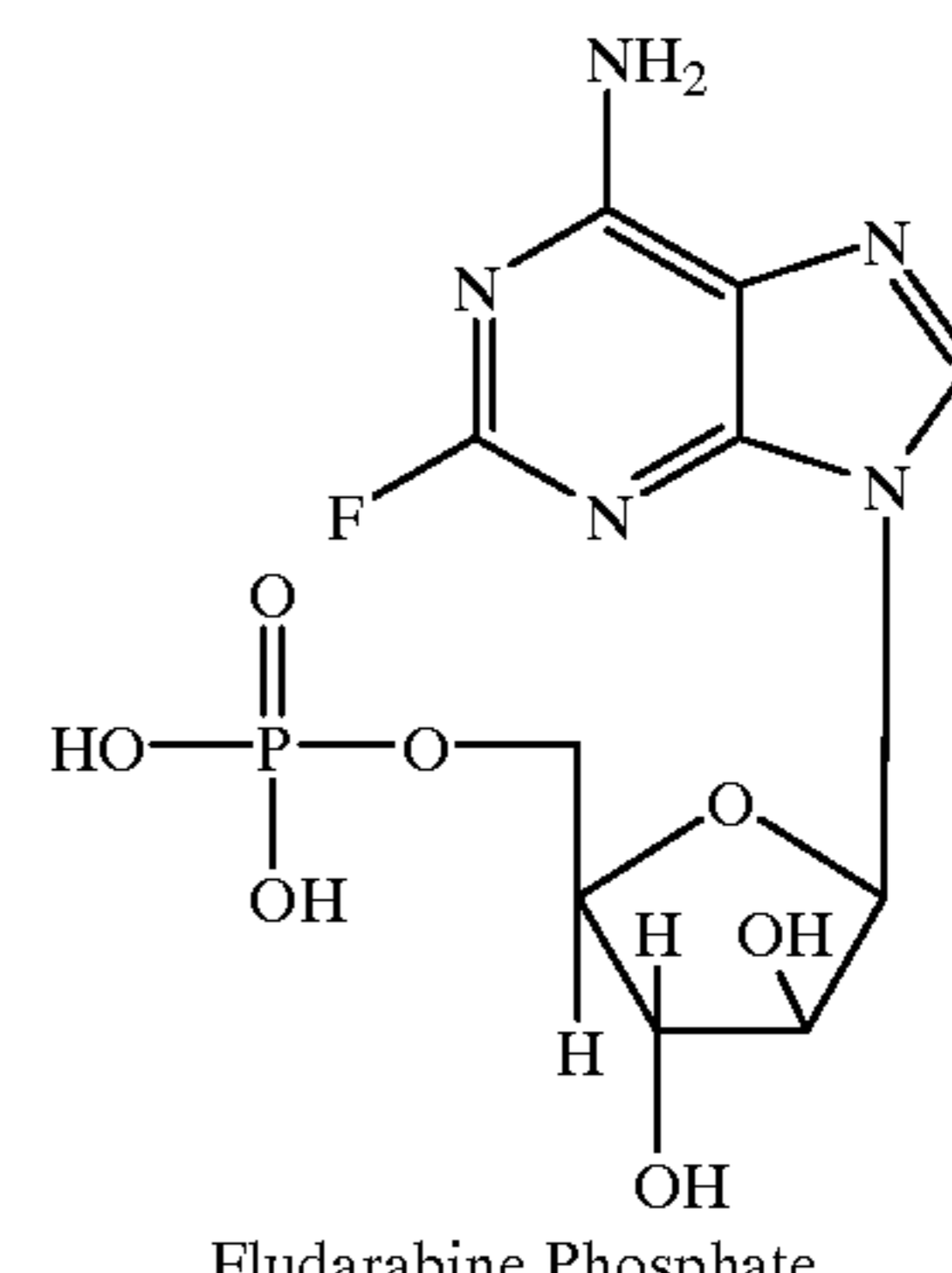
Fludarabine Phosphate
