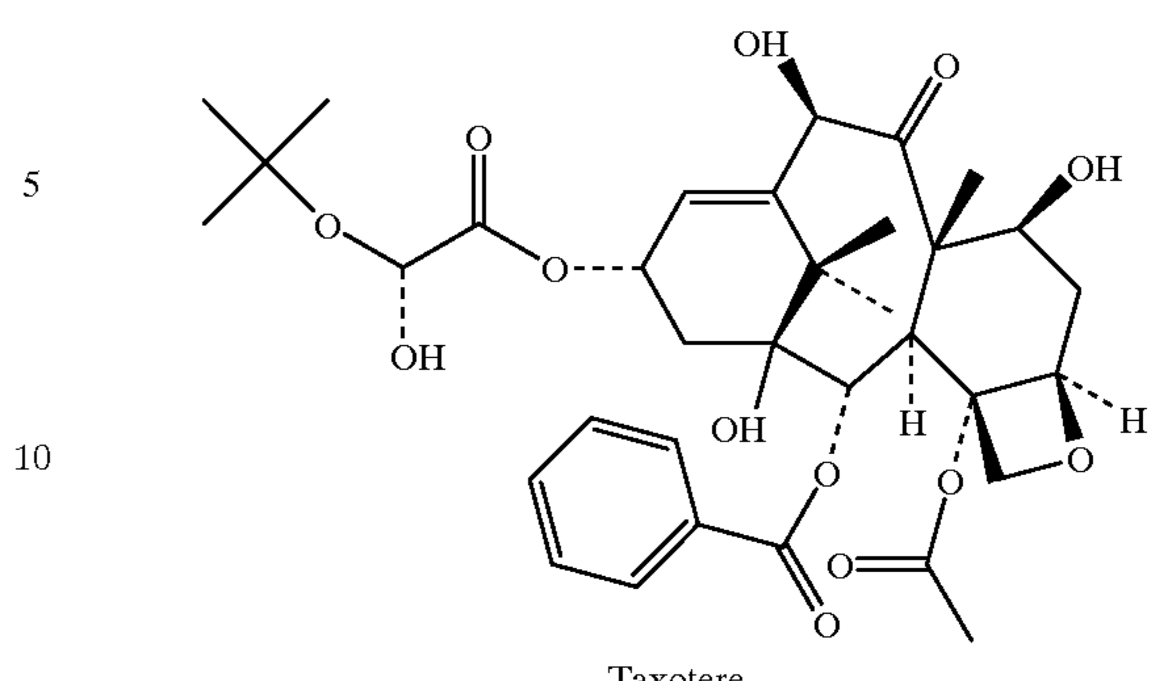
Taxotere
