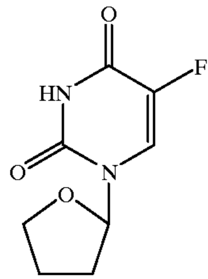
Ftorafur
