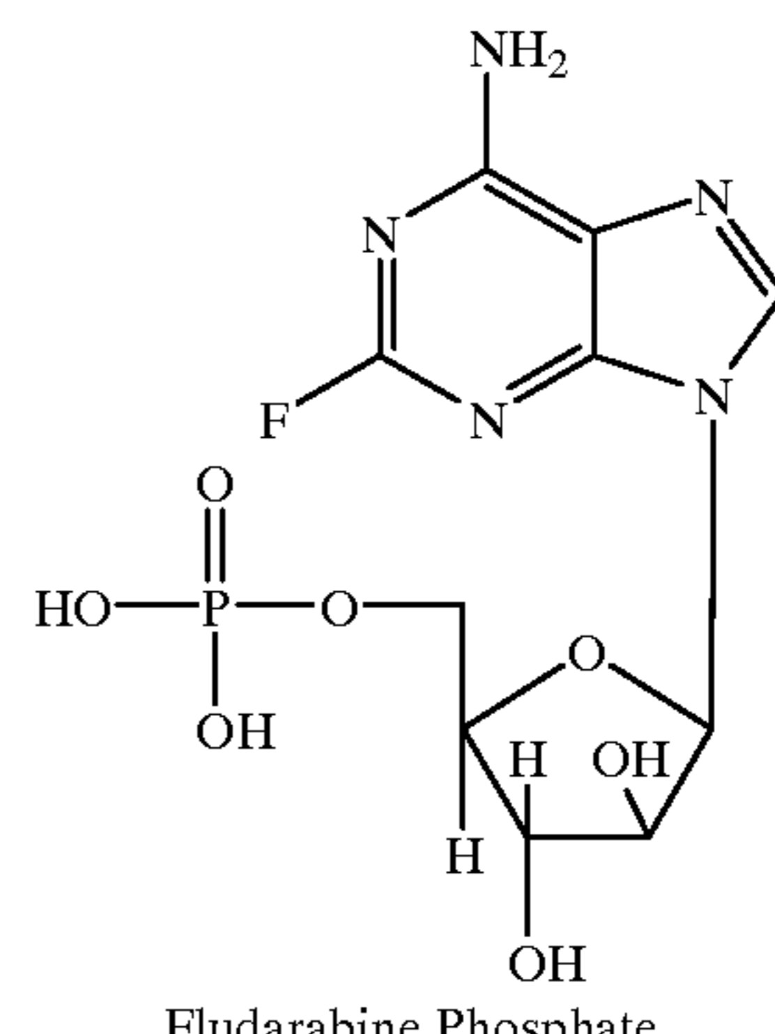
Fludarabine Phosphate
