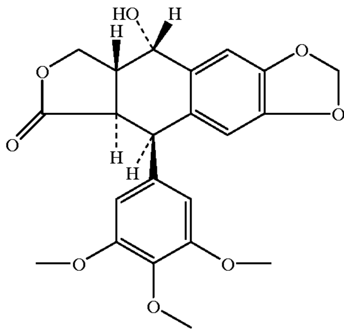
Podophyllotoxin
