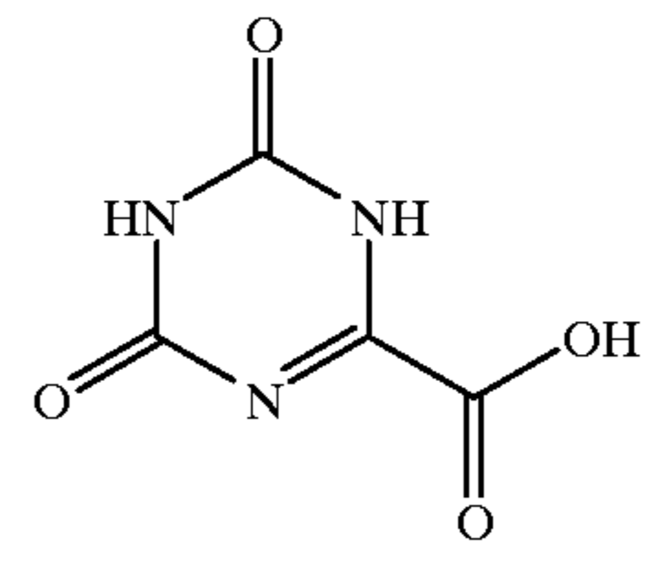
Oxonic Acid
