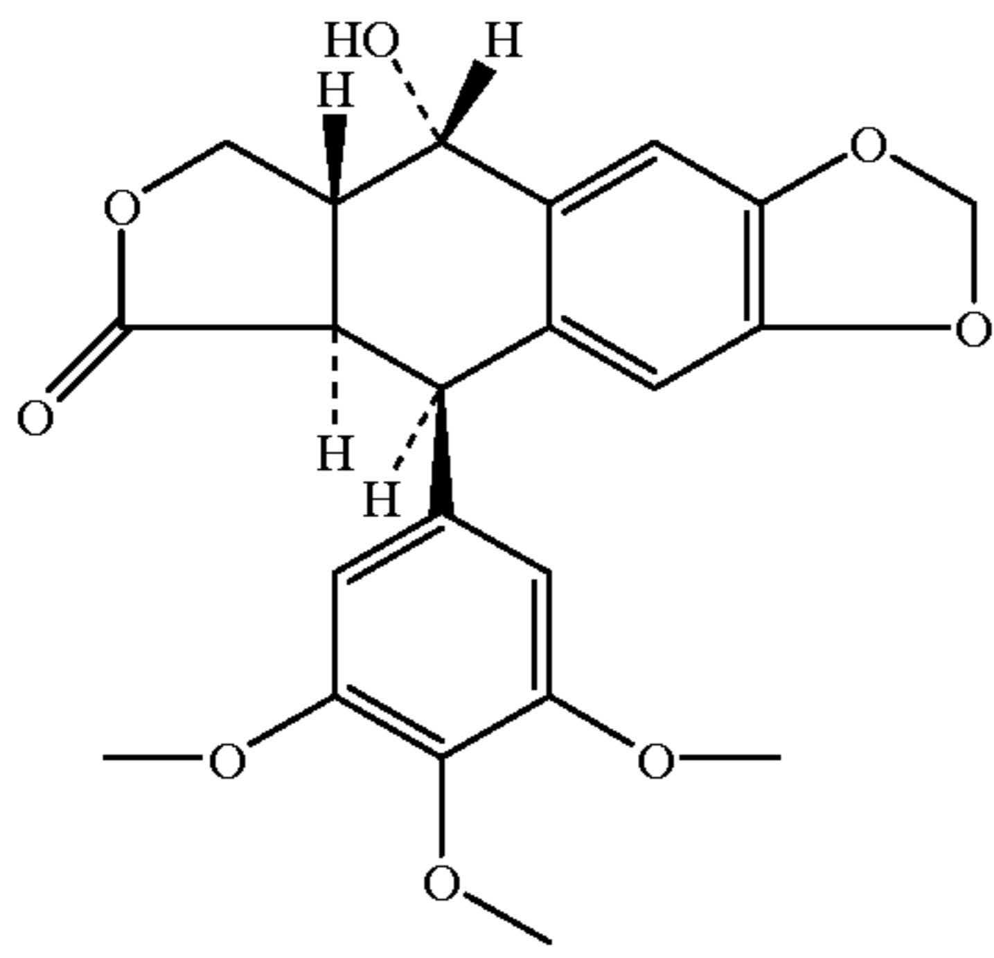
Podophyllotoxin
