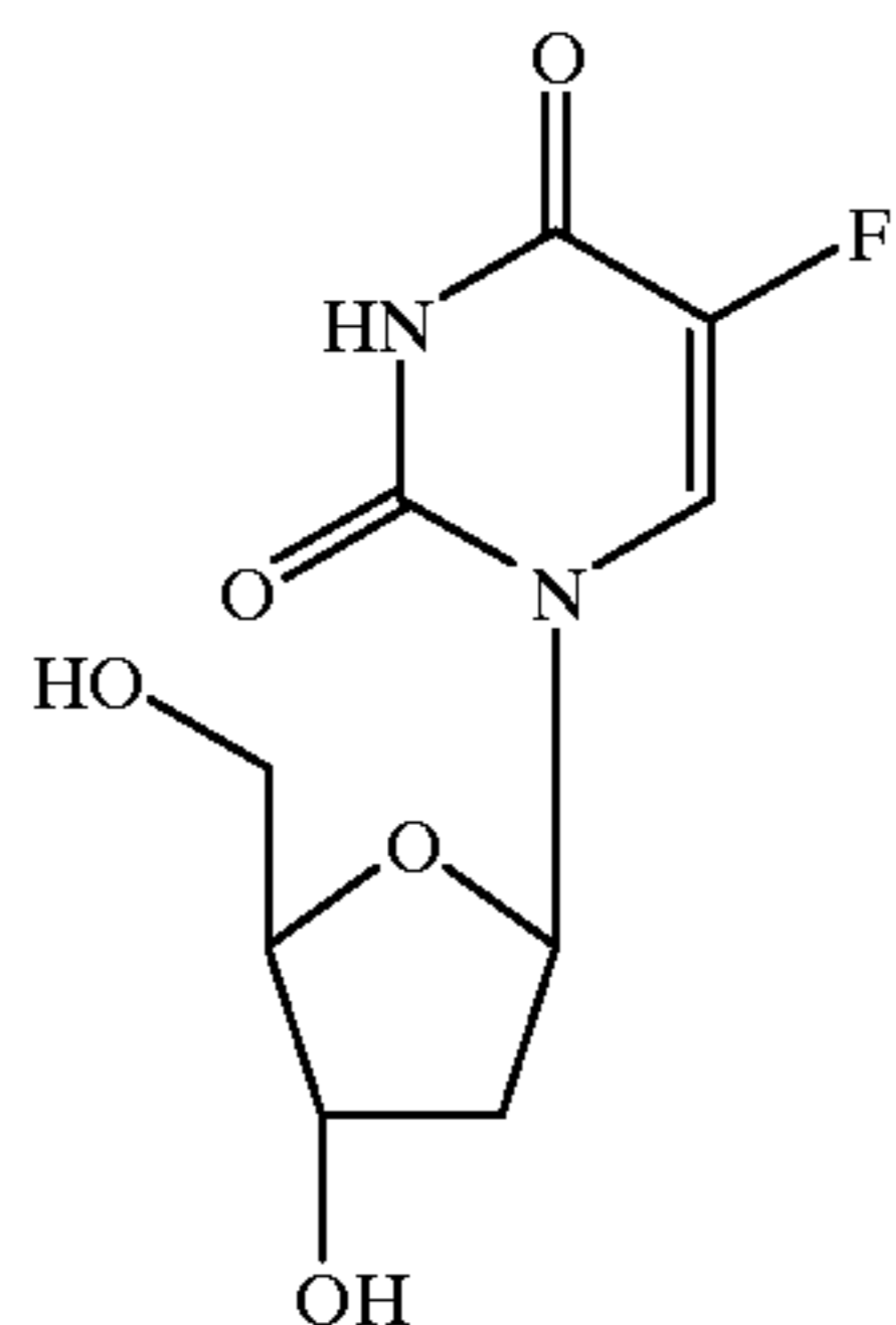
Floxuridine
