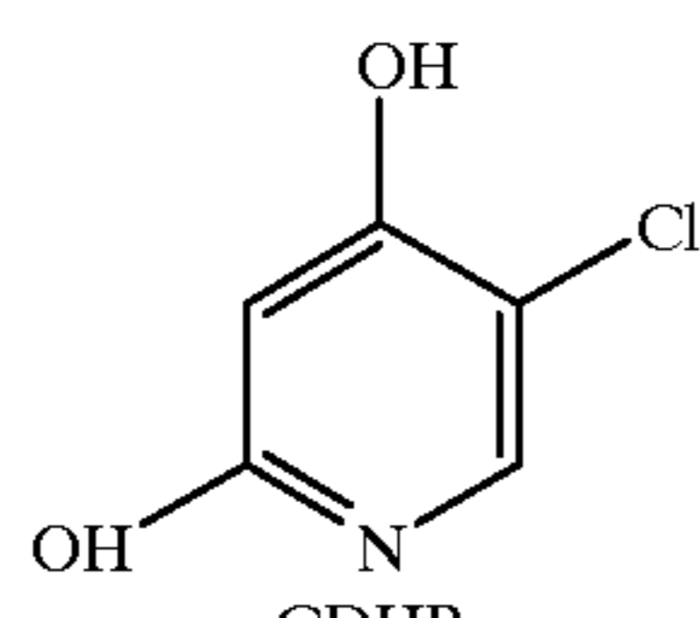
CDHP
