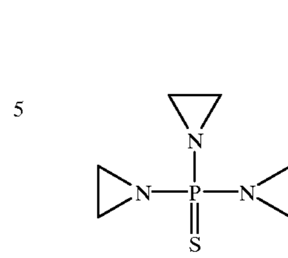
Thiotepa
