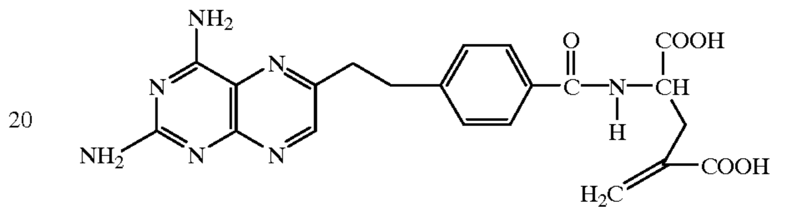
\gamma -methylene-10-deaza aminopterin (MDAM)
