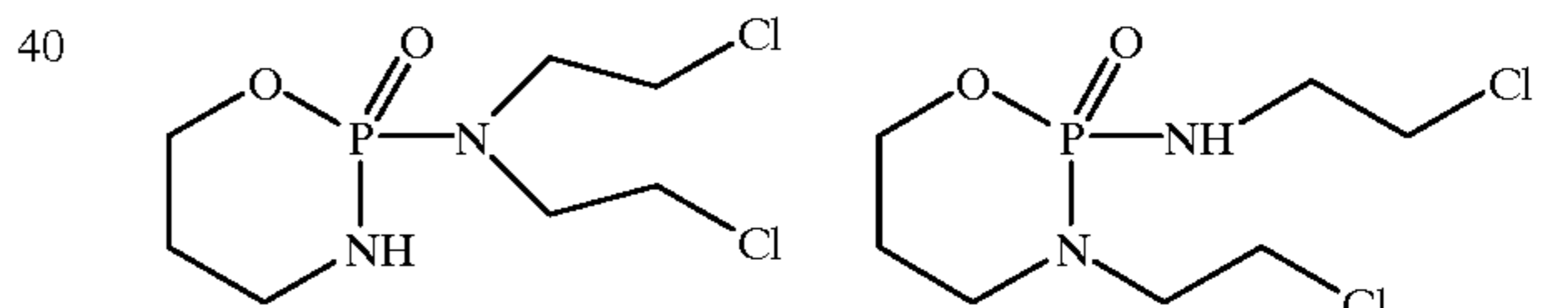
Cyclophosphamide
