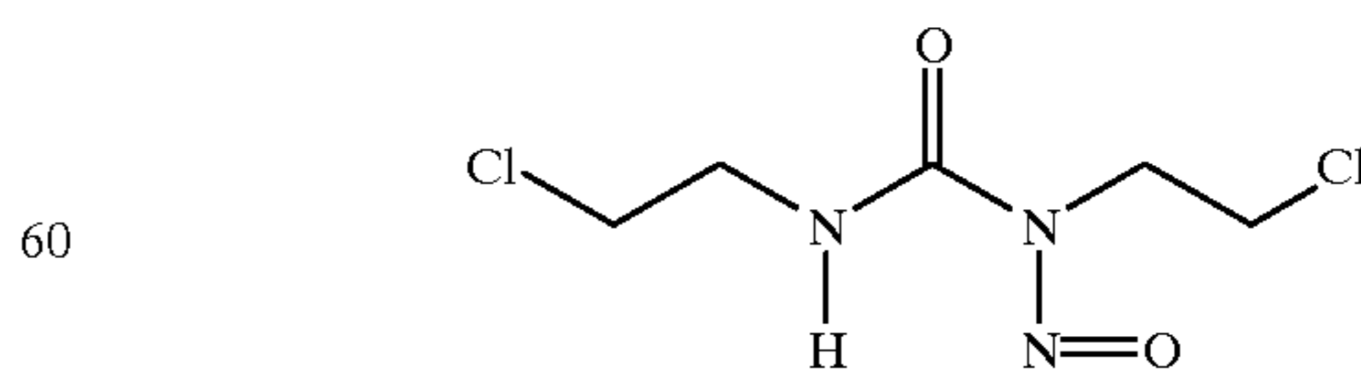
Carmustine (BCNU)
