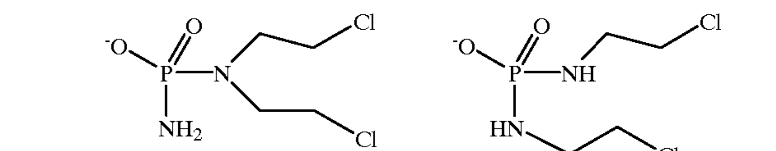
Phosphoramidate Mustard
