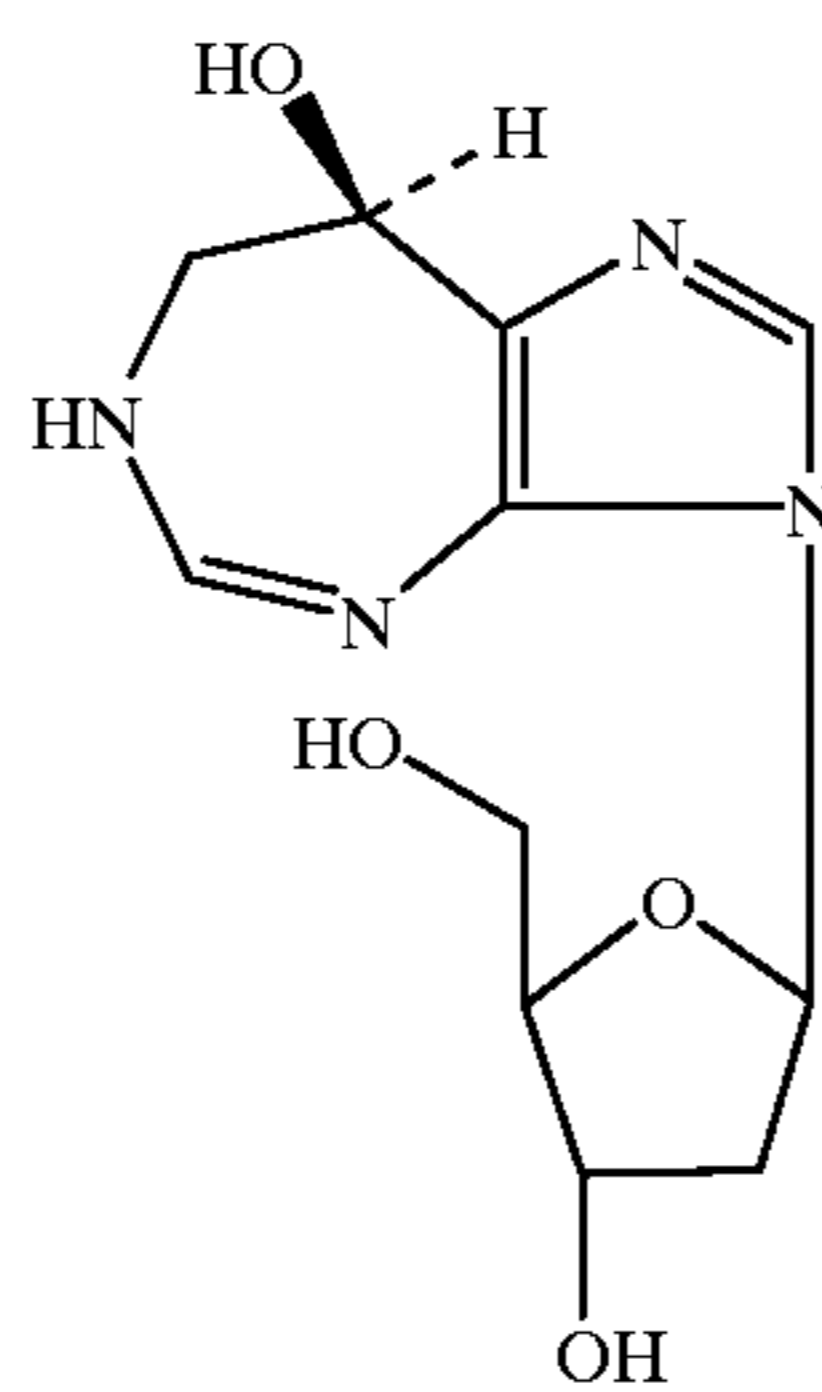
Pentostatin
