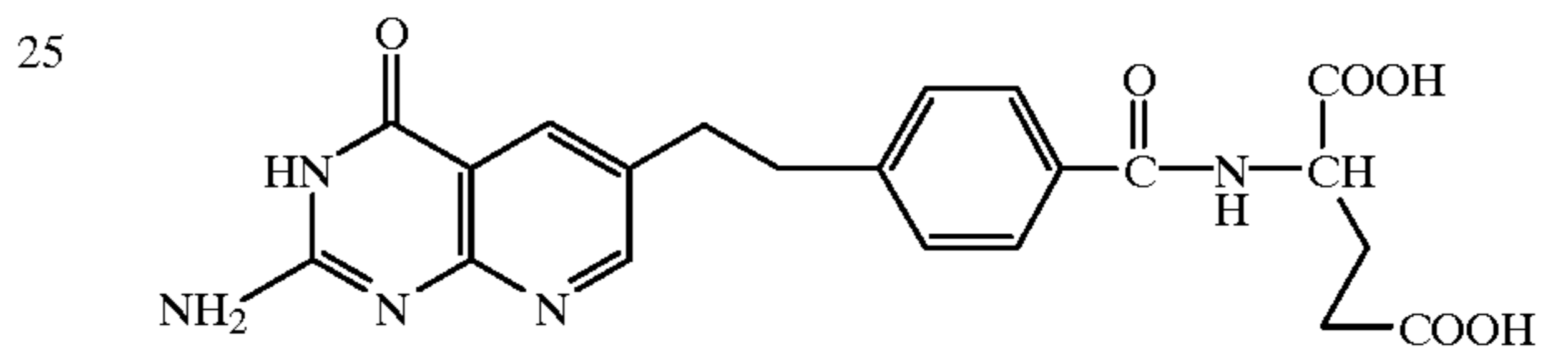
5, 10-dideaza tetrahydrofolate
