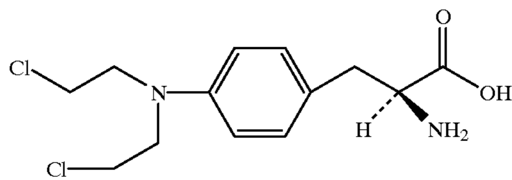
Melphalan
