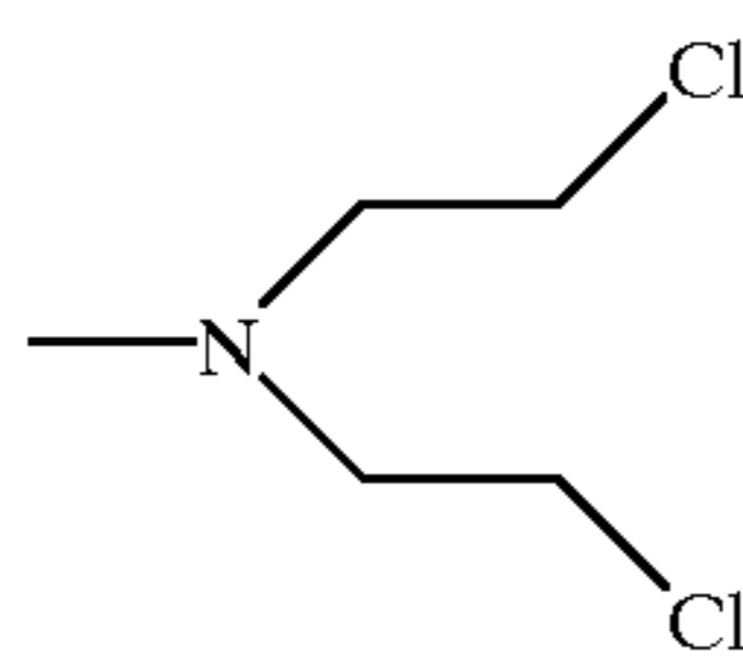
Mechlorethamine
