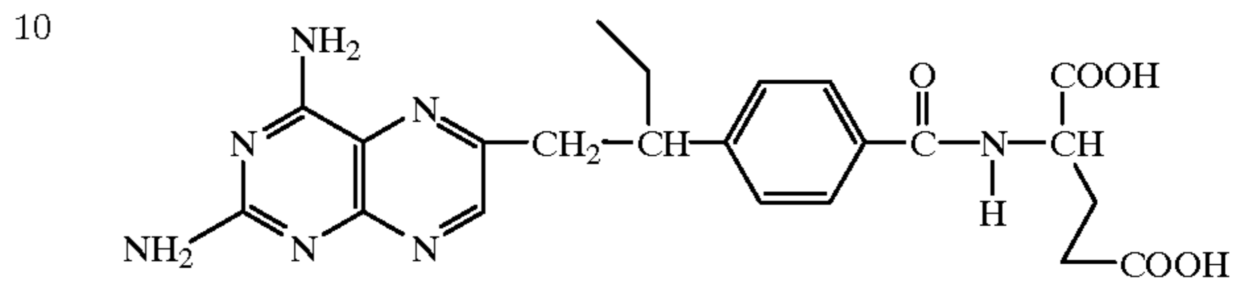
10-ethyl-10-deaza aminopterin (EDAM)
