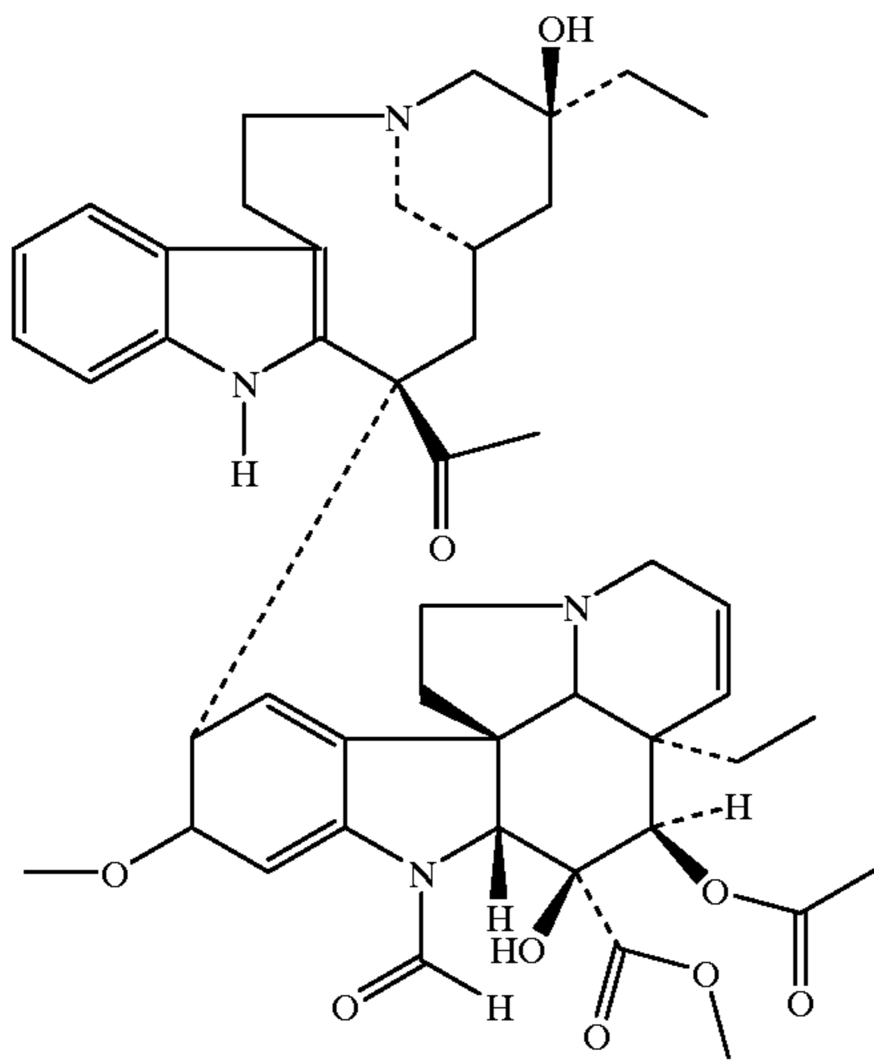
Vincristine
