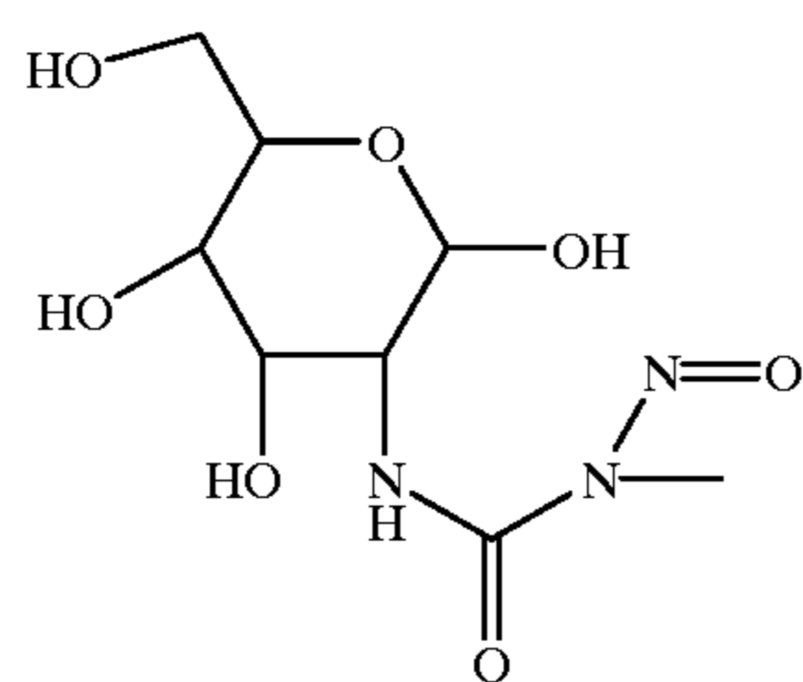
Streptozocin
