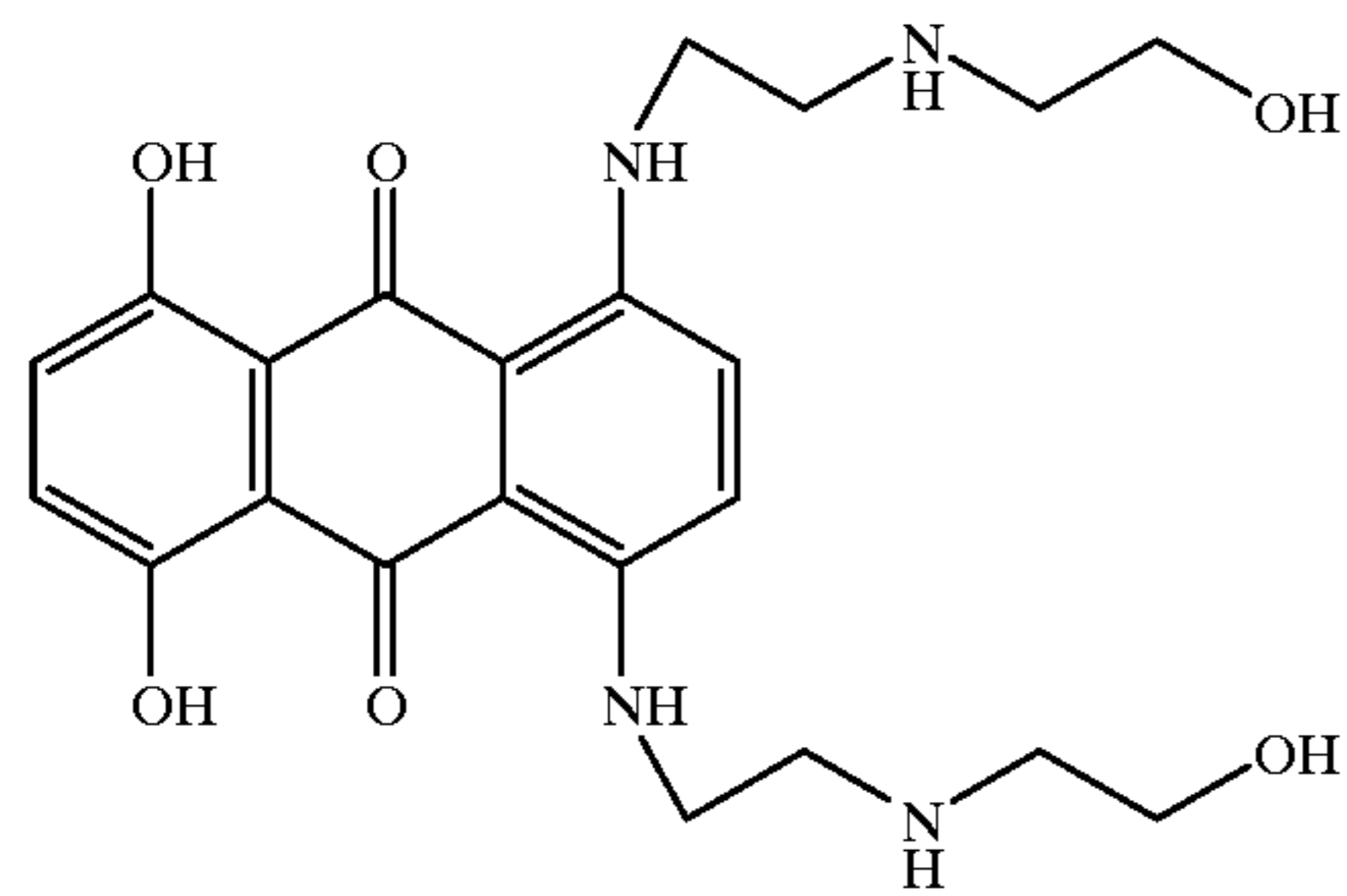
Mitoxantrone
