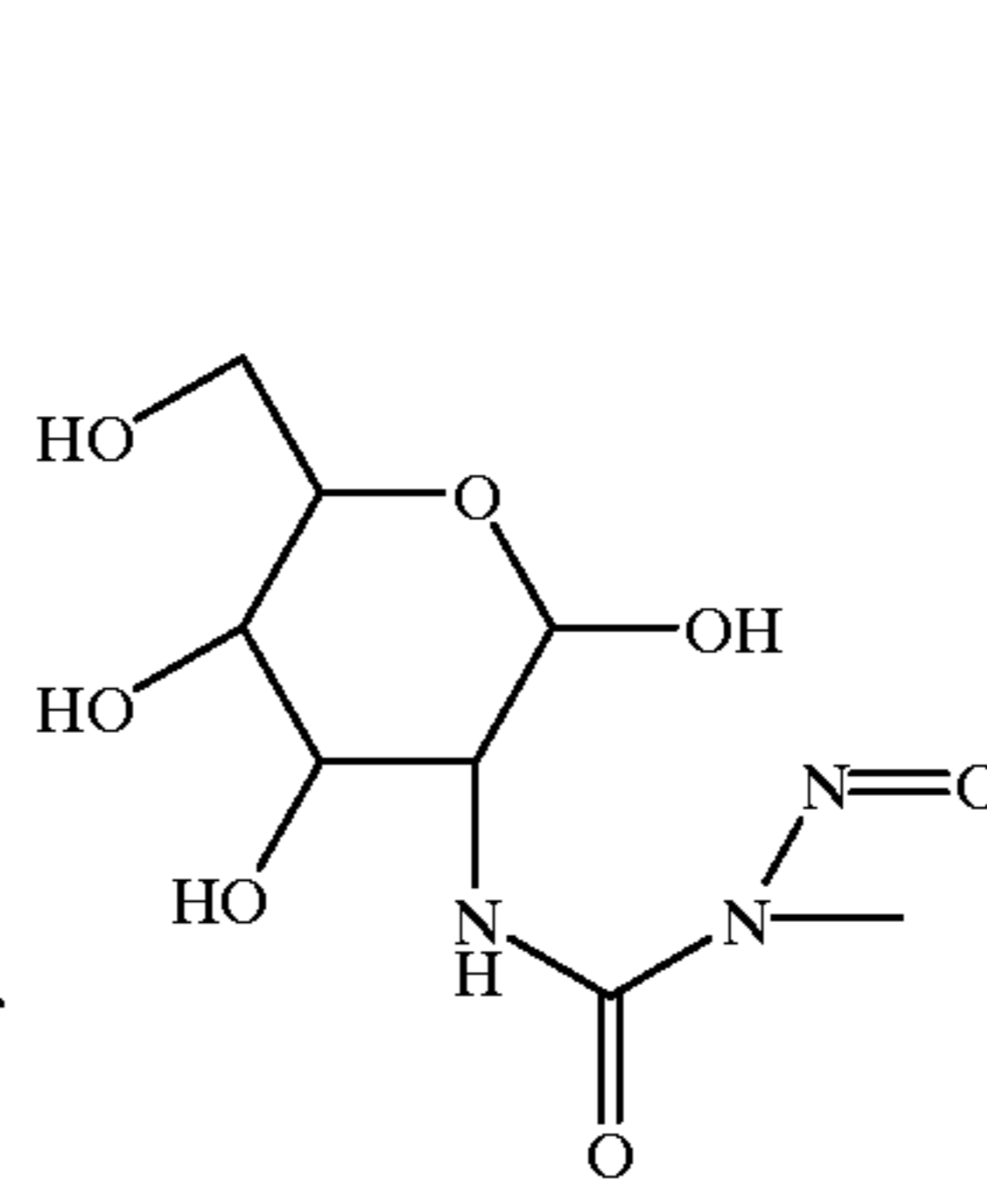
Streptozocin
