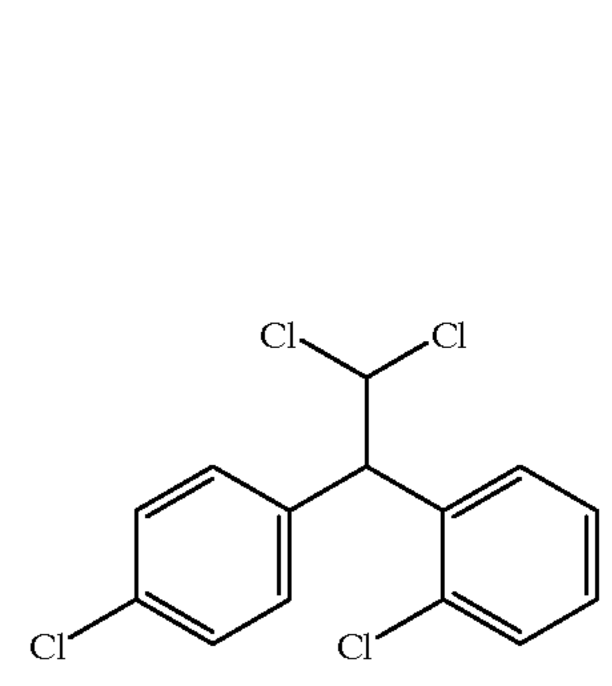
Mitotane
