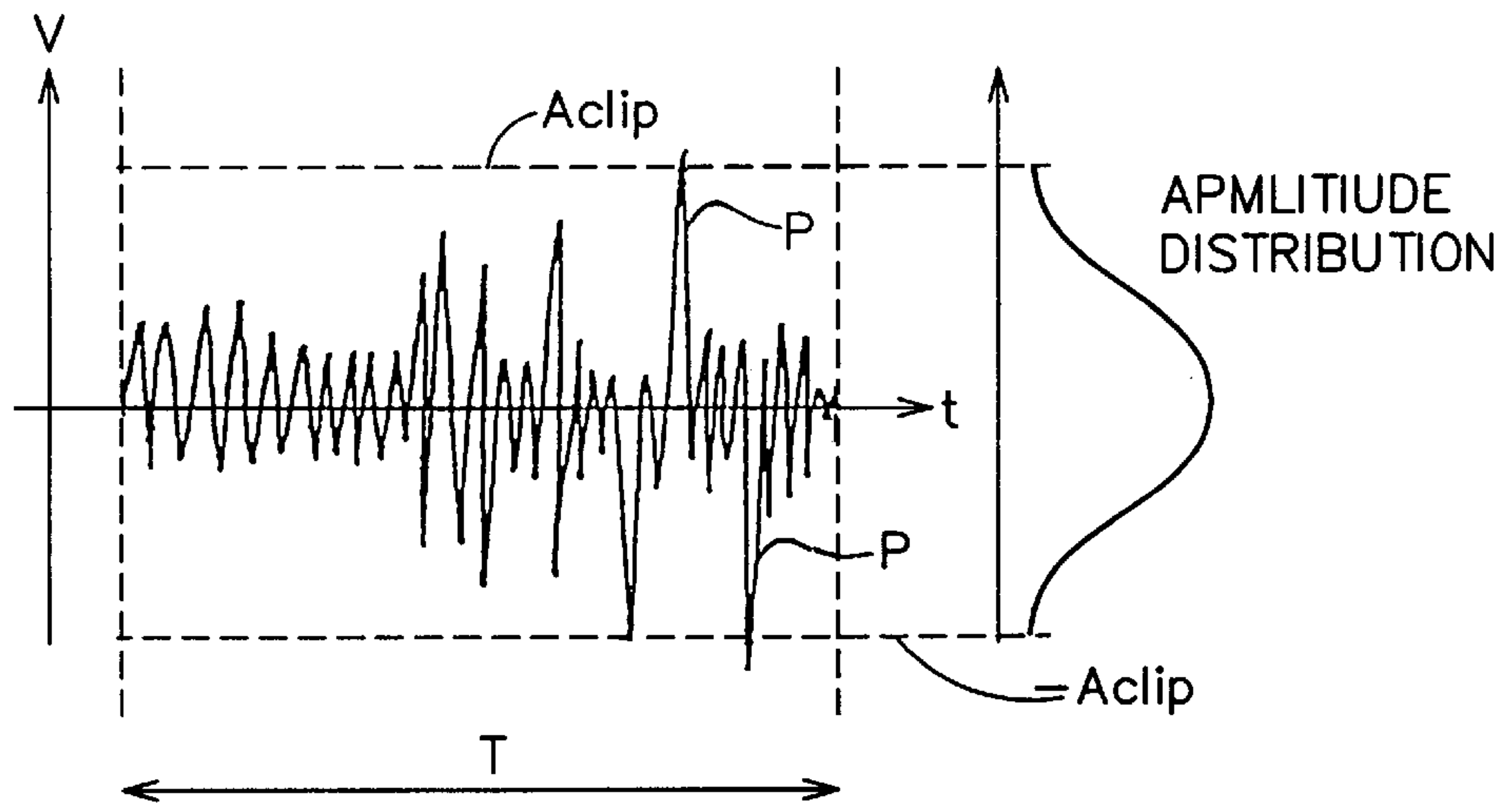
FIG. 1 (PRIOR ART)
