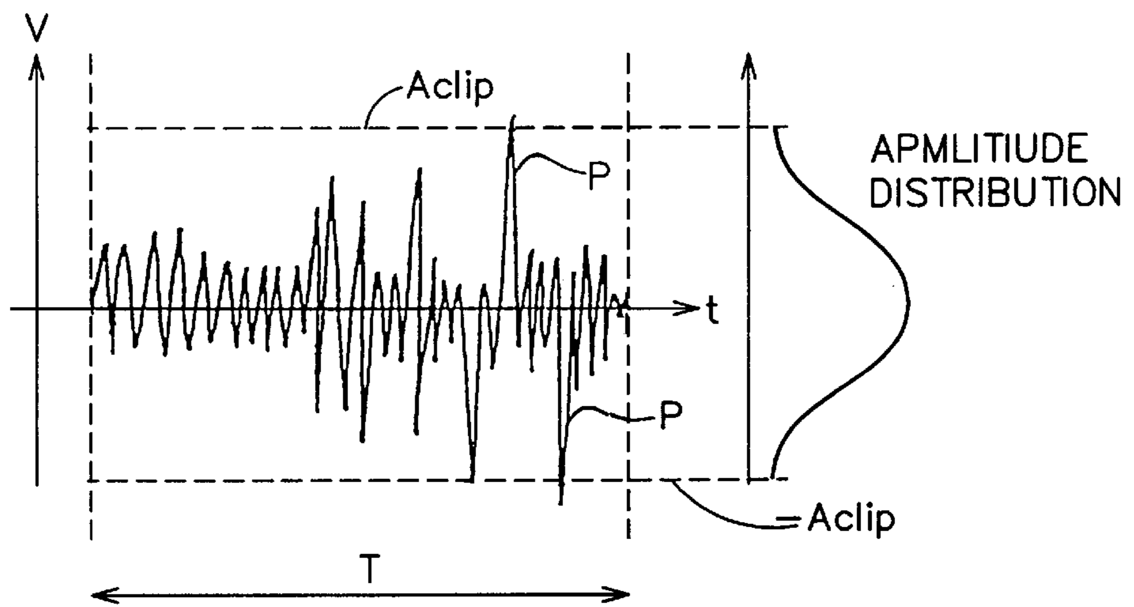
FIG. 1 (PRIOR ART)
