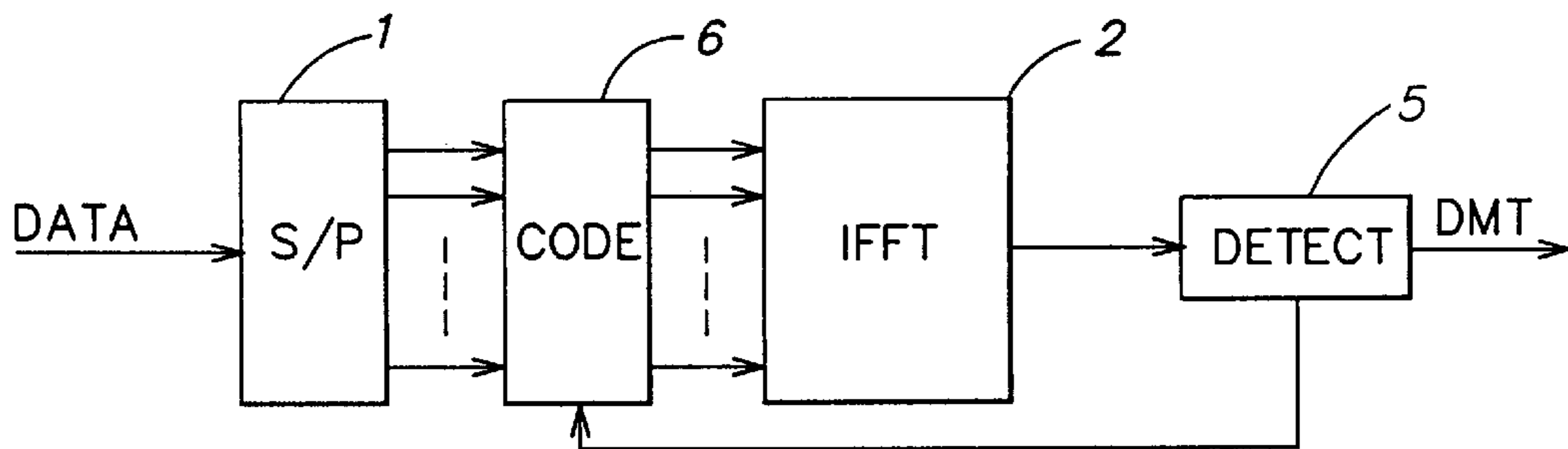
FIG. 3 (PRIOR ART)
