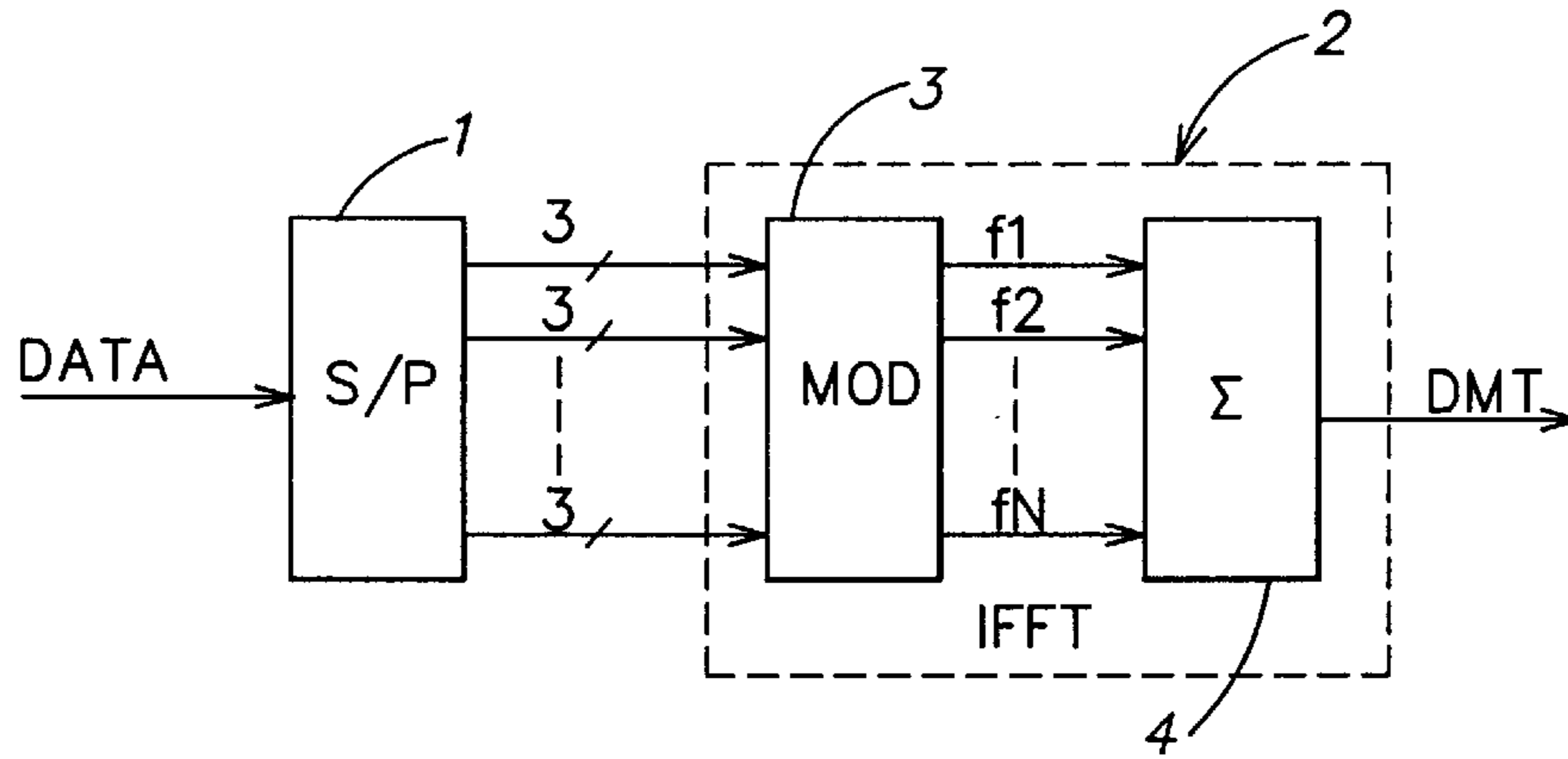
FIG. 1 (PRIOR ART)
