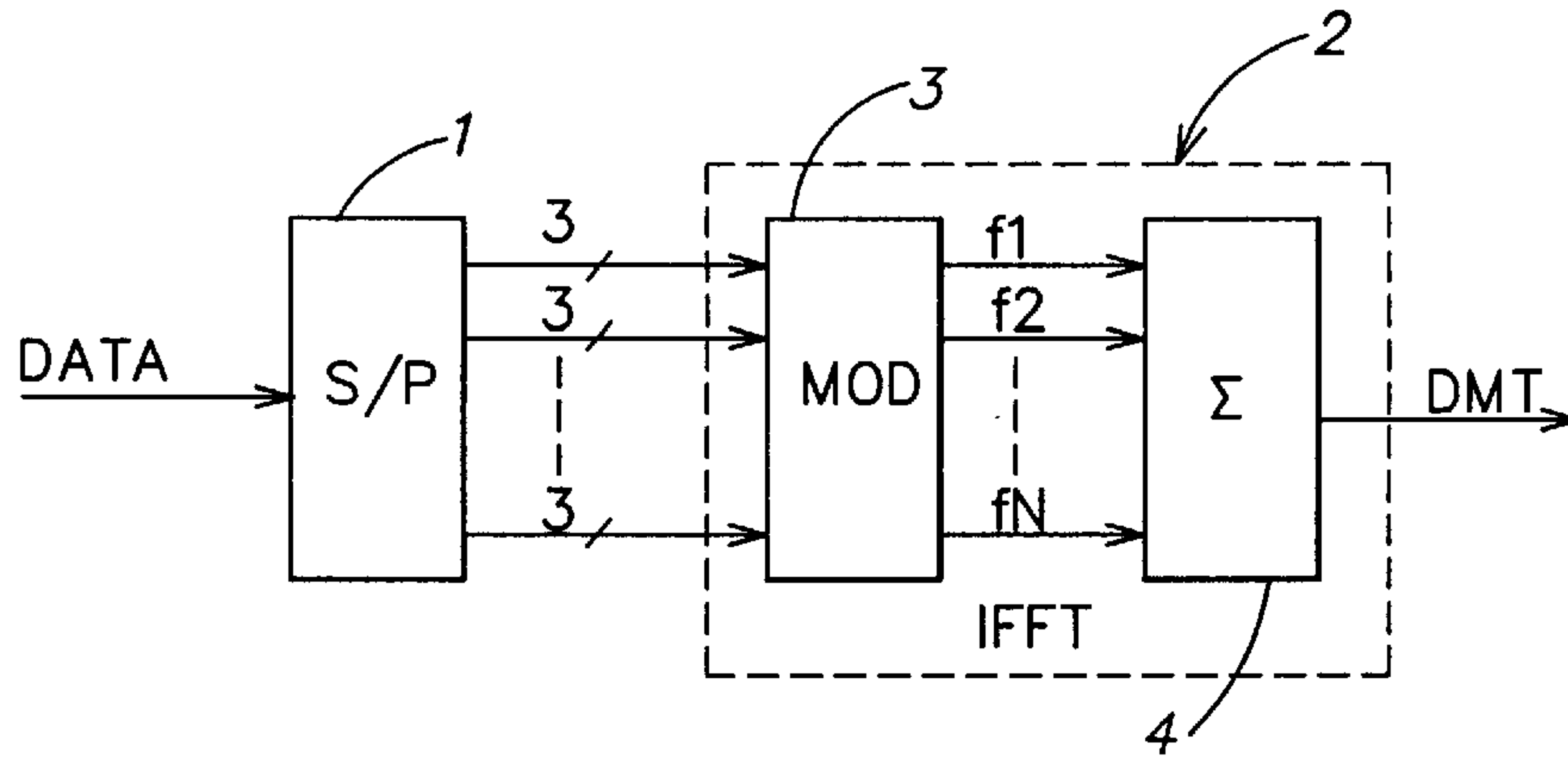
FIG. 1 (PRIOR ART)
