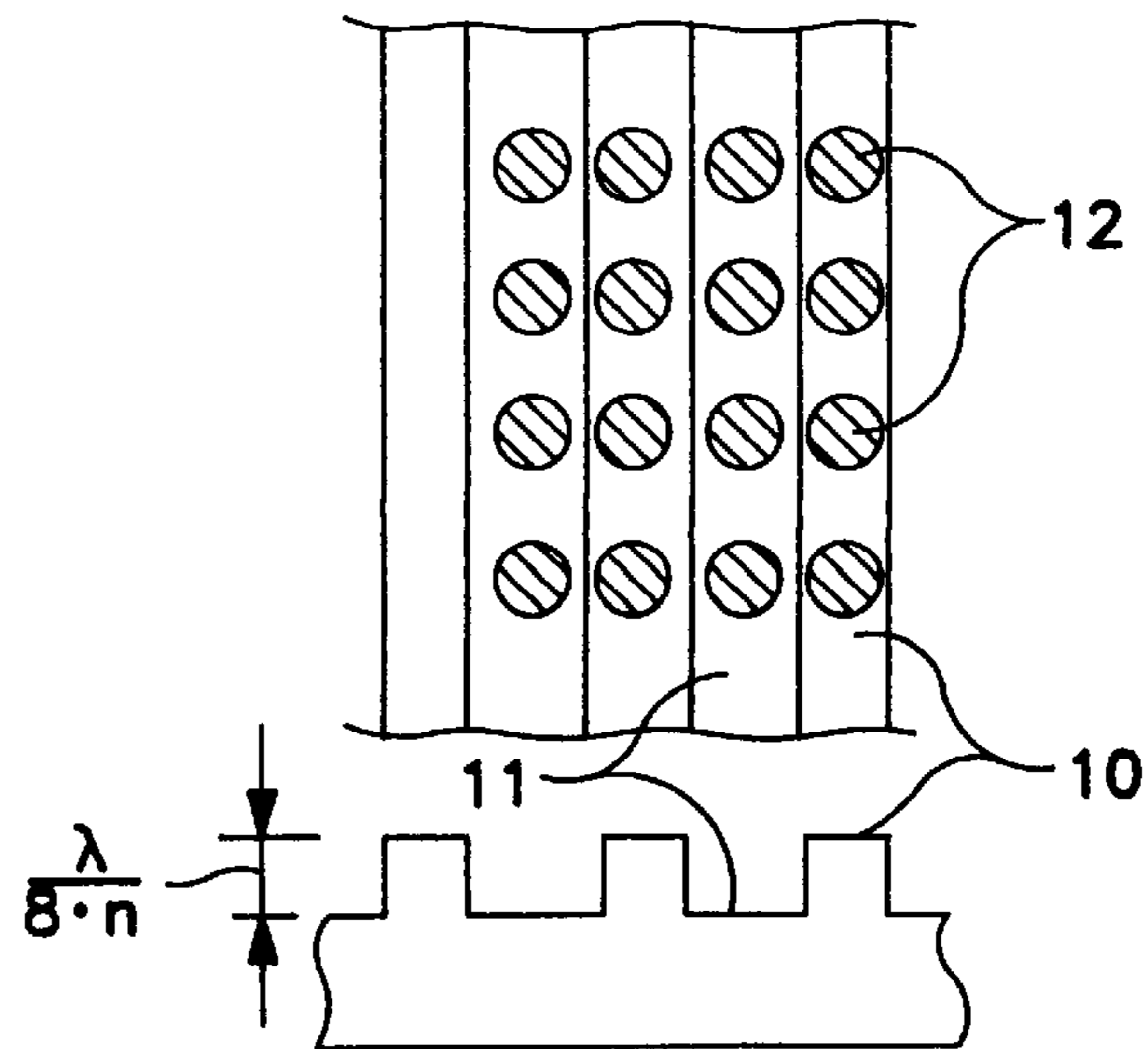
FIG. 10C PRIOR ART
