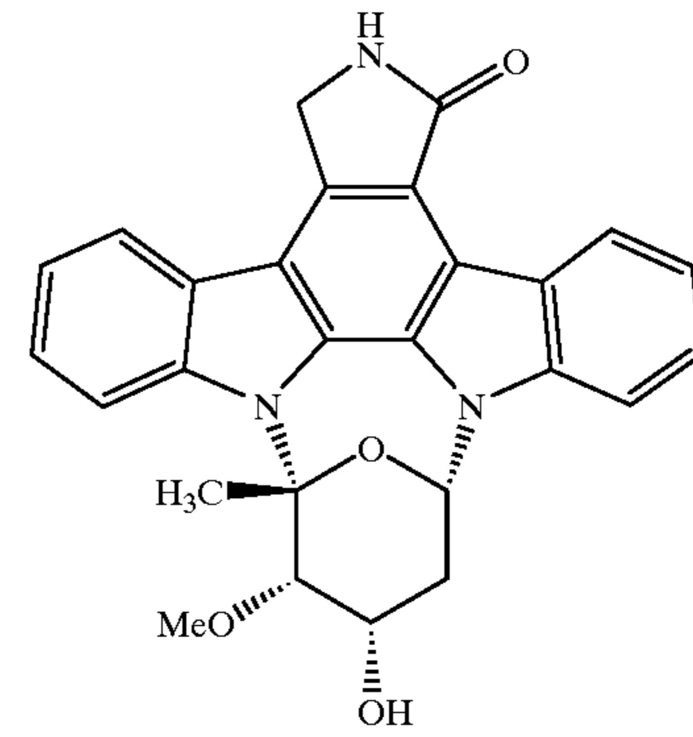
(-)-RK286c
