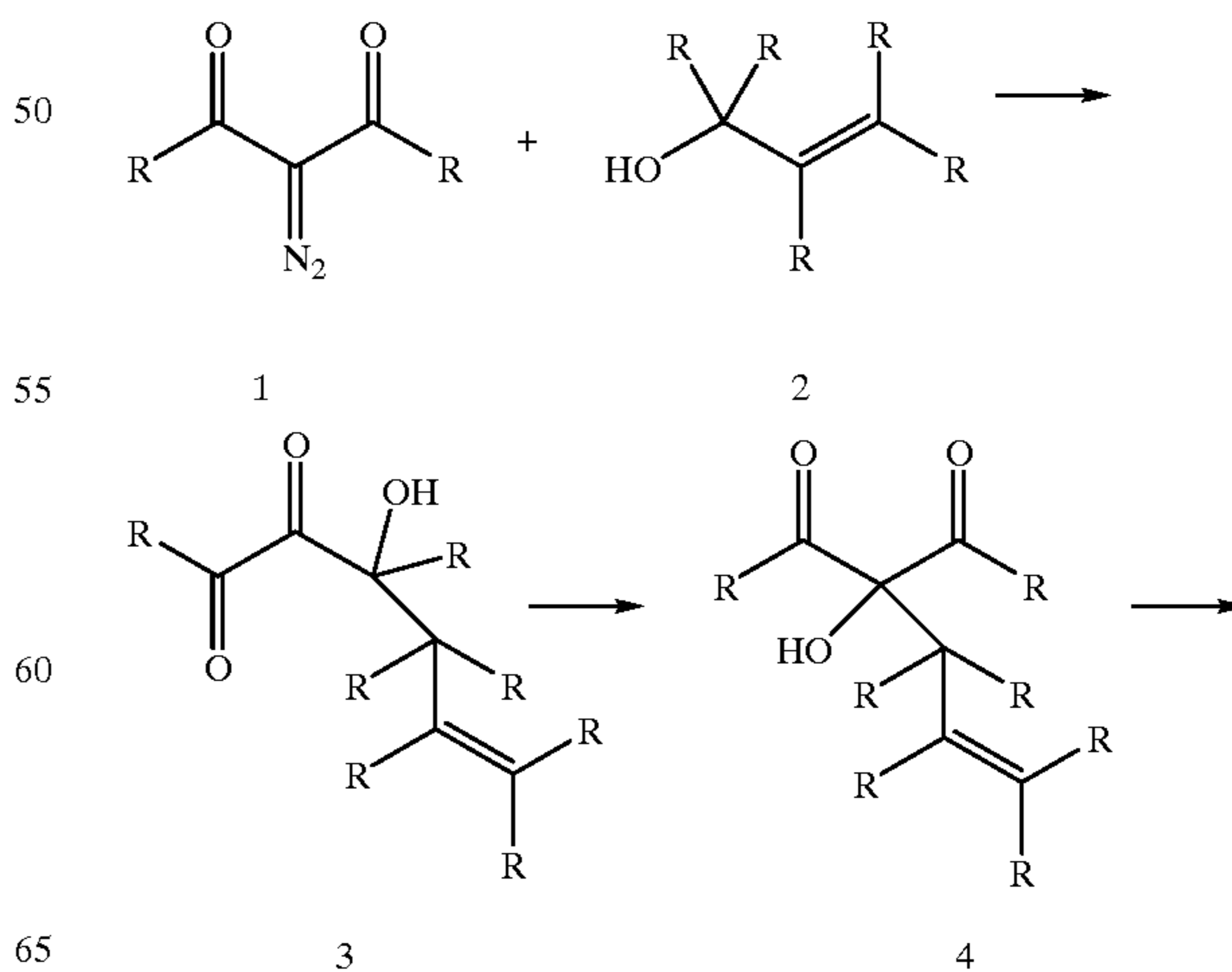
Scheme III
