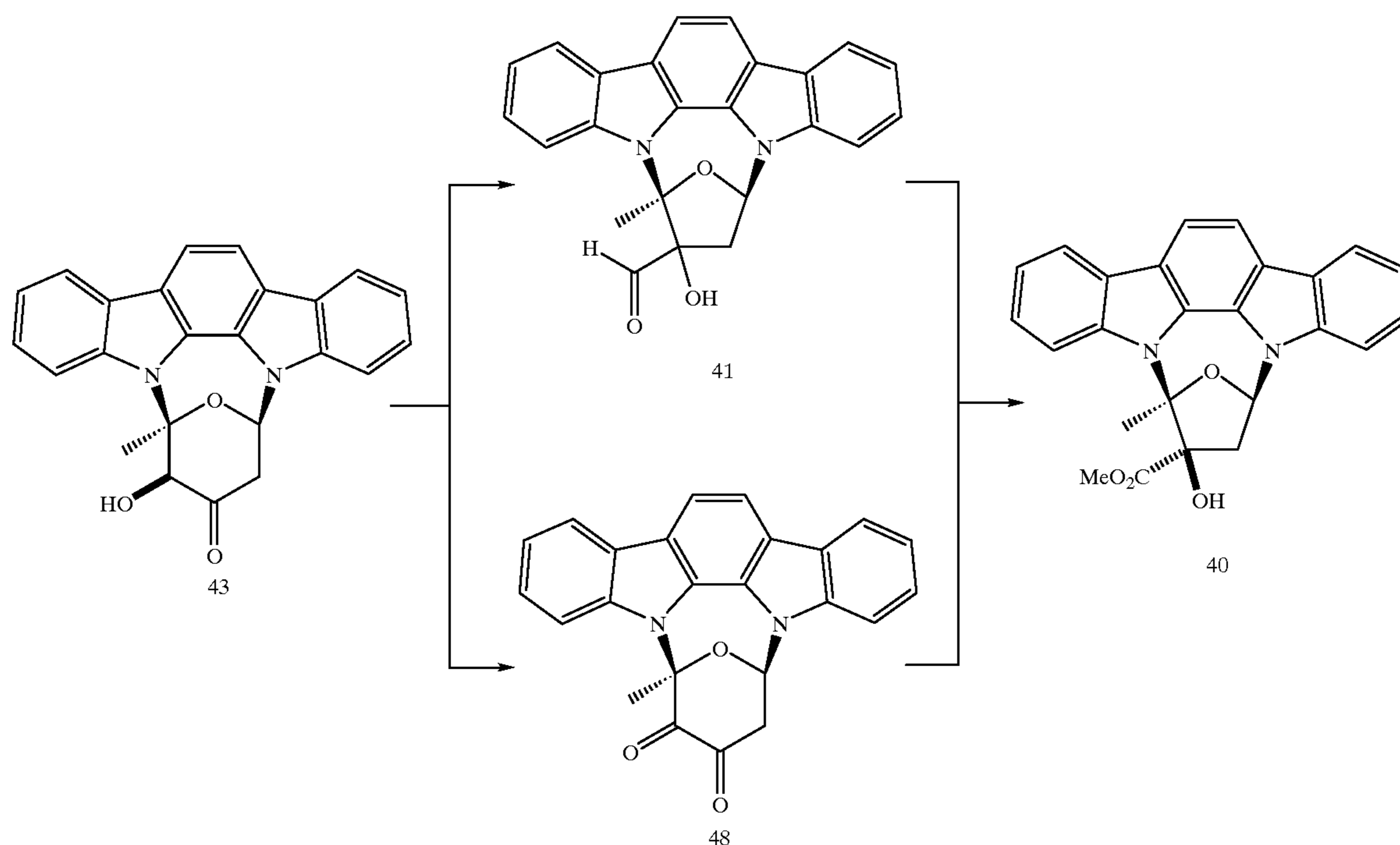
Scheme XIX
