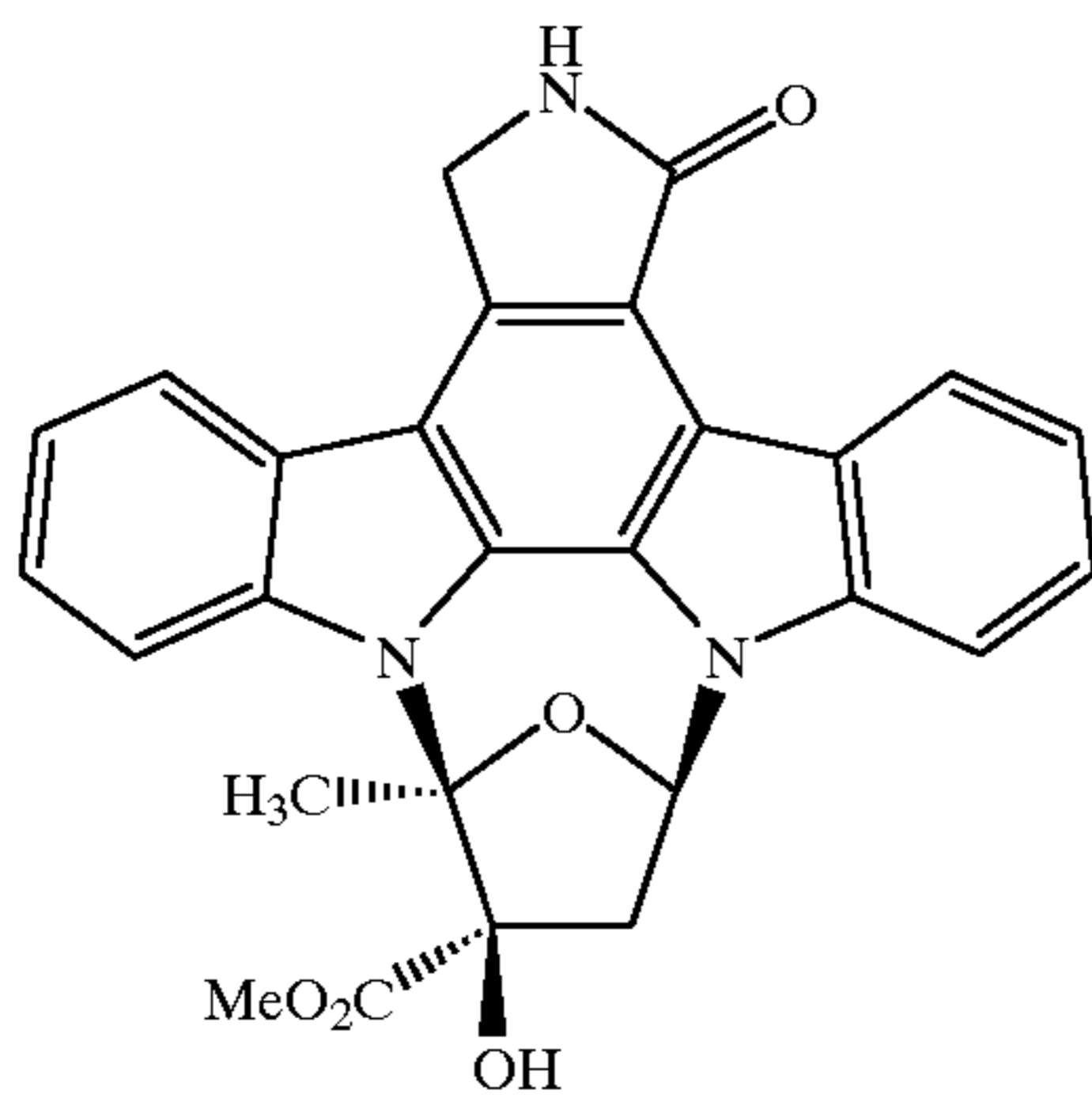
(+)-K252a
