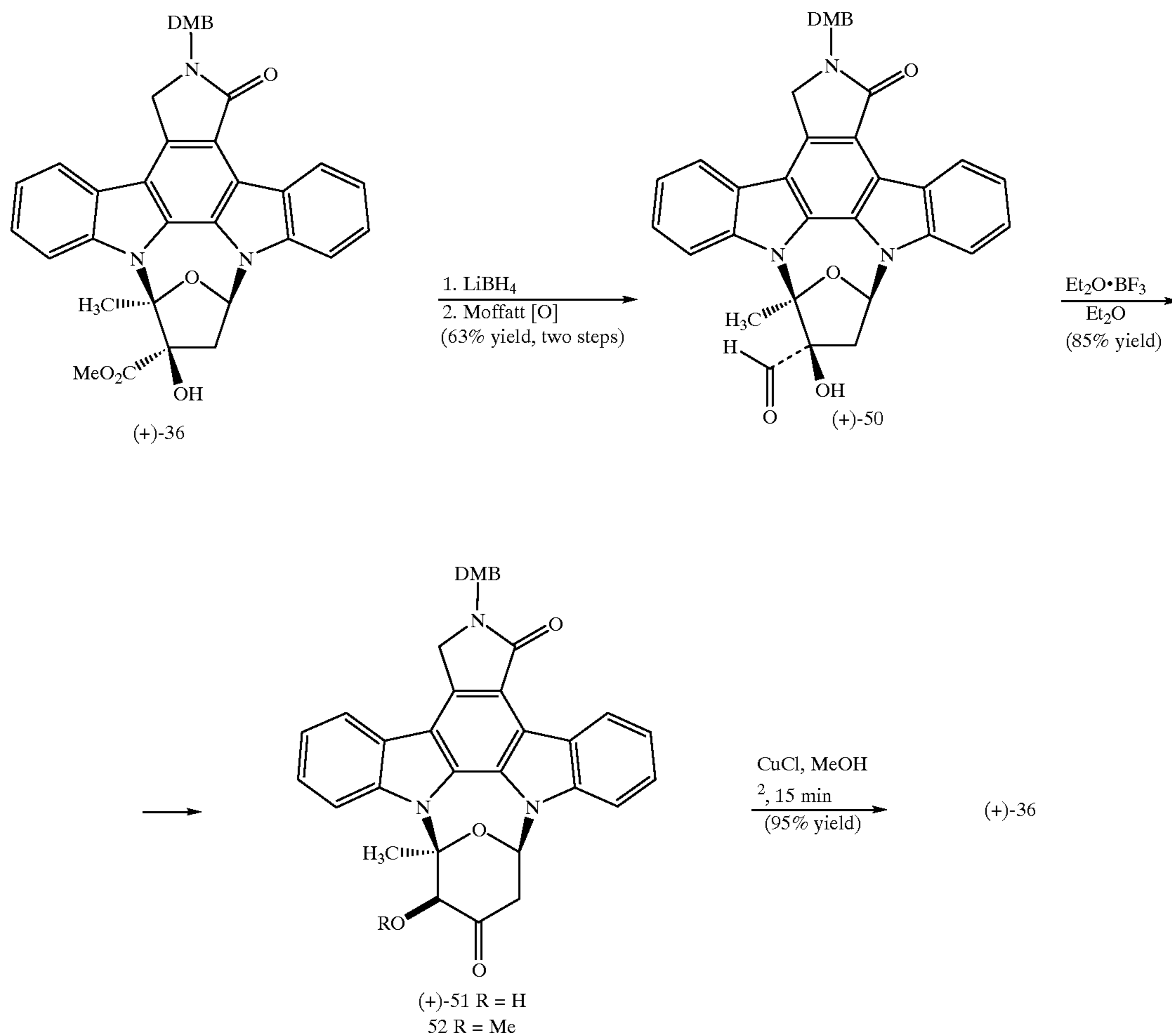
Scheme XX
