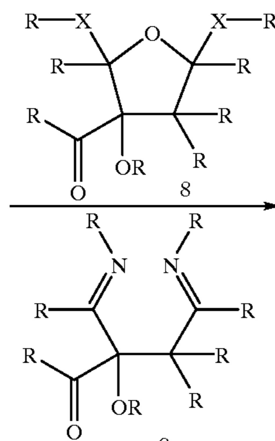
Scheme V
