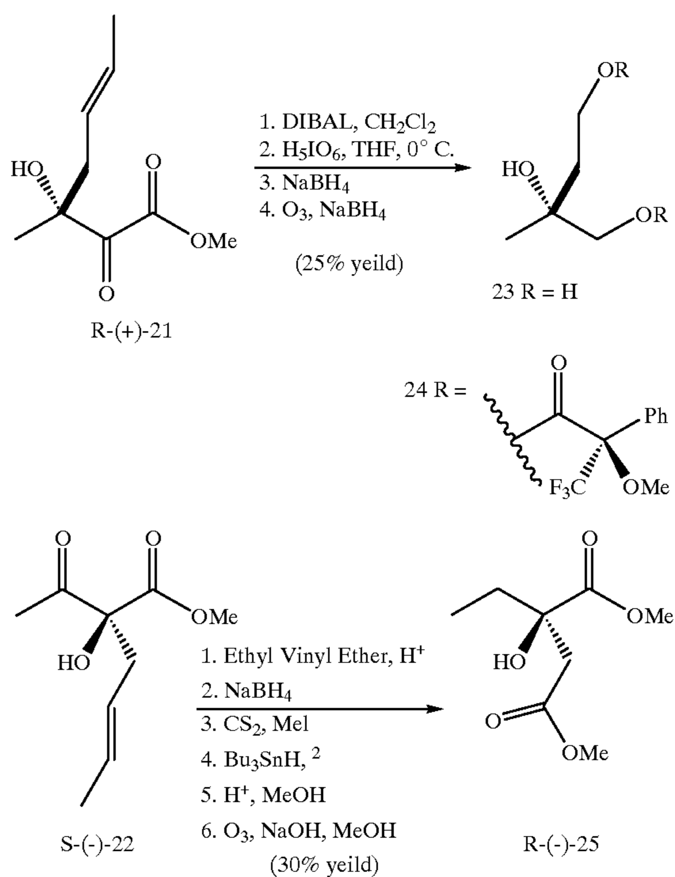
Scheme IX
