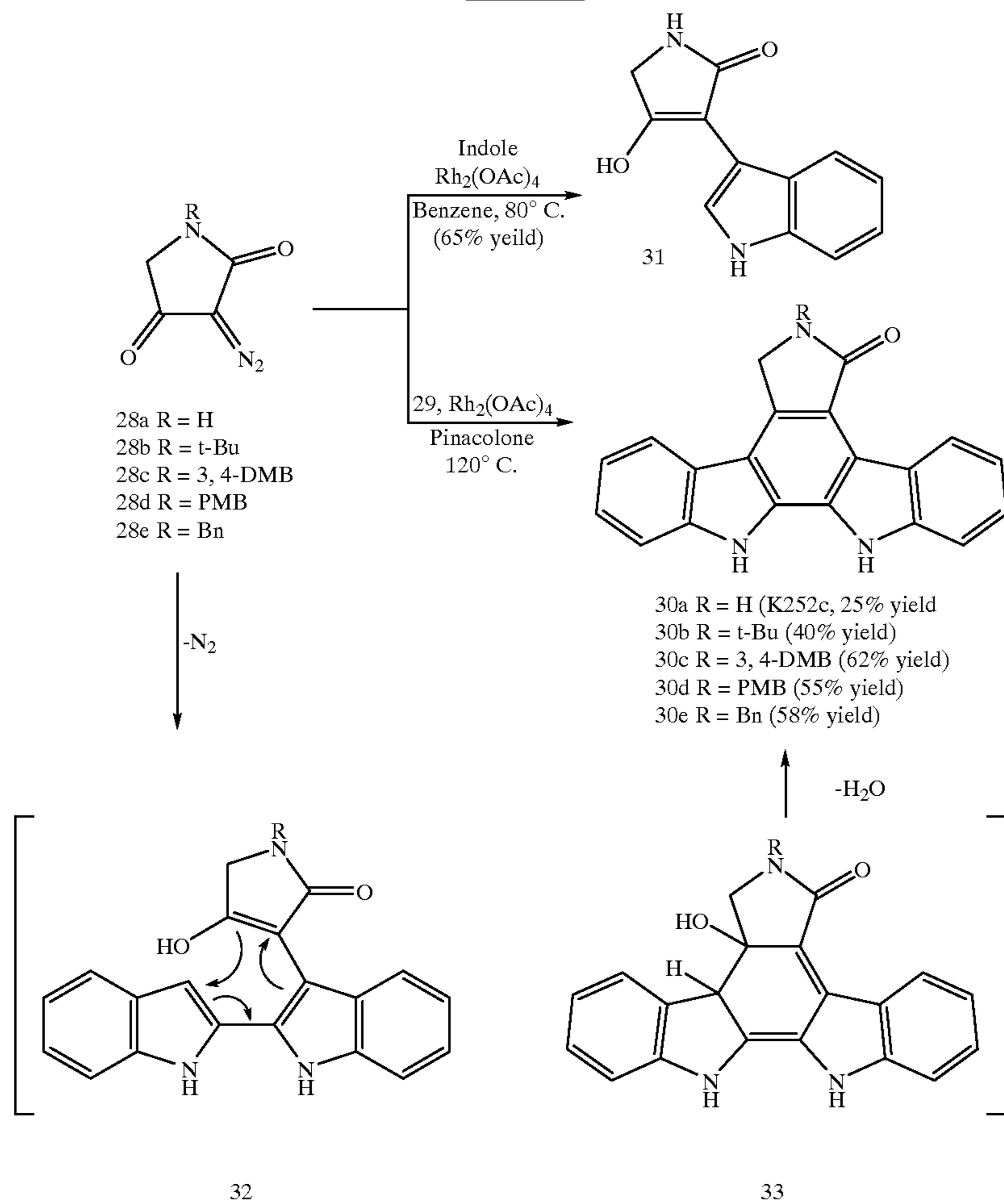
Scheme XII
