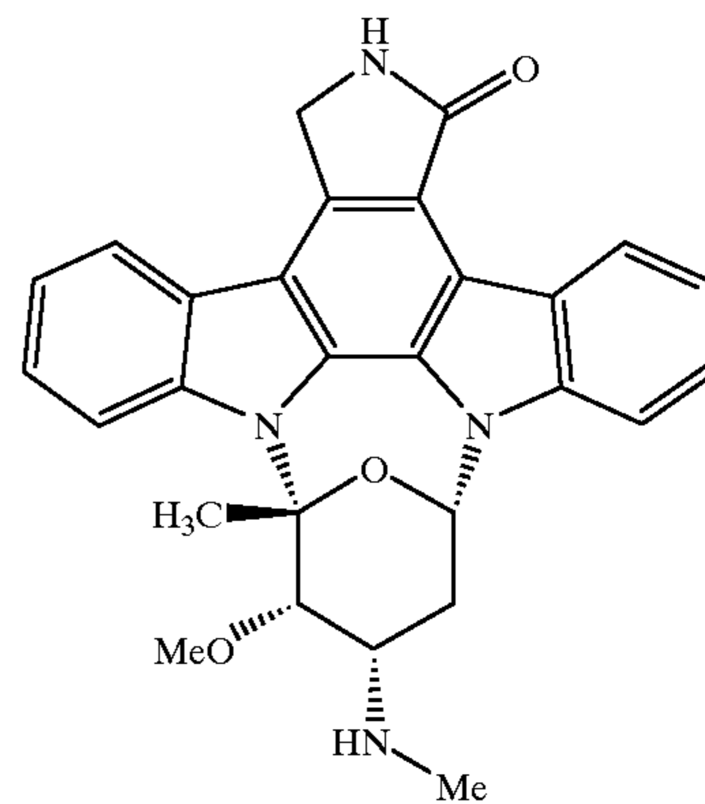
(-)-Straurosporine
