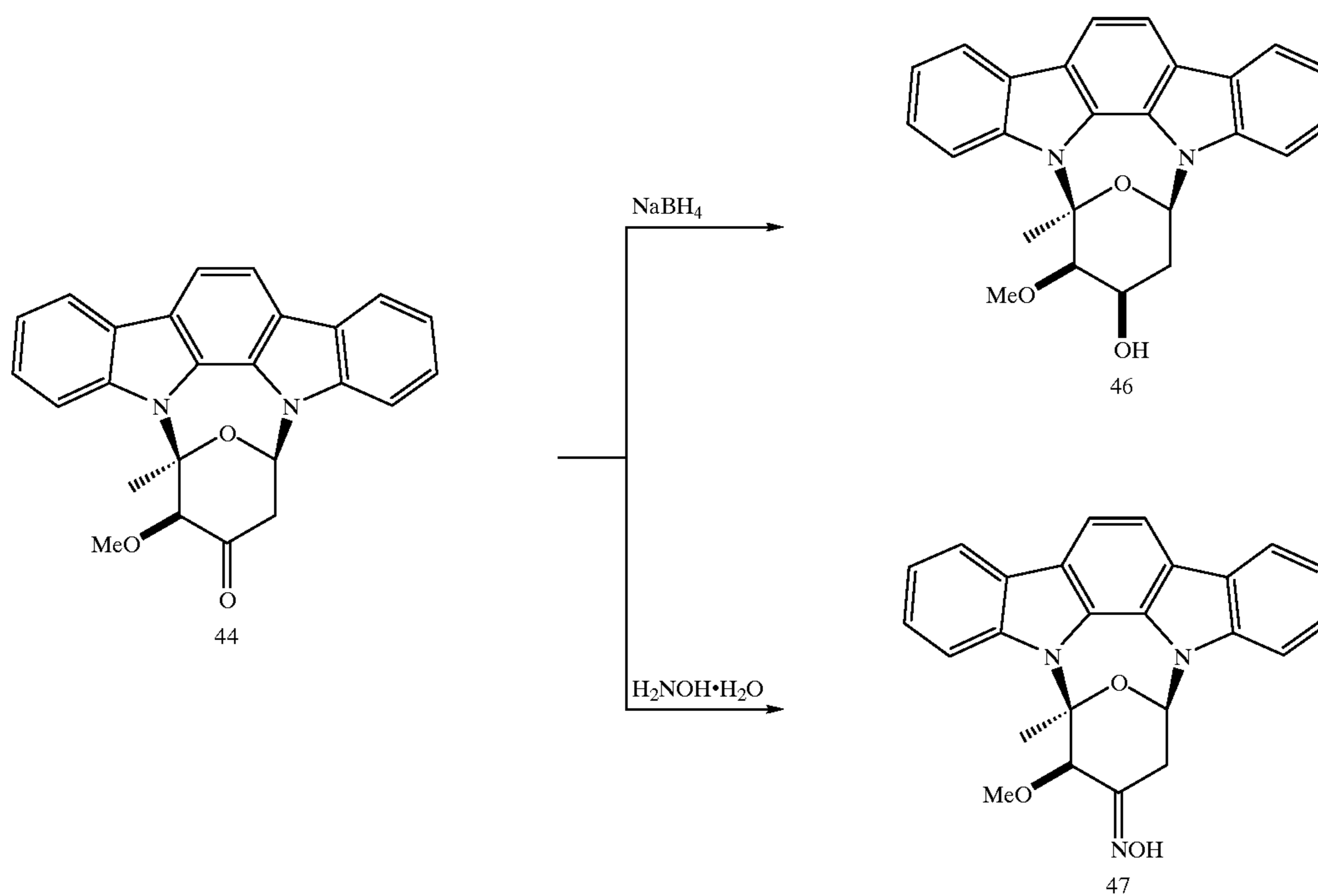
Scheme XVIII
