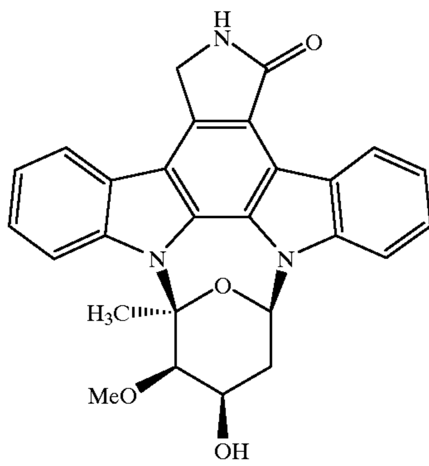
(+)-RK286c
