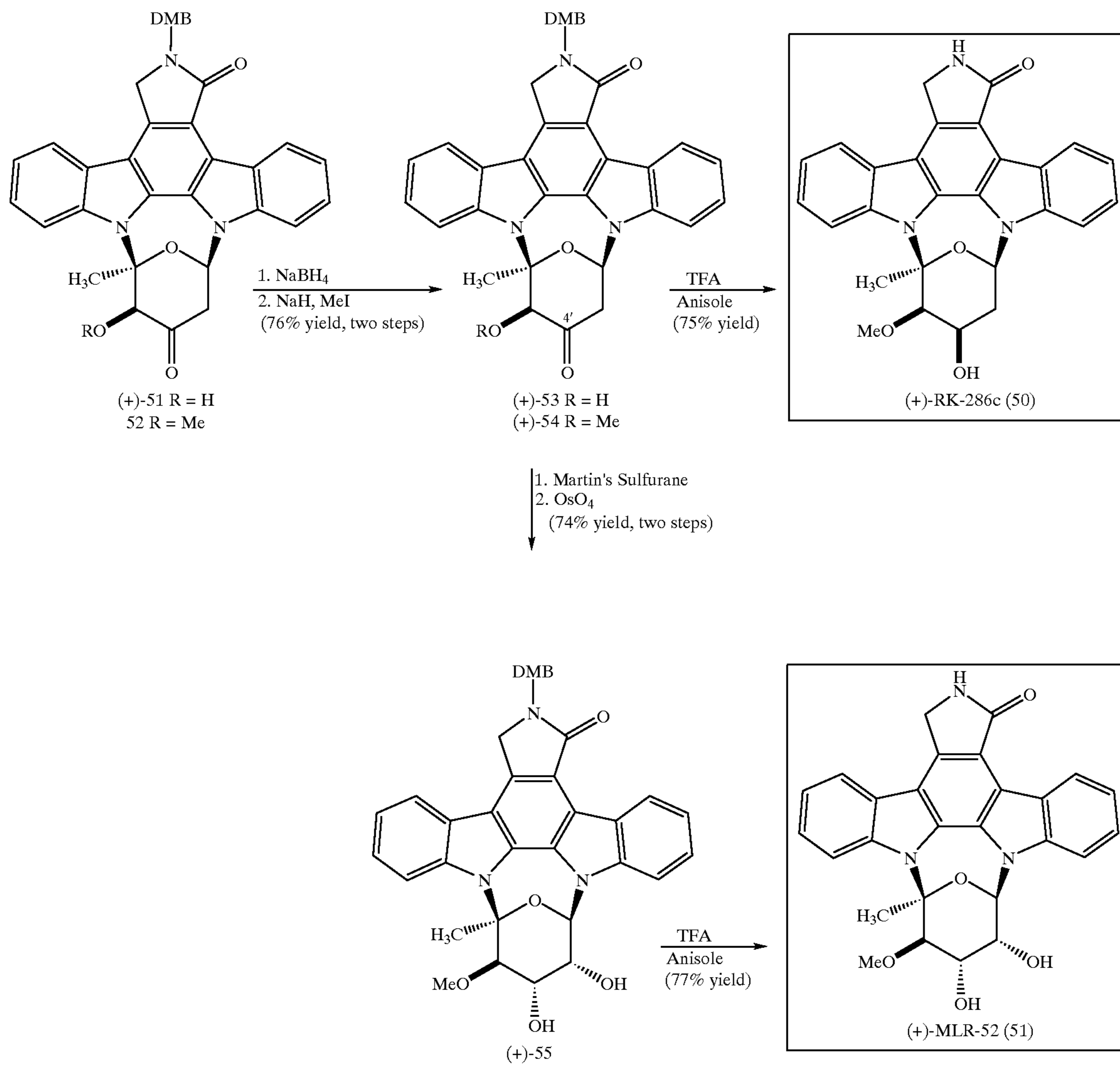
Scheme XXI
