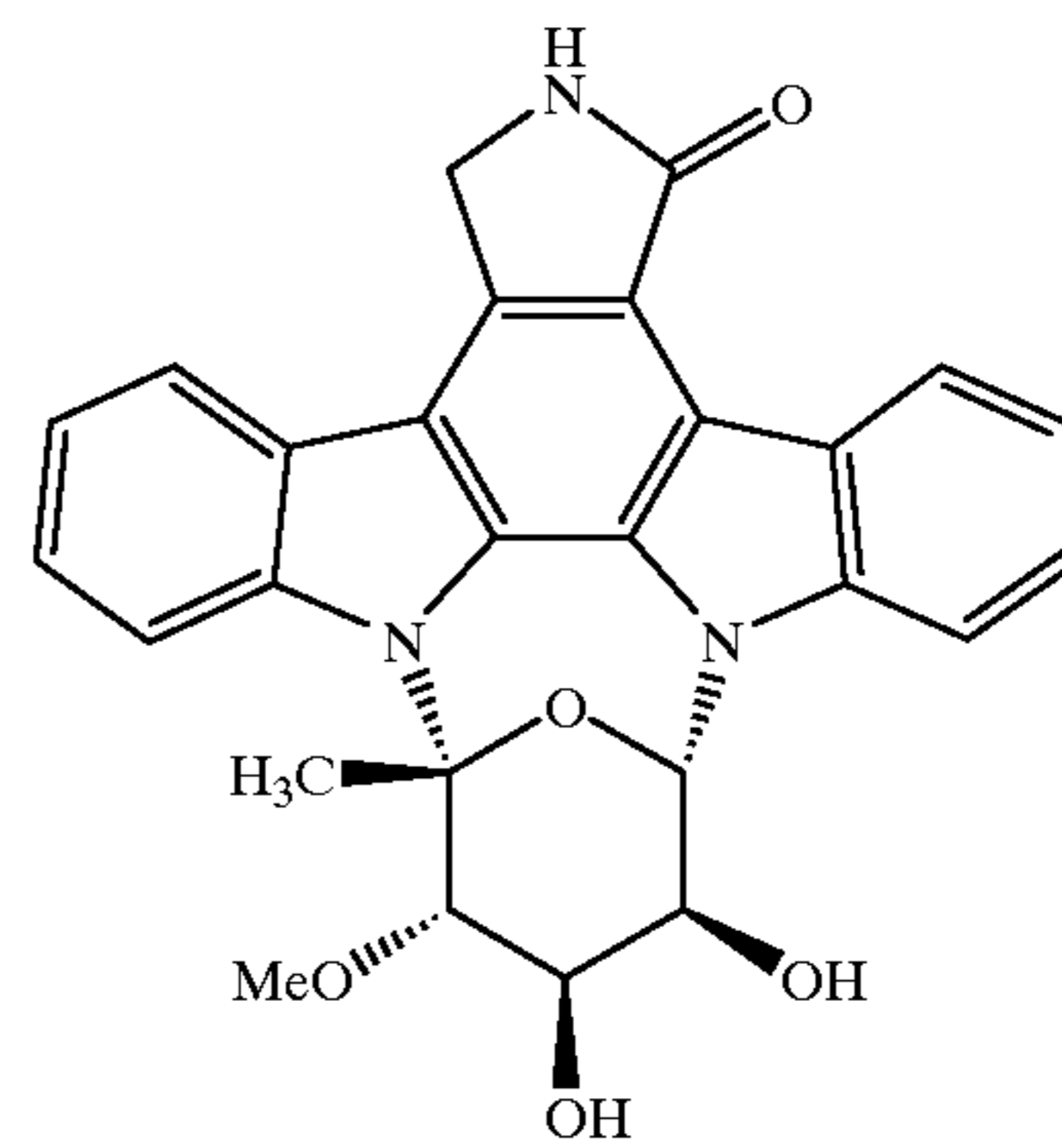
(-)-MLR-52
