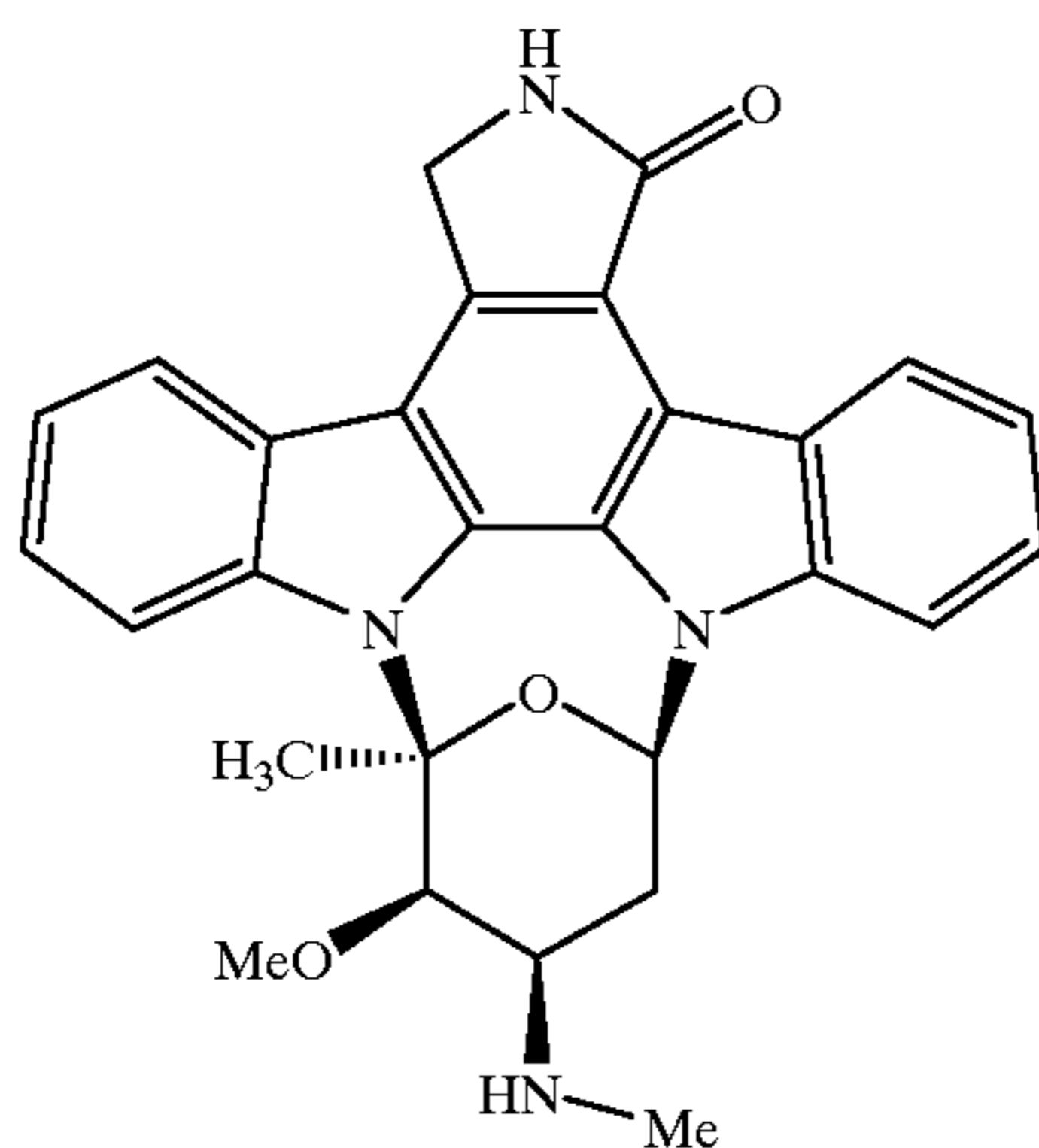
(+)-Straurosporine
