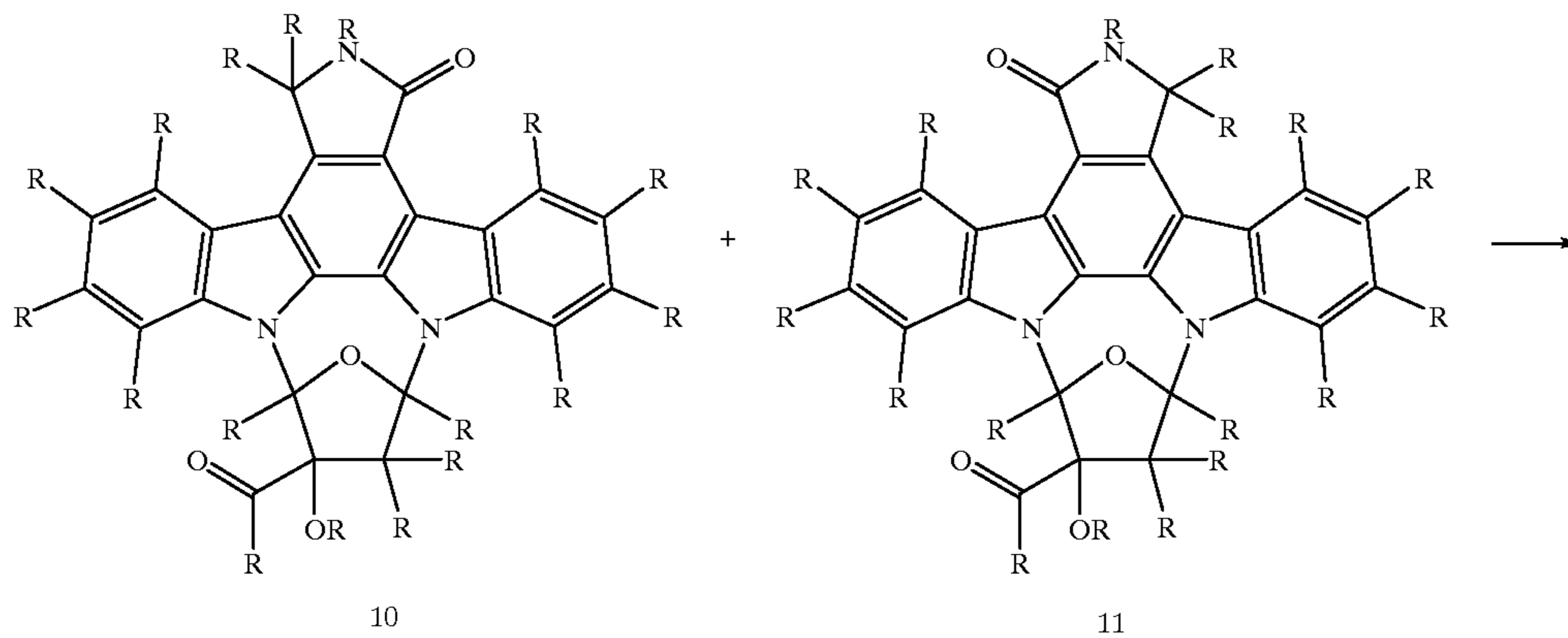
Scheme VII
