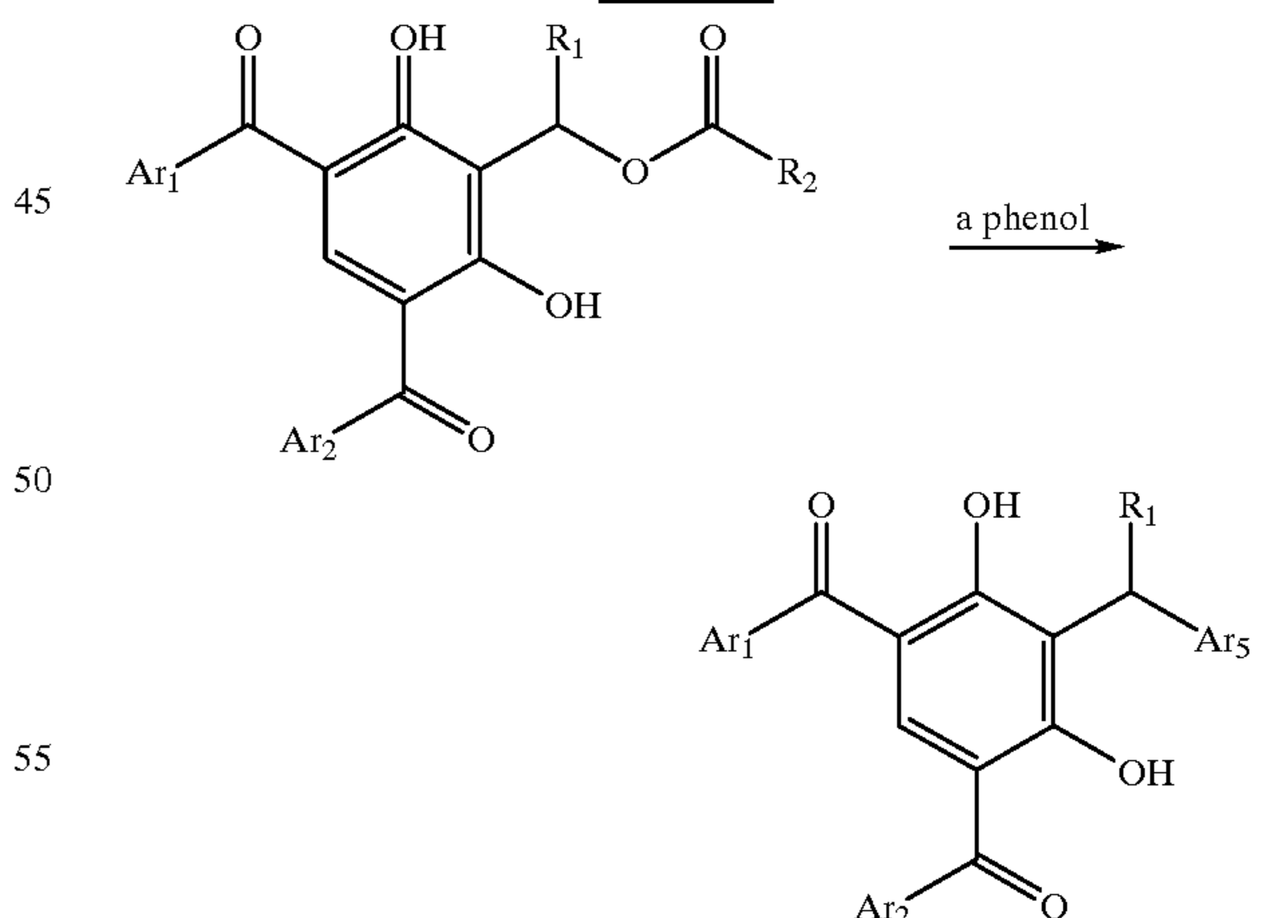
Scheme II.
