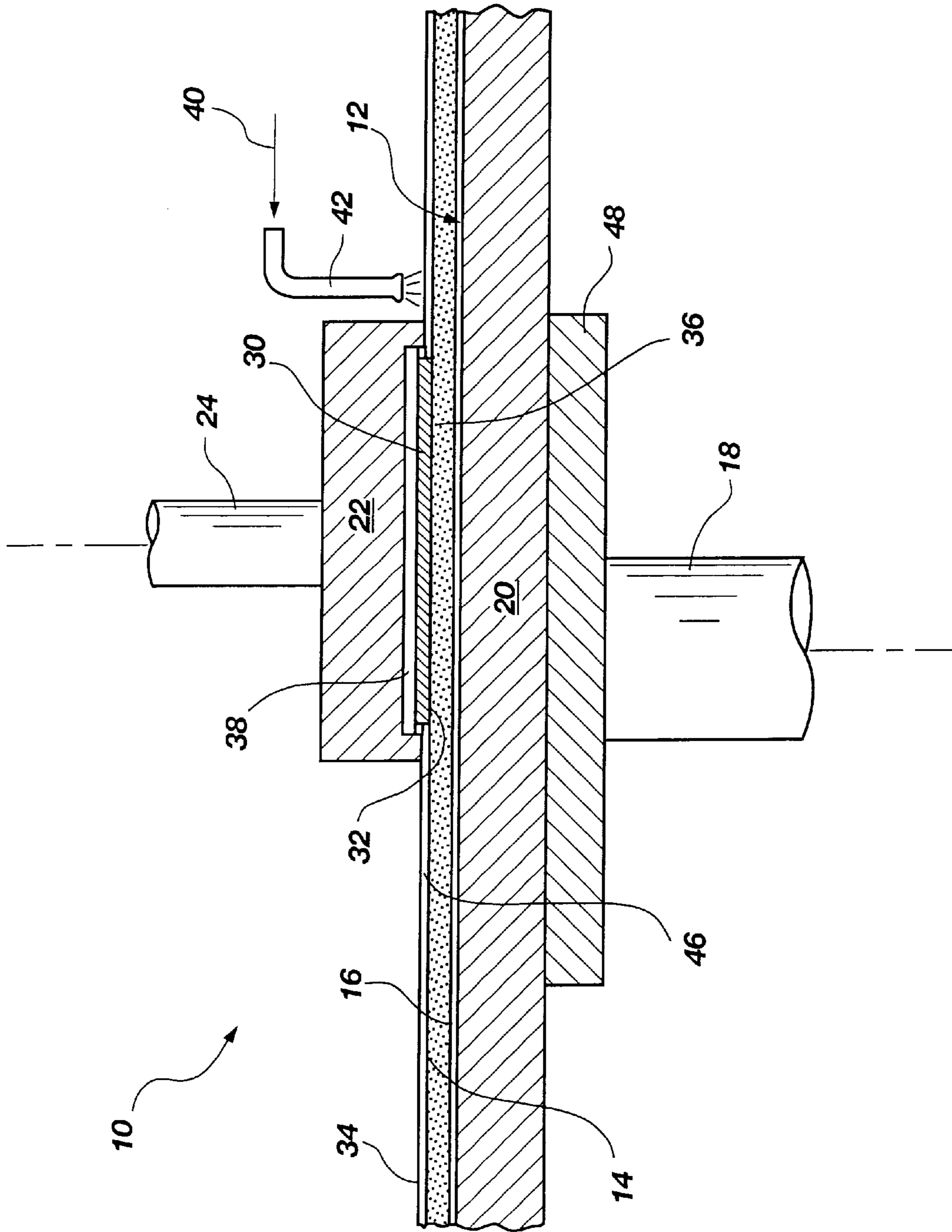
Fig. 2 (PRIOR ART)
