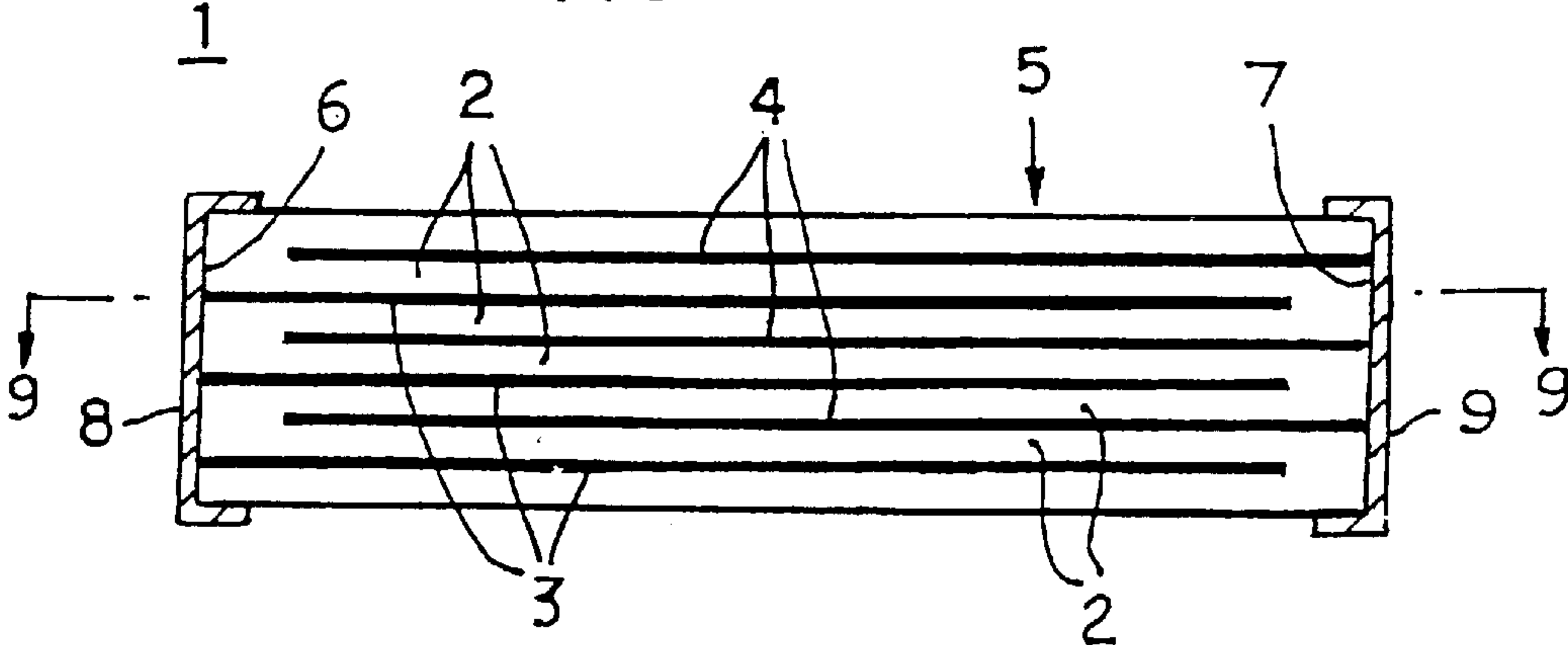
FIG. 7 PRIOR ART
