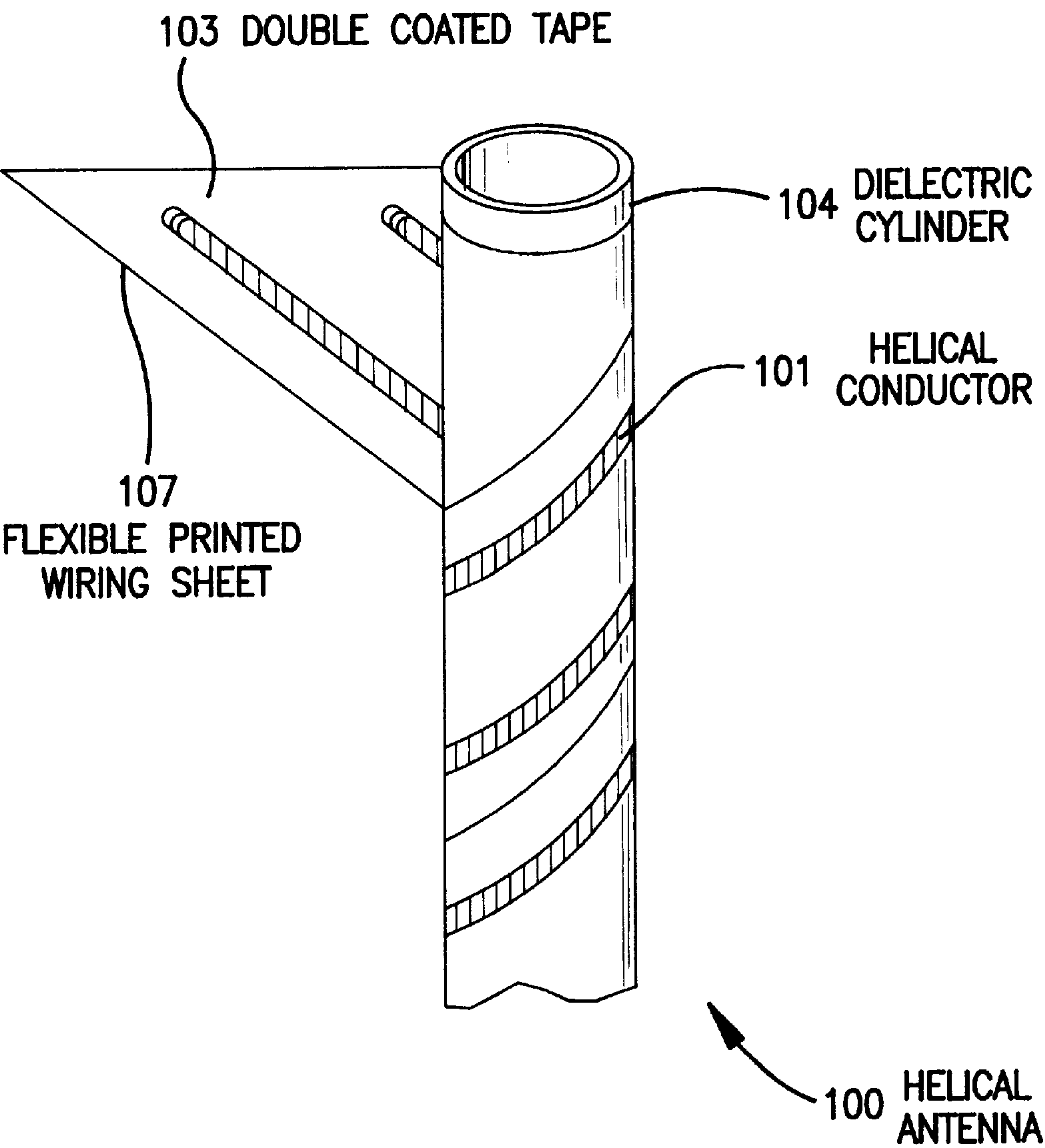
FIG. 8 PRIOR ART
