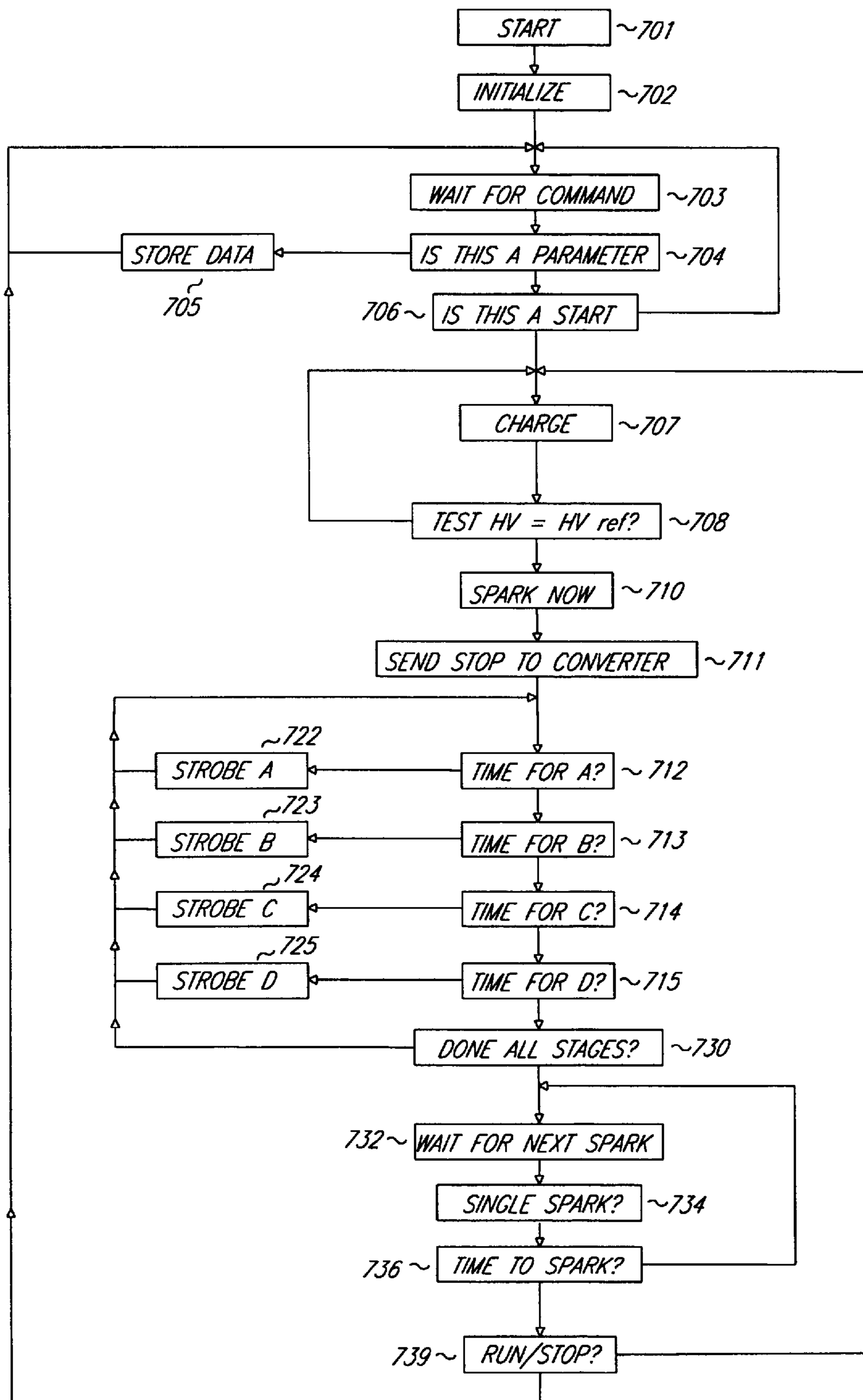
FIGURE 7 FLOWCHART
