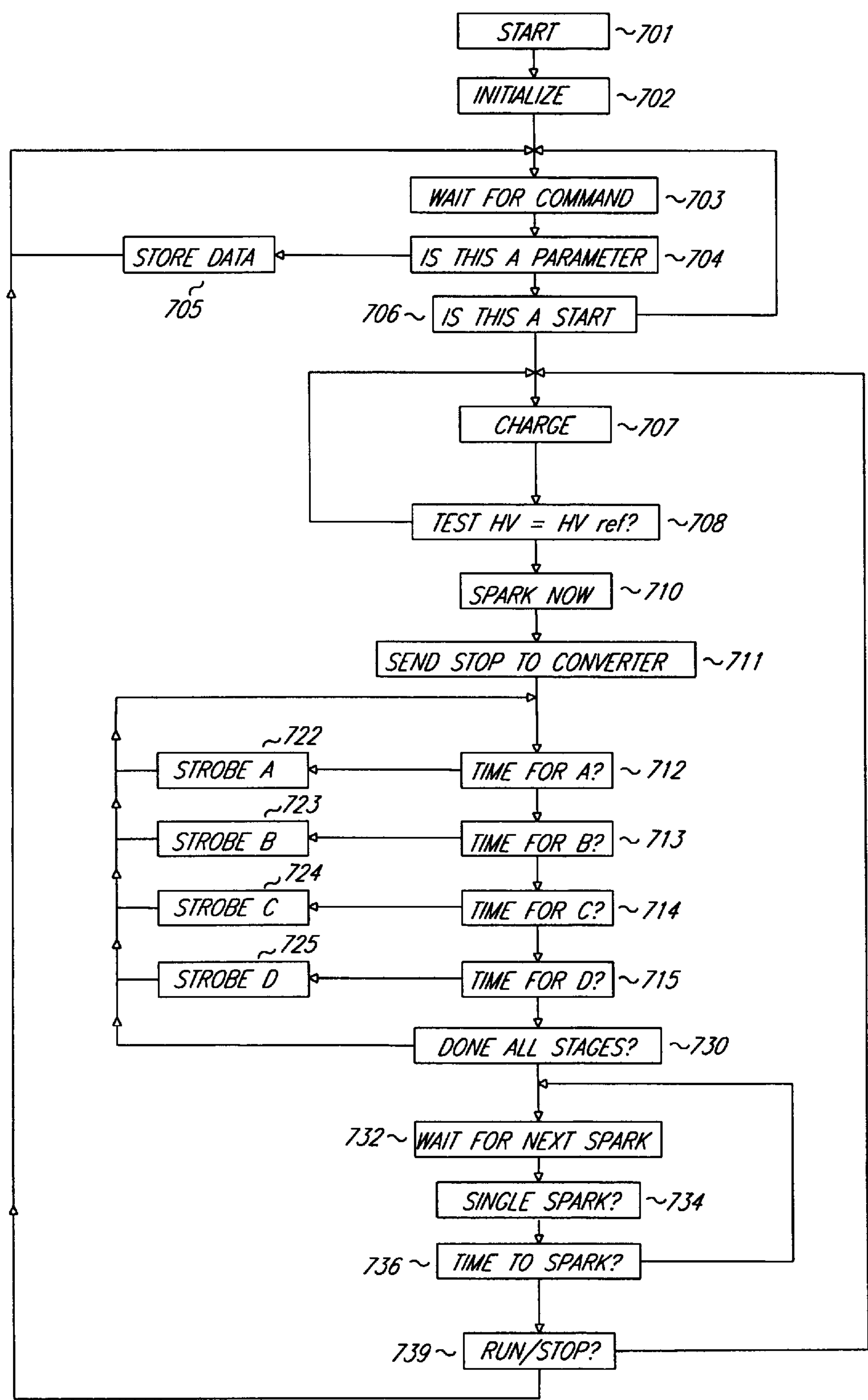
FIGURE 7 FLOWCHART
