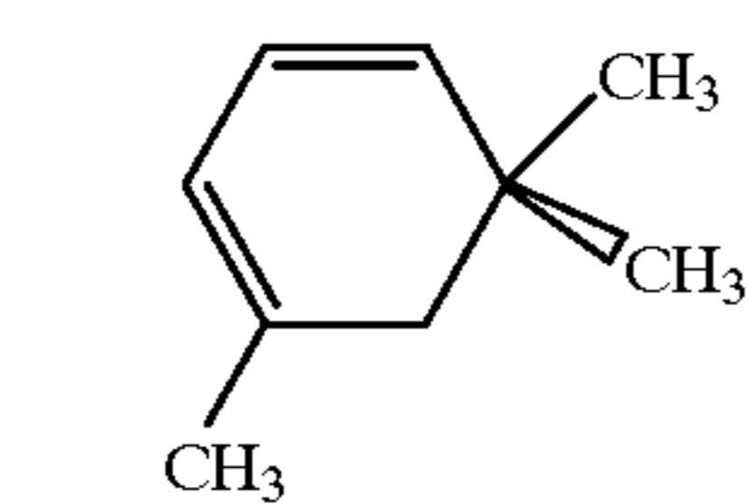
Cyclohexadiene compound
