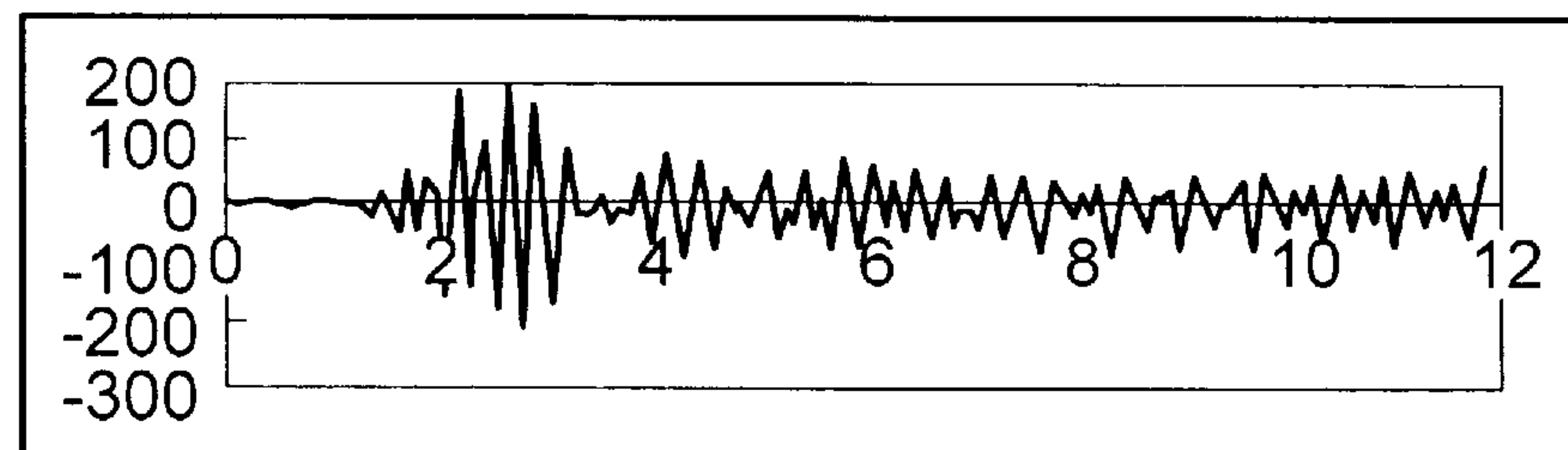
90 rpm VIBRATION WAVEFORM
