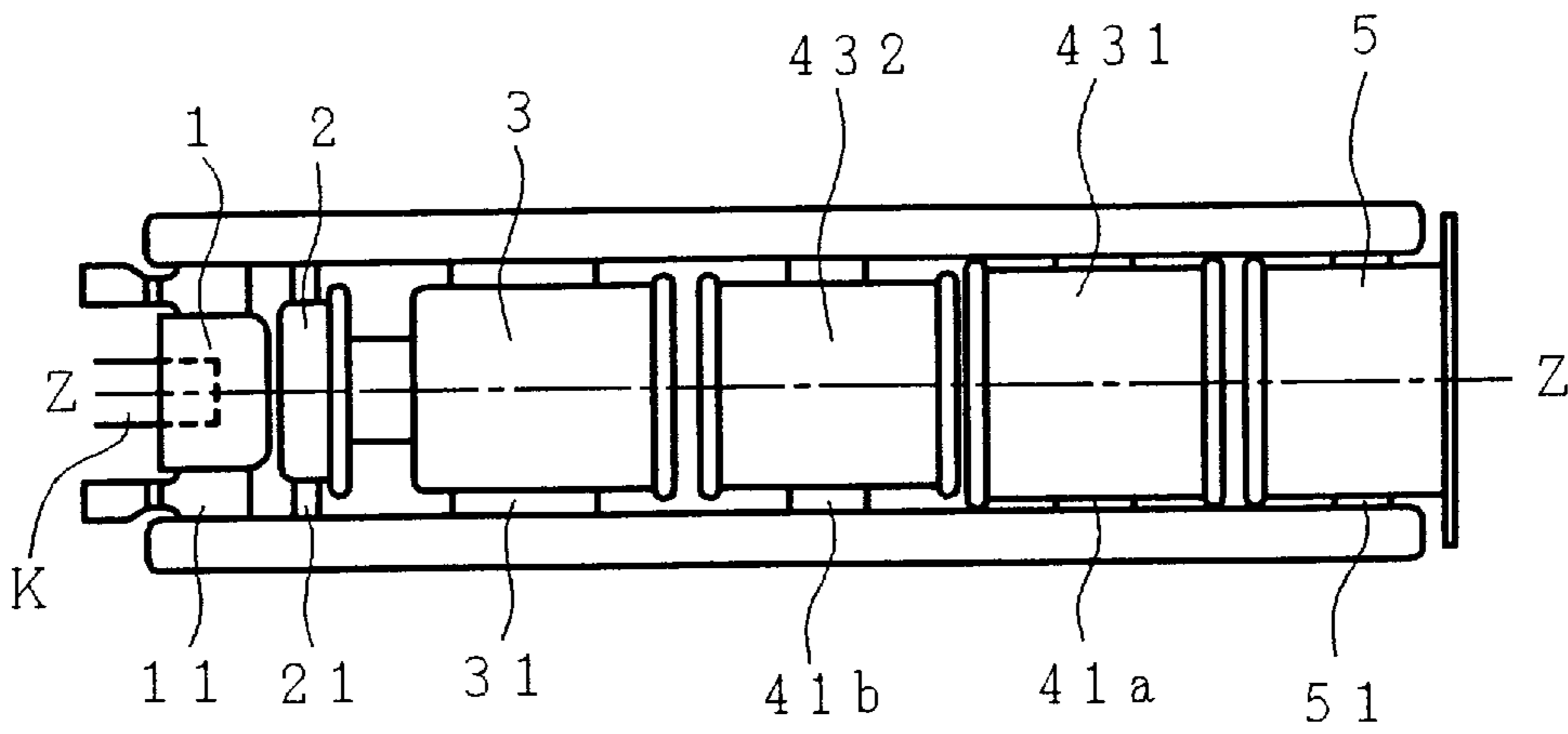
FIG. 17 (Prior art)
