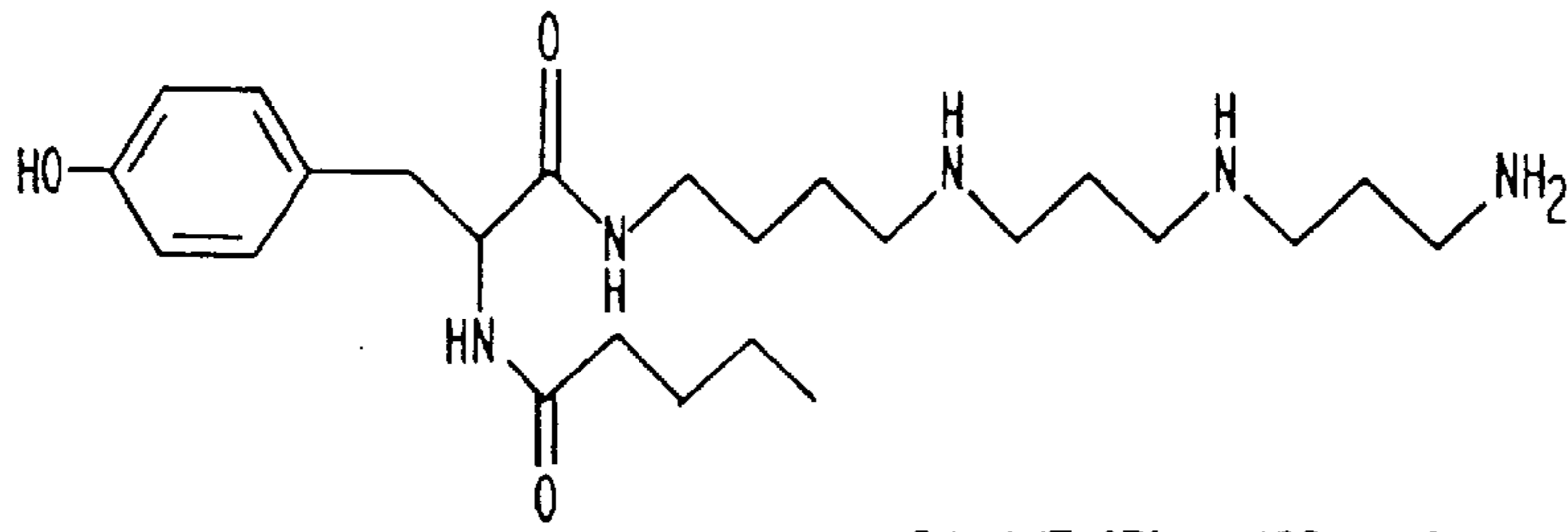
PHILANTHOTOXIN 433 +3
