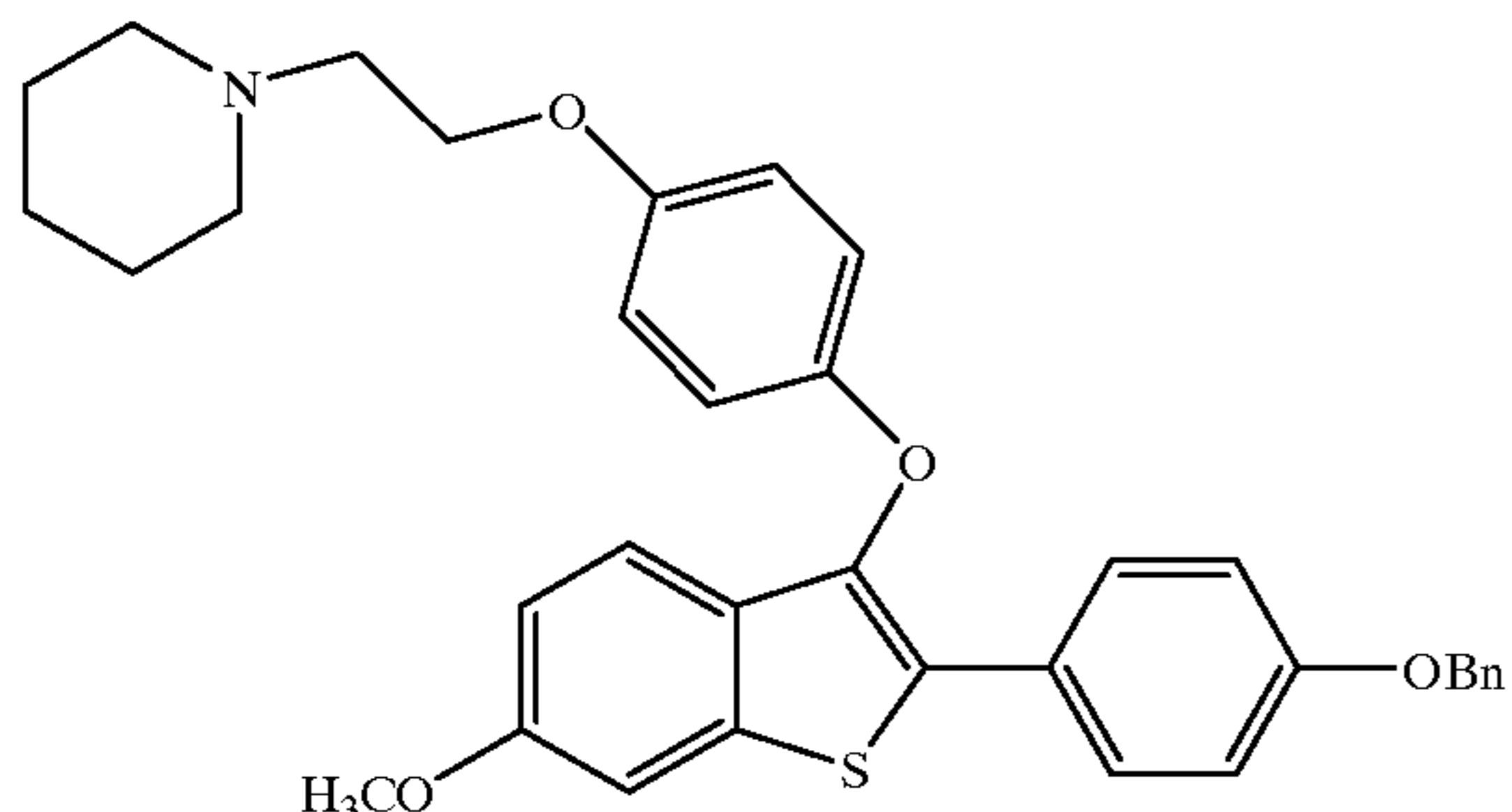
[6-Methoxy-3-[4-[2-(1-piperidinyloxy)]phenoxy]-2-(4-benzyloxyphenyl)]benzo[b]thiophene
