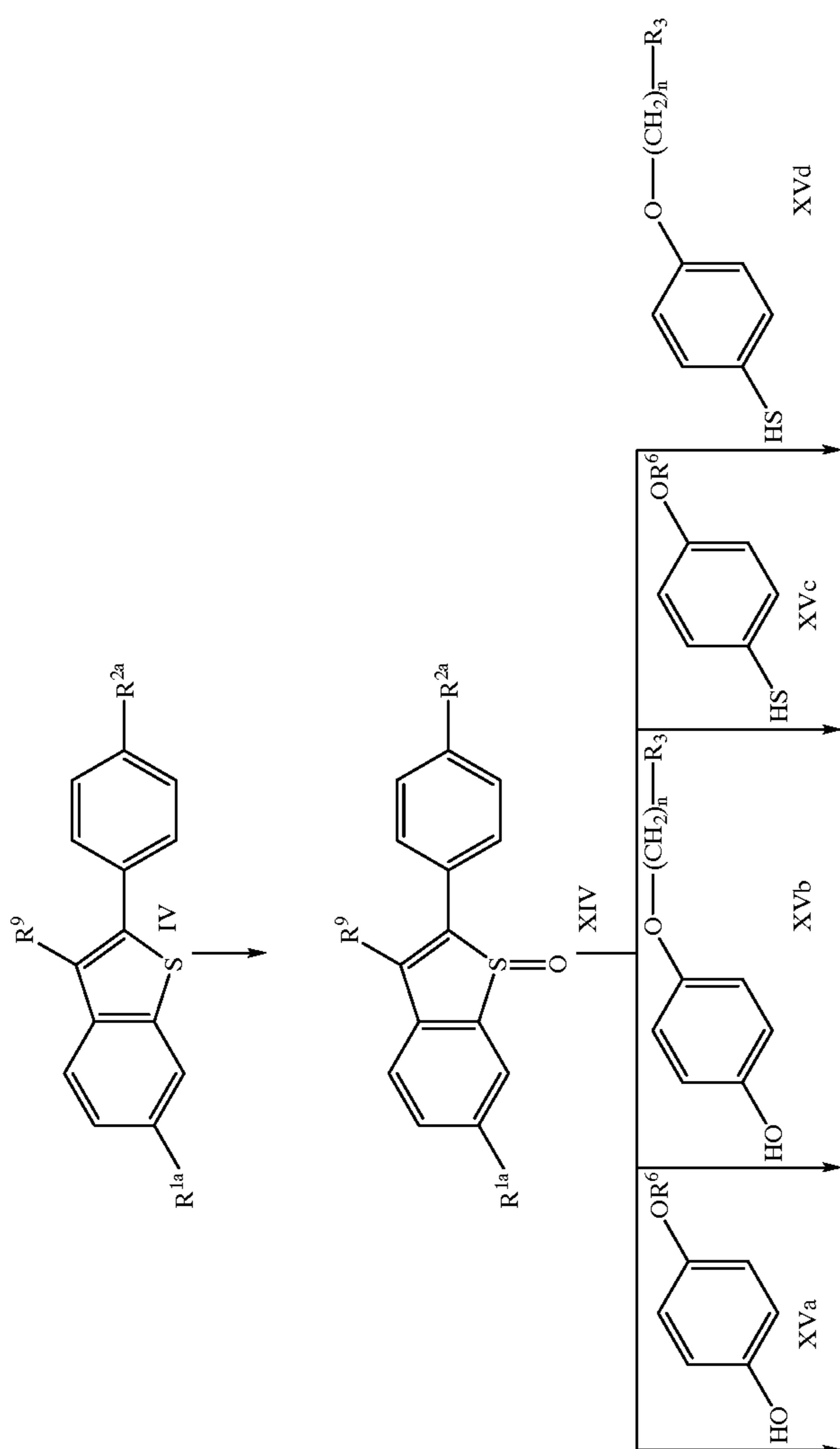
Scheme V
