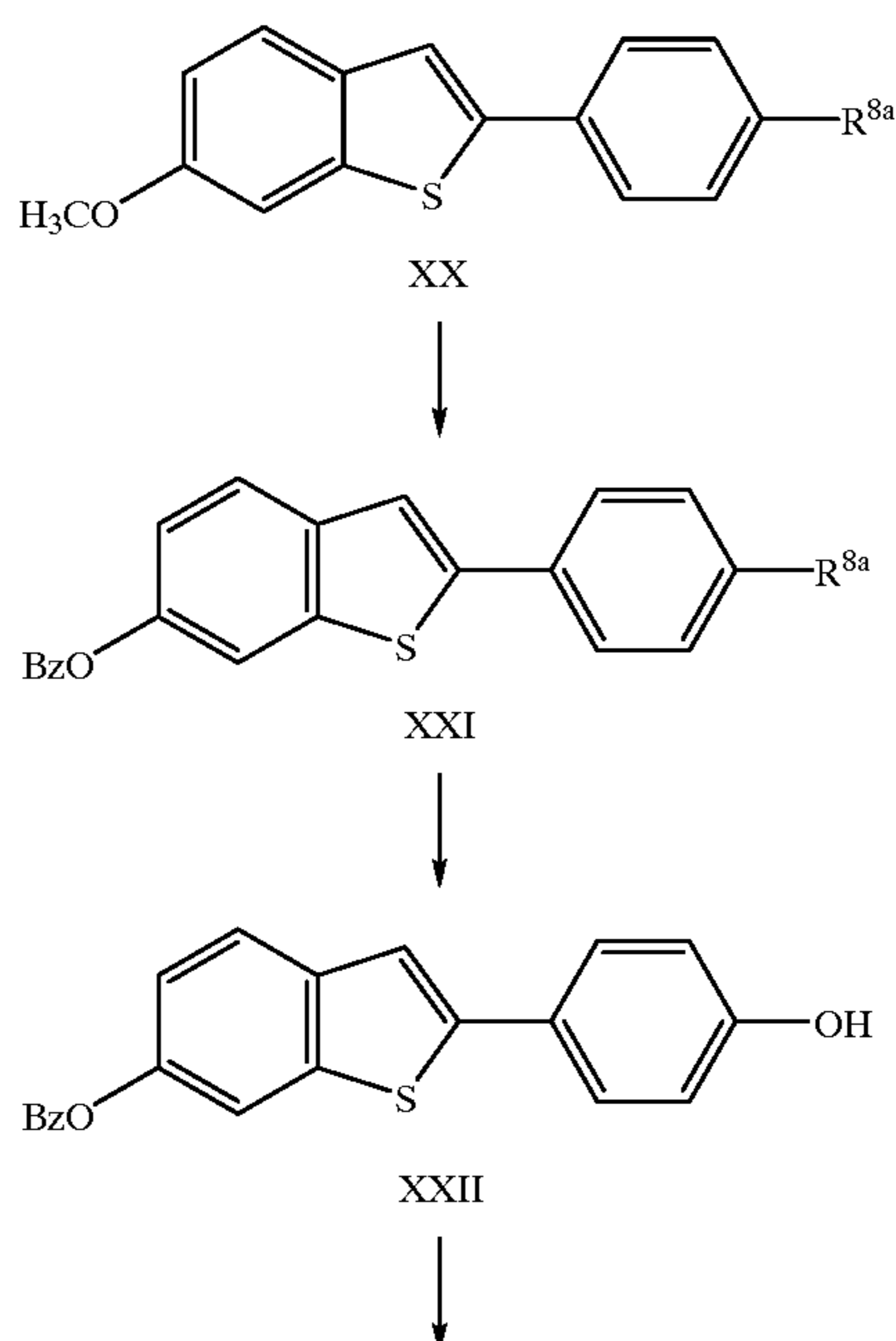
Scheme VII
