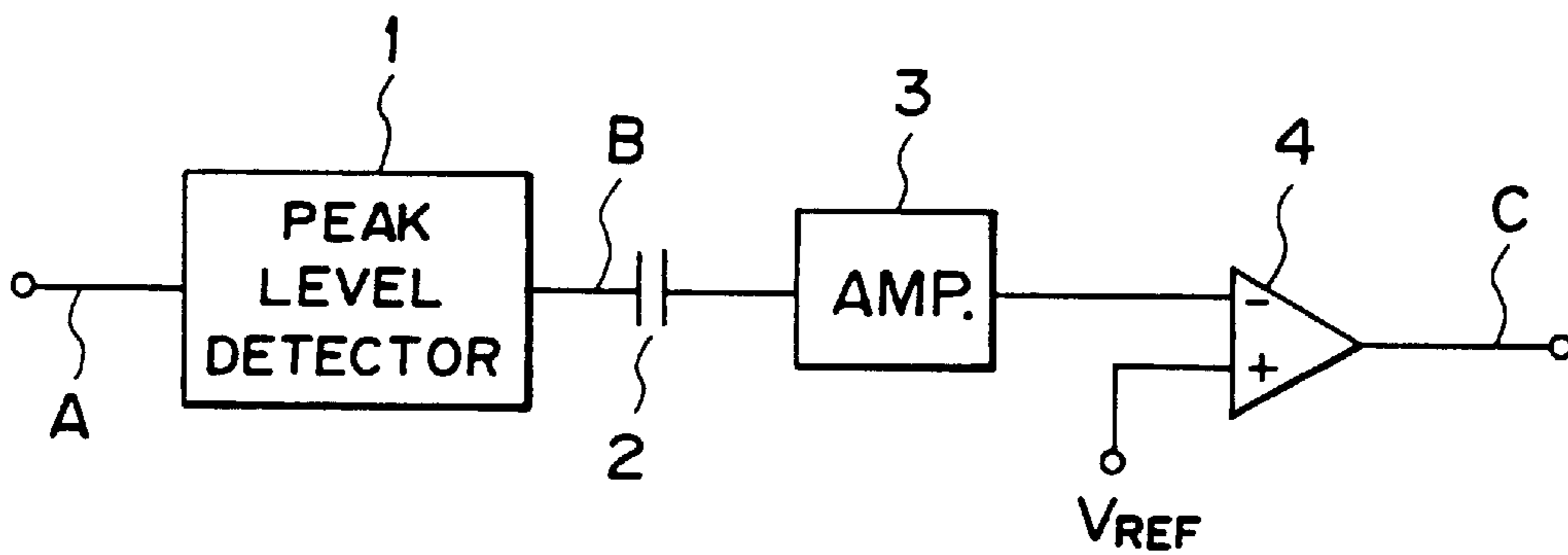
FIG. 2 PRIOR ART
