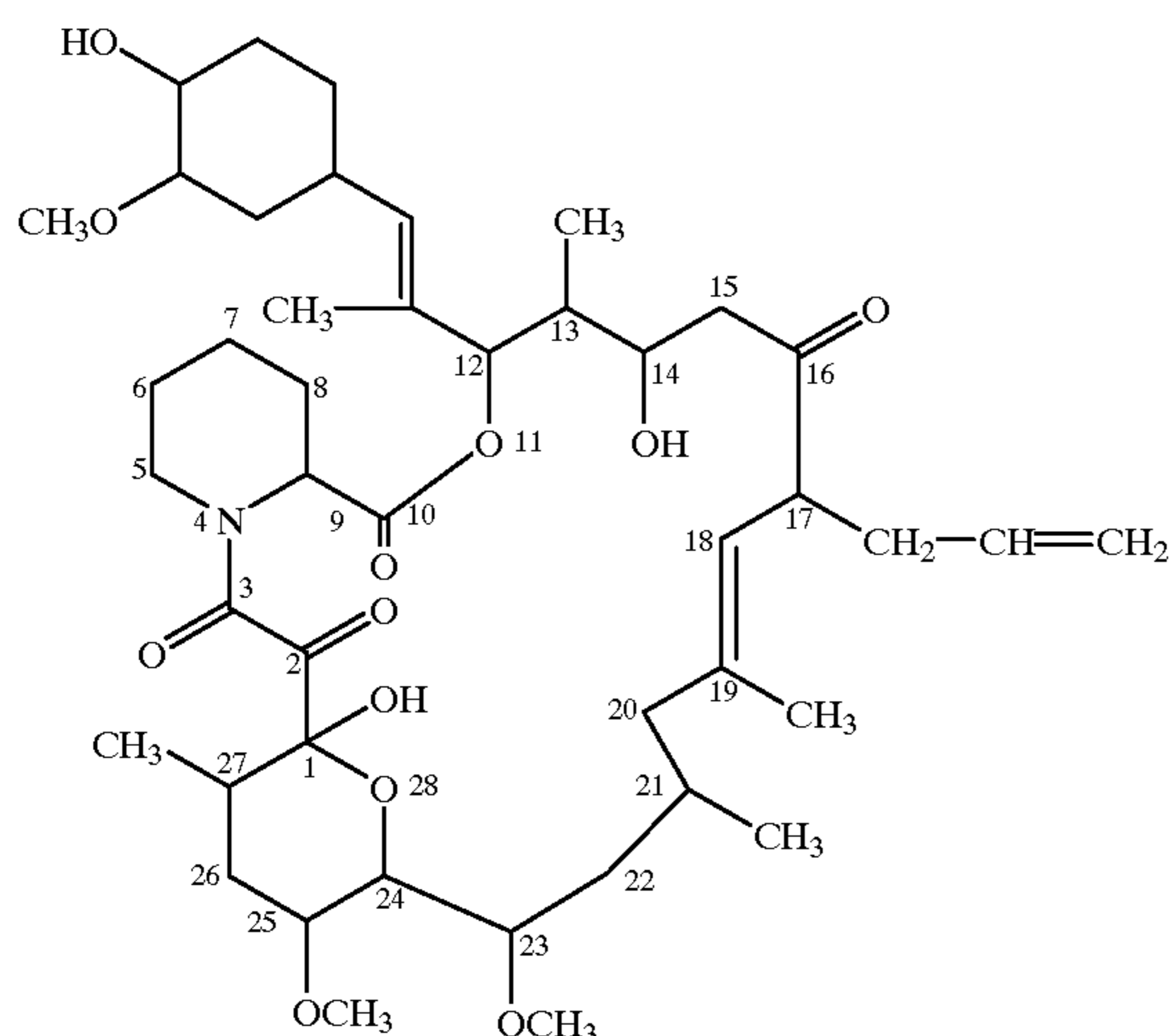
17-Allyl-1,14-dihydroxy-12-[2-(4-hydroxy-3-methoxycyclohexyl)-1-methylvinyl]-23,25-dimethoxy-13,19,21,27-tetramethyl-11,28-dioxo-4-azatricyclo[22.3.1.0 4,9 ]octacos-18-ene-2,3,10,16-
