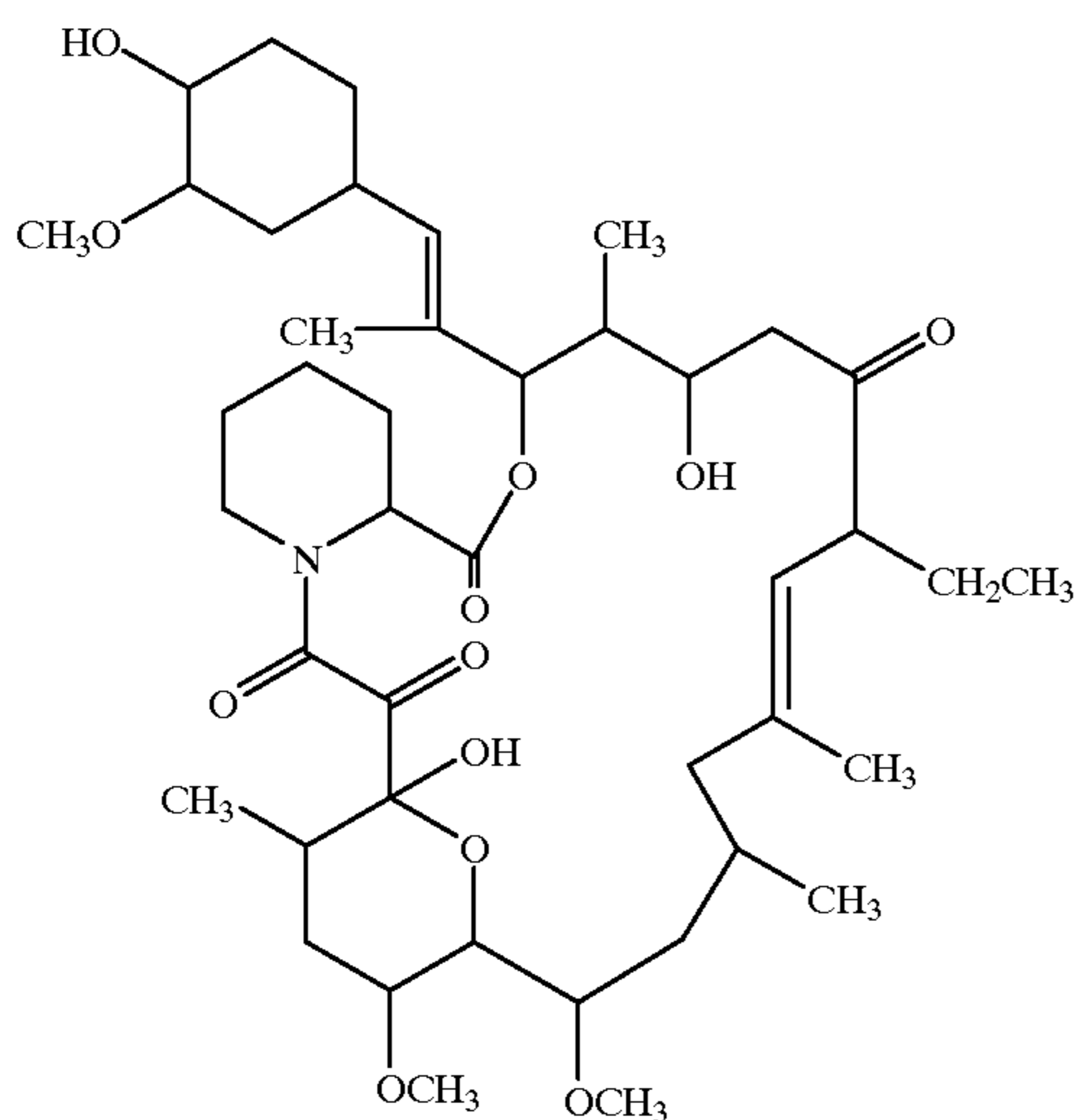
17-Ethyl-1,14-dihydroxy-12-[2-(4-hydroxy-3-methoxycyclohexyl)-1-methylvinyl]-23,25-dimethoxy-13,19,21,27-tetramethyl-11,28-dioxo-4-azatricyclo-[22.3.1.0 4,9 ]octacos-18-ene-2,3,10,16-tetraone
