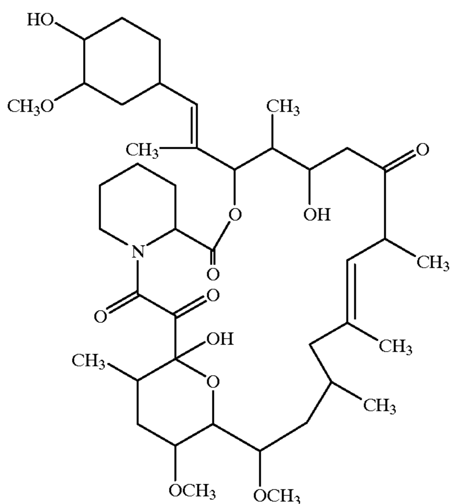
1,14-Dihydroxy-12-[2-(4-hydroxy-3-methoxycyclohexyl)-1-methylvinyl]-23,25-dimethoxy-13,19,17,21,27-pentamethyl-11,28-dioxo-4-azatricyclo[22.3.1.0 4,9 ]octacos-18-ene-2,3,10,16-tetraone
