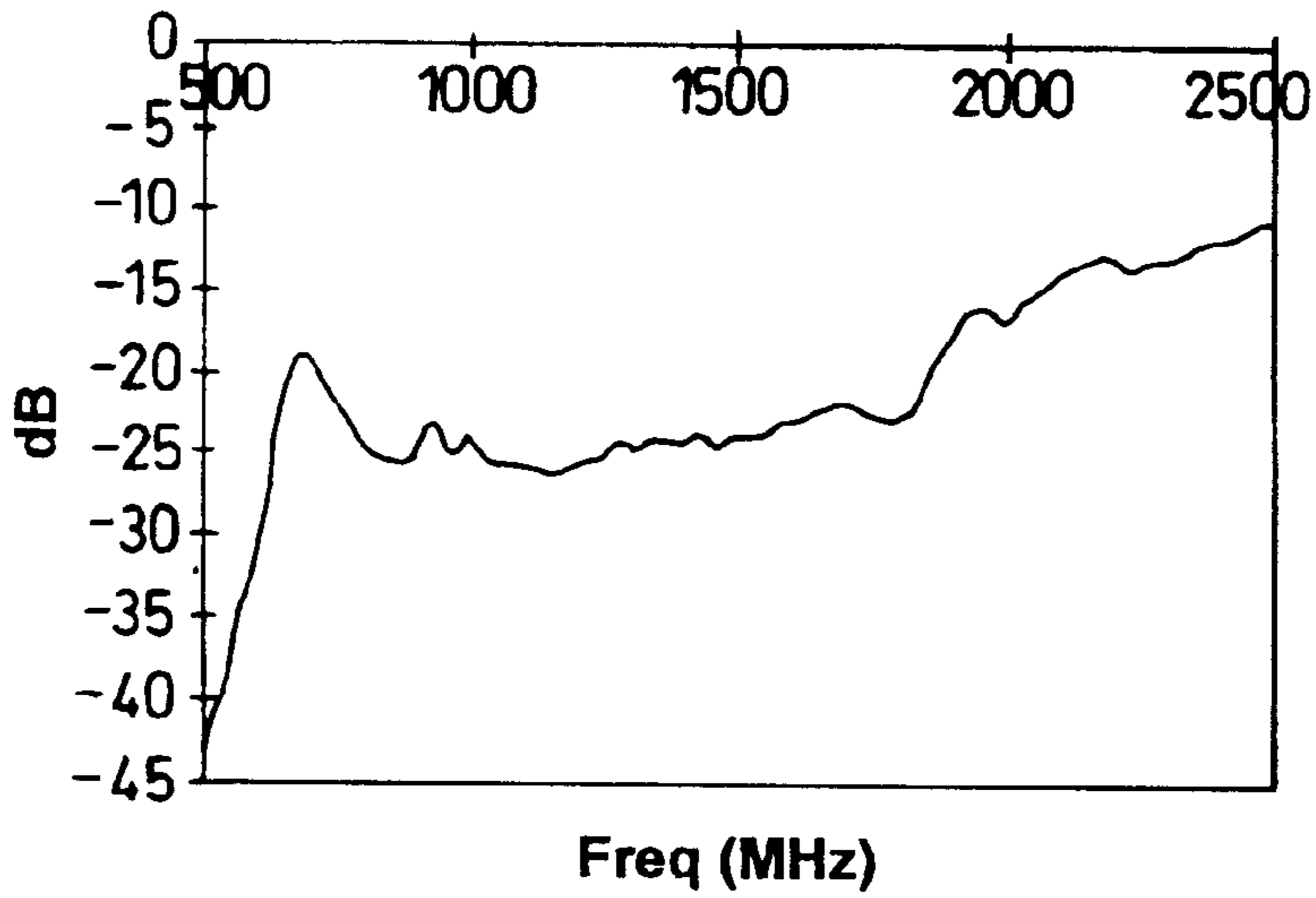
Inter-antenna Coupling
