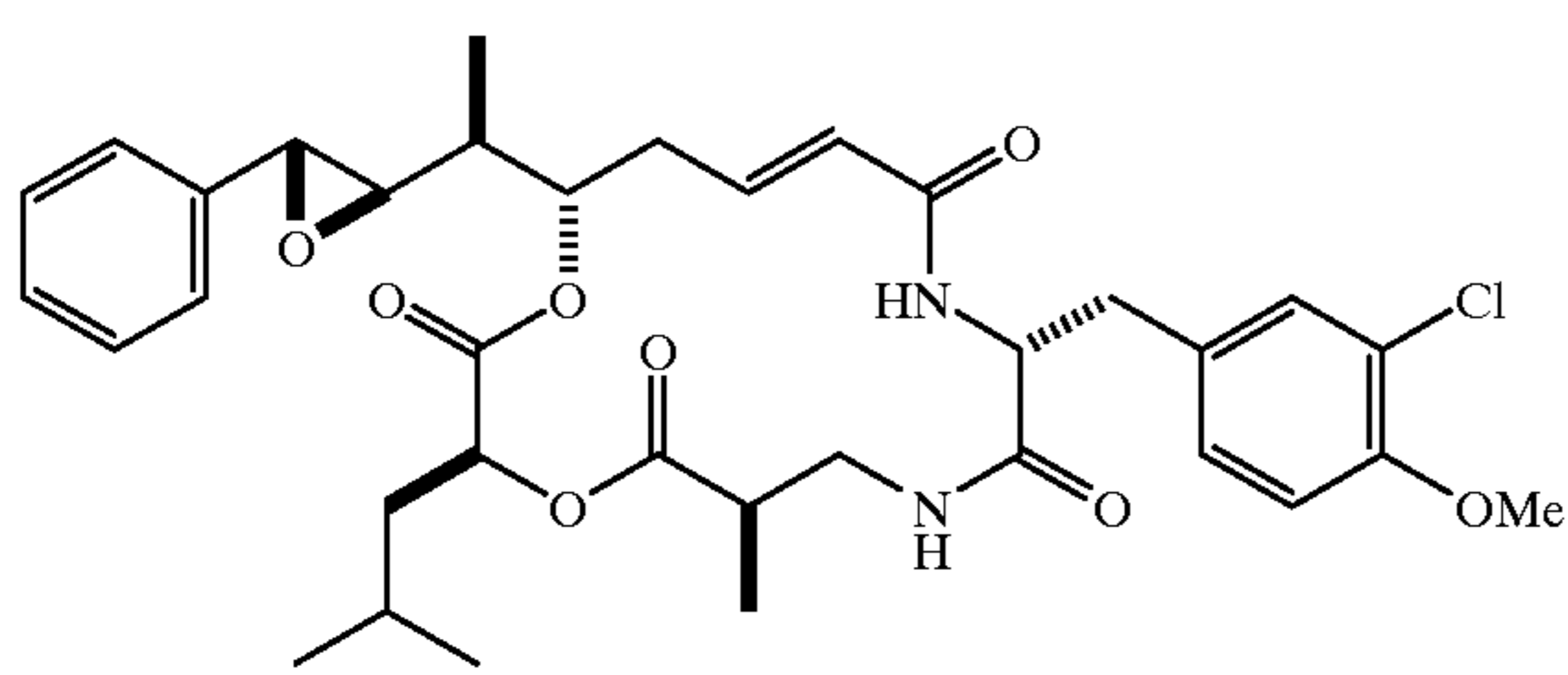
Cryptophycin
