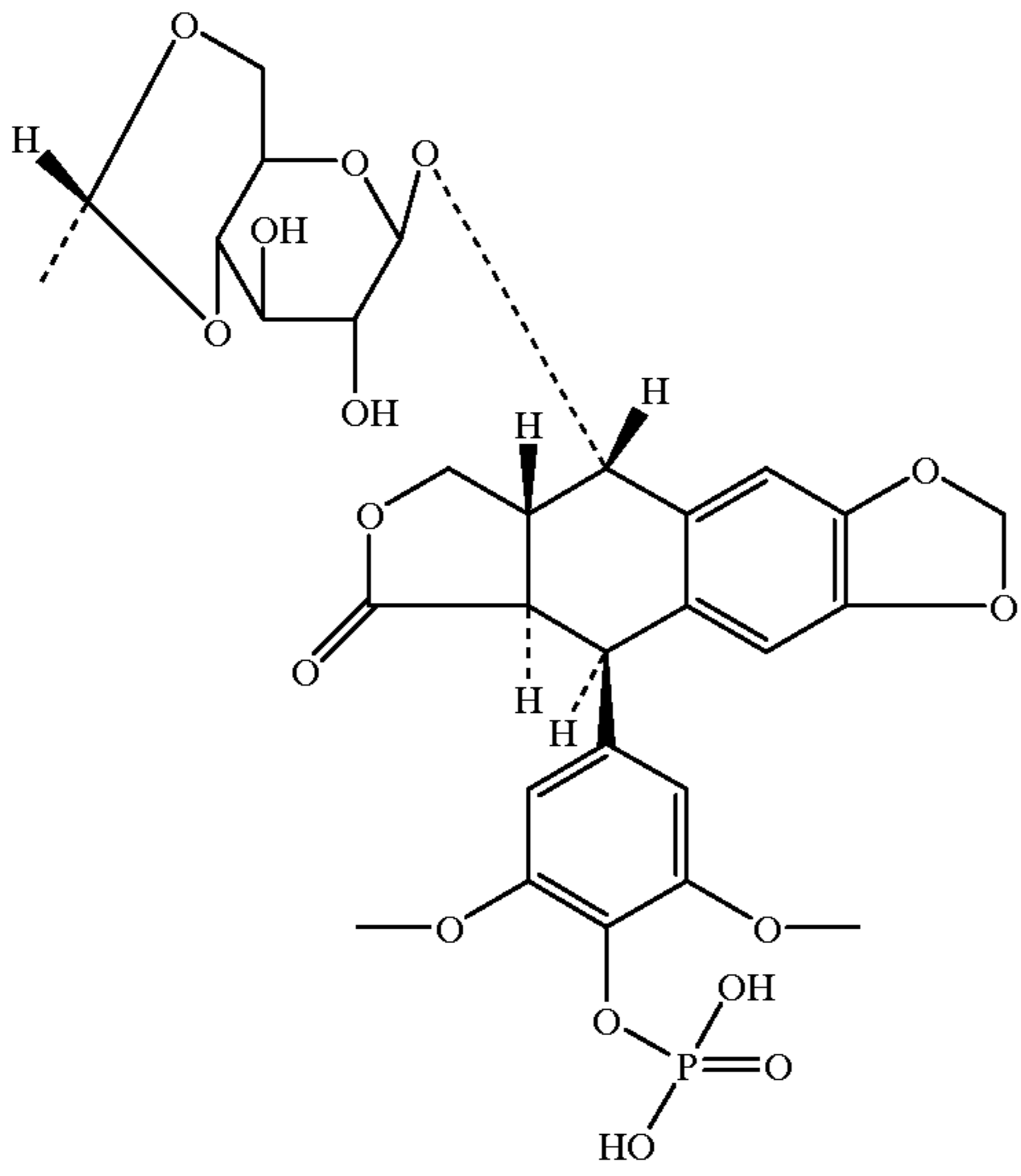
Etoposide Phosphate
