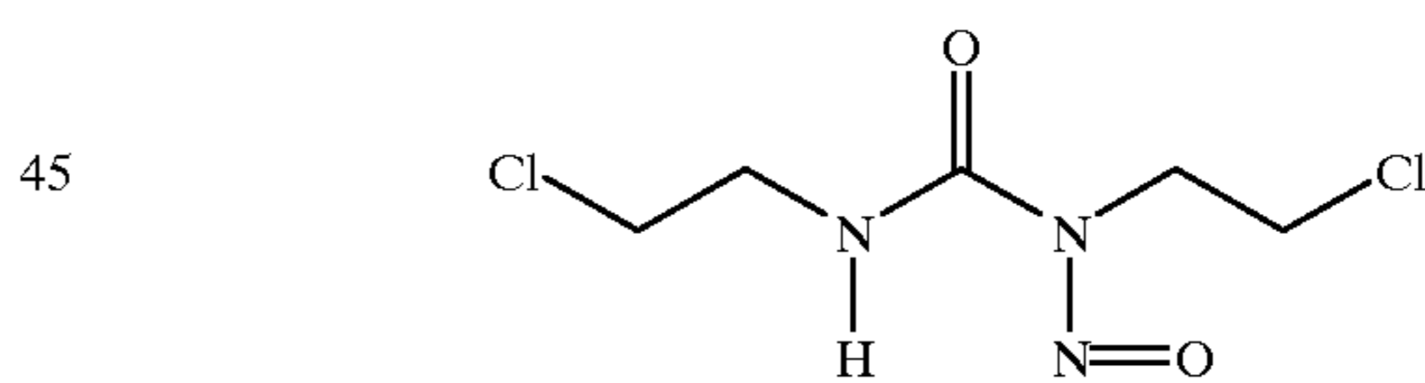
Carmustine (BCNU)
