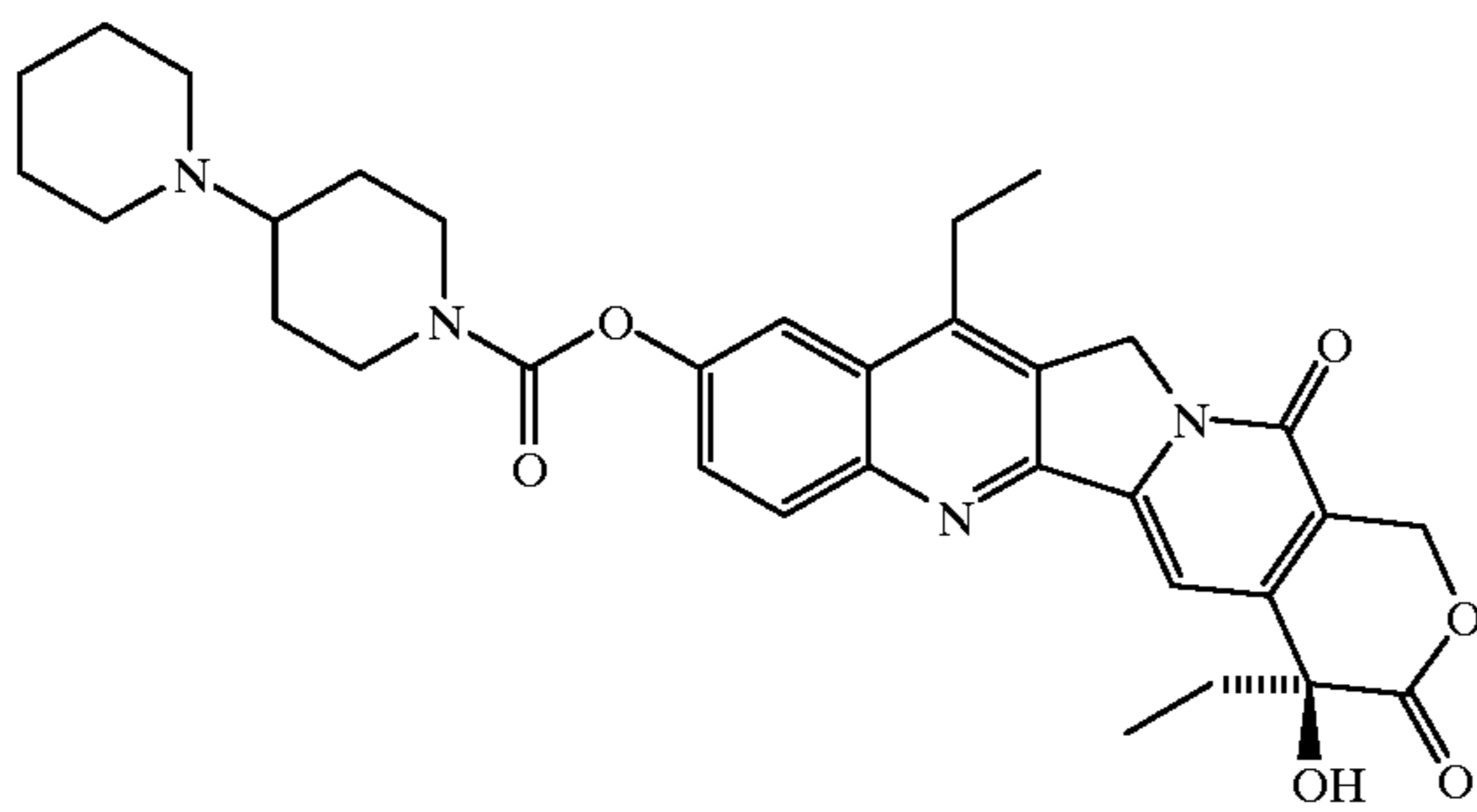
Irinotecan
