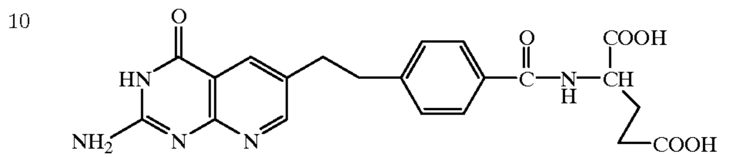
5,10-dideaza tetrahydrofolate
