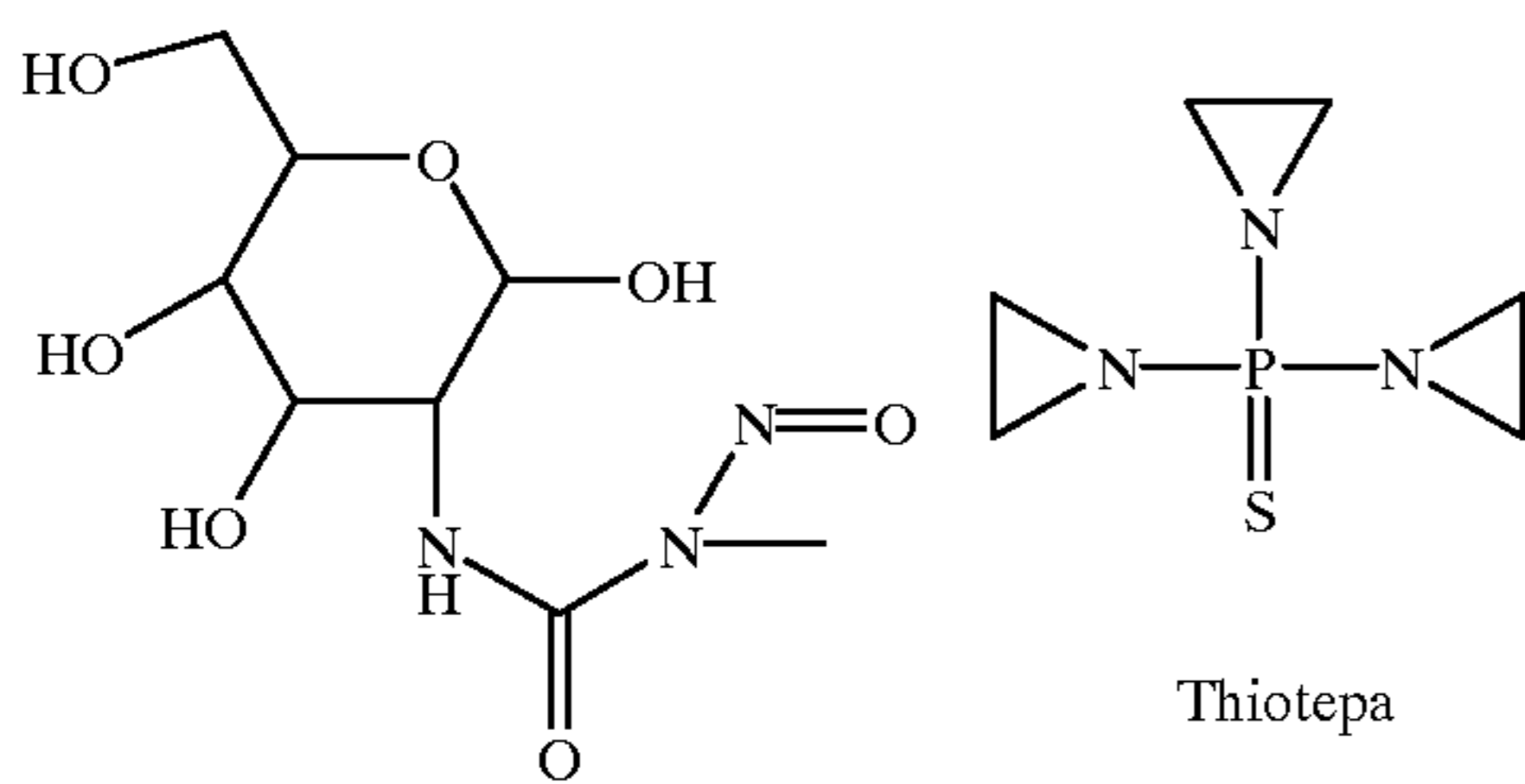
Streptozocin
