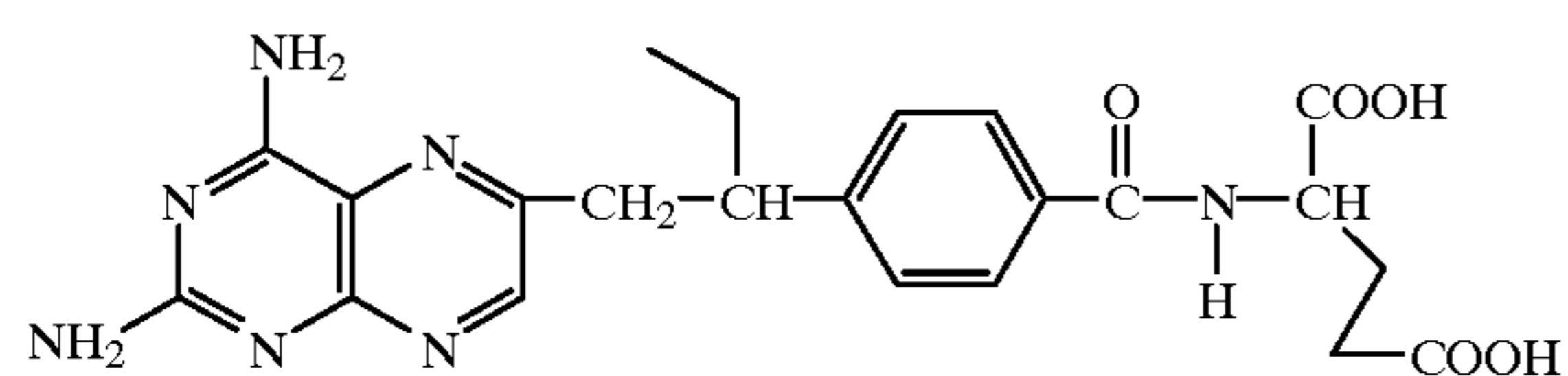
10-ethyl-10-deazaaminopterin (EDAM)
