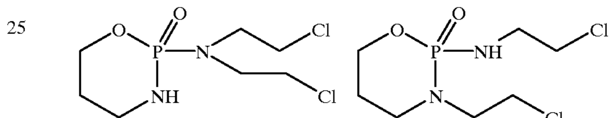
Cyclophosphamide
