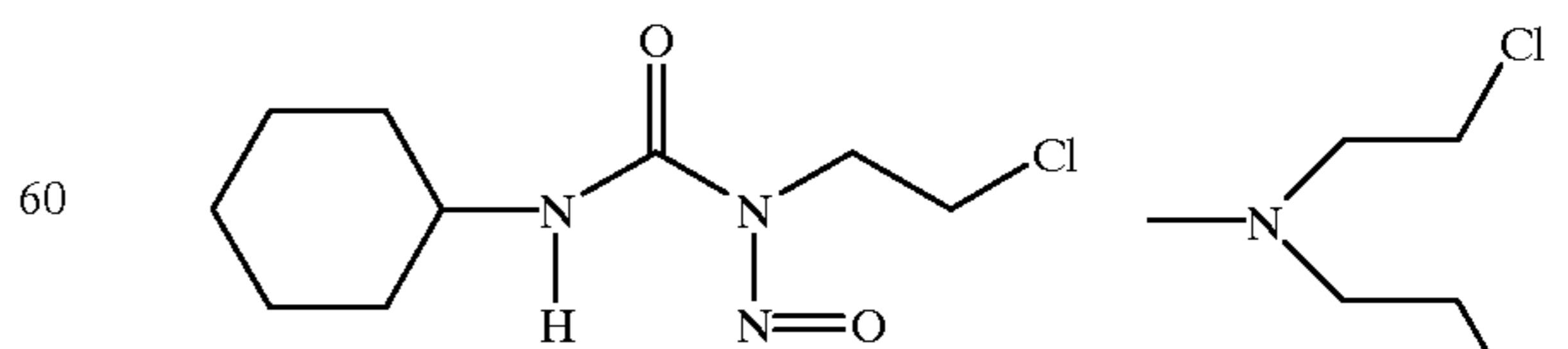
Lomustine (CCNU)
