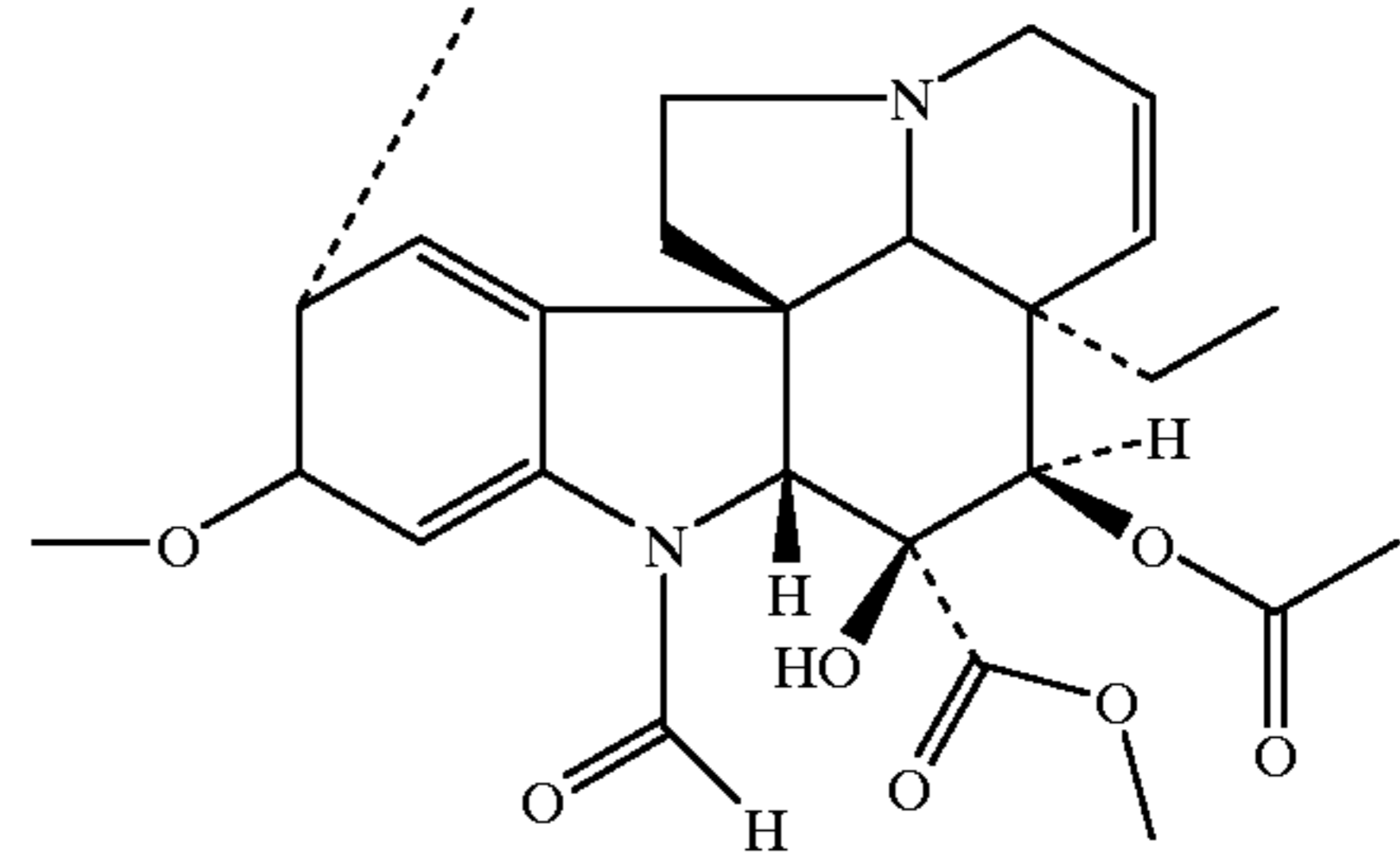
Vincristine
