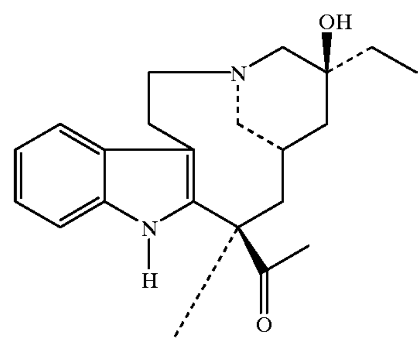
Taxotere
