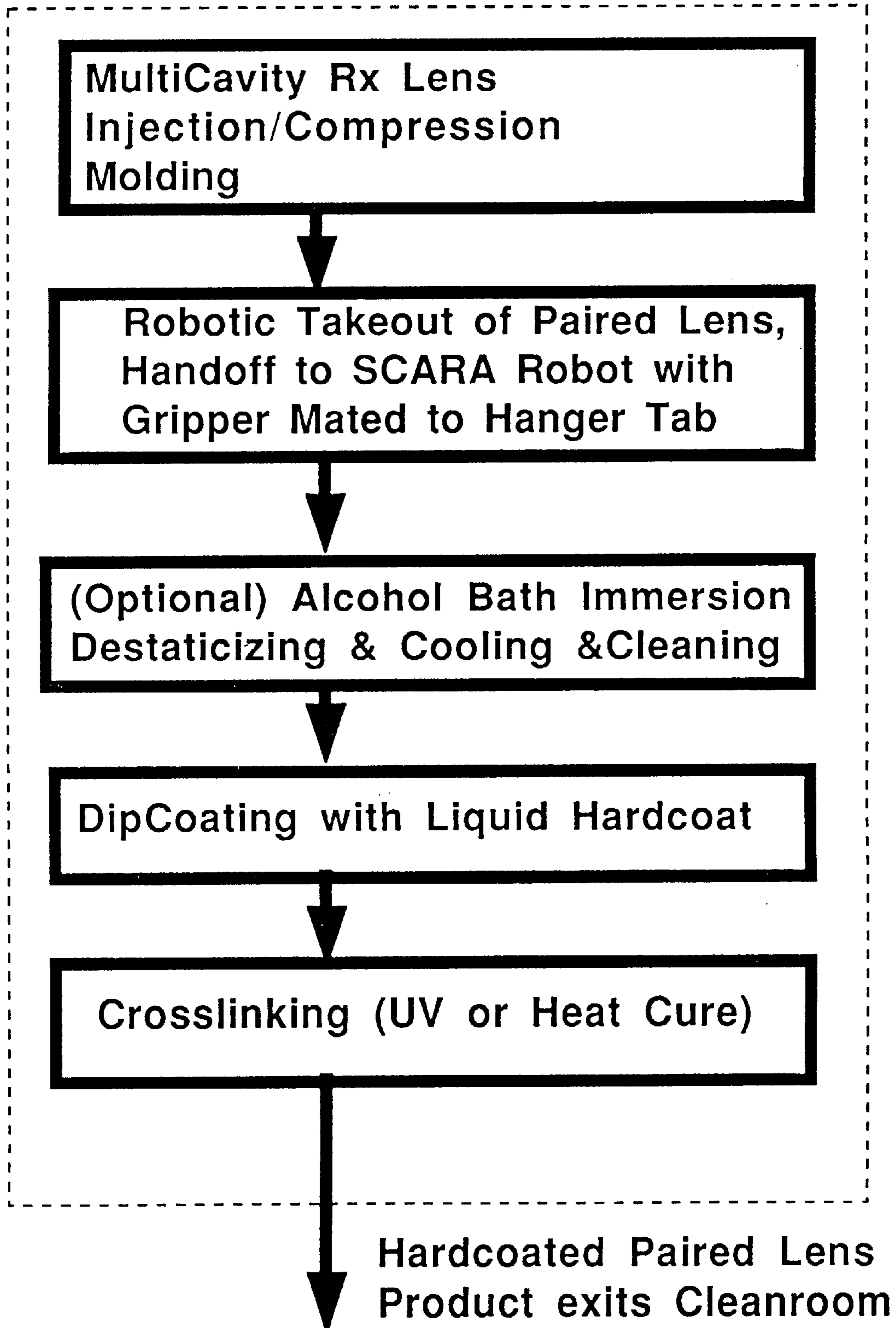
Figure 4B: Automated "Mold and Dipcoat" ("Continuous Process")
