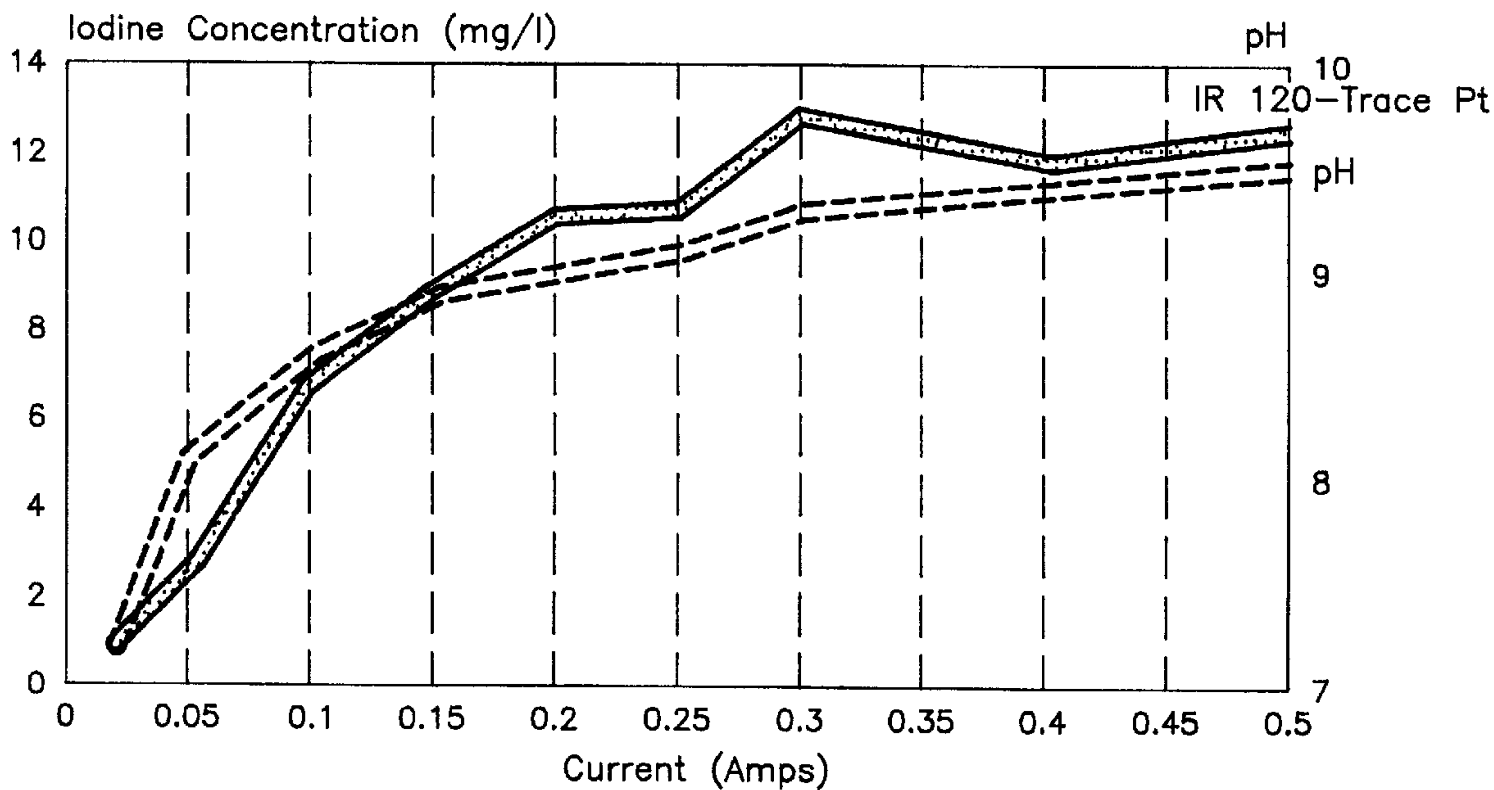
Iodine Concentration (mg/l) at 1 LPM
