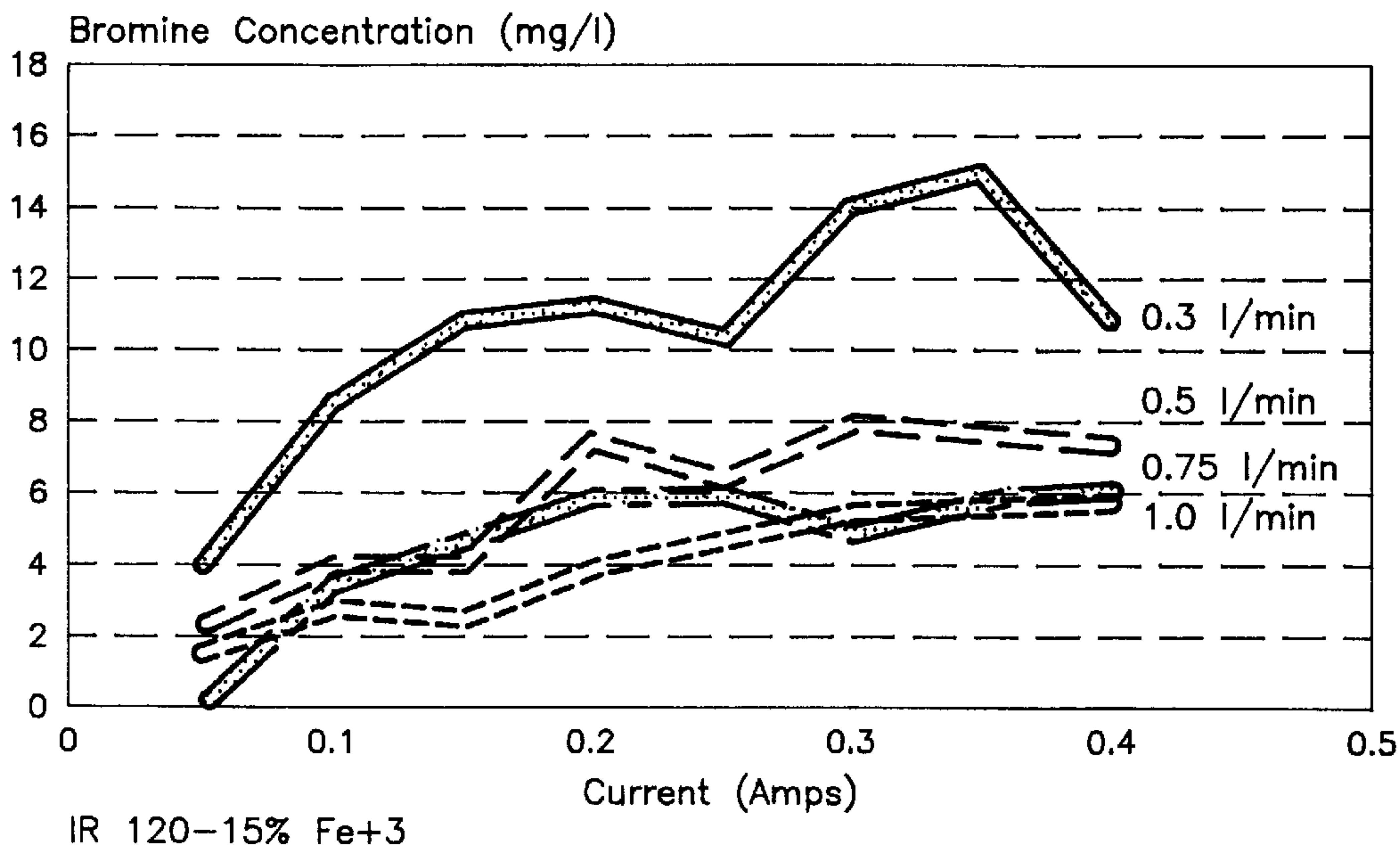
Bromine Concentration (mg/l) at Various Flowrates
