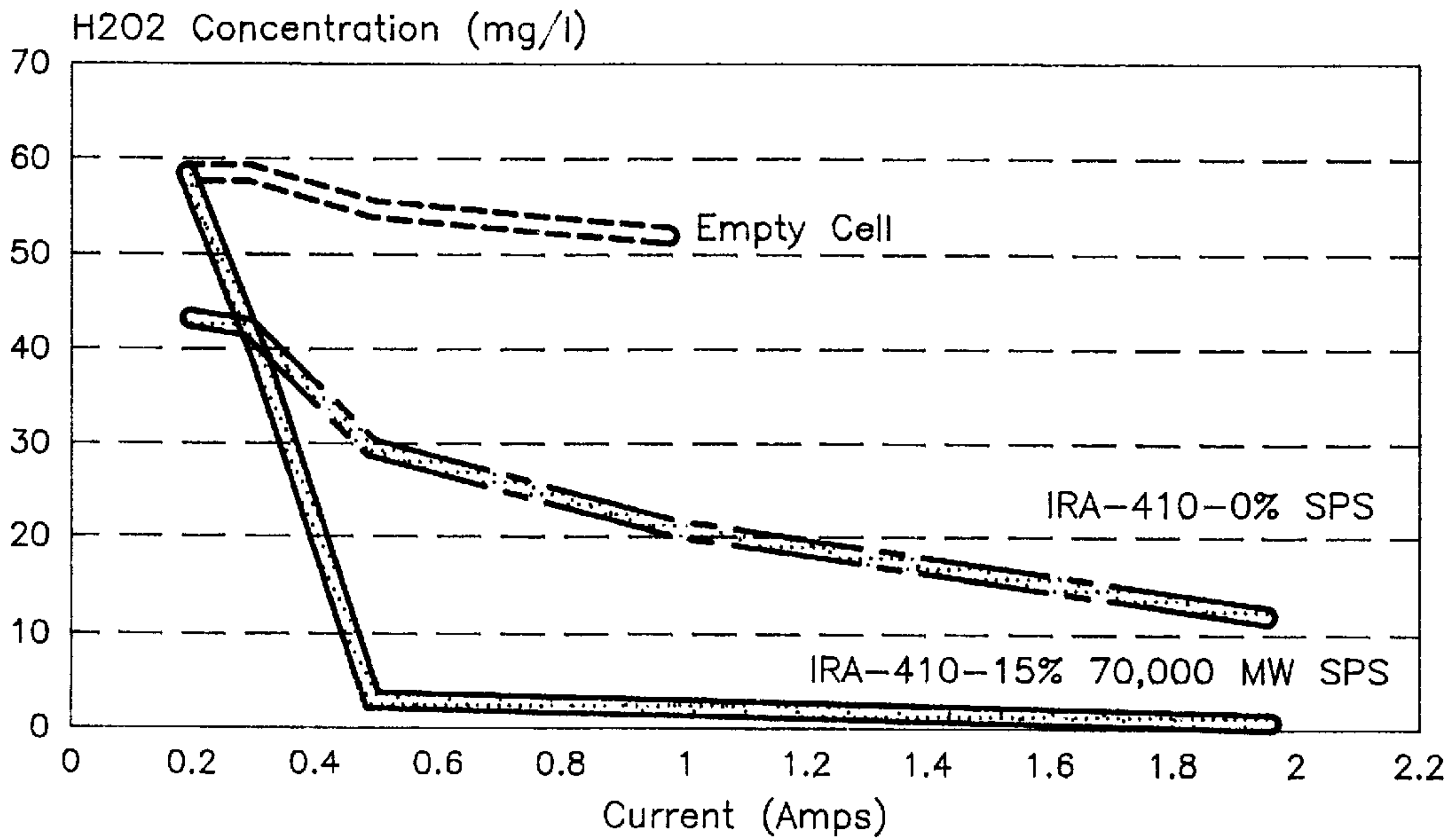
FIG. 12 Reduction of Hydrogen Peroxide (mg/l)
