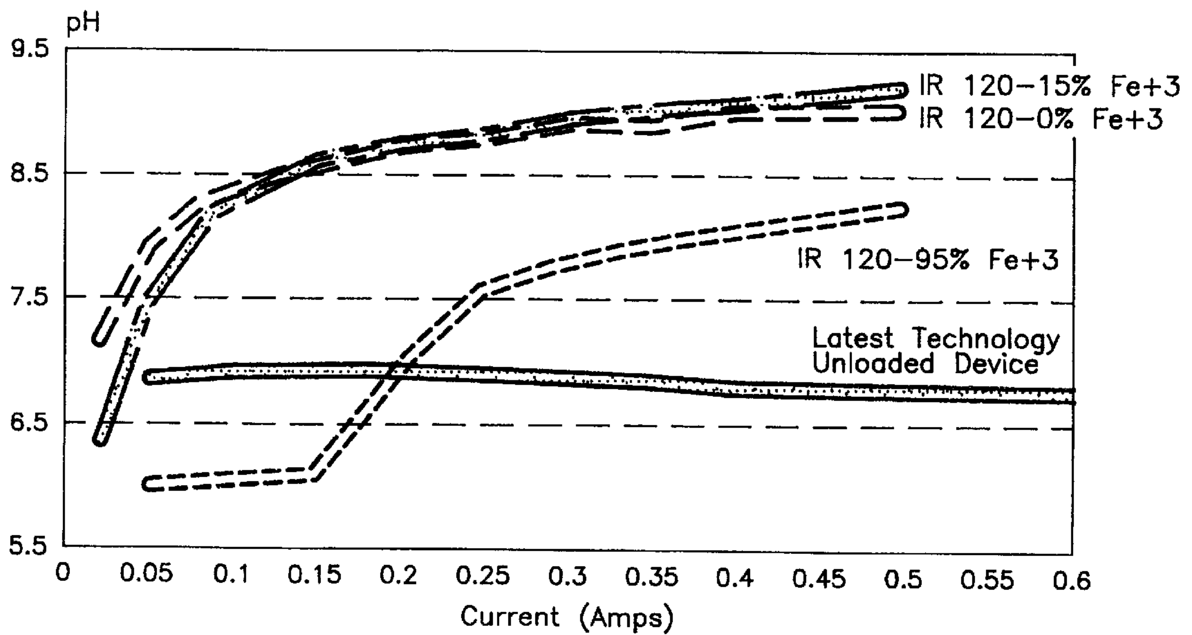
FIG. 4 pH at 1 LPM
