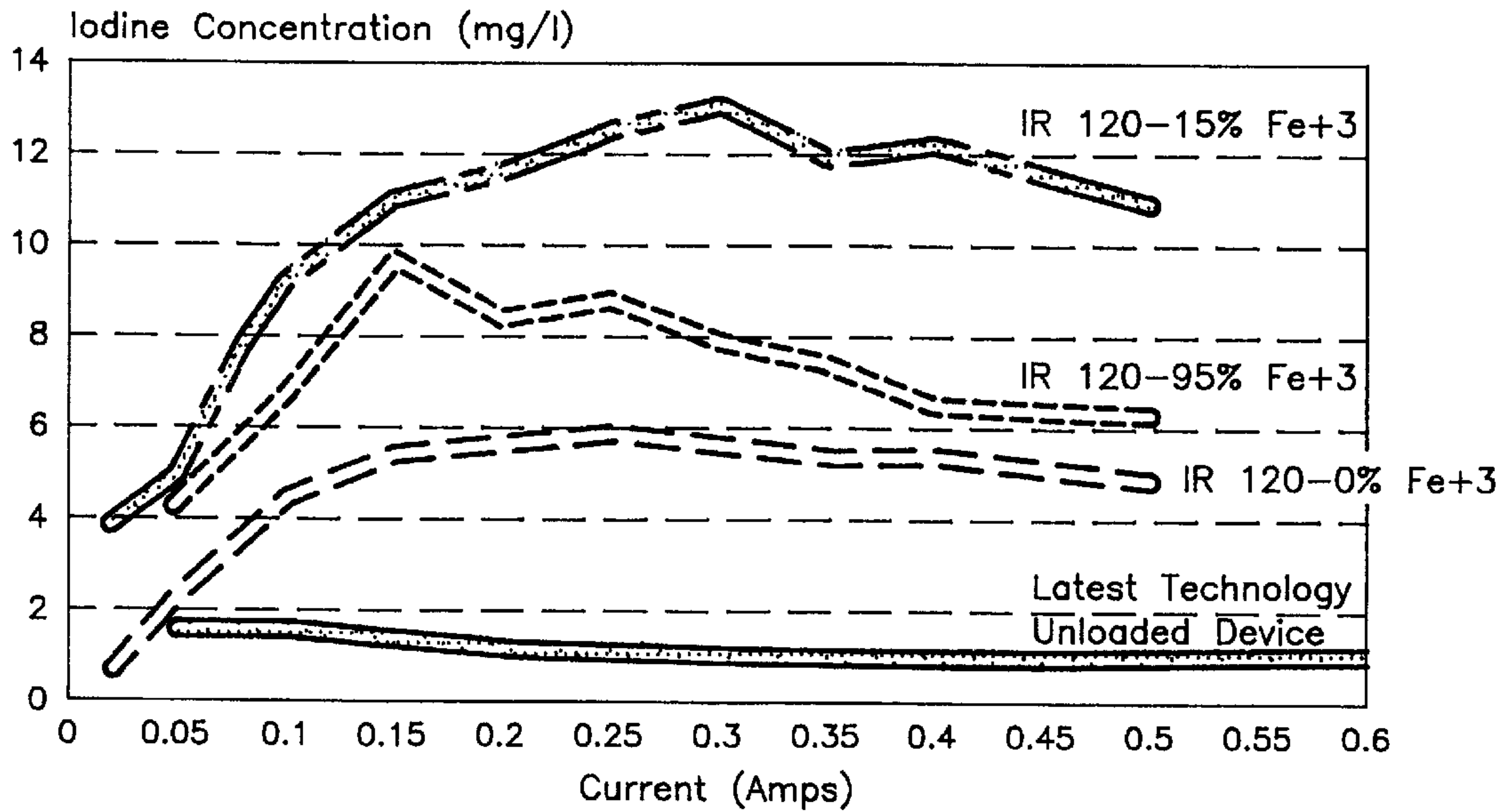
FIG. 3 Iodine Concentration (mg/l) at LPM
