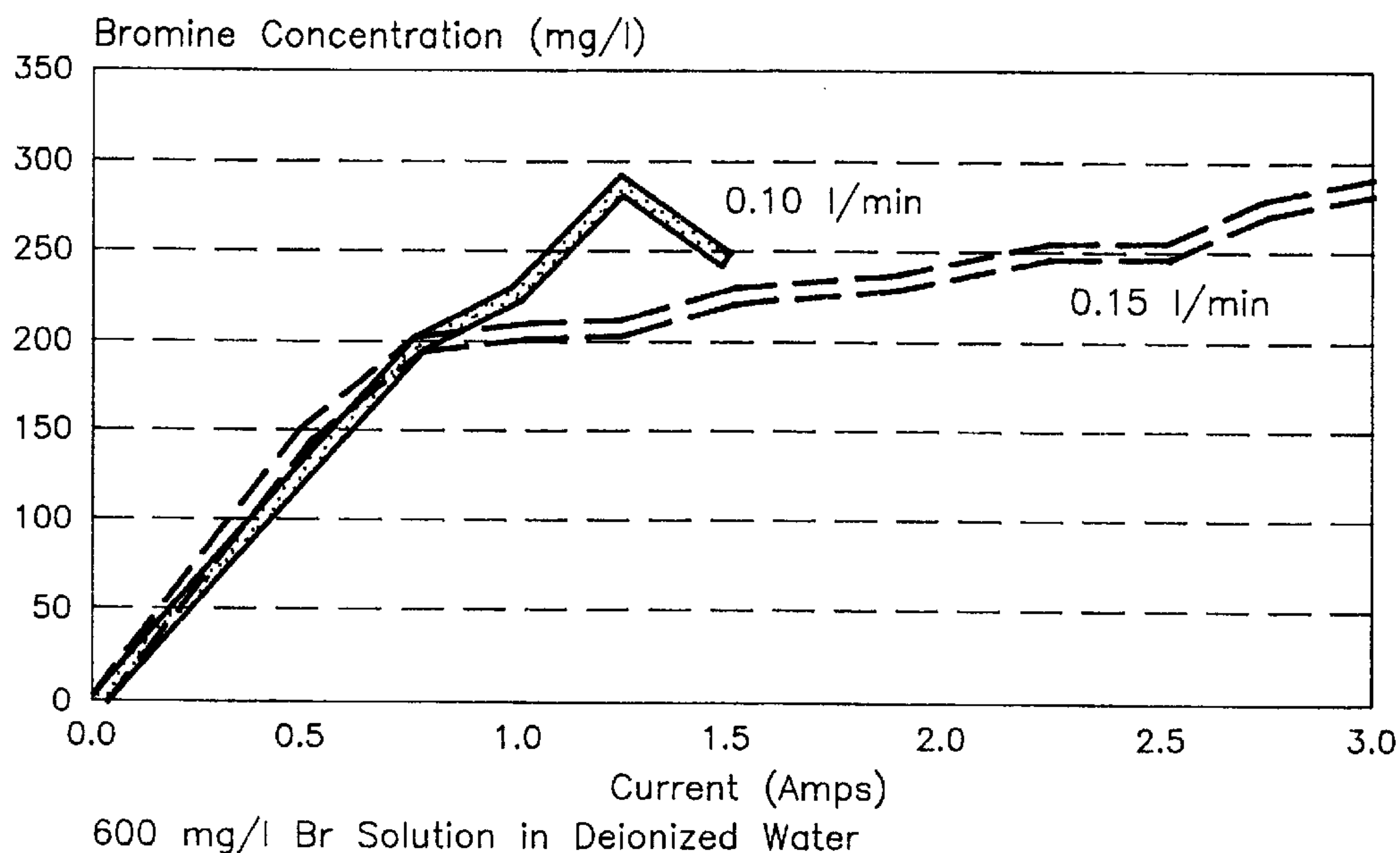
FIG. 9 Bromine Concentration (mg/l) at Various Flowrates
