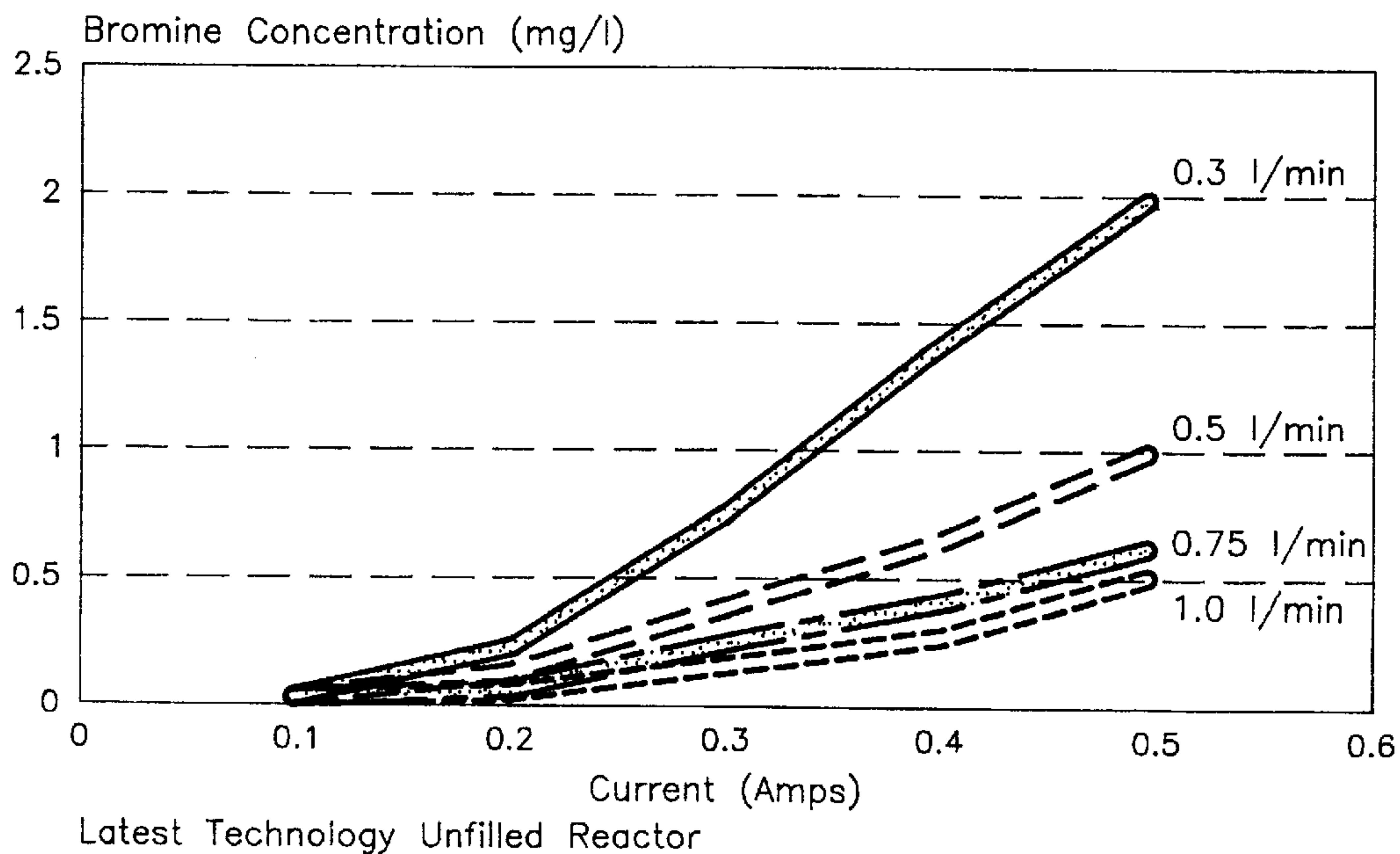
FIG. 10 Bromine Concentration (mg/l) at Various Flowrates
