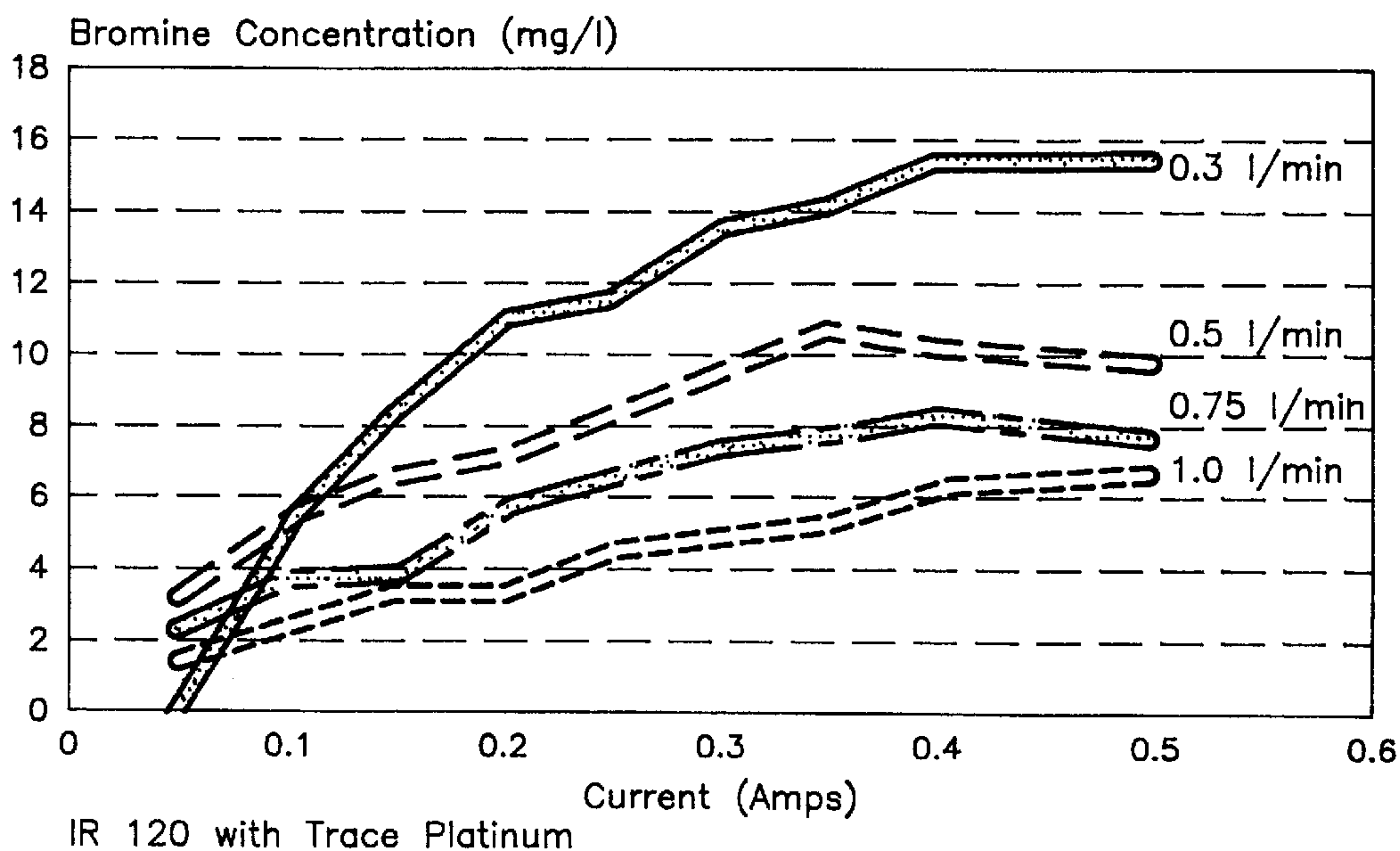
Bromine Concentration (mg/l) at Various Flowrates
