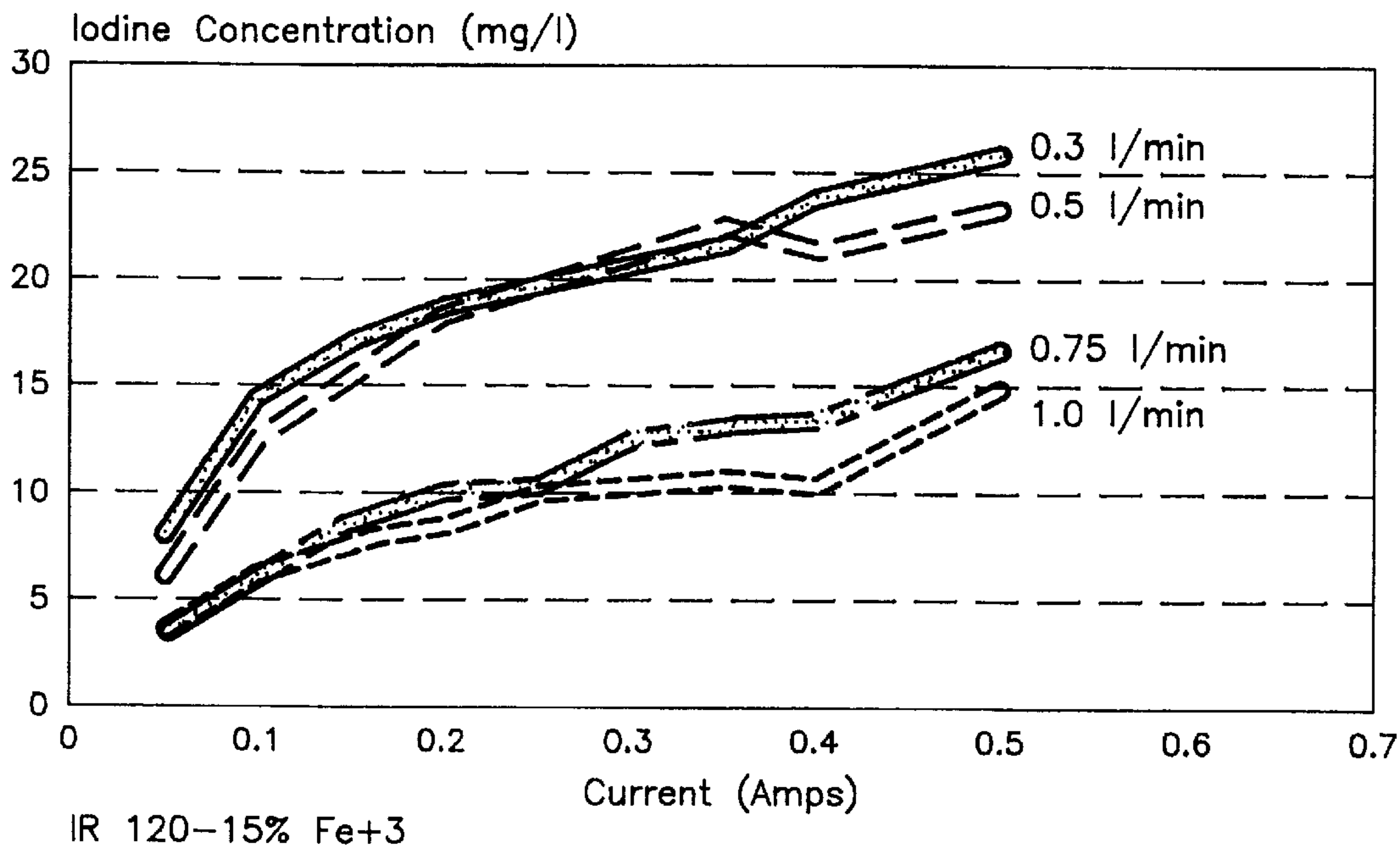
Iodine Concentration (mg/l) at Various Flowrates
