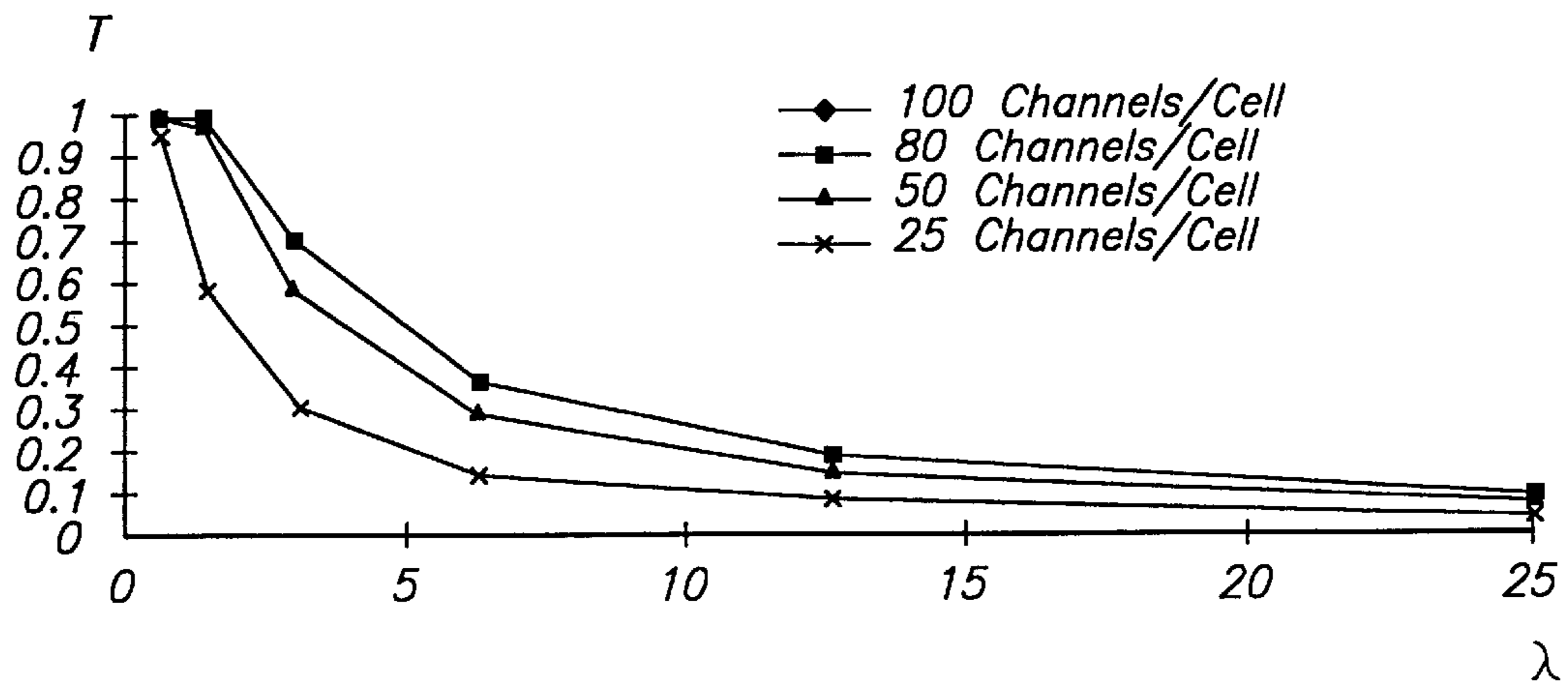
Throughput vs. Offered Load for Varied Configurations of Base Stations (Uniform Load)
