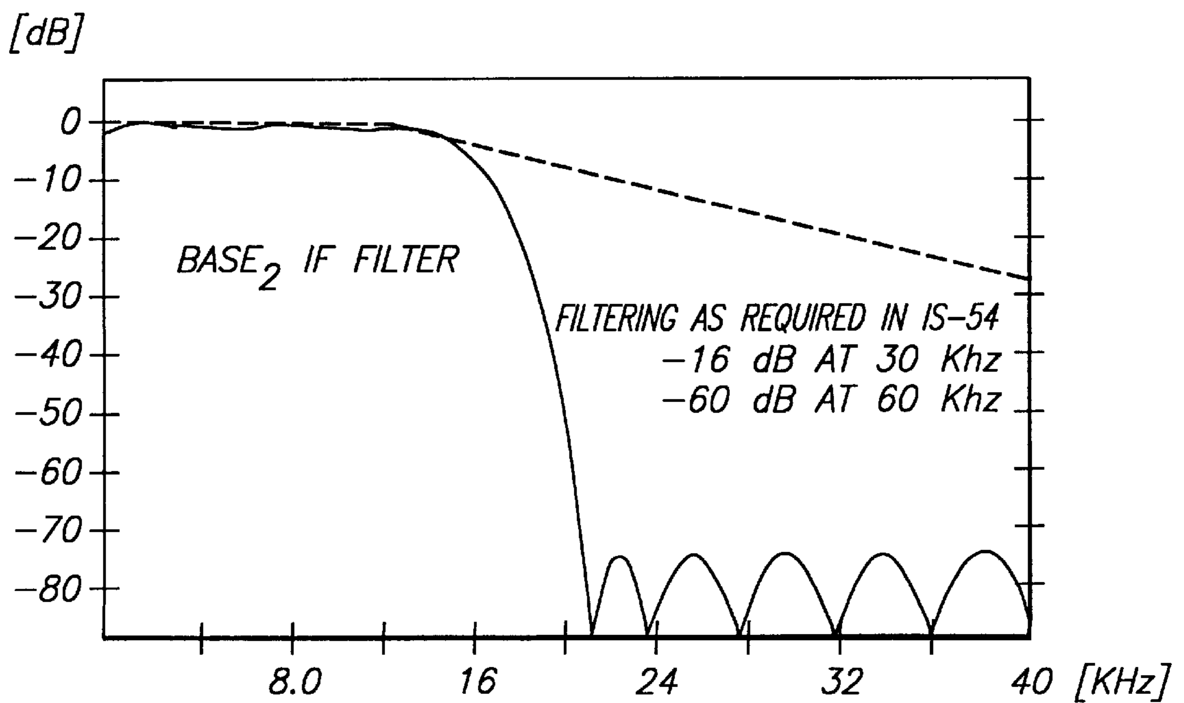
Selectivity Using DSP Techniques
