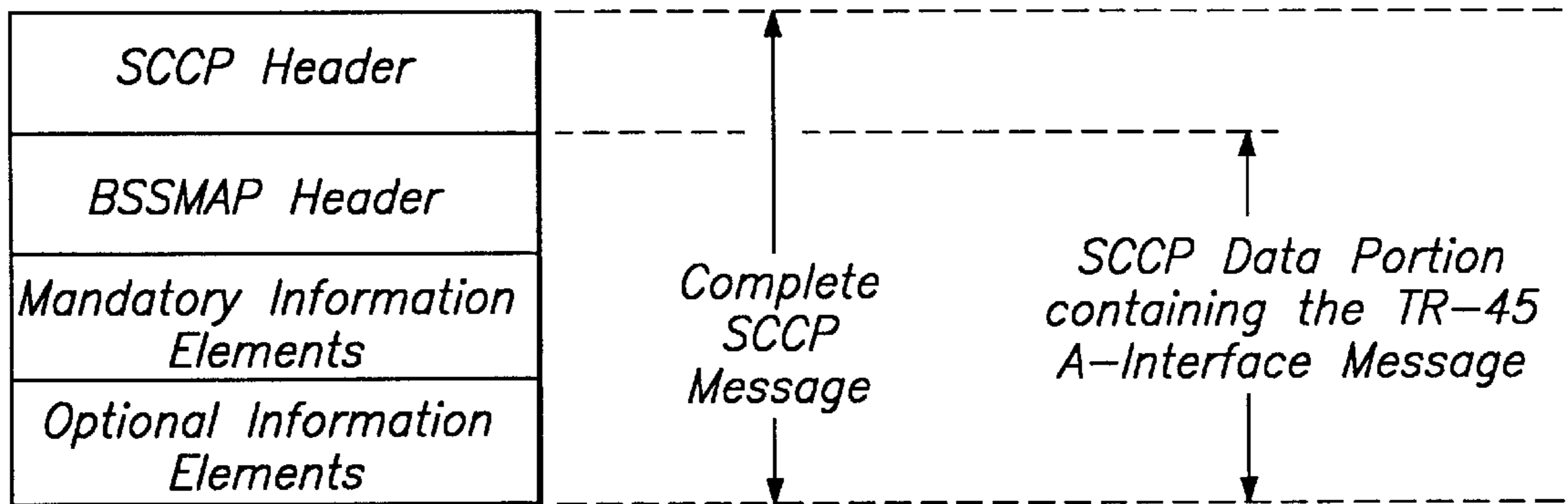
Format of SCCP Messages
