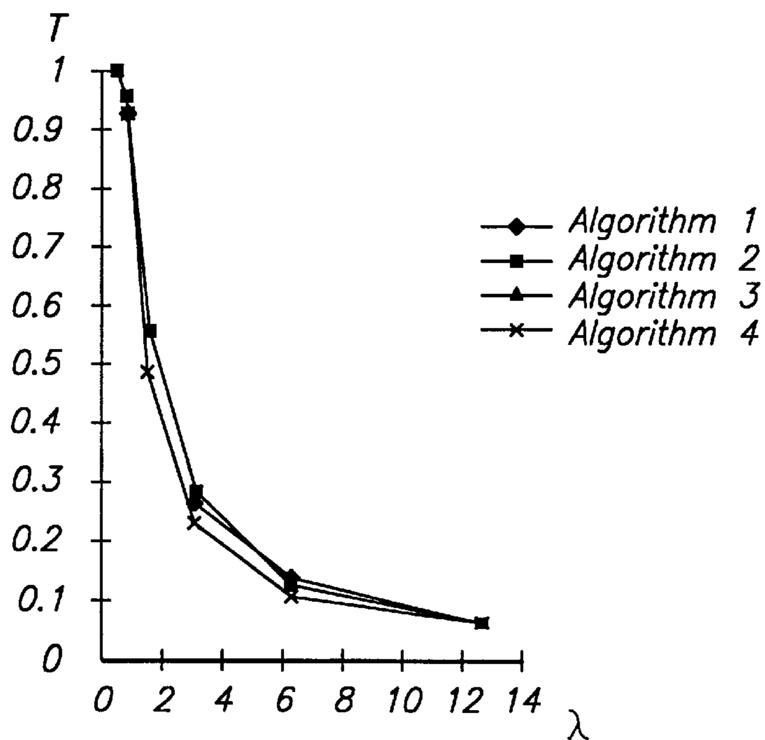
Throughput vs. Offered Load for Different Channel Allocation Algorithms (Uniform Load)
