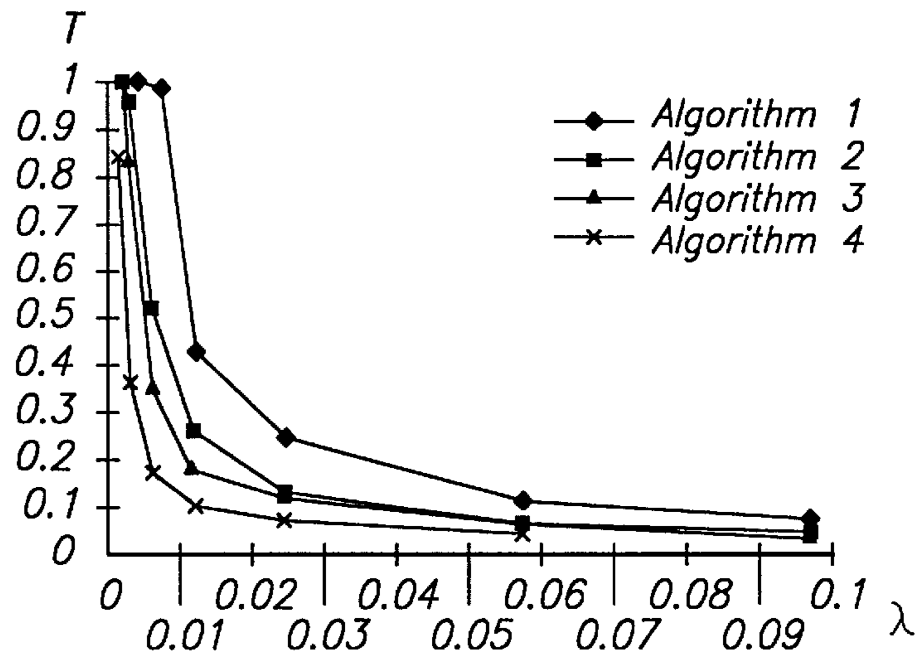
Throughput vs. Offered Load for Different Channel Allocation Algorithms (Non-Uniform Load)
