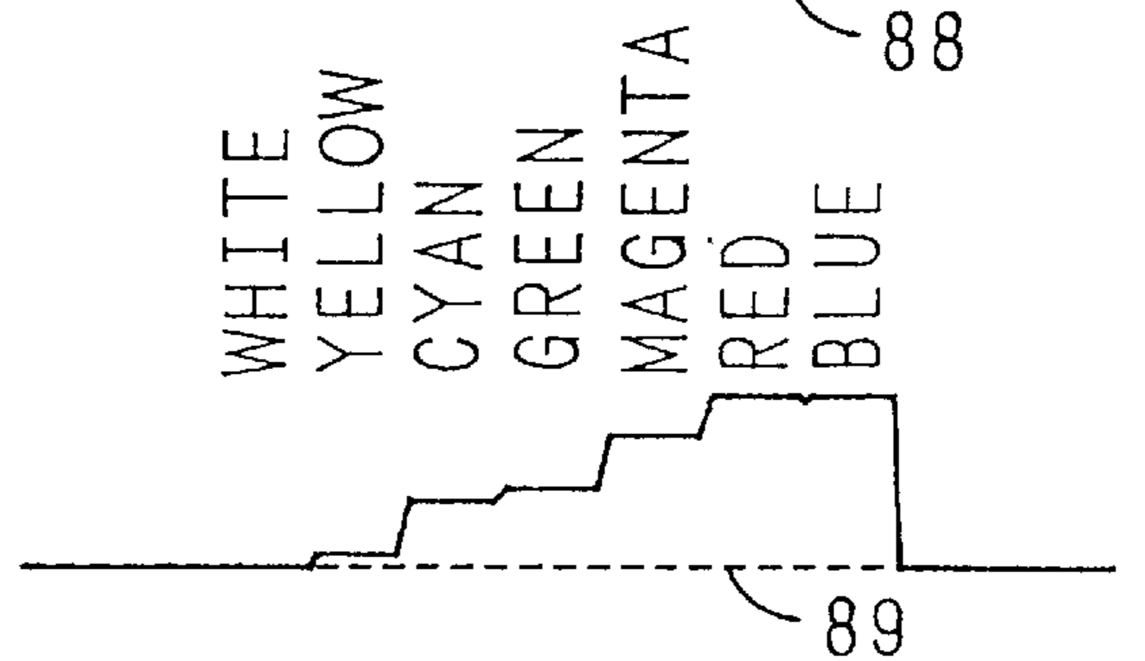
Fig. 14H COLOR DENSITY DETECTION SIGNAL 26
