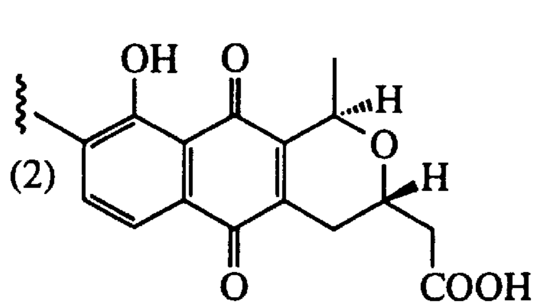
ACTINORHODIN (3)
