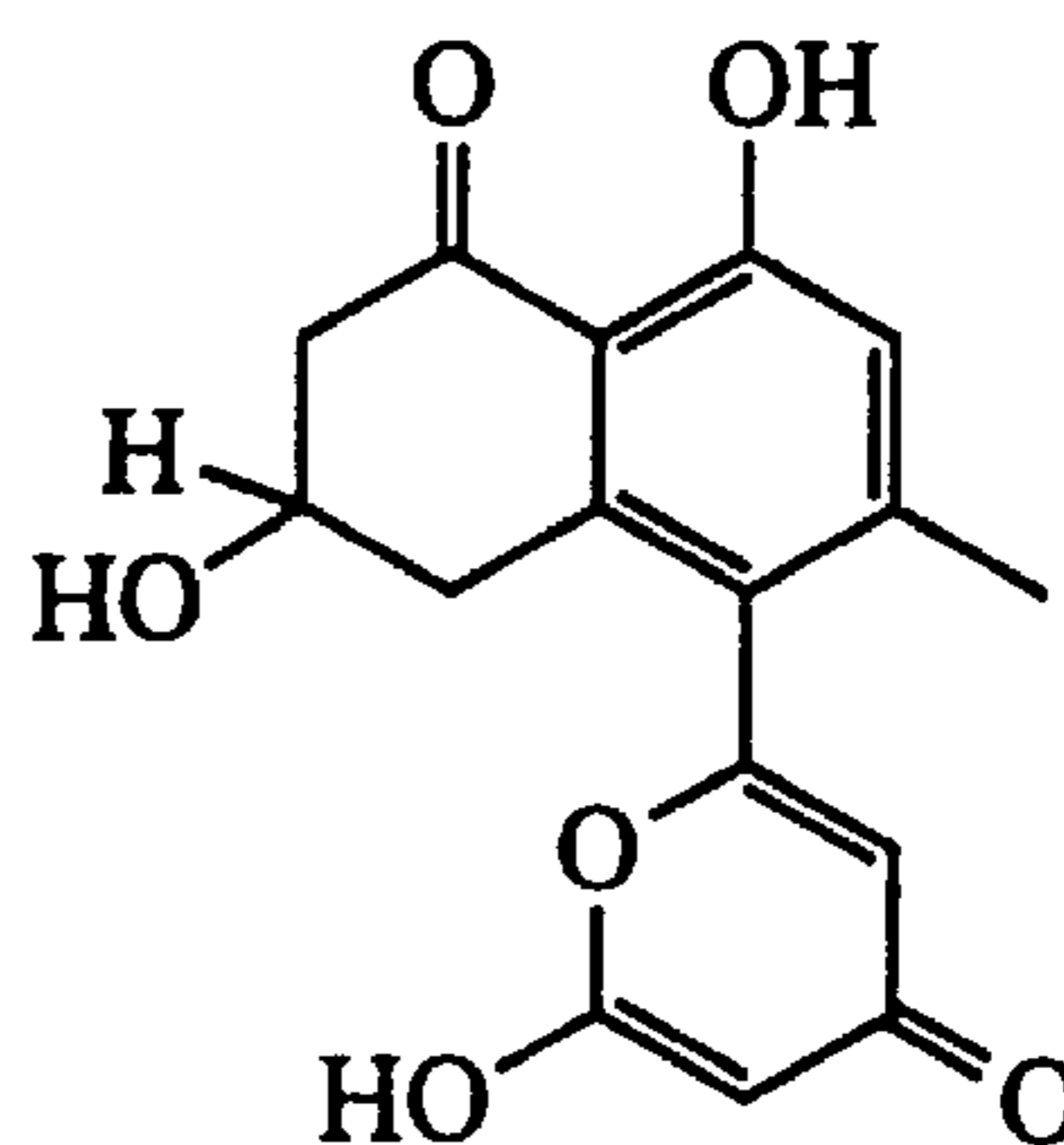
MUTACTIN (6)
