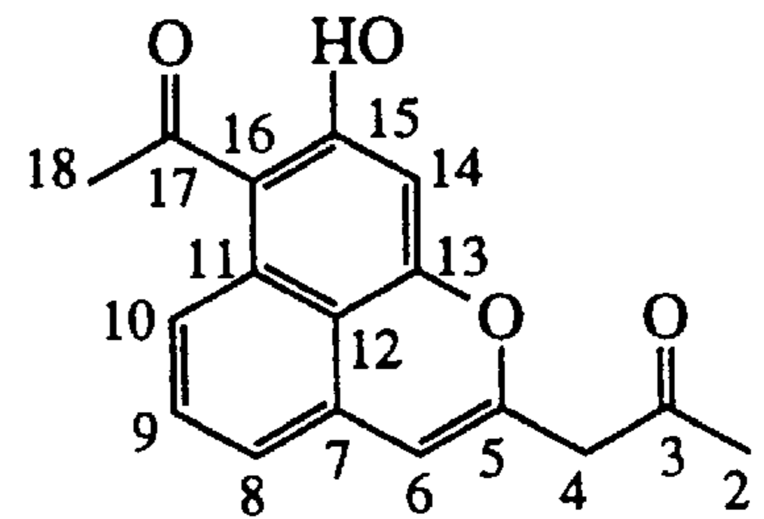
RM 18 (10)
