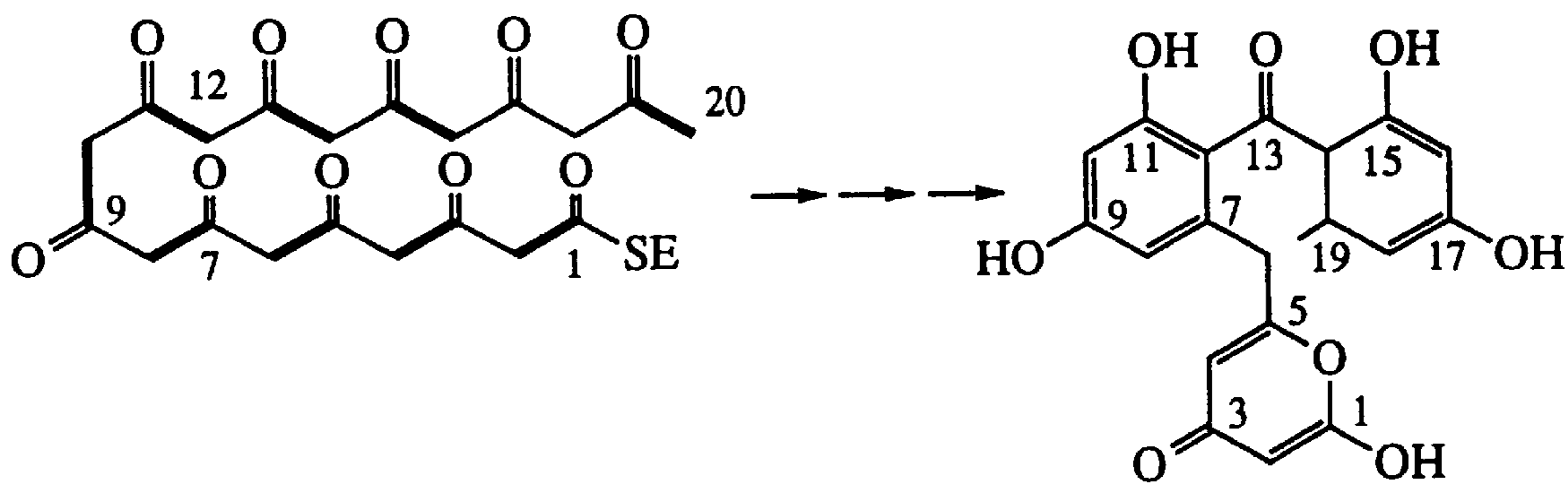
SEK15 (13)
