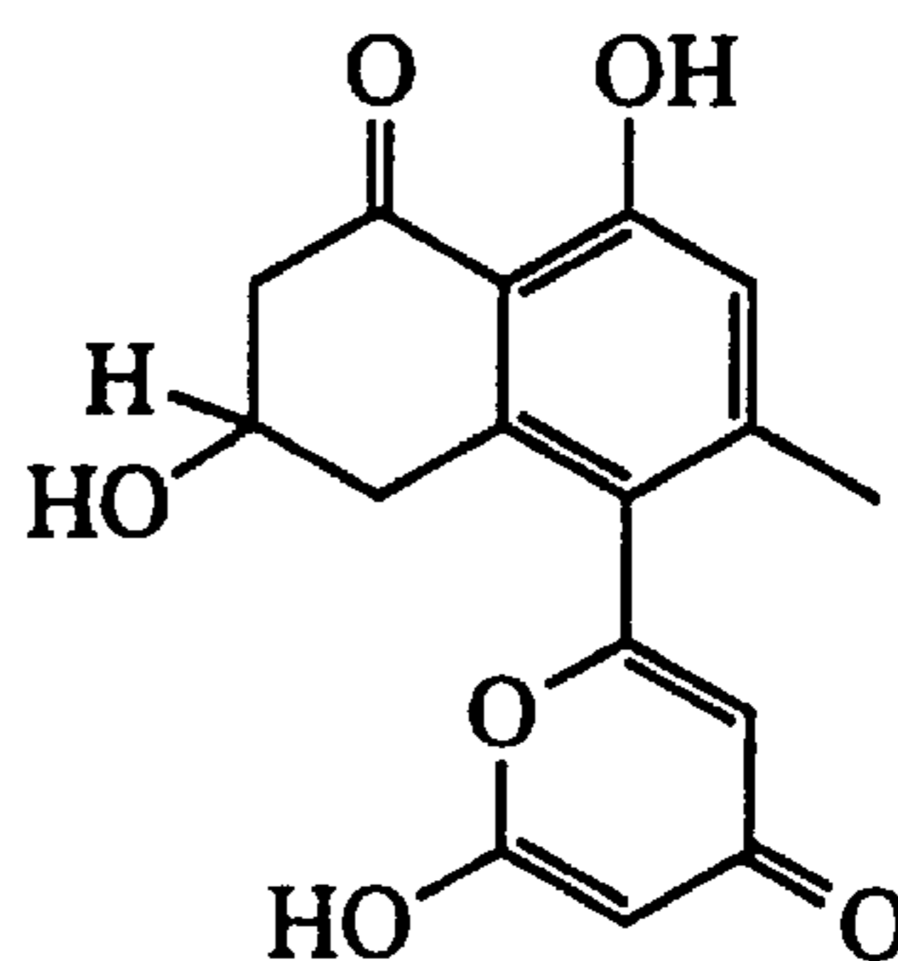
MUTACTIN (6)
