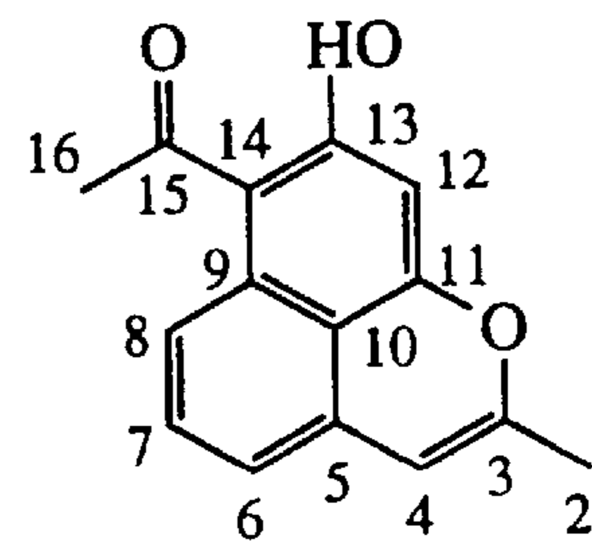
RM 18b (11)
