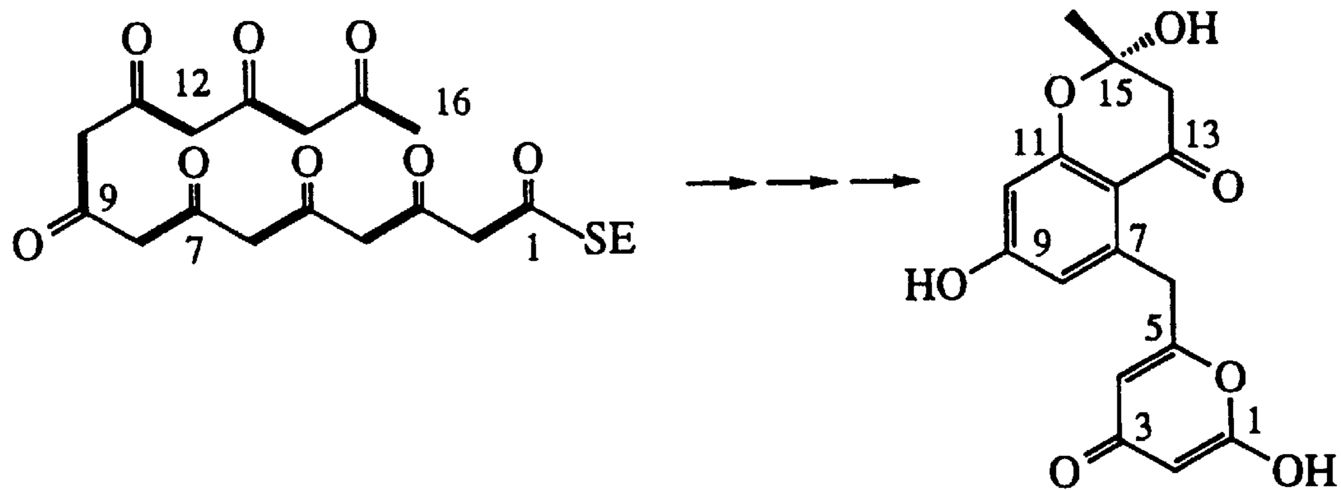
SEK4 (12)
