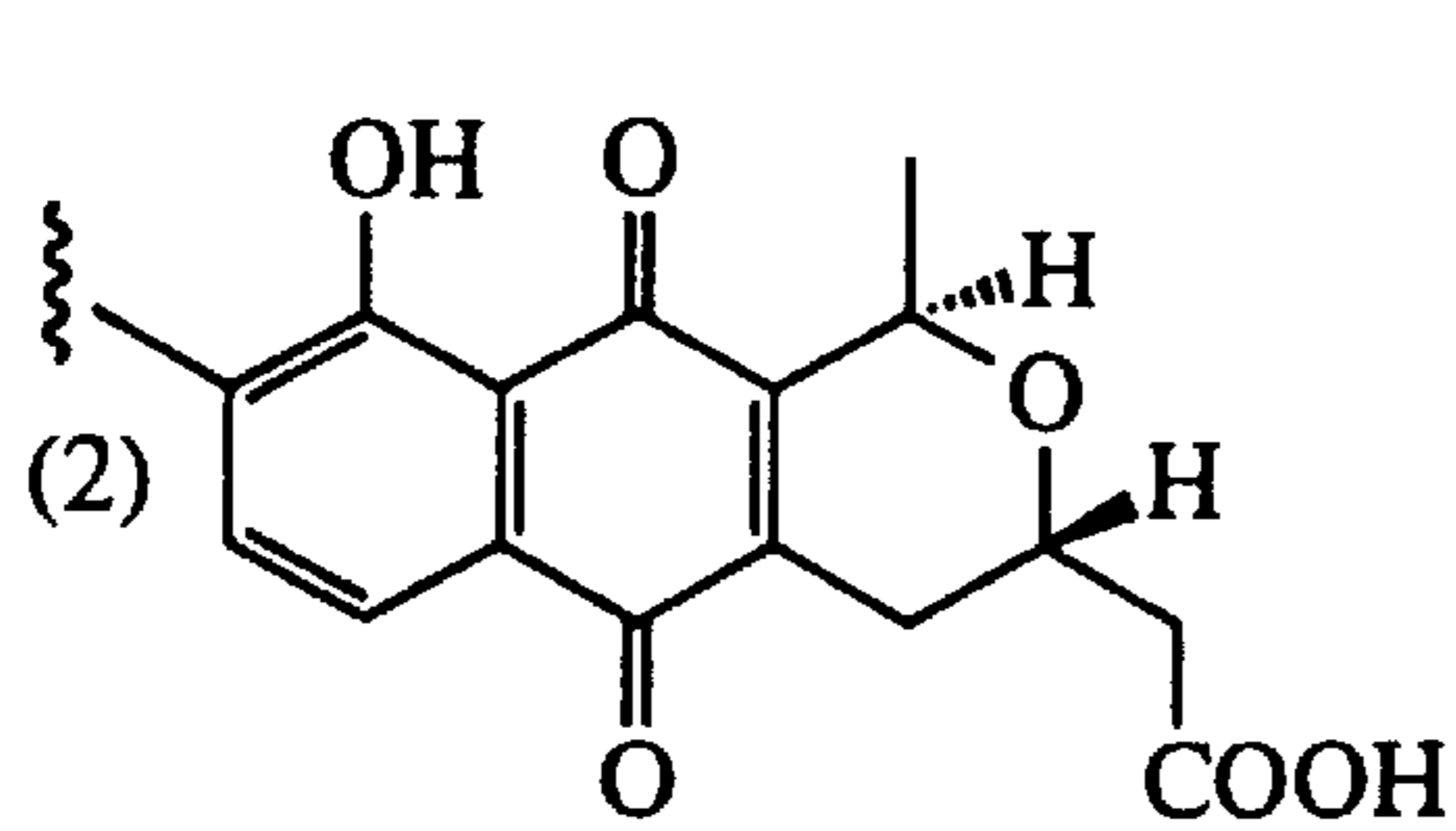
ACTINORHODIN (3)
