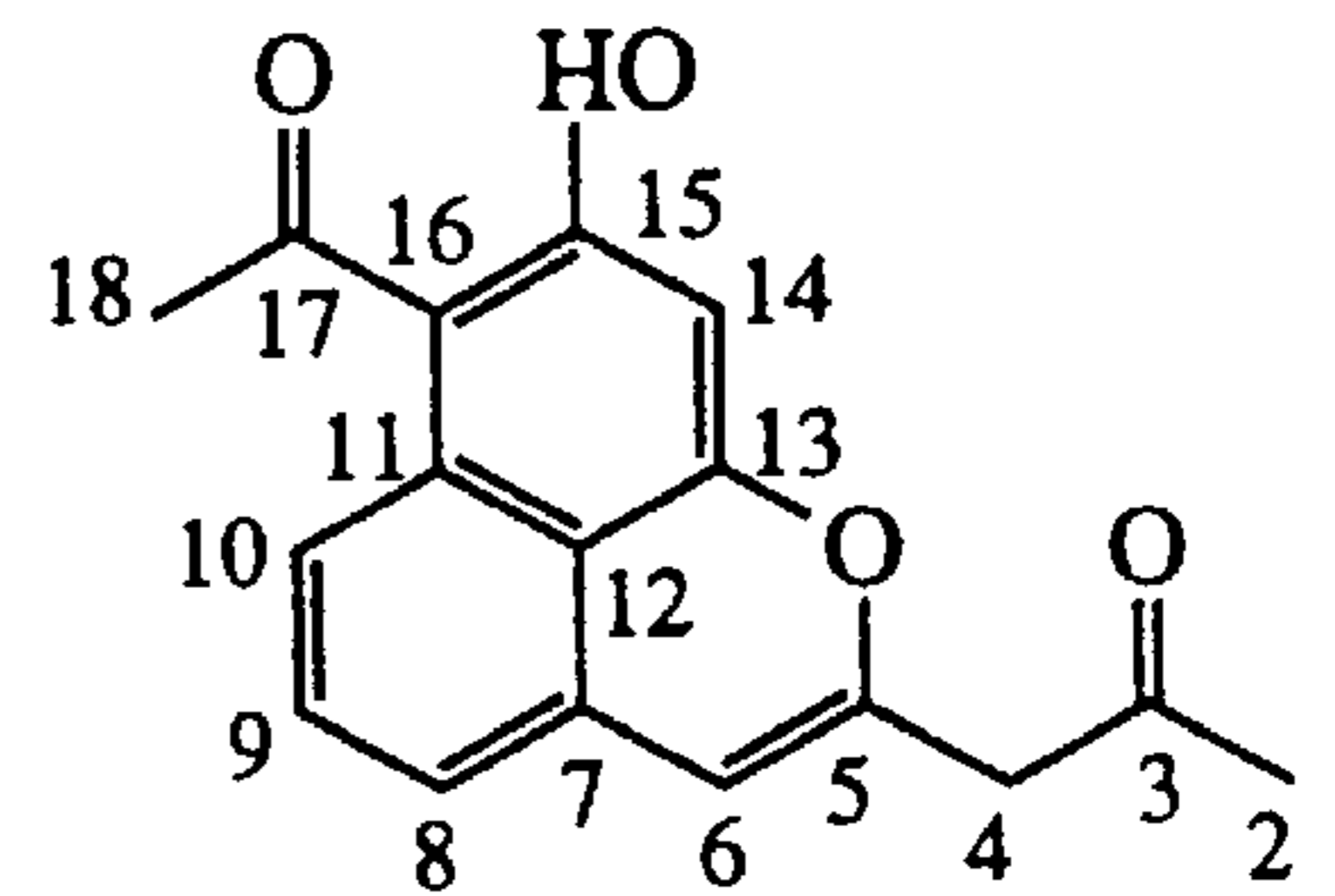
RM 18 (10)
