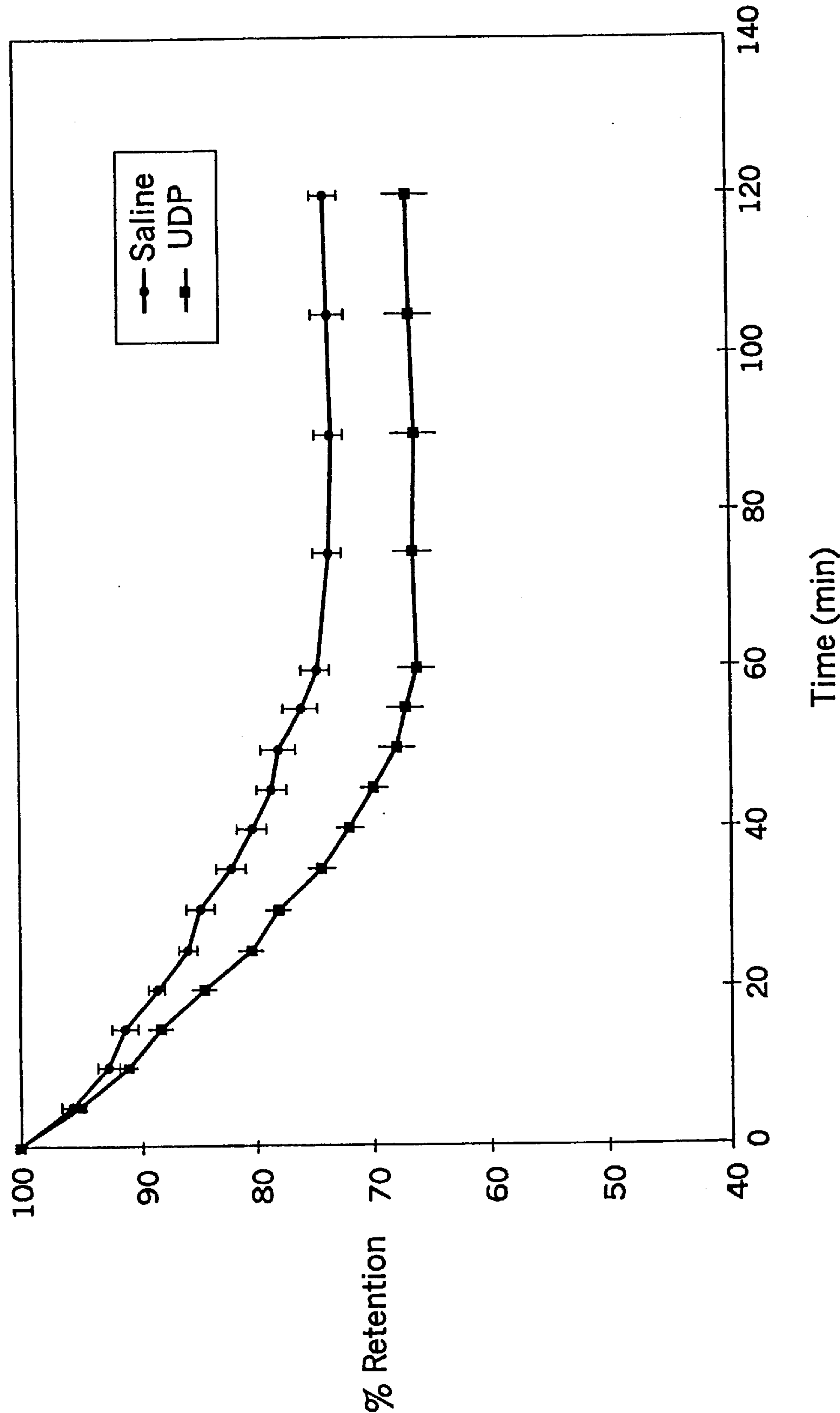
FIG. 6 Mucociliary Clearance in Sheep
