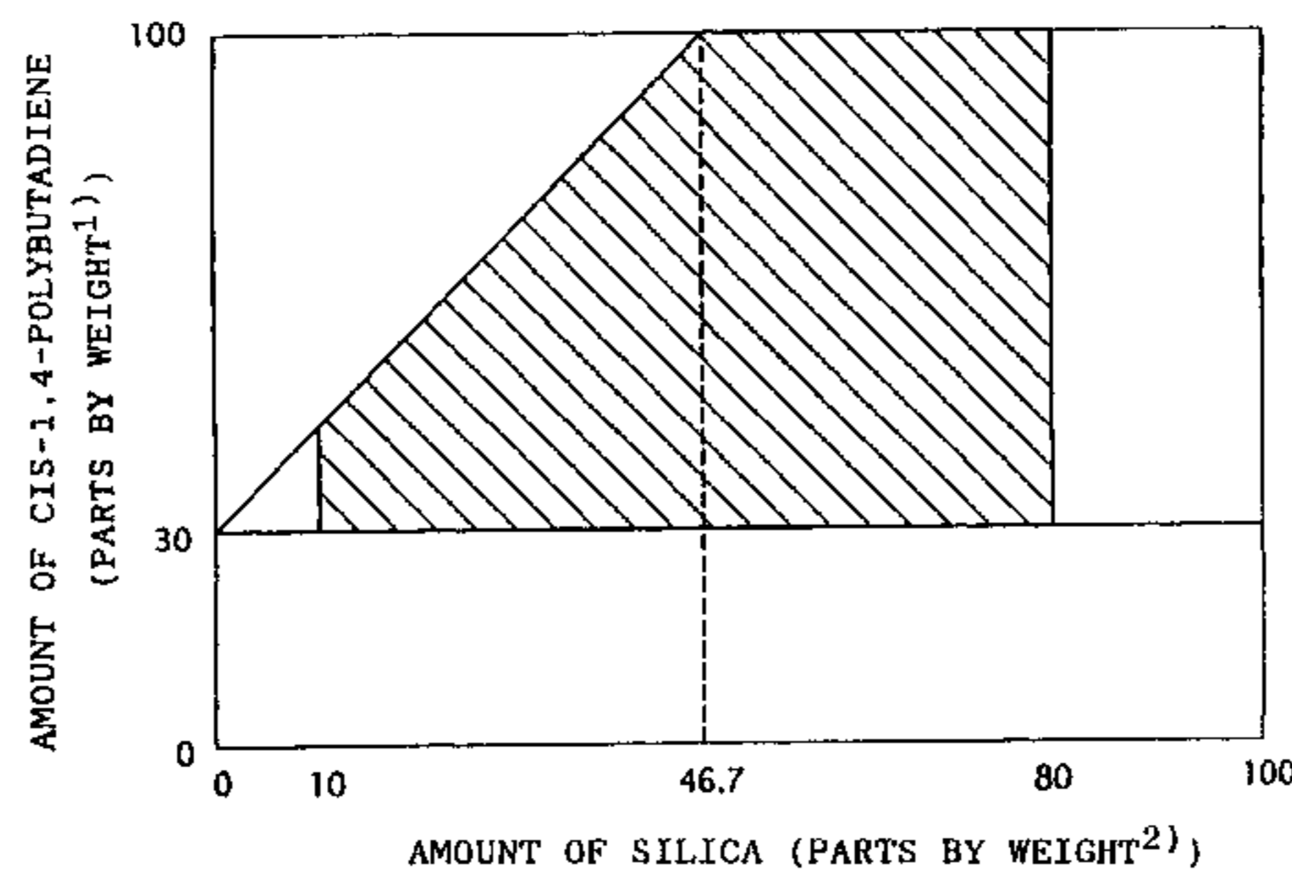
RELATIONSHIP BETWEEN AMOUNT OF CIS-1,4-POLYBUTADIENE AND AMOUNT OF SILICA
