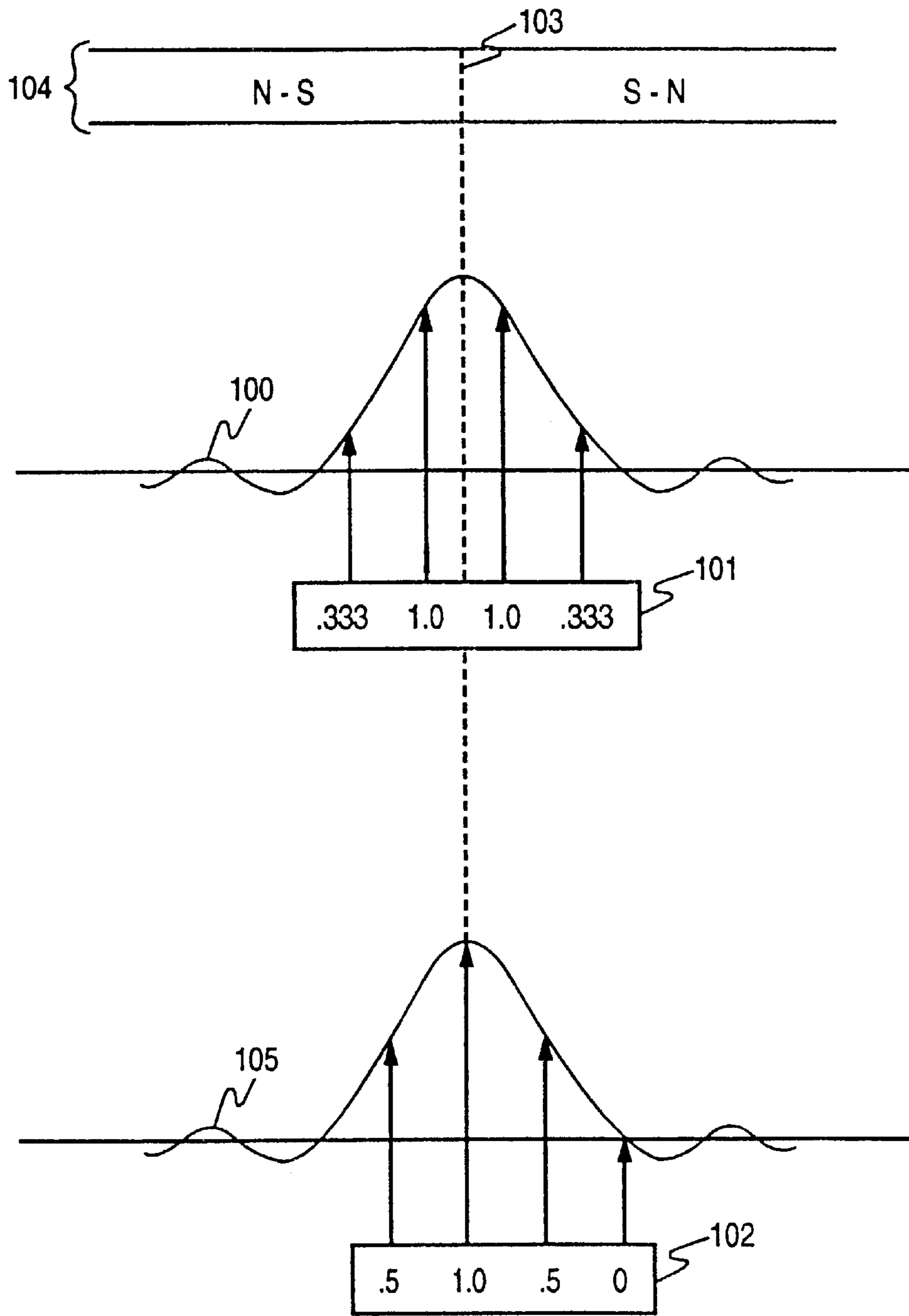
FIG. 1 (PRIOR ART)
