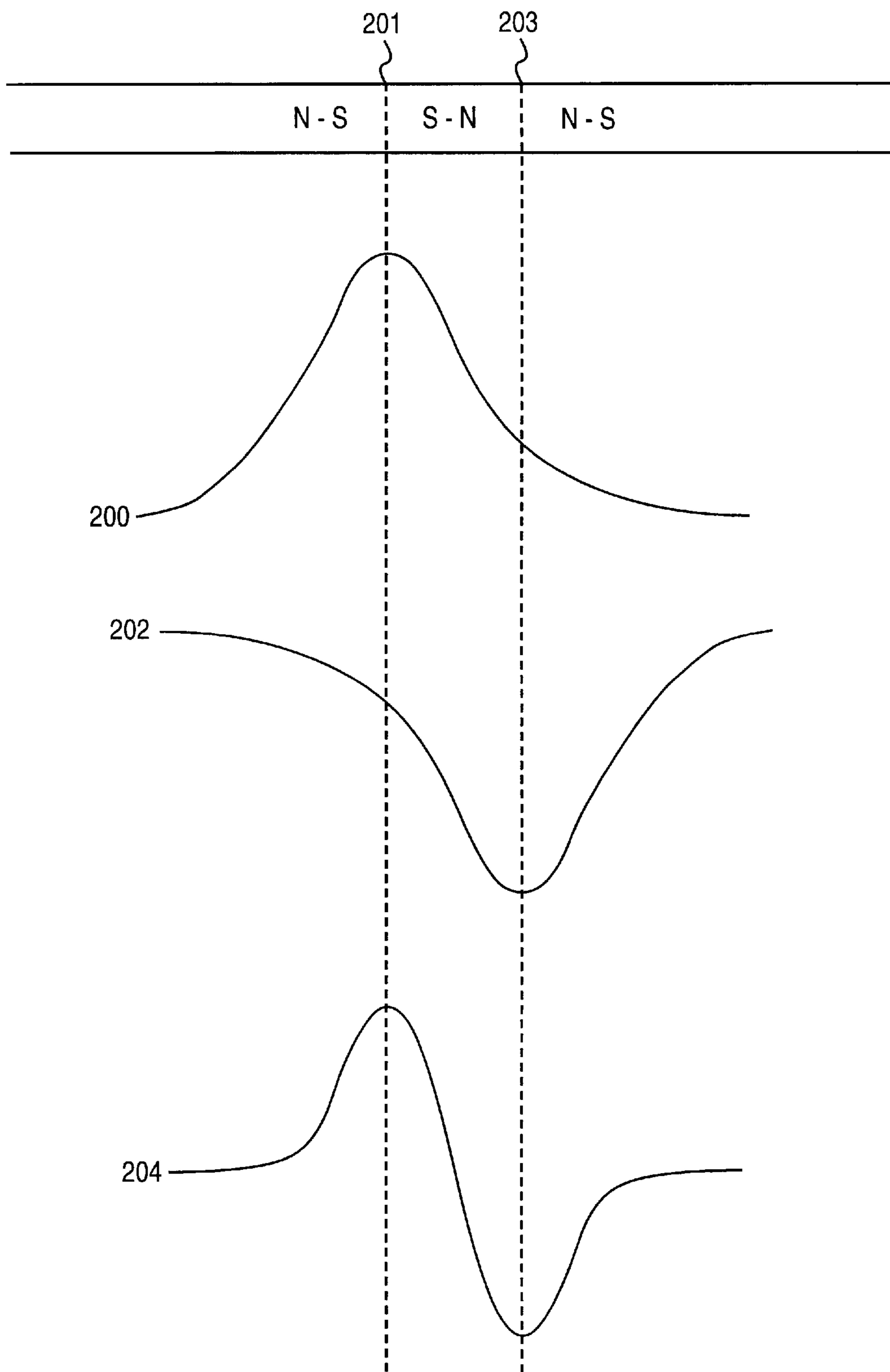
FIG. 2 (Prior Art)
