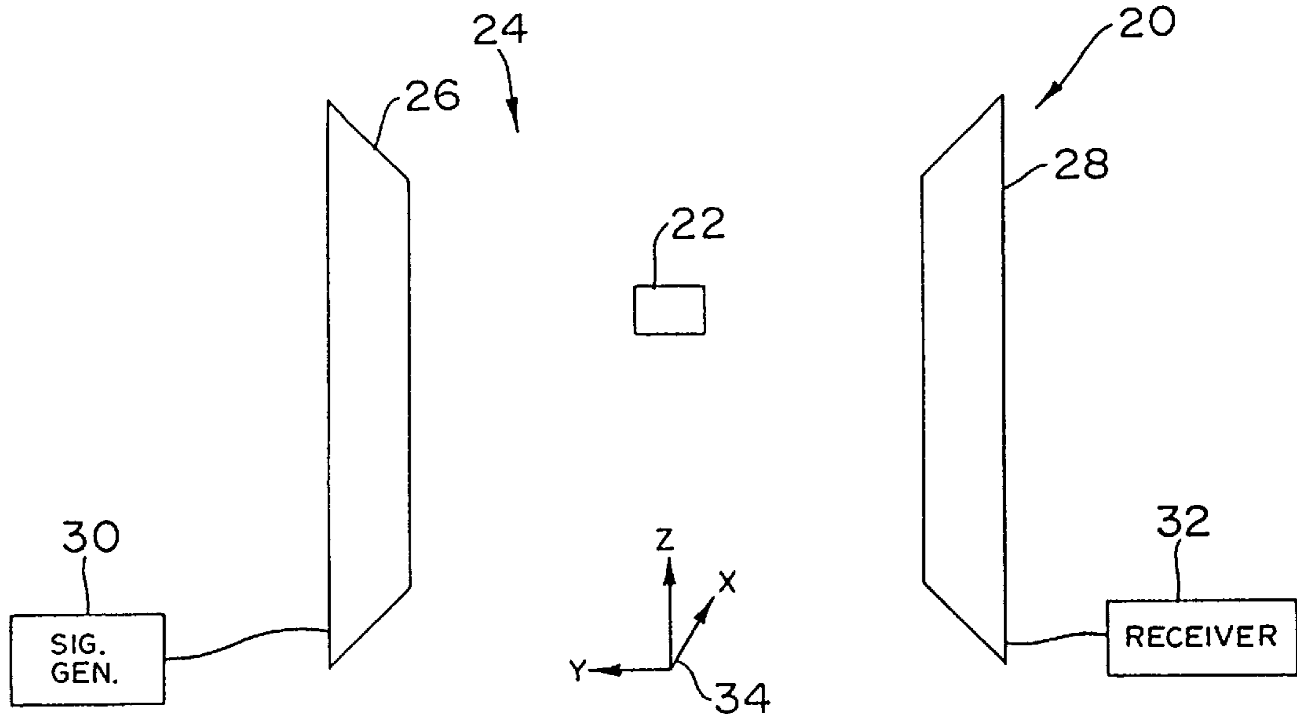
FIG. 1 (PRIOR ART)
