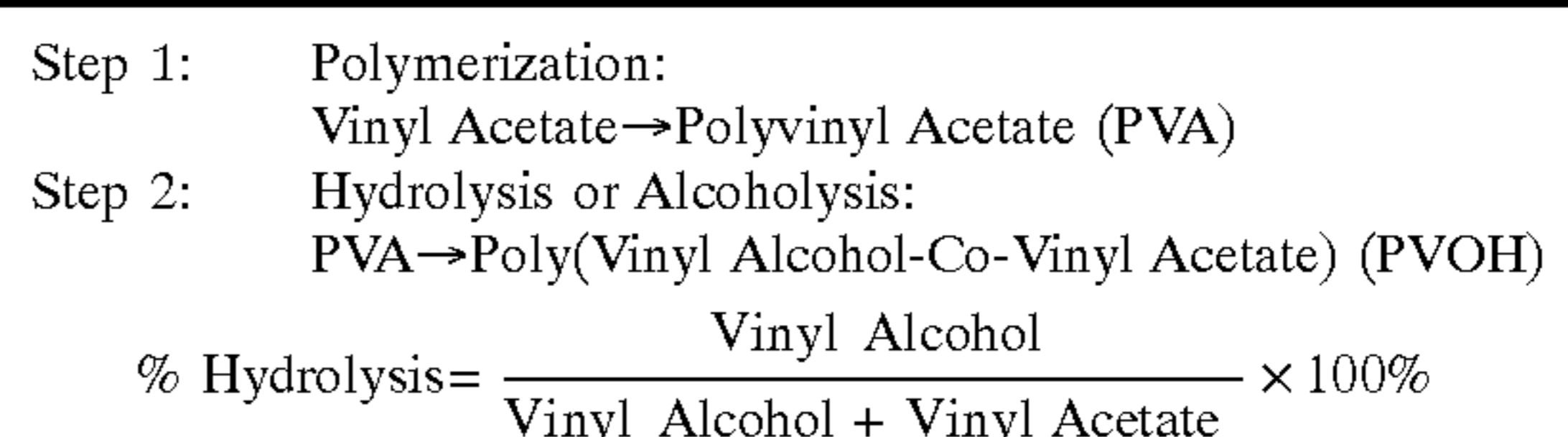
Scheme 1 Two-Step Process of Making PVOH
