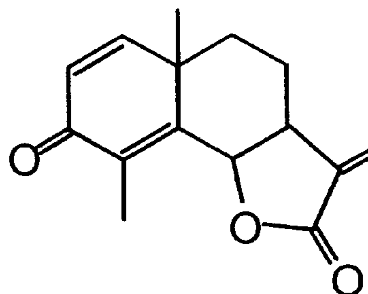
3-KETO-EUDISM-1(2), 4(5), 11(13)-TRIENE-6-12-OLID 18
