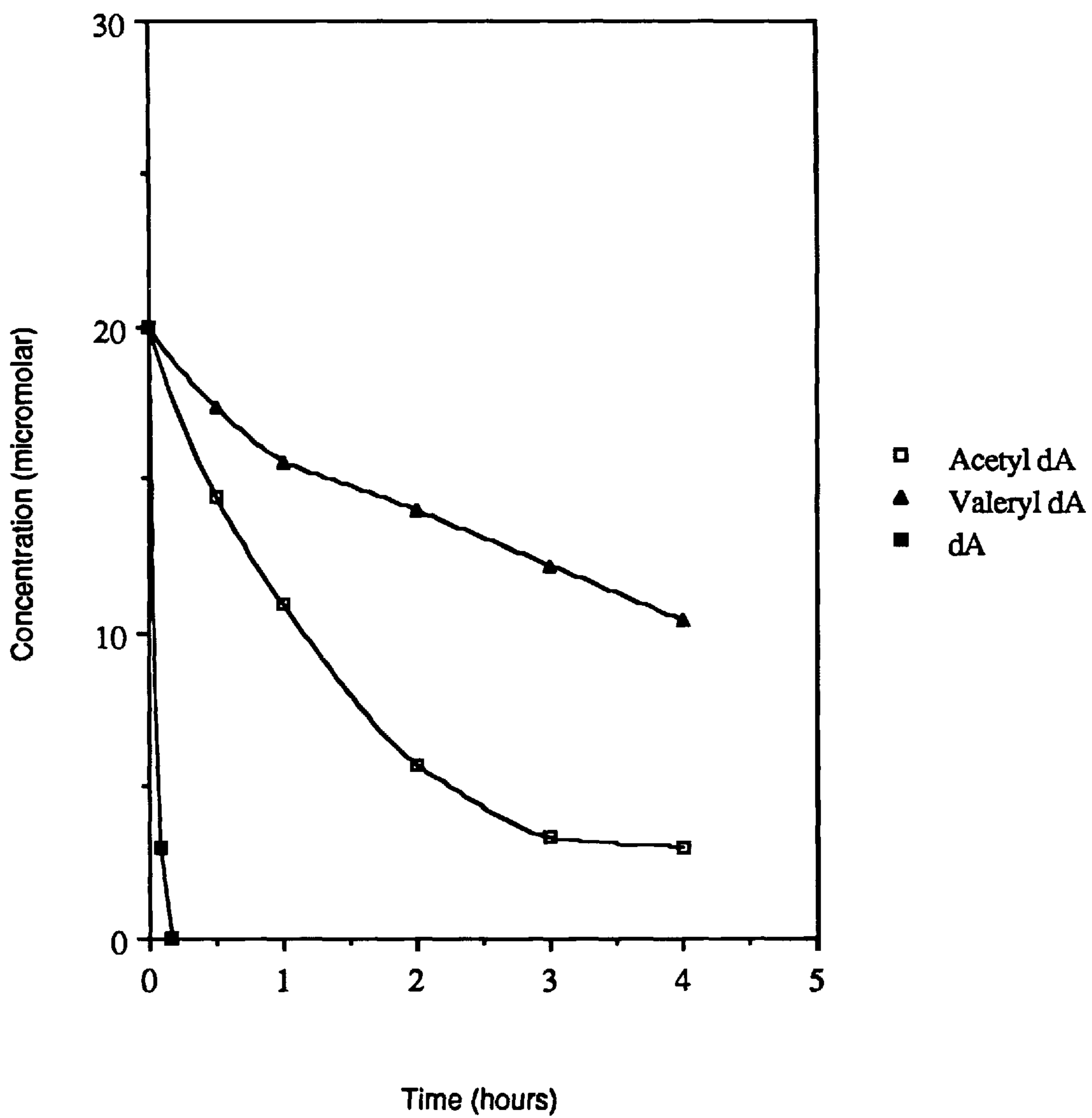
Fig.2: Disappearance of deoxyadenosine derivatives in plasma
