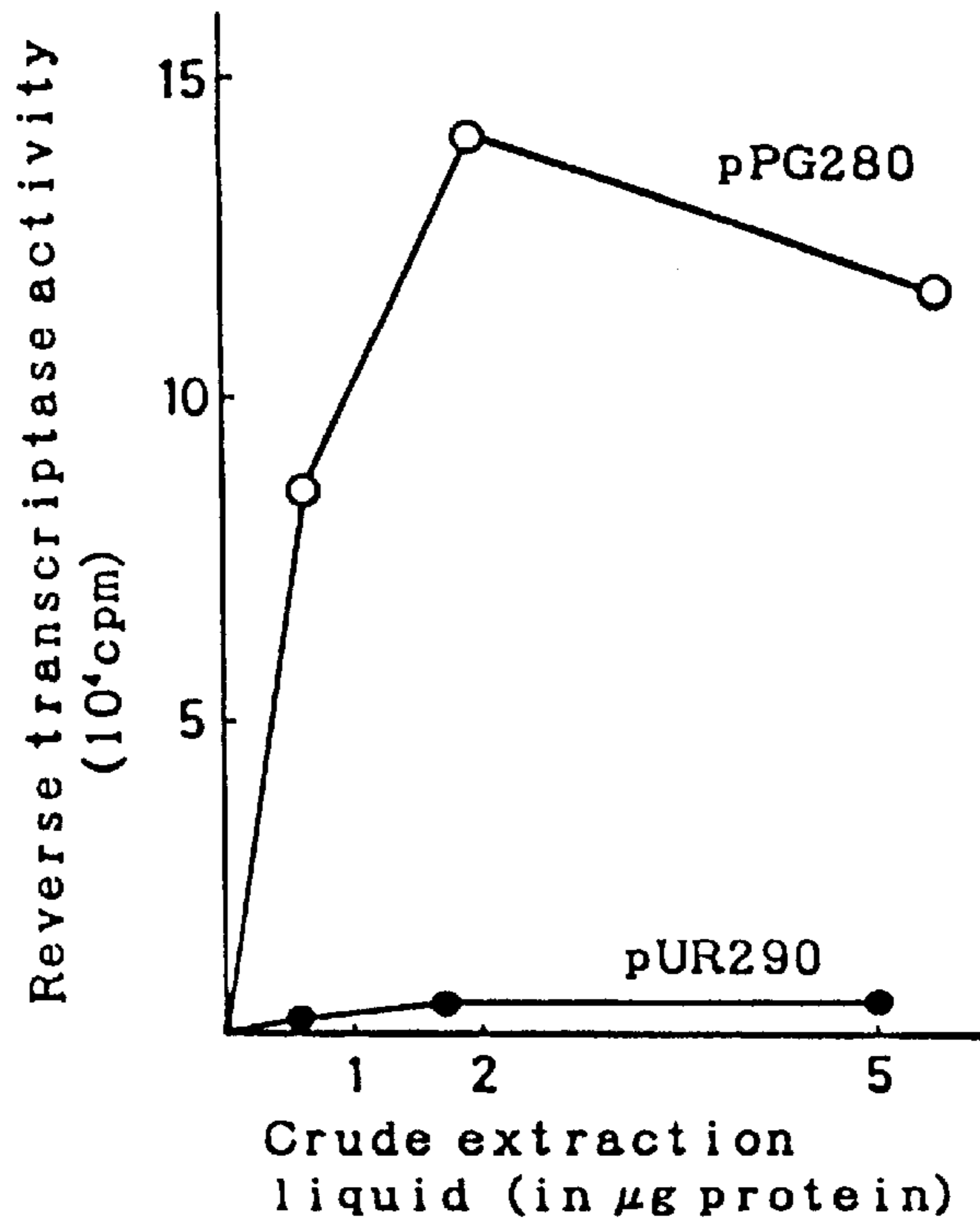
Reverse transcriptase activity of crude extraction liquid
