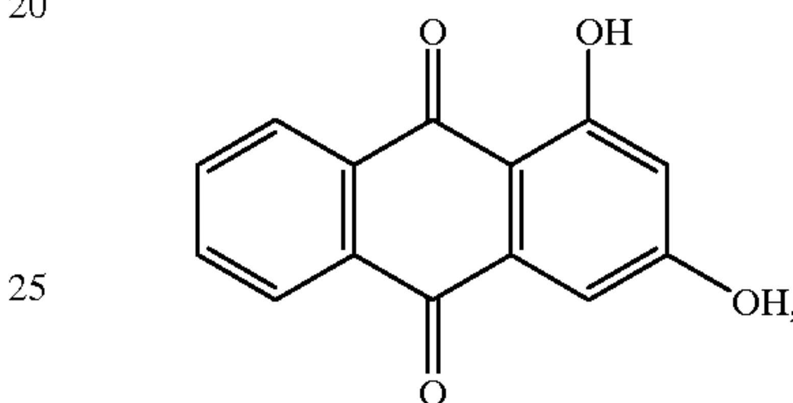
purpuroxanthin (1,3-dihydroxyanthraquinone) represented by the formula:
