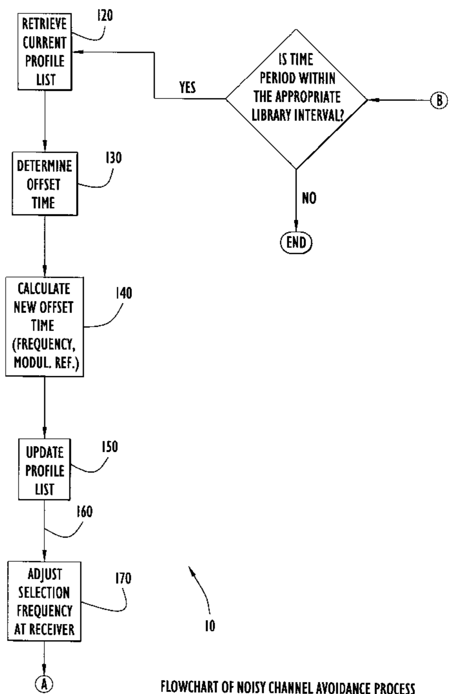
FLOWCHART OF NOISY CHANNEL AVOIDANCE PROCESS
