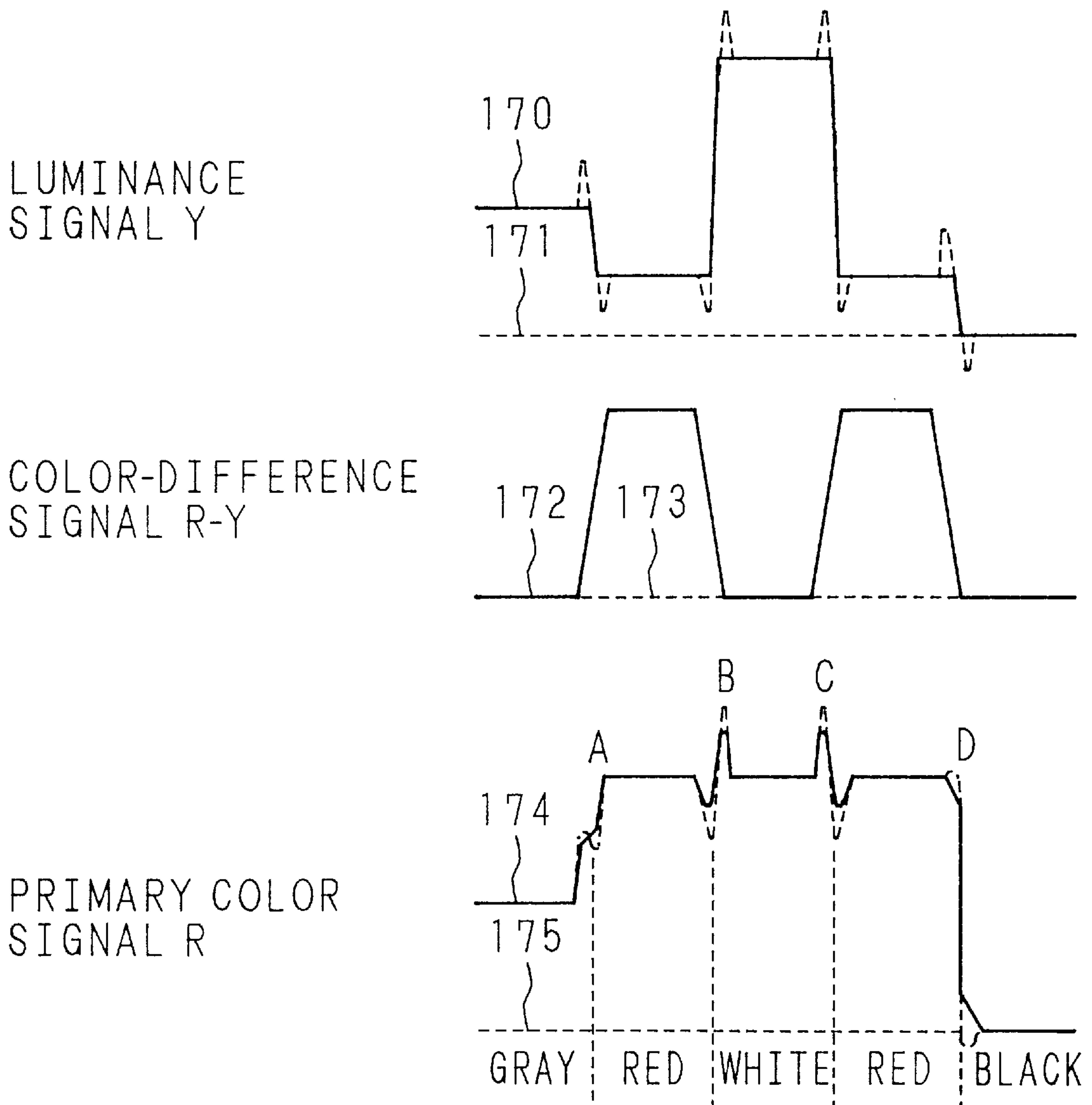
Fig. 2 Prior Art
